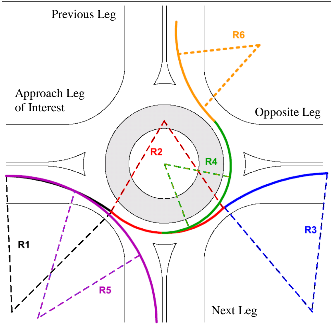
Figure 11. Trajectory radii
