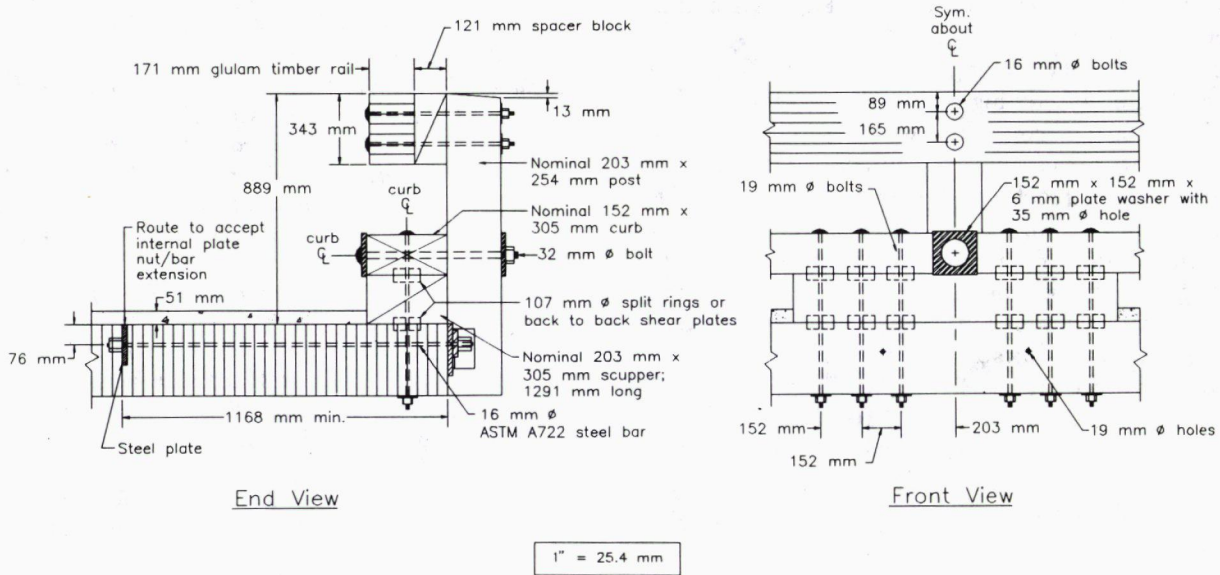
FIGURE 5 Glulam timber bridge railing successfully crash tested to NCHRP Report 350 TL-4 (photograph taken before testing).
