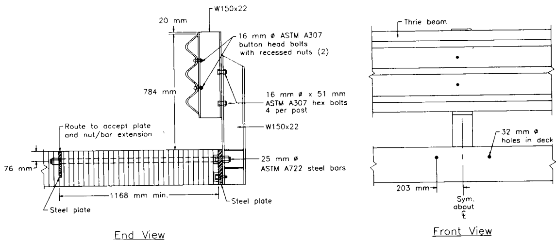
FIGURE 3 Drawings of bridge railings successfully crash tested to AASHTO PL-1: top, glulam timber rail with curb; middle, glulam timber rail without curb; bottom, steel rail.
