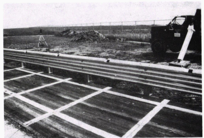
FIGURE 2 Bridge railings successfully crash tested to AASHTO PL-1 (photographs taken before testing).
