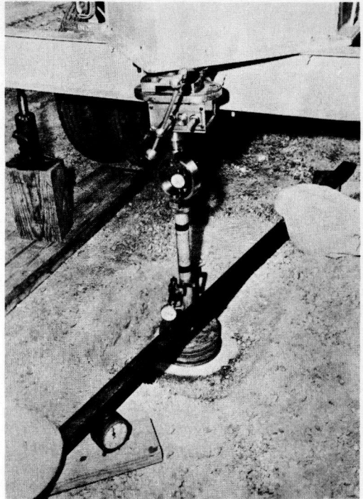
Figure 25. In-place CBR apparatus just prior to start of test.
