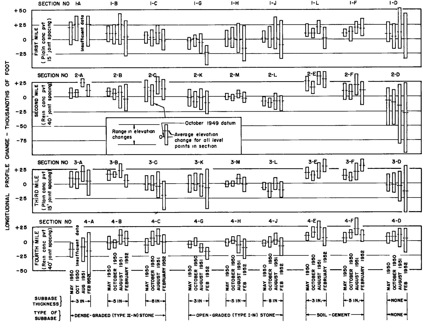
Figure 27. Longitudinal profile changes for each section at centerline of traffic (outer) lane.
