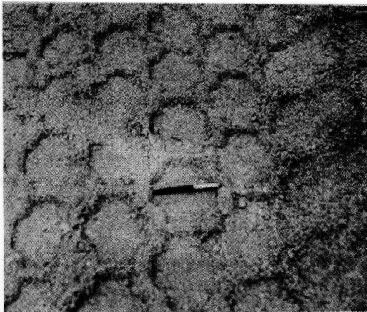
Figure 20. Condition of surface of open-graded stone subbase after rolling with a loaded earth scraper.
