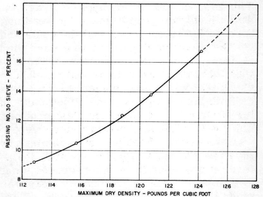
Figure 21. Relation between the percentage of the material passing the No. 30 sieve and the maximum dry density (laboratory compaction test) of the open-graded stone (type I-M). This chart was used in field compaction control.
