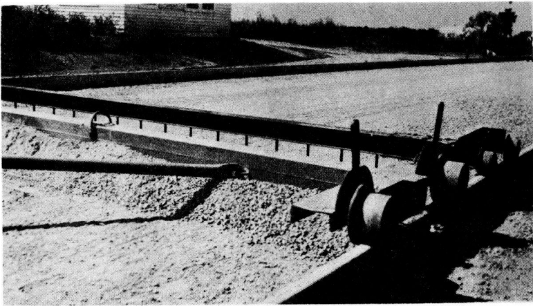
Figure 17. Segregation obtained during initial fine-grading of the open-graded stone subbase.
