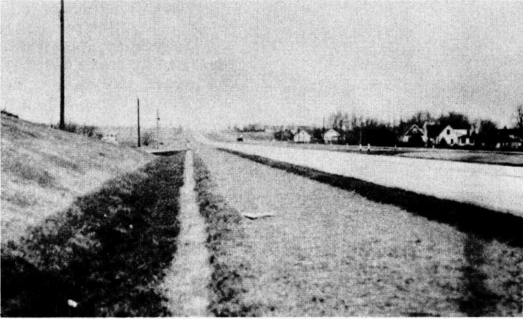
Figure 19. Completed open-graded stone section with subbase extending through shoulder.
