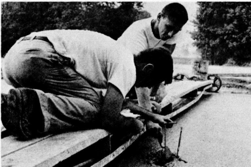
Figure 27. Taking slab temperature and steel depth measurements.
