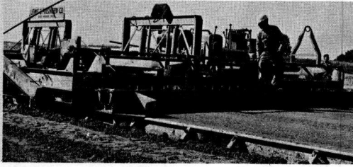
Figure 14. Final machine finishing with Heltzel Flexplane.
