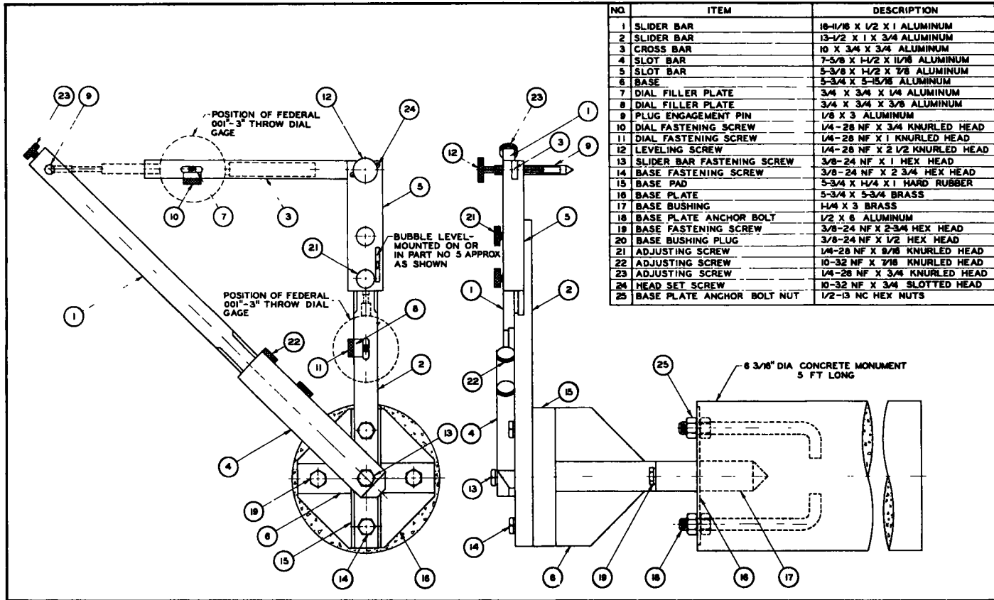
Figure 25. Assembly drawing of pavement displacemeter.
