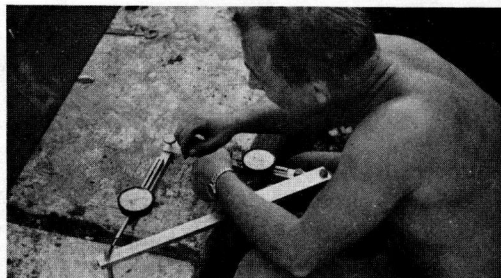
Figure 43. Measuring absolute slab displacement with pavement displacometer.
