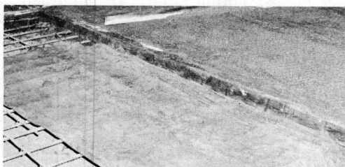
Figure 23. Burlap covering on extended bar mat reinforcement.
