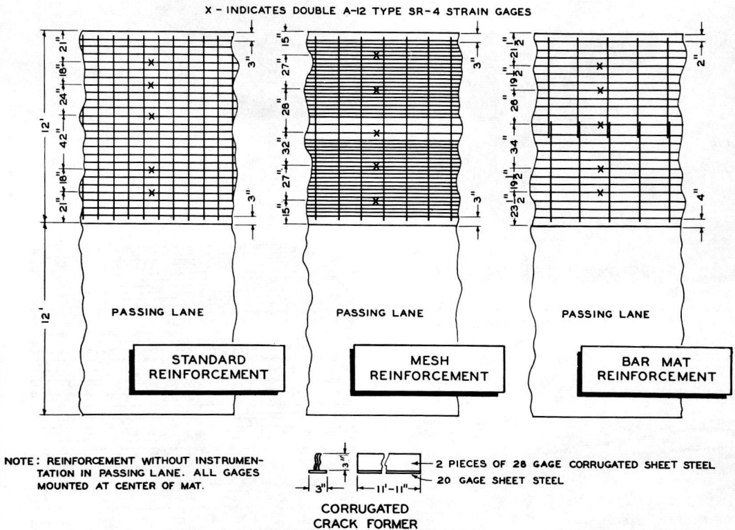
Figure 26. Details of strain gage placement and corrugated crack former.
