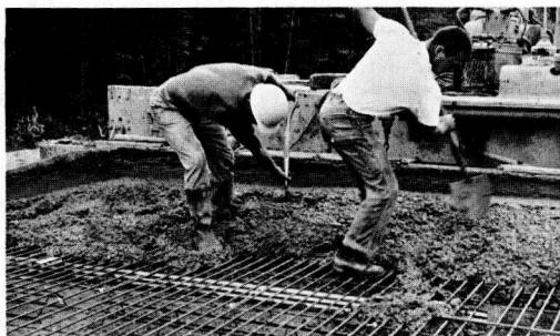
Figure 37. Placing concrete around corrugated crack former in heavy mesh reinforcement.
