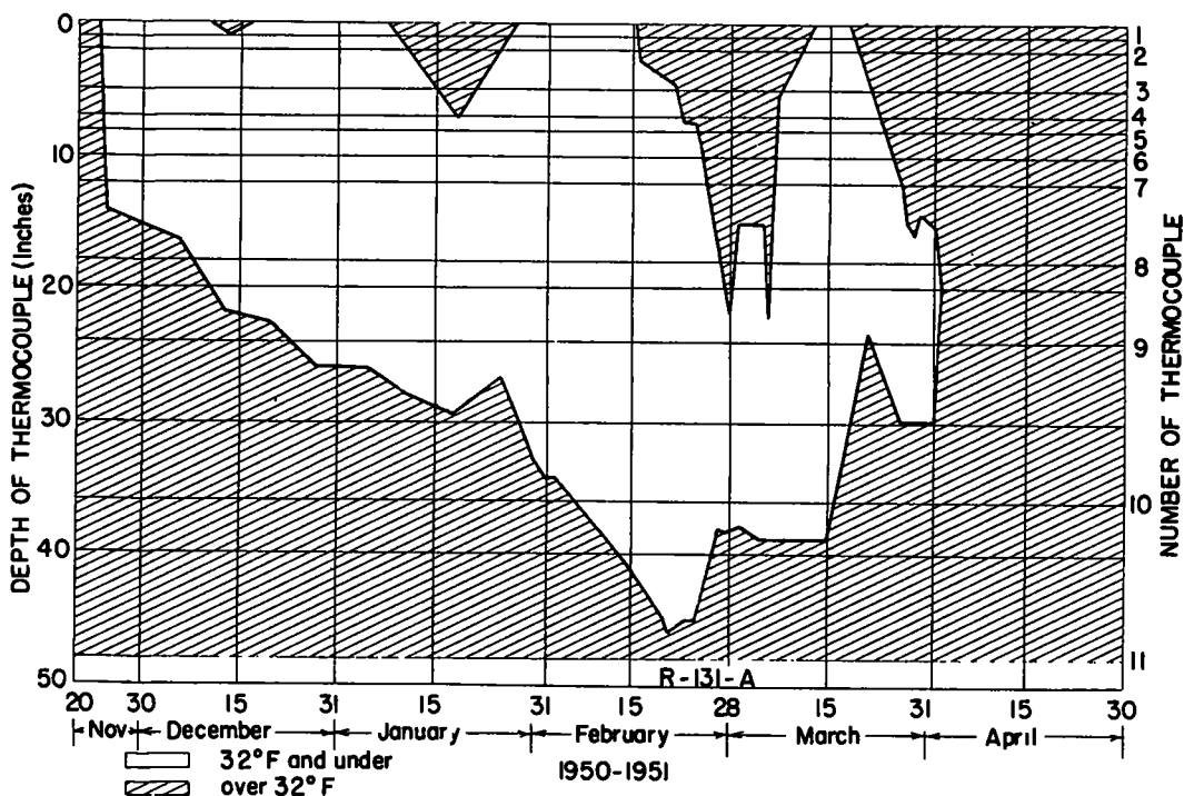
Figure 5. Temperature record (frost) as obtained by copper-constantan thermocouples and Brown Potentionmeter on Iowa, No. 144 2\frac{1}{2} mi. south of Grand Junction, 1950-1951.
