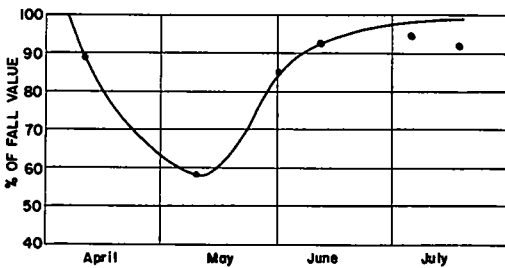
Figure 9. Test Point 3, 1948 construction; 2½-in. asphaltic concrete surface; 2-in. stabilized base; 5 in. pit-run base. Bearing tests with North Dakota cone device.
