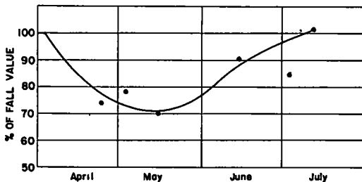
Figure 11. Test Point 5, 1948 resurface with 2½ in. of asphaltic concrete on 4-in. stabilized-gravel base with bituminous armor coat.
