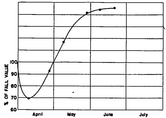
Figure 12. Test Point 6, 1947 construction: 2½ in. bituminous mat (cold laid), 5-in. stabilized base not closed to traffic during construction.
