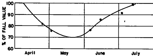
Figure 10. Test Point 4, 1948 construction; 2½-in. asphaltic-concrete surface, 2-in. stabilized base; 5 in. pit-run base. Bearing tests with North Dakota cone device.
