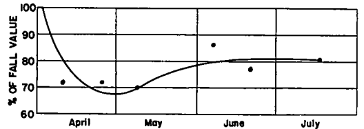
Figure 14. Test Point 8, 1947 construction: 2½-in. asphaltic concrete surface, 2-in. stabilized base, 5-in. pit-run base. Base and mat of original project about 1.3 ft. below current subgrade surface.
