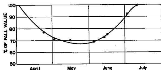
Figure 16. Test Point 10, 1948 construction: 2½-in. asphaltic-concrete surface, 2-in. stabilized base, 5-in. pit-run base.
