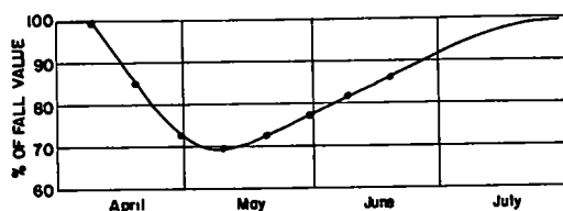
Figure 20. Average bearing for the 10 test points at the 24-in. depth below subgrade surface.
