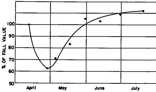
Figure 8. Test Point 2, original construction 1930; latest regravels 1947. Gravel surface bearing tests with North Dakota cone device.
