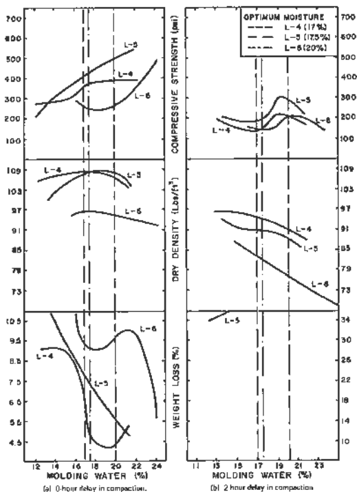
Figure 3. Effect of compaction moisture on silty clay foam soil-cement mixes at various detention times.
