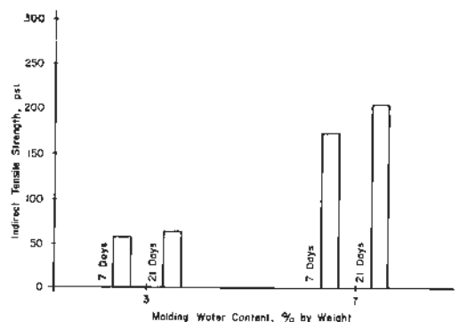
Figure 12. Effect of interaction between molding water content and curing time (interaction A x B).
