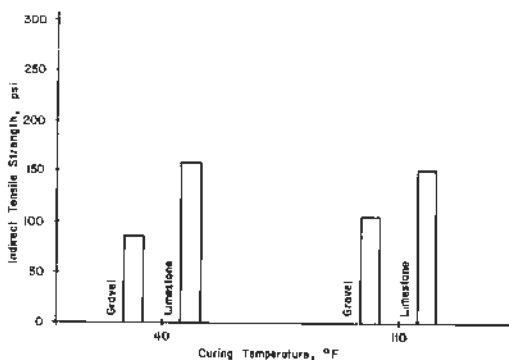
Figure 11. Effect of interaction between aggregate type and curing temperature (interaction E x F).
