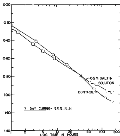
Figure 7. Shrinkage versus time for Na-montmorillonitic soil-cement with 0.5 percent salt added in solution form and cured under 90 percent relative humidity for 7 days.
