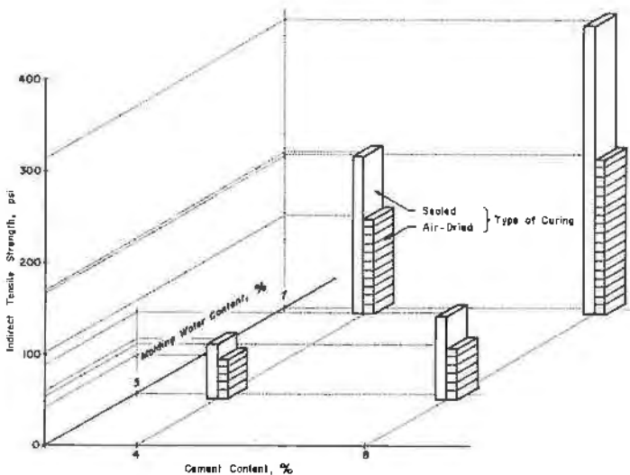
Figure 2. Effect of interaction among molding water content, type of curing, and cement content (interaction A x D x J).
