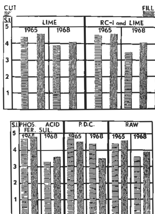
Figure 35. Serviceability index, all treated materials.
