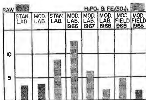
Figure 33. CBR, PDC formula stabilization.
