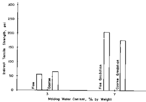
Figure 9. Effect of interaction between molding water content and aggregate gradation (interaction A x C).
