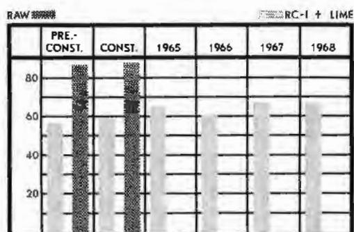
Figure 11. Liquid limit, lime-asphalt stabilization.
