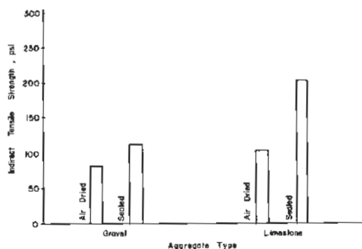
Figure 5. Effect of interaction between type of curing and aggregate type (interaction D \times E).
