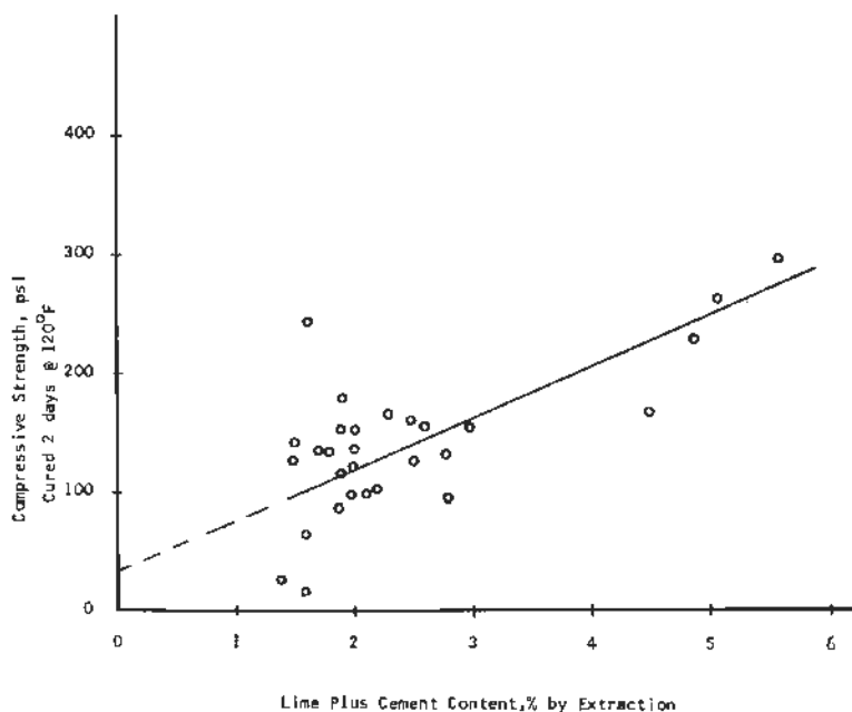
Figure 7. Correlation between lime plus cement content and compressive strength of field samples.
