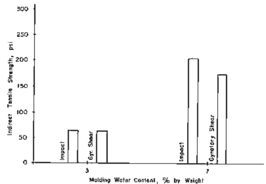
Figure 10. Effect of interaction between molding water content and type of compaction (interaction A x H).
