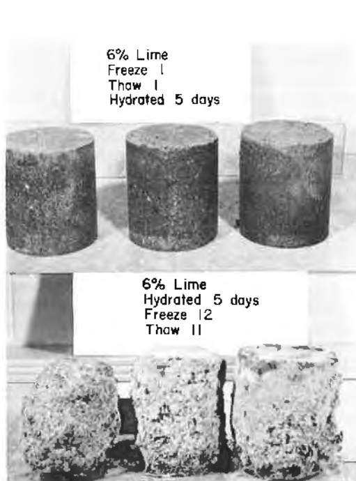
Figure 6. Samples after air thaw.
