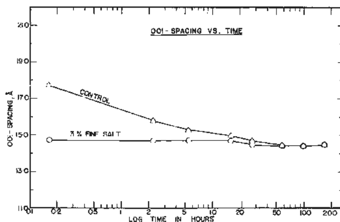
Figure 11. Basal (001) lattice spacing of Na-montmorillonite versus curing time in soil-cement specimens.
