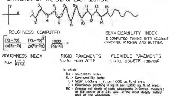
Figure 29. Formulas for determining SI.
