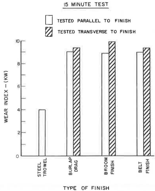
Figure 1. Influence of concrete finish on skid resistance.
