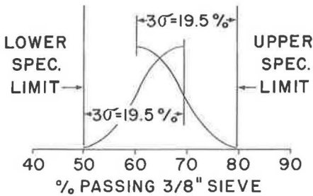
Figure 4. Location of the mean of the 3/8-in. material produced as it relates to specification limits.
