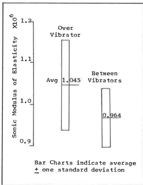
Figure 26. Sonic modulus of elasticity on cores from the fine-aggregate mix on project 1805.
