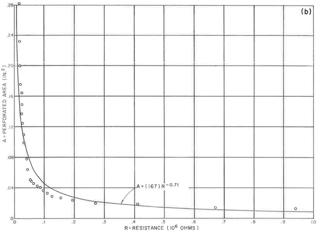
Figure 6. Area of perforations versus ohms resistance with epoxy coating.
