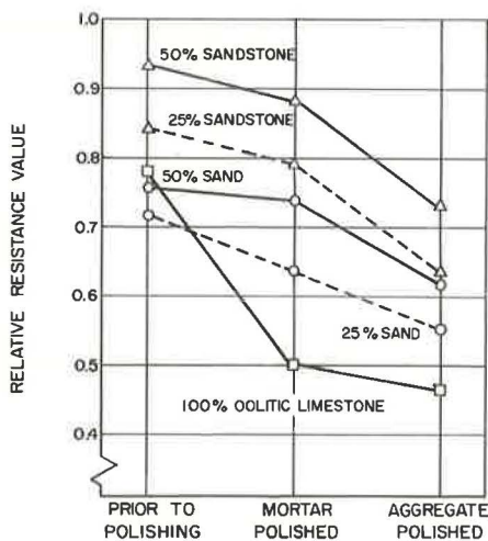
Figure 4. Fine aggregate replacement in portland cement concrete.
