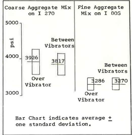
Figure 20. Comparison of compressive strength as indicated by Swiss hammer.
