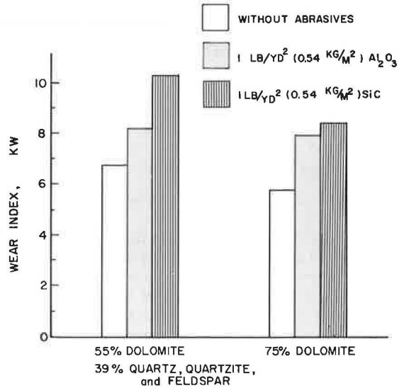
Figure 2. Use of abrasives to develop superior friction surfaces.
