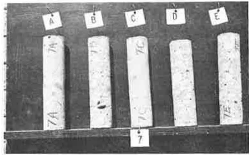
Figure 16. Cores from section 7 on project 1270 where coarse-aggregate mix was used (cores A and C were taken over path of vibrator, and cores B, D, and E were taken between paths of 1 5 / 8 -in. diameter eccentric vibrator).
