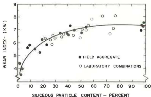
Figure 3. Effect of siliceous particle content on wear index.
