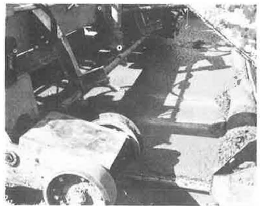
Figure 7. Internal vibrator mounted on paver and "wake" developed as vibrator passes through 1½-in. slump concrete.
