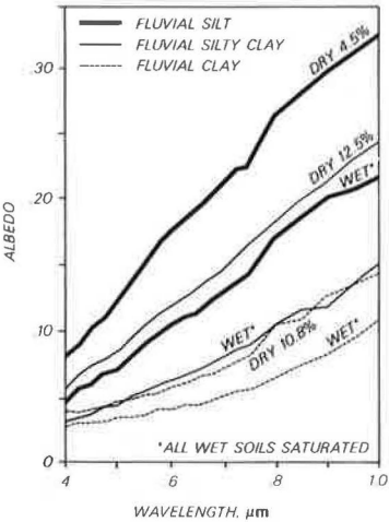
Figure 1. Representative reflectance readings for alluvial soils.
