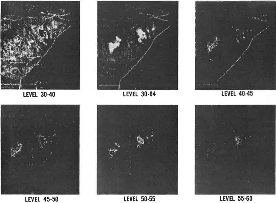
Figure 5. Computer-generated gray scale slices of a coal refuse pile fire in Pennsylvania (slicing is illustrated at discrete voltage levels that can be converted to radiation temperatures).
