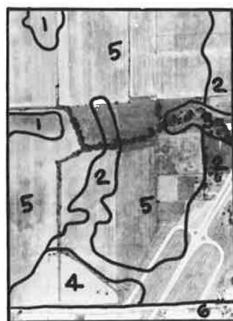
Figure 6. Soil map.
