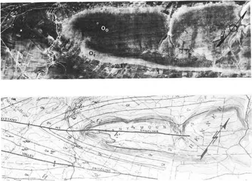
Figure 2. Comparison of thermal image and geological map of Nittany Mountain, October 21, 1959, 5,000 ft m.s.l., 9:30 p.m., InSb detector ( O_r = Reedsville shale, and O_o = Oswego sandstone).
