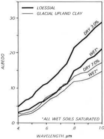
Figure 2. Representative reflectance readings for upland soils.
