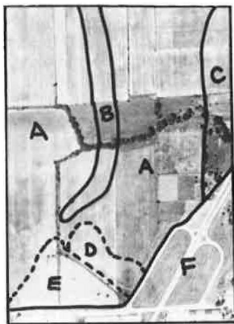
Figure 5. Landform map.
