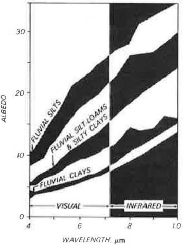
Figure 3. Variation of reflectance of major alluvial soils.
