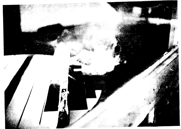
FIGURE 10 Plate No. 4: General view of model wall showing pollutant entrainment cavity. Note: Flow is left to right at approximately 45 degrees with respect to wall. Pollutant entrainment cavity can be seen as a white cloud near center of photograph and just downwind of wall. Random motion, vortices, aerodynamic eddies, and flow reversal are indicated by the wisps of smoke in cavity. Above and downwind of cavity, smoke (seen as less dense than in cavity) is moving uniformly.
