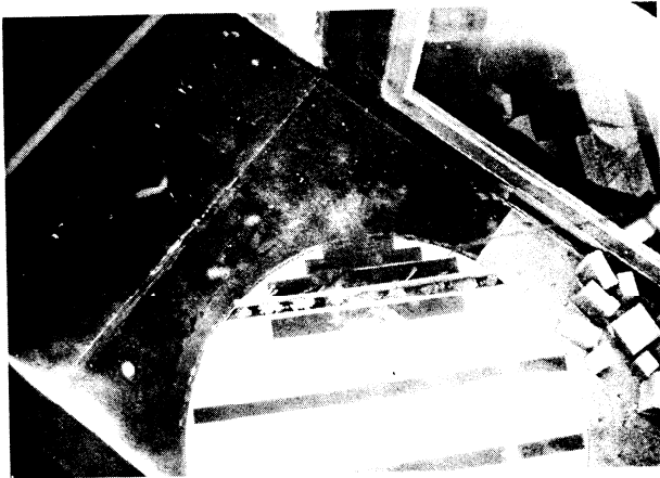
FIGURE 8 Plate No. 2: View of model wall and turntable from top viewing window. Note: Flow is from lower right corner to upper left corner and is approximately 45 degrees with respect to wall. Blocks in lower right corner are part of model city. A side viewing window can be seen in the upper right.
