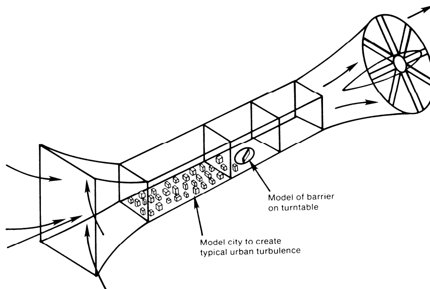
FIGURE 3 Schematic of wind tunnel and model for experiments.
