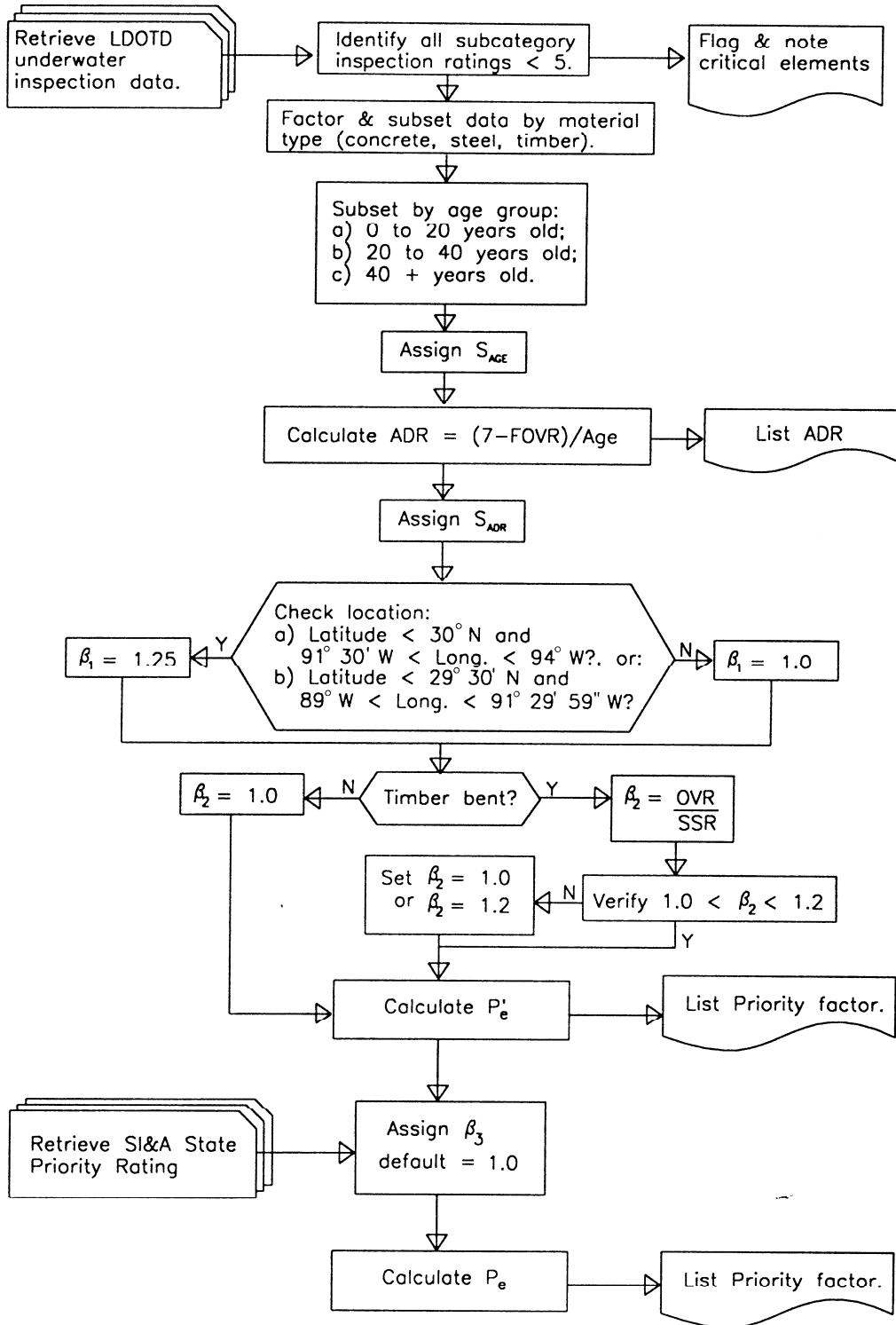
FIGURE 1 Decision flow process for establishing underwater bridge inspection priorities.
