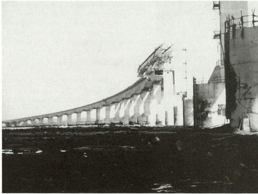
Figure 16. The concrete viaducts of the Second Severn Crossing Bridge.
