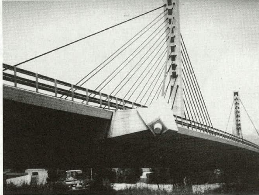
Figure 12. The Chandoline Bridge at Sion.
