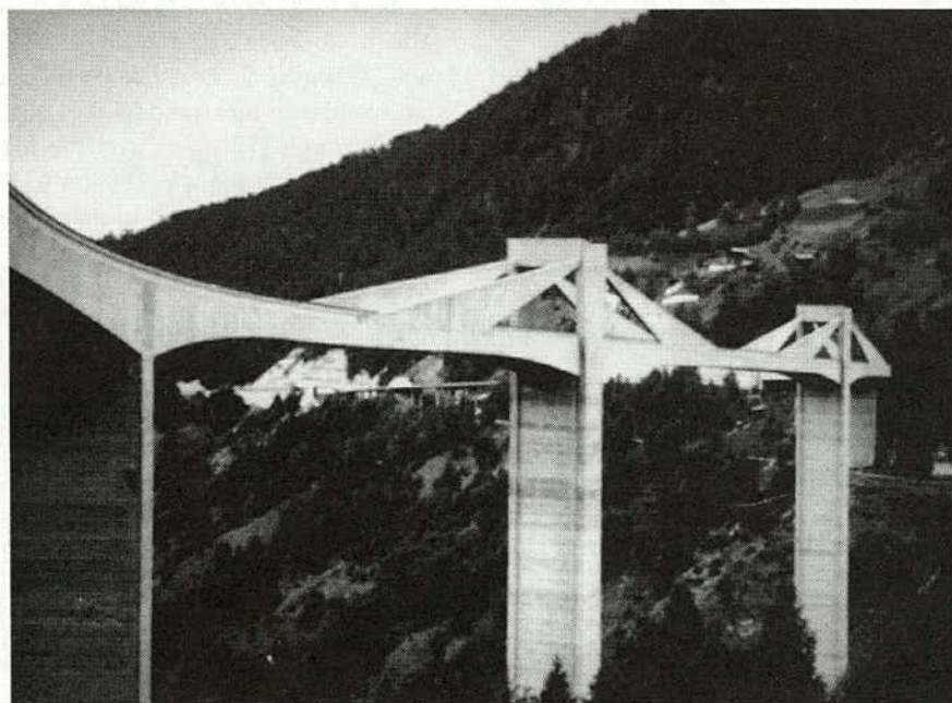
Figure 13. The Ganter Bridge at Simplon Pass.
