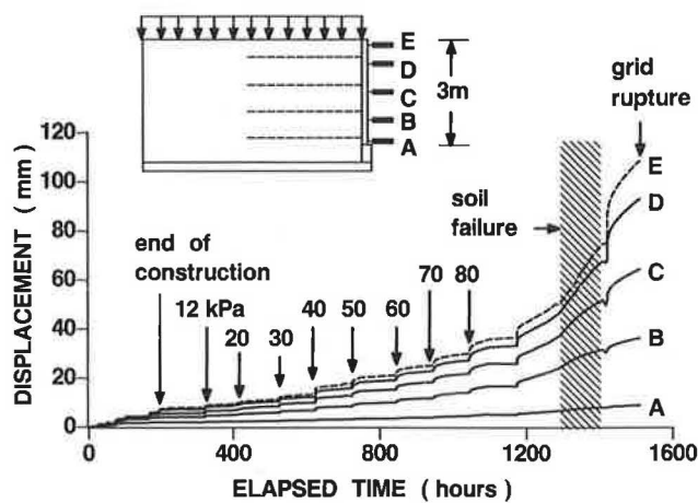
FIGURE 7 Panel displacements.
