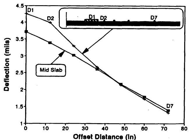
FIGURE 6 Effect of cracks/joints on surface deflection (Configuration 1).
