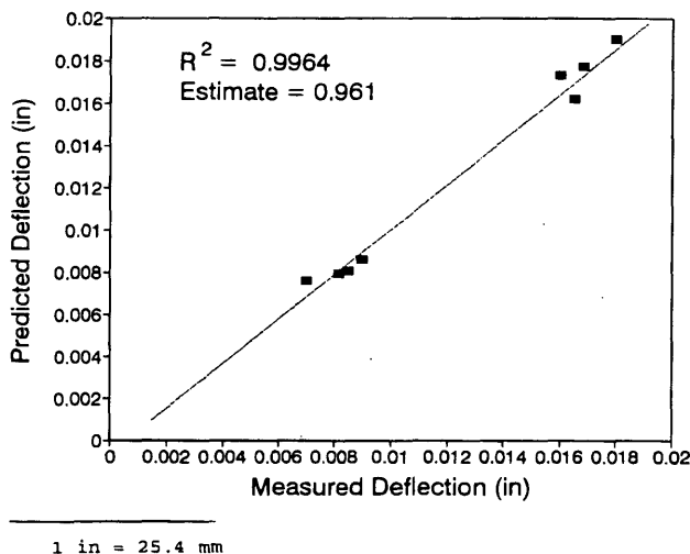
FIGURE 4 Dynamic analysis verification (moving loads).
