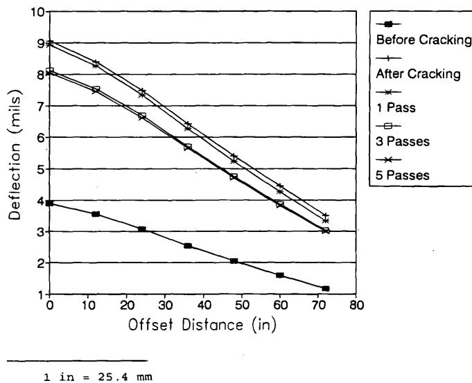
FIGURE 10 Effect of the number of passes on surface deflection (FWD).
