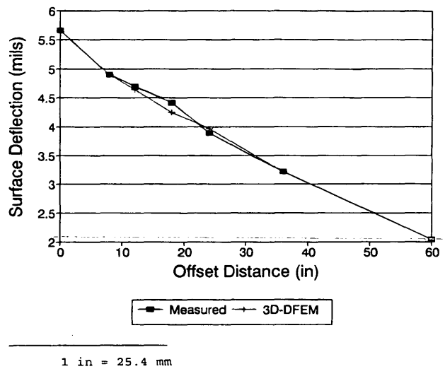
FIGURE 5 Dynamic analysis verification (FWD).
