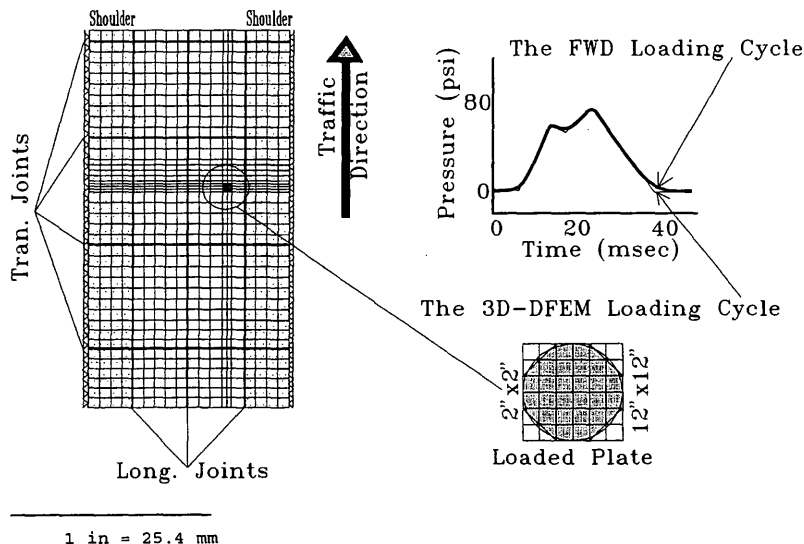
FIGURE 3 The 3D-DFEM configuration.
