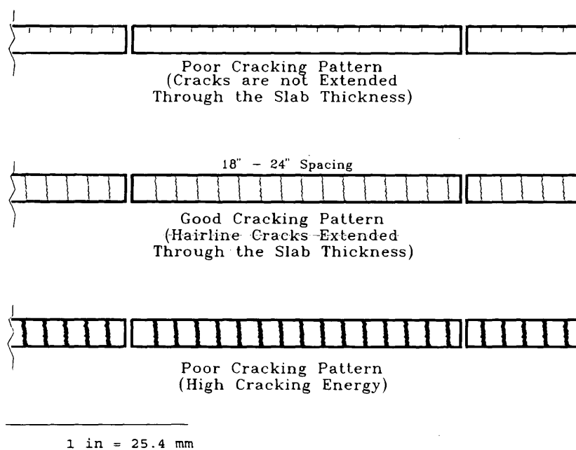
FIGURE 1 Different cracking patterns.
