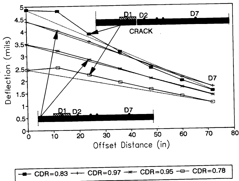
FIGURE 8 Effect of crack conditions on surface deflection.
