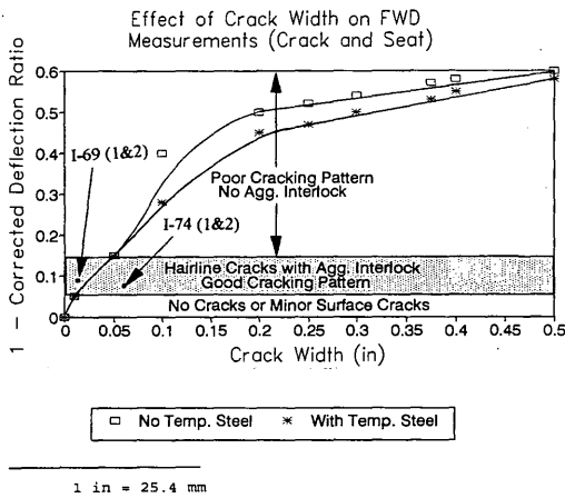
FIGURE 9 Effect of crack width on FWD measurements.
