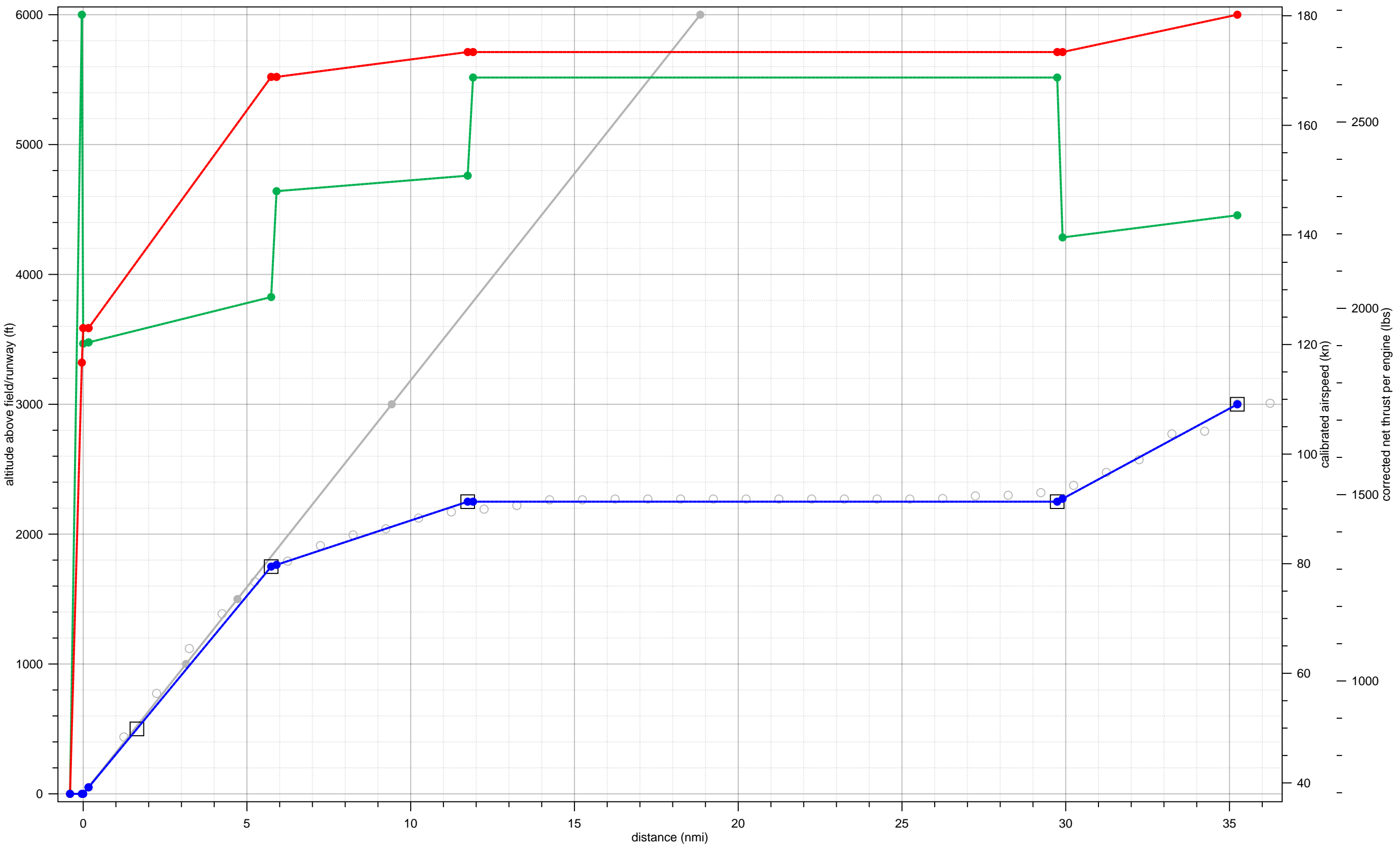
BAE146 fit to 07-A-B737-LJ-1-2000-20to29-5to14
