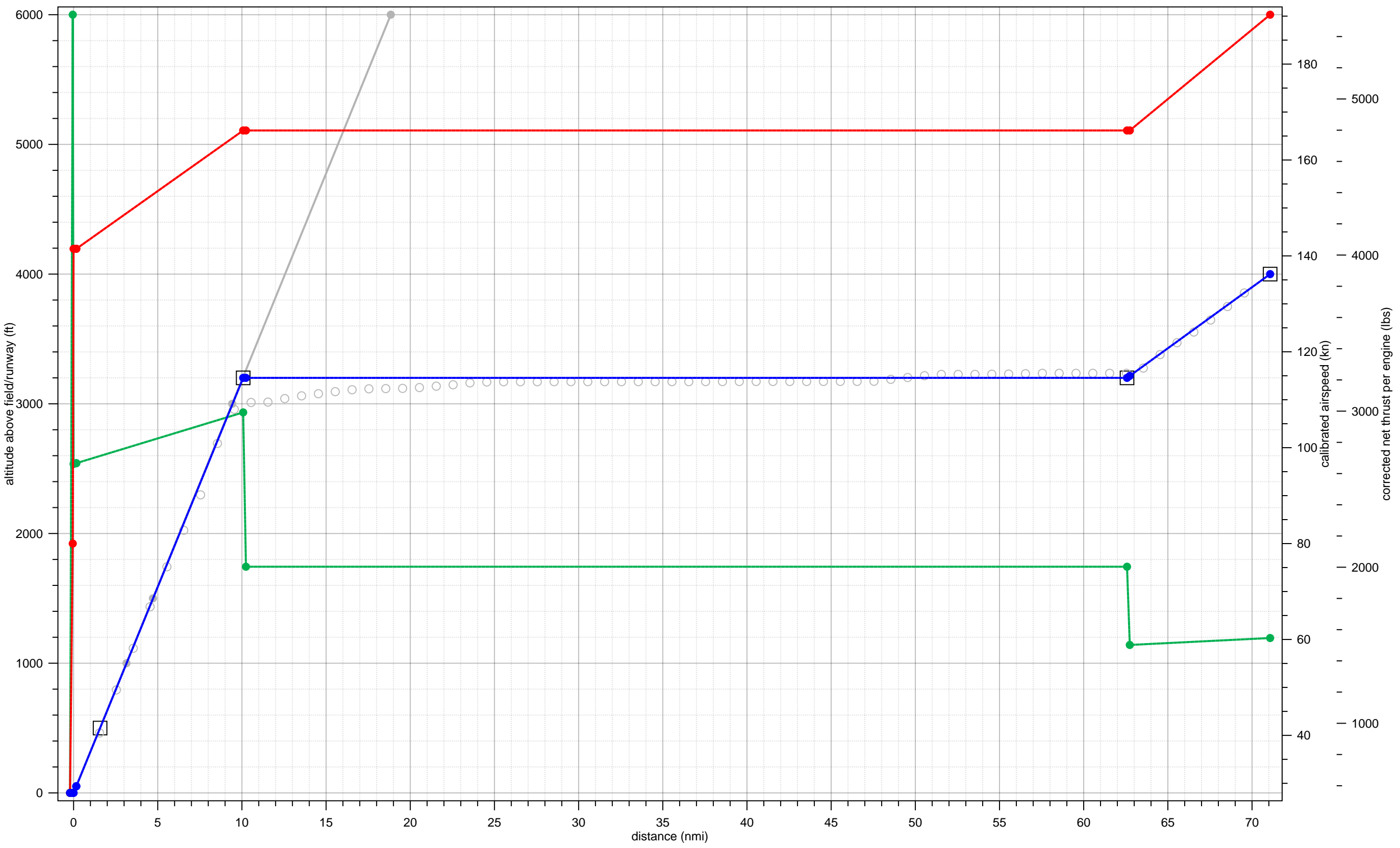
GIV fit to 12-A-E145-LJ-1-3000-50andup-5to14
