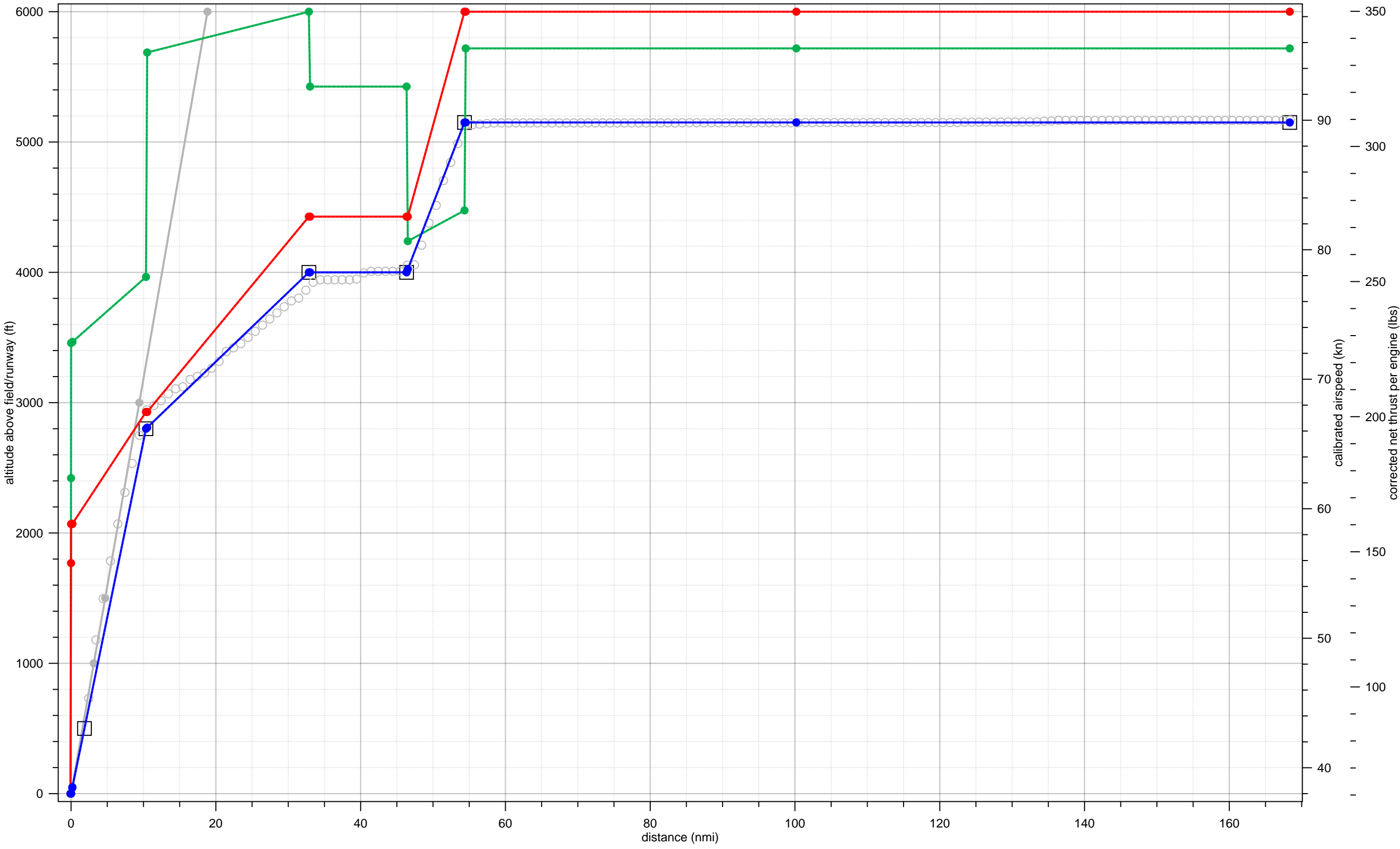
COMSEP fit to 28-A-C172-SP-1-5000-61andup-0to20
