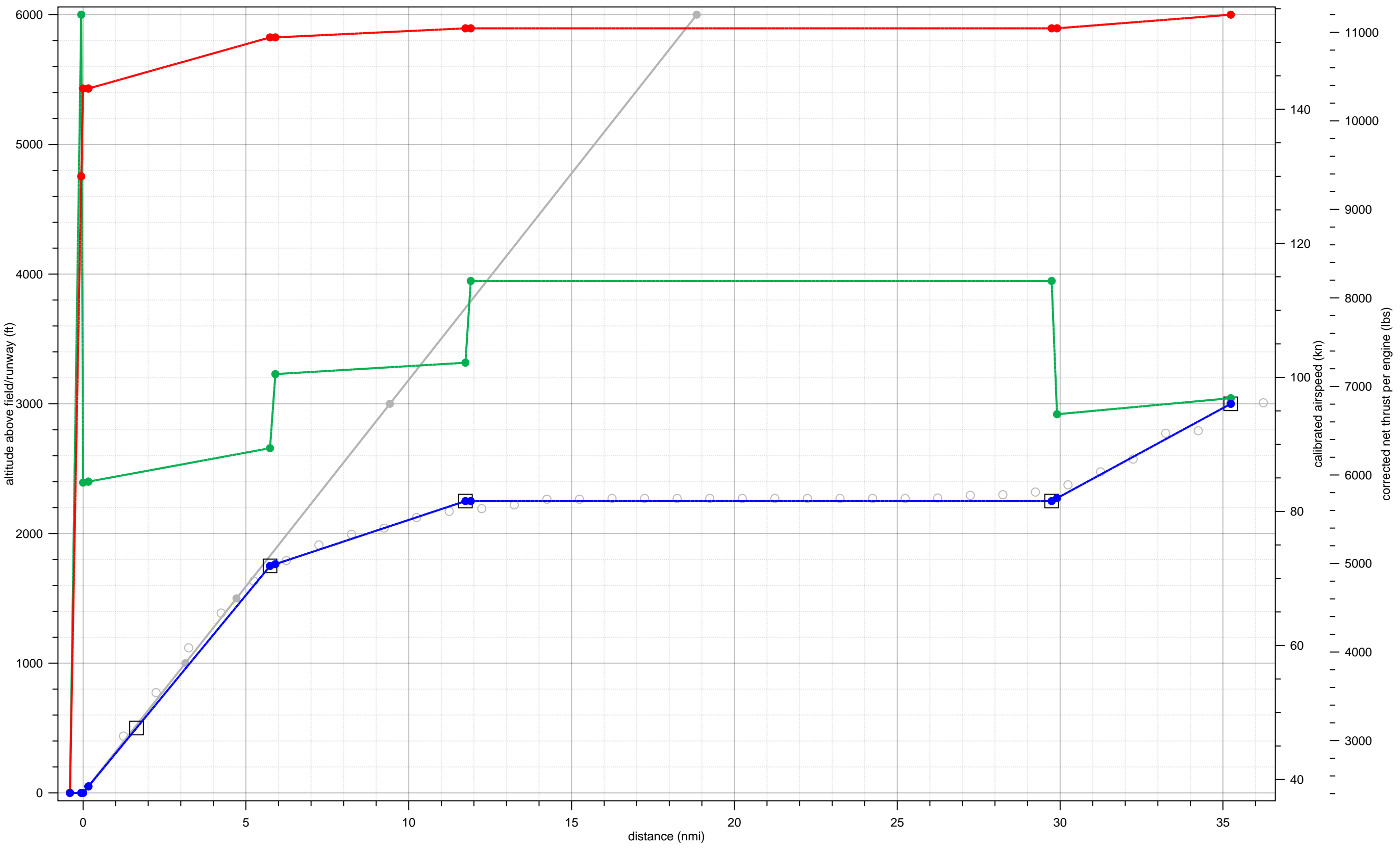
MD9028 fit to 07-A-B737-LJ-1-2000-20to29-5to14
