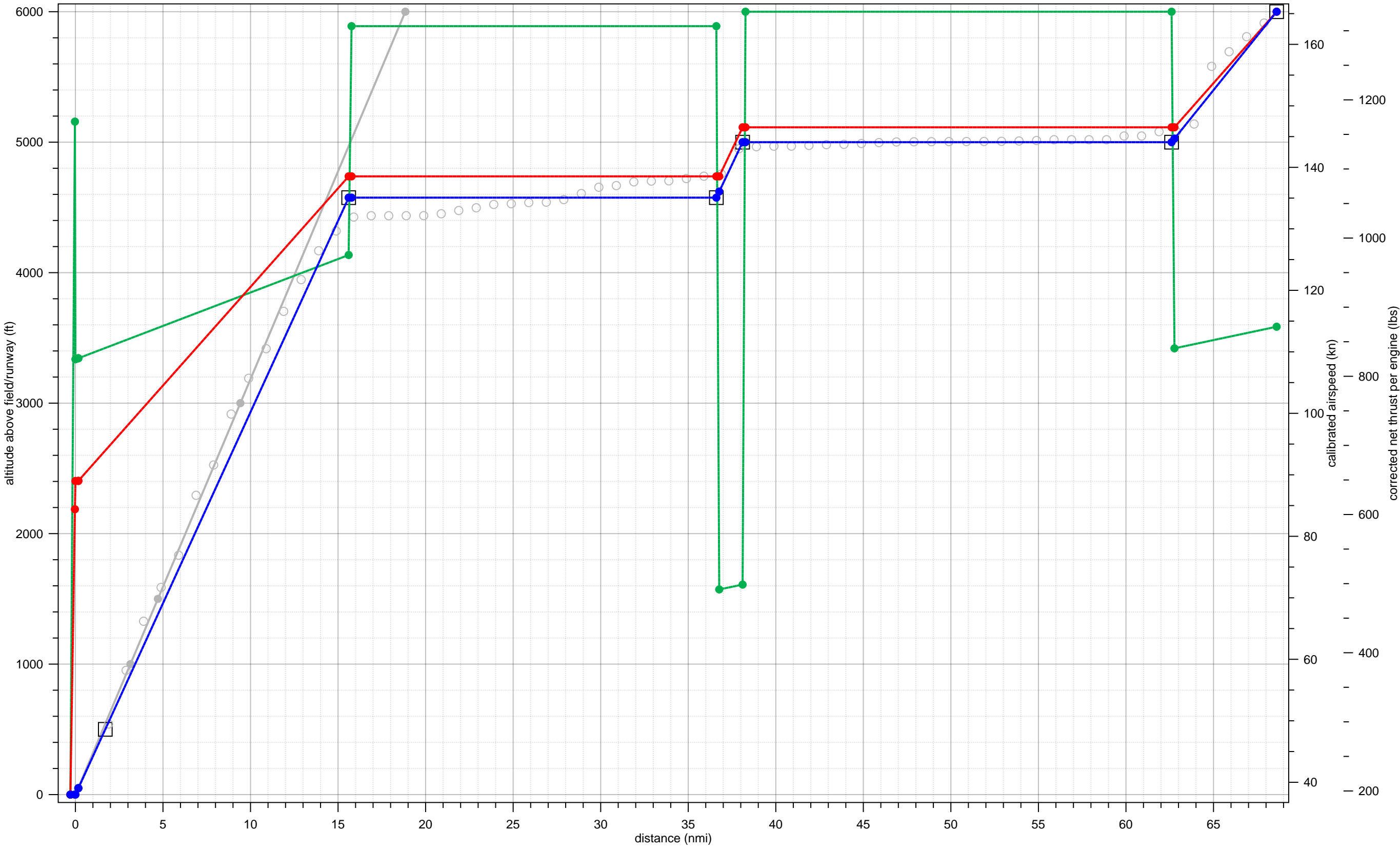
DHC8 fit to 17-A-DH8A-LT-1-5000-40to49-6to15
