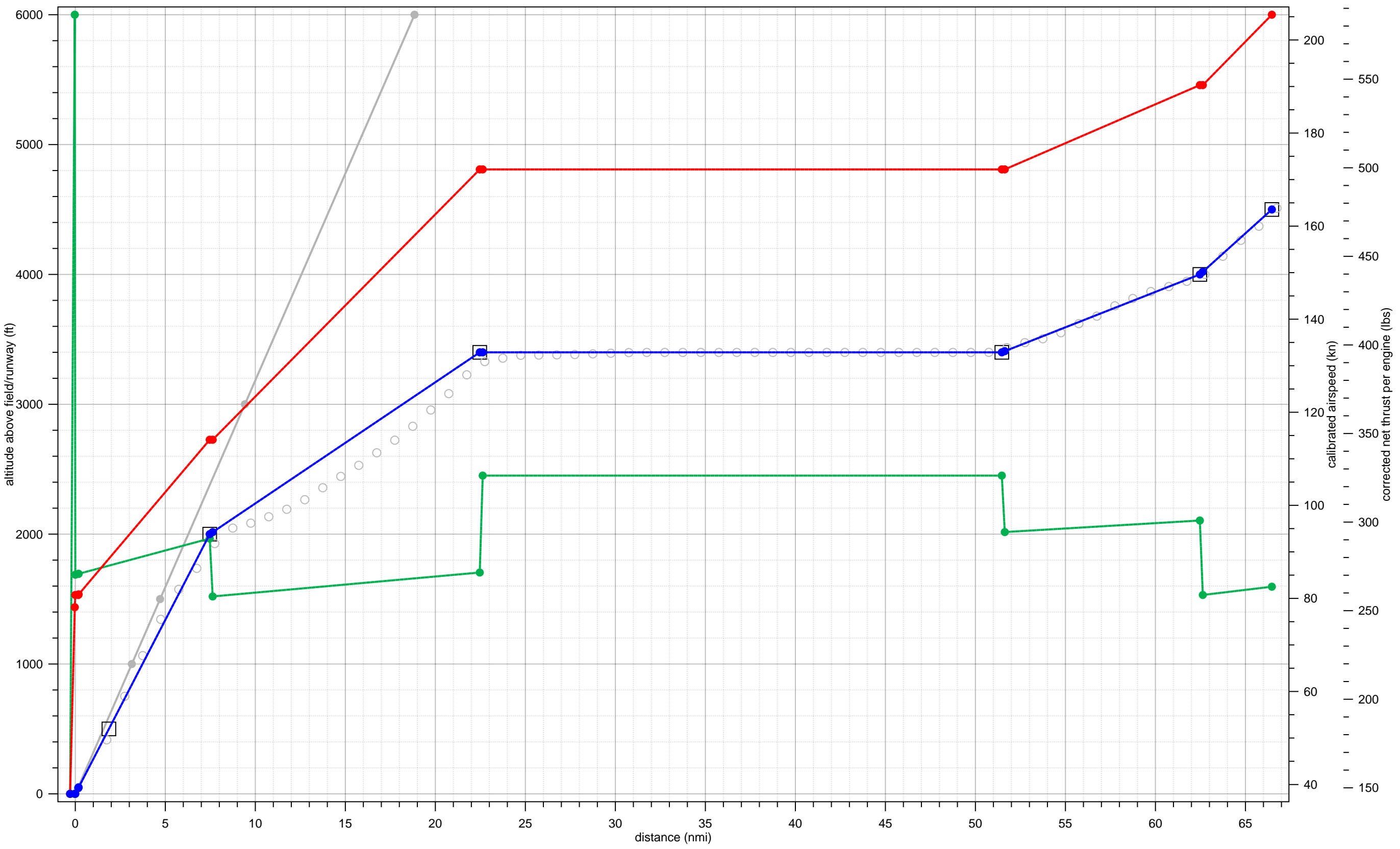
CNA510 fit to 23-A-C750-SJ-1-3000-30andup-15to24
