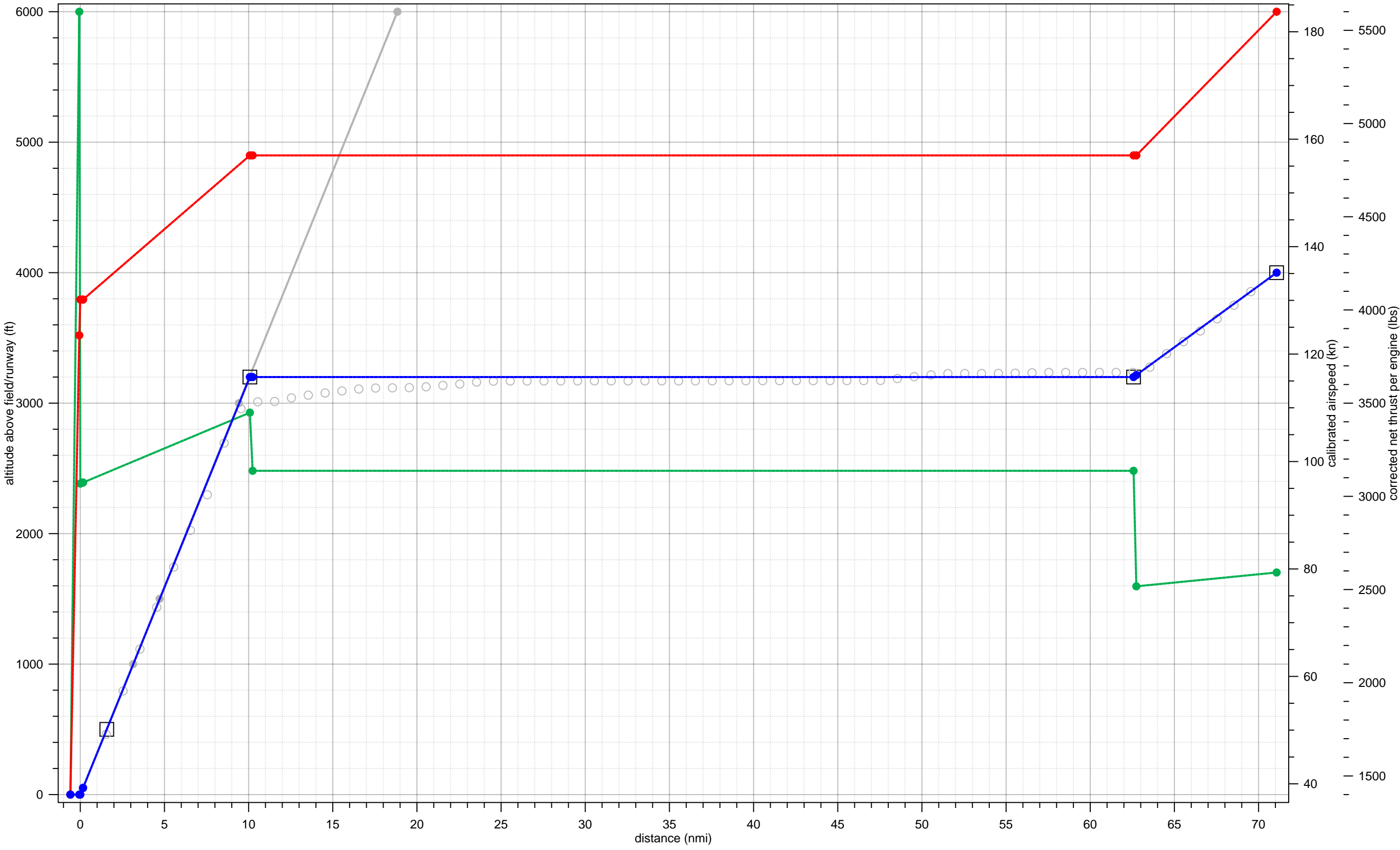
DC910 fit to 12-A-E145-LJ-1-3000-50andup-5to14
