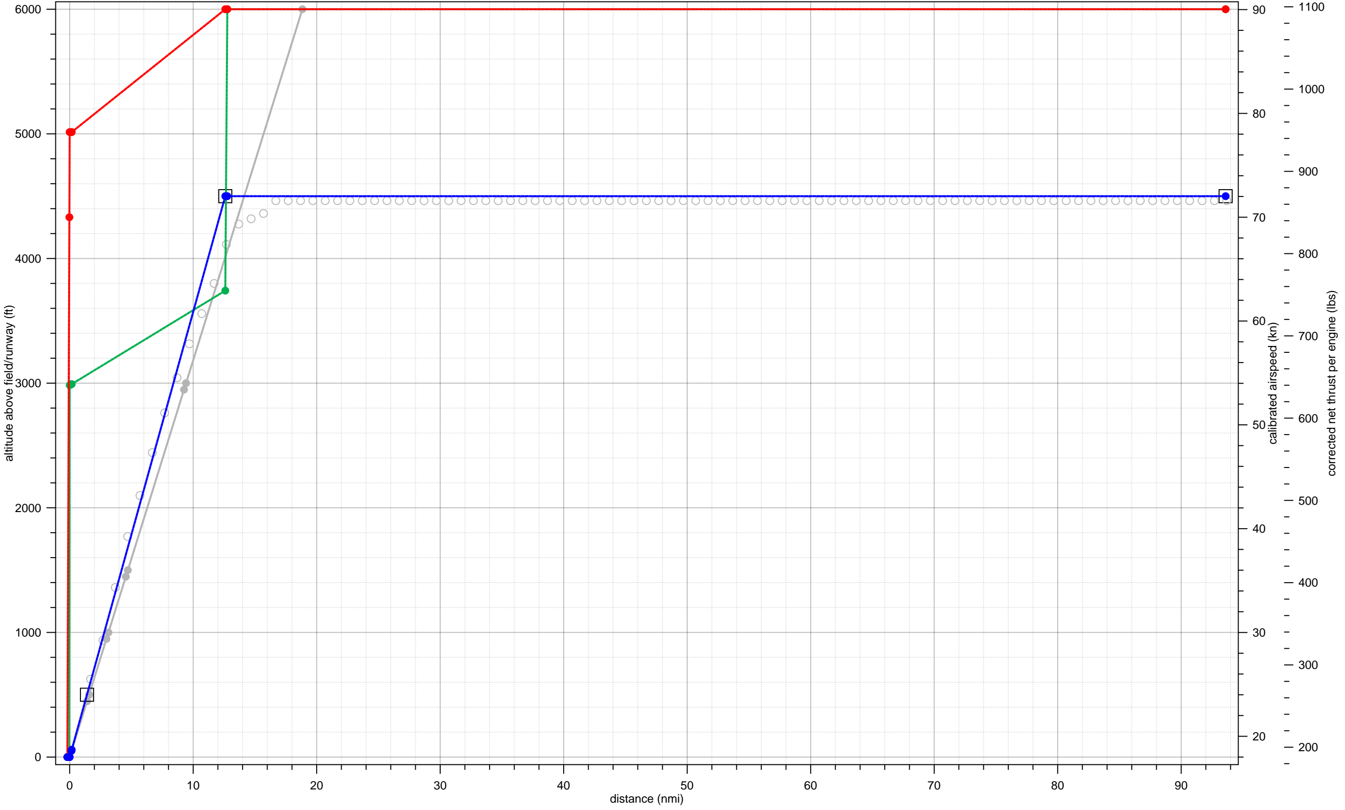
DHC-2FLT fit to 27-A-C172-SP-1-4000-61andup-0to20
