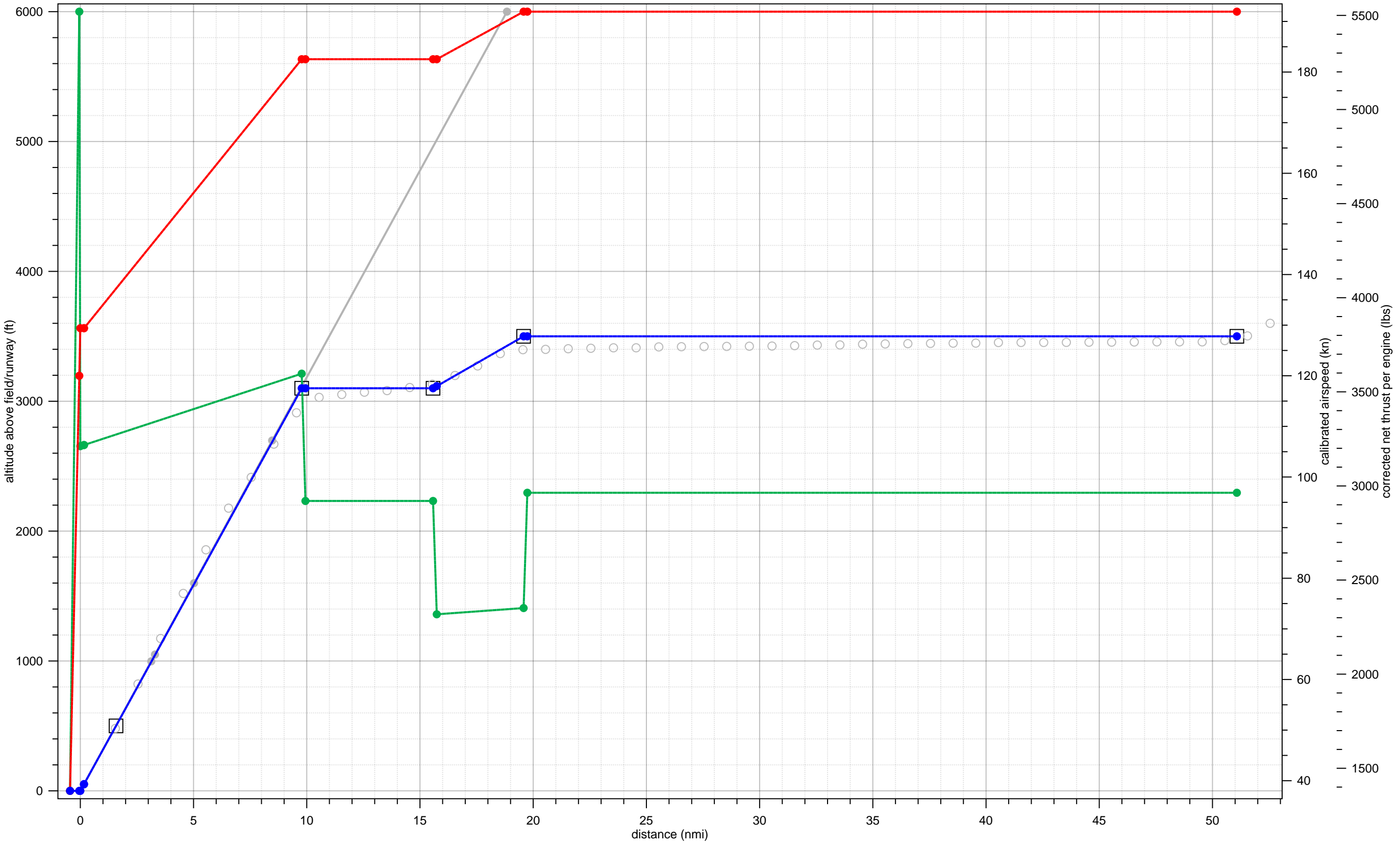
EMB175 fit to 11-A-E145-LJ-1-3000-40to49-5to14
