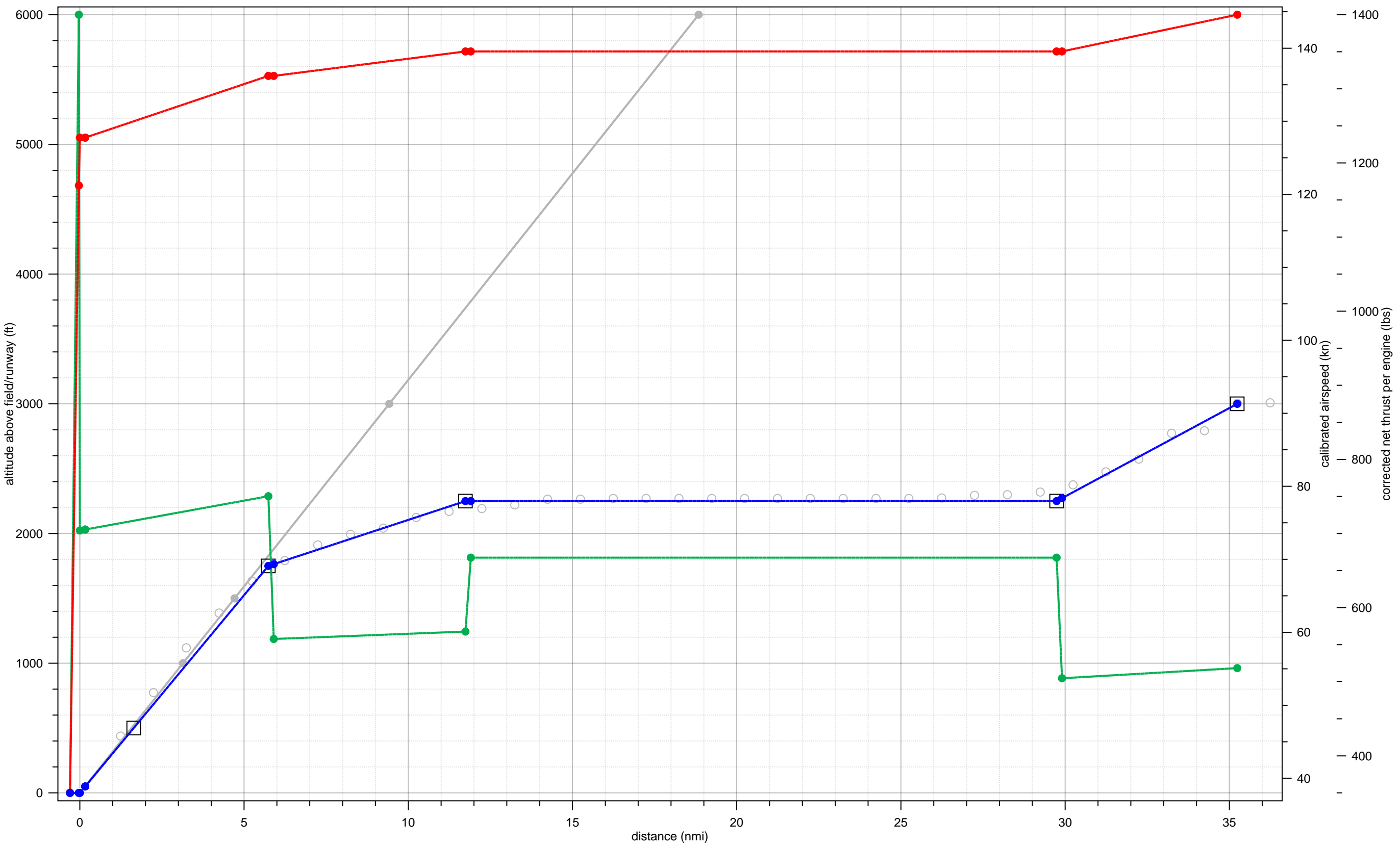
LEAR35 fit to 07-A-B737-LJ-1-2000-20to29-5to14
