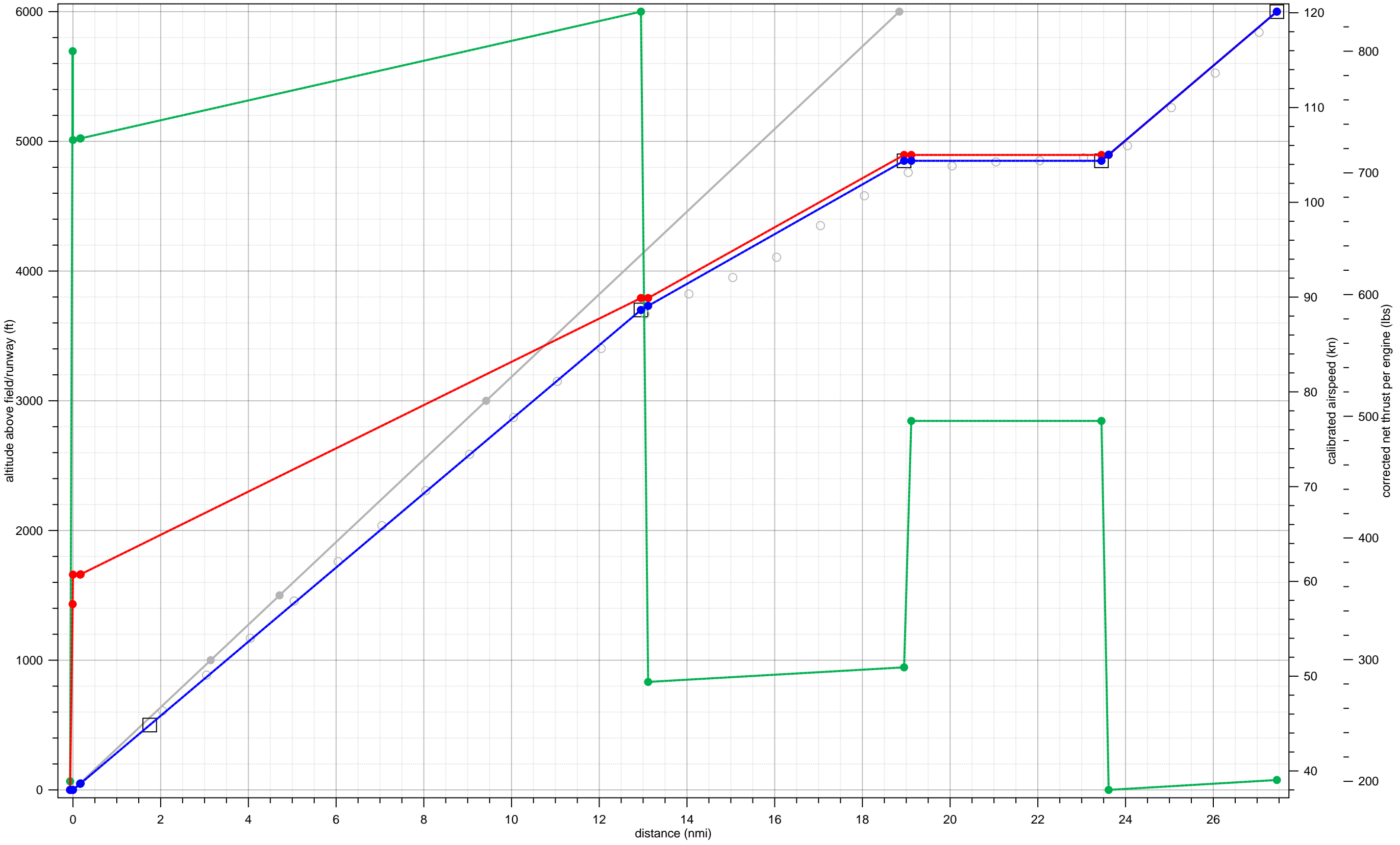
DHC6QP fit to 32-A-B190-ST-1-5000-3to9-16to25
