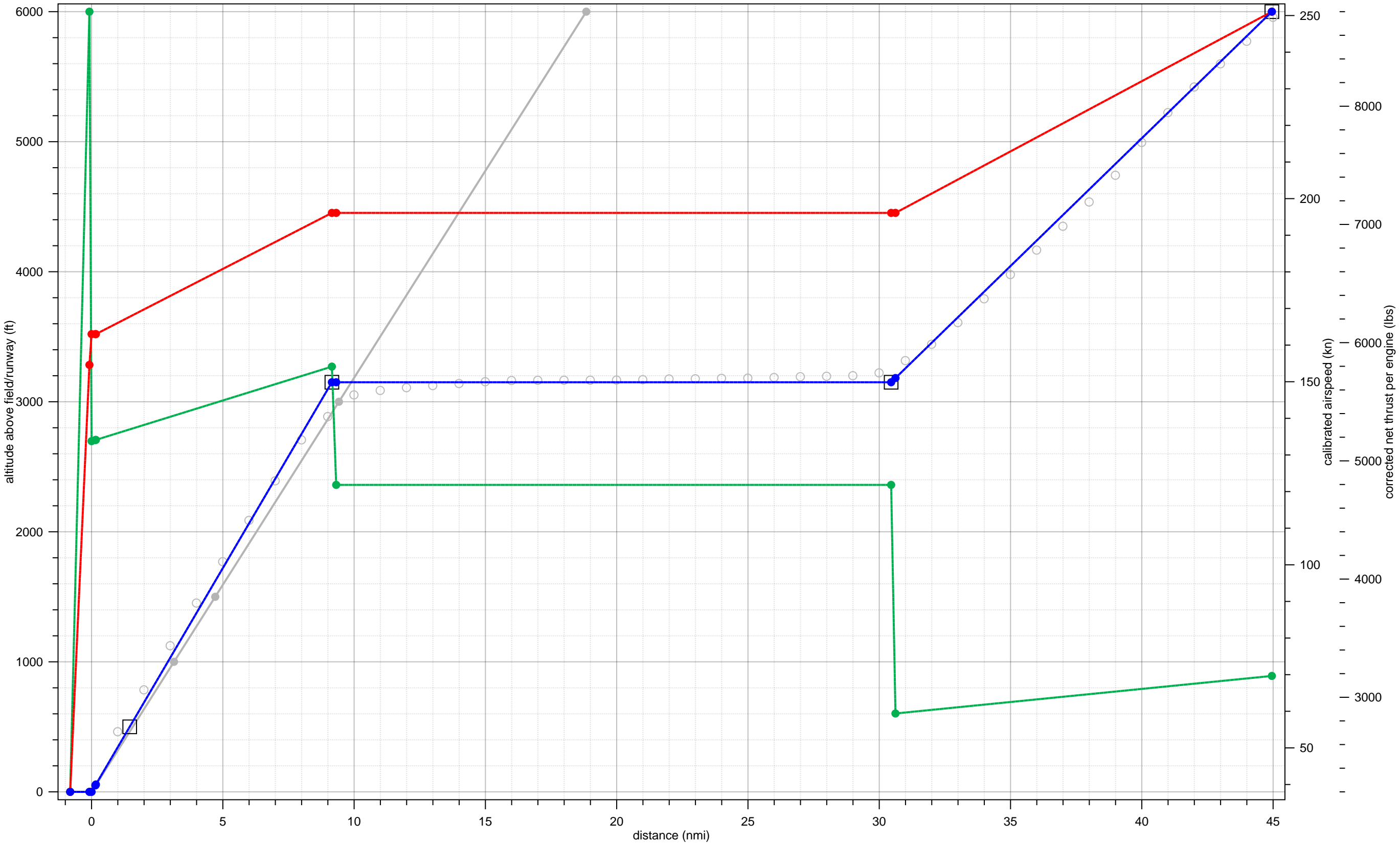
KC135R fit to 02-A-B763-HJ-1-3000-20to29-5to13
