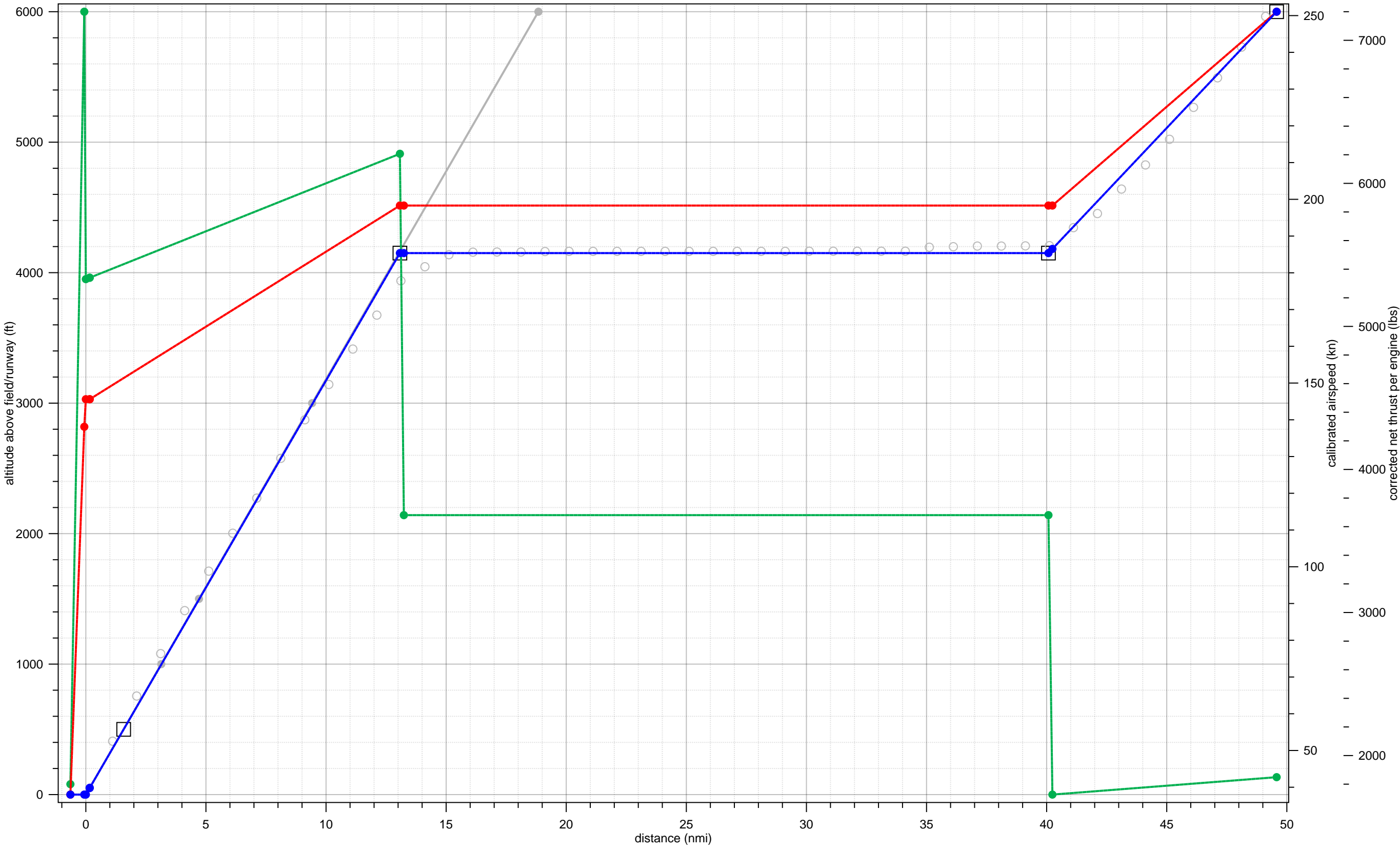
DC850 fit to 03-A-B763-HJ-1-4000-20to29-14to23
