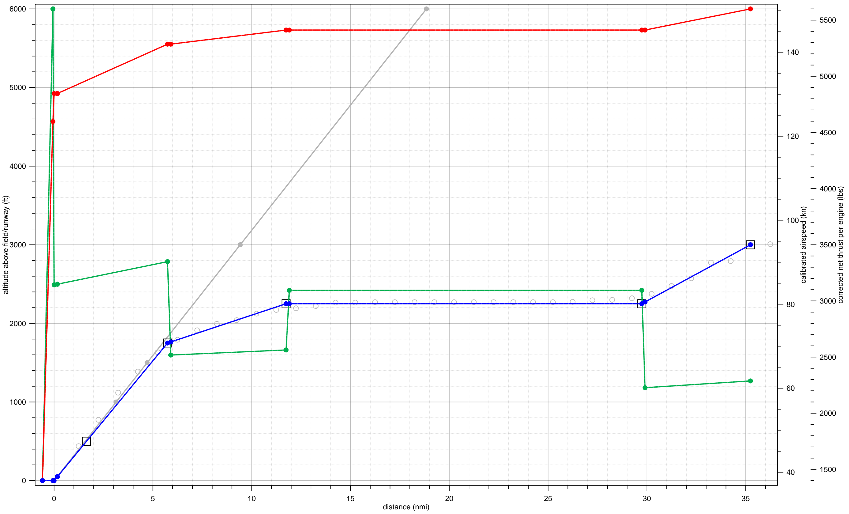
DC910 fit to 07-A-B737-LJ-1-2000-20to29-5to14
