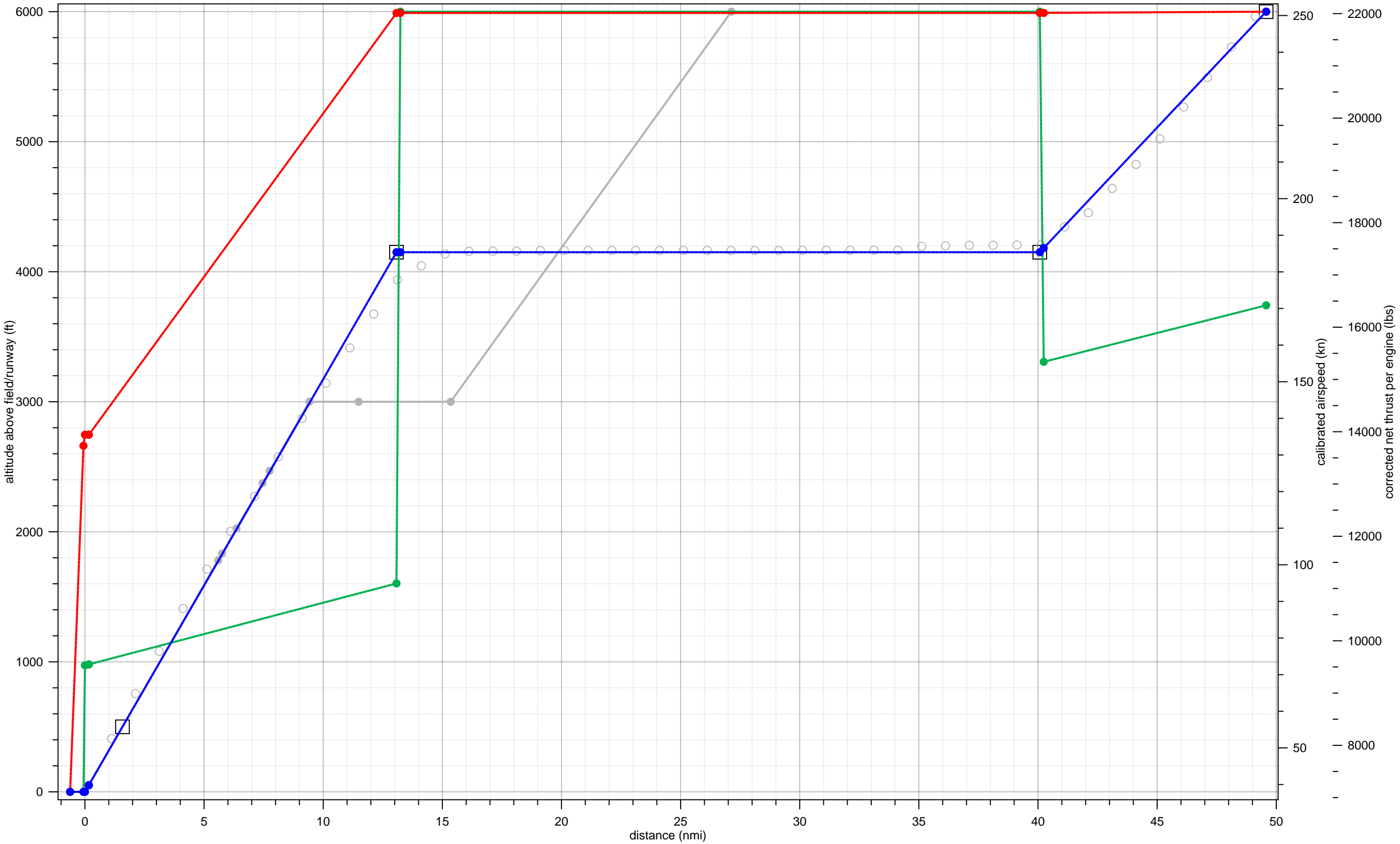
A330-343 fit to 03-A-B763-HJ-1-4000-20to29-14to23
