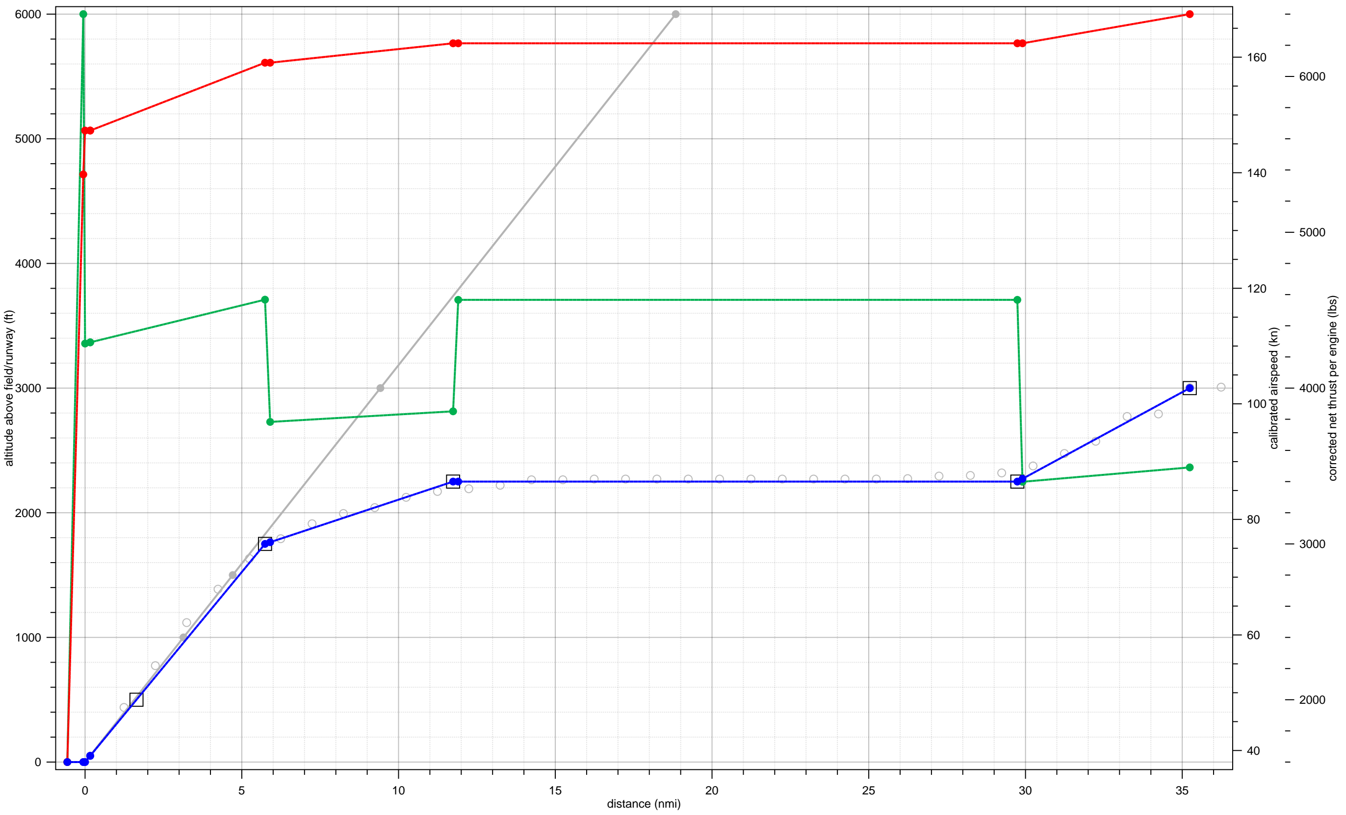
DC950 fit to 07-A-B737-LJ-1-2000-20to29-5to14
