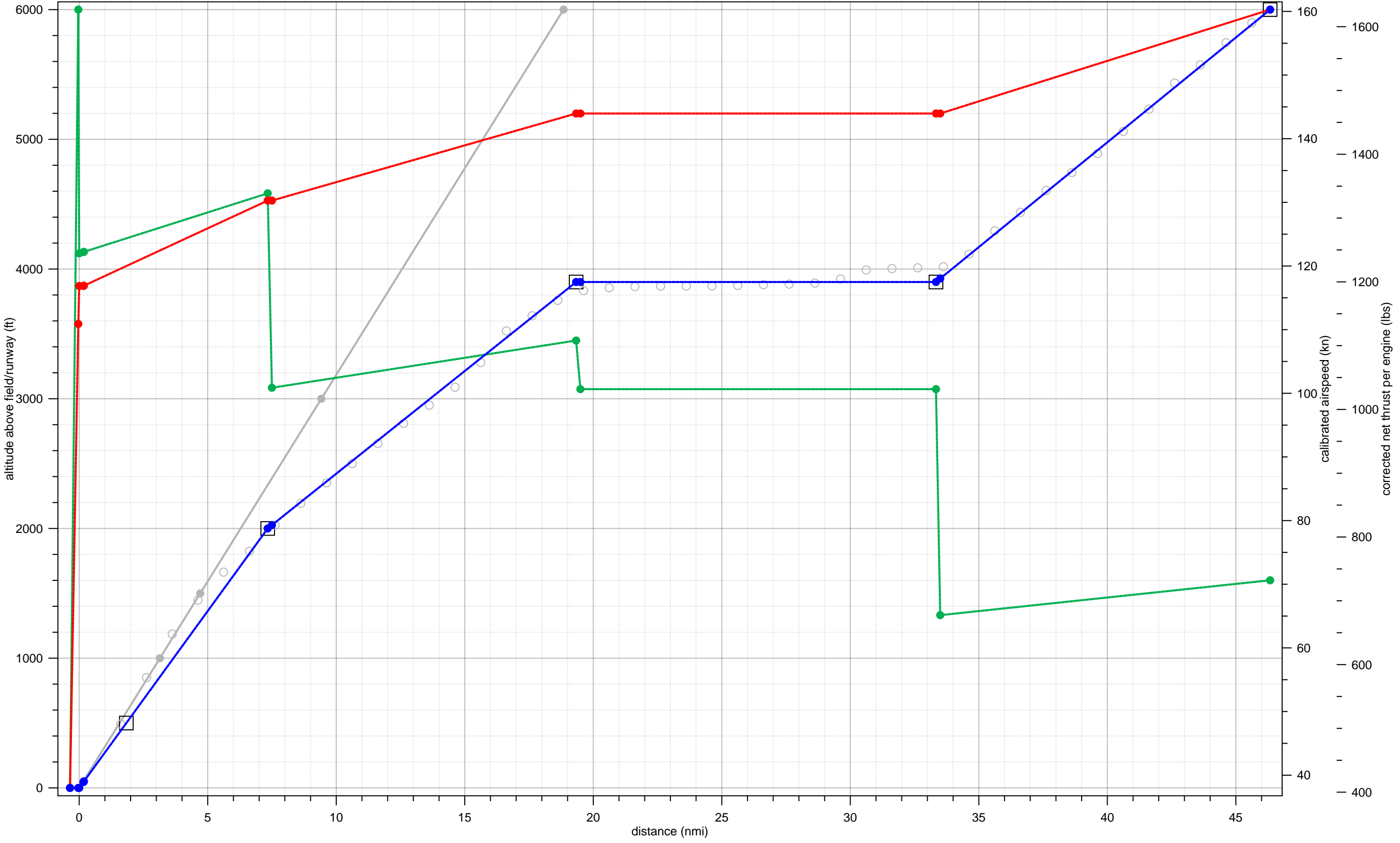
SF340 fit to 14-A-DH8A-LT-1-4000-10to19-16to25
