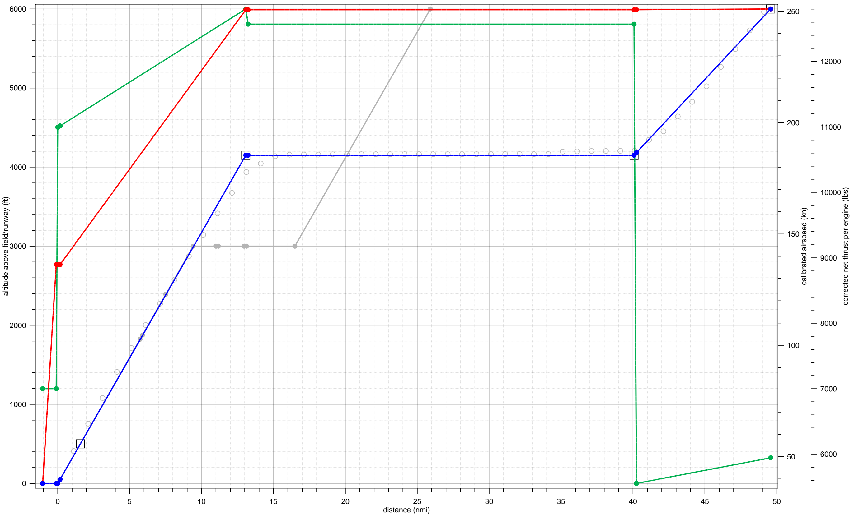
A380-841 fit to 03-A-B763-HJ-1-4000-20to29-14to23
