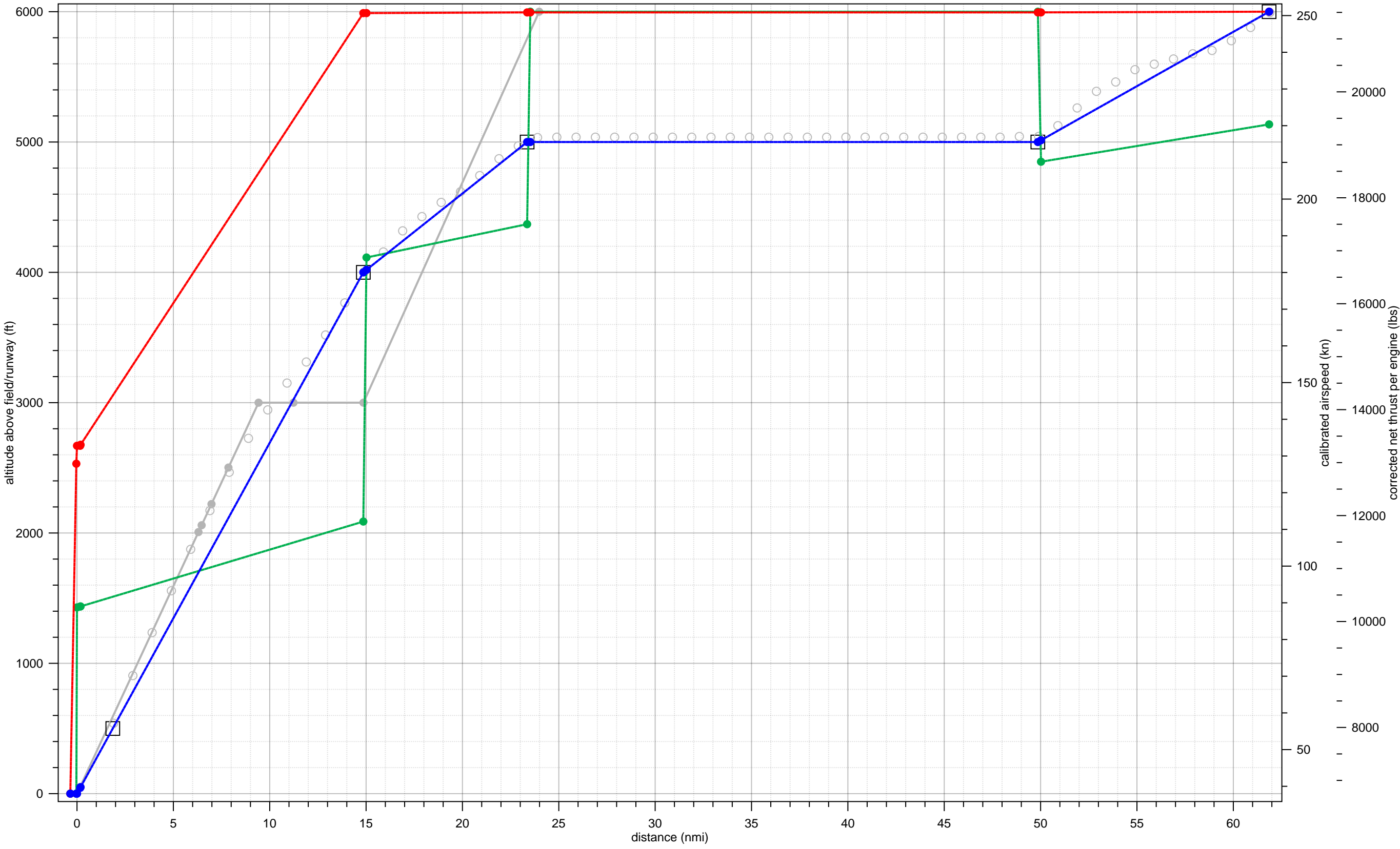
A330-301 fit to 06-A-B764-HJ-1-5000-30to39-14to23
