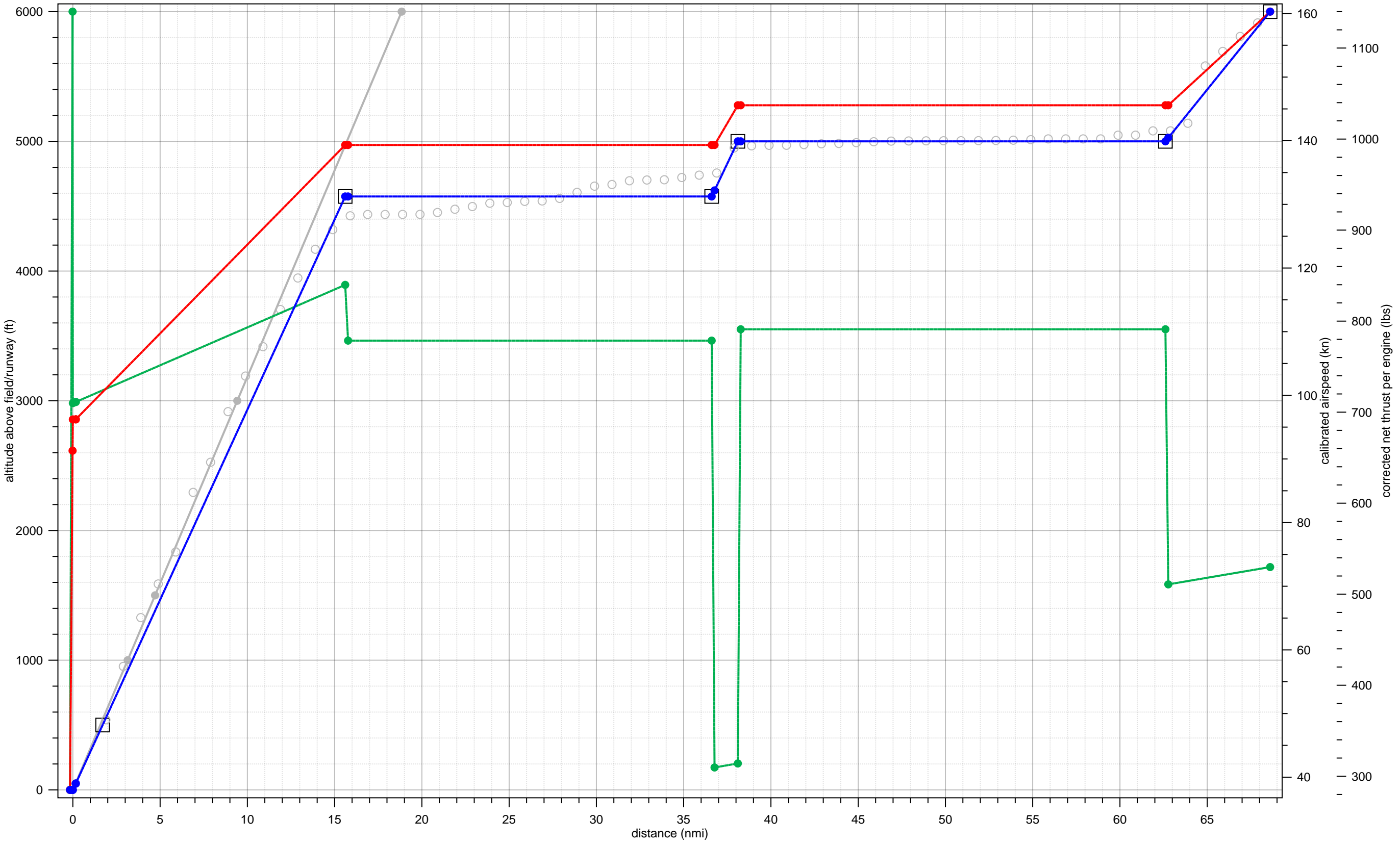
DHC7 fit to 17-A-DH8A-LT-1-5000-40to49-6to15
