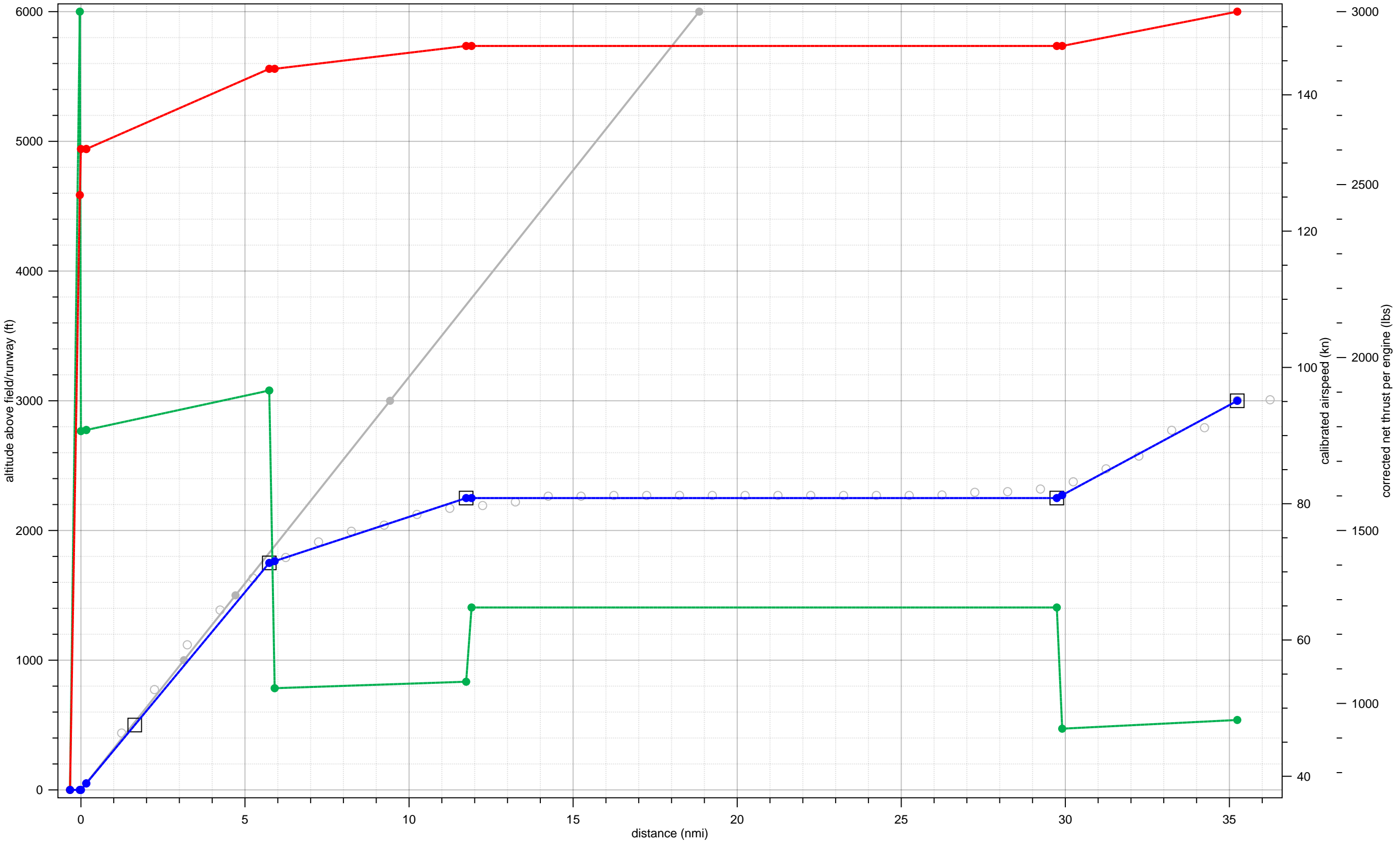
CL600 fit to 07-A-B737-LJ-1-2000-20to29-5to14
