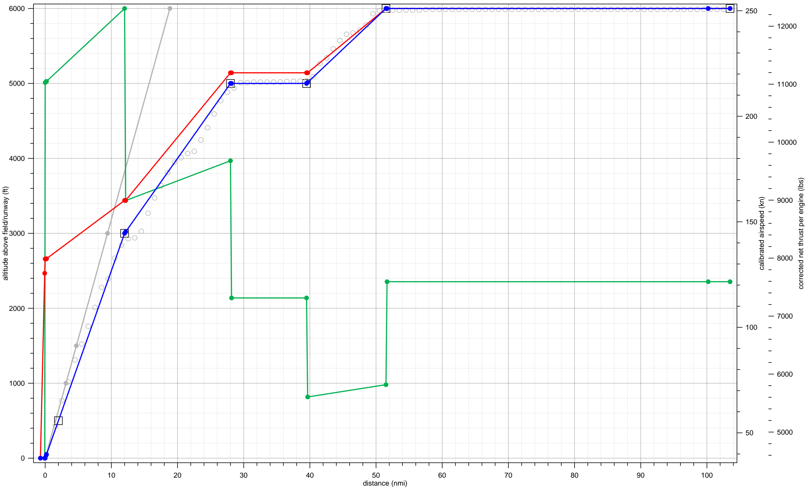
747SP fit to 01-A-B753-HJ-1-6000-40andup-34andup
