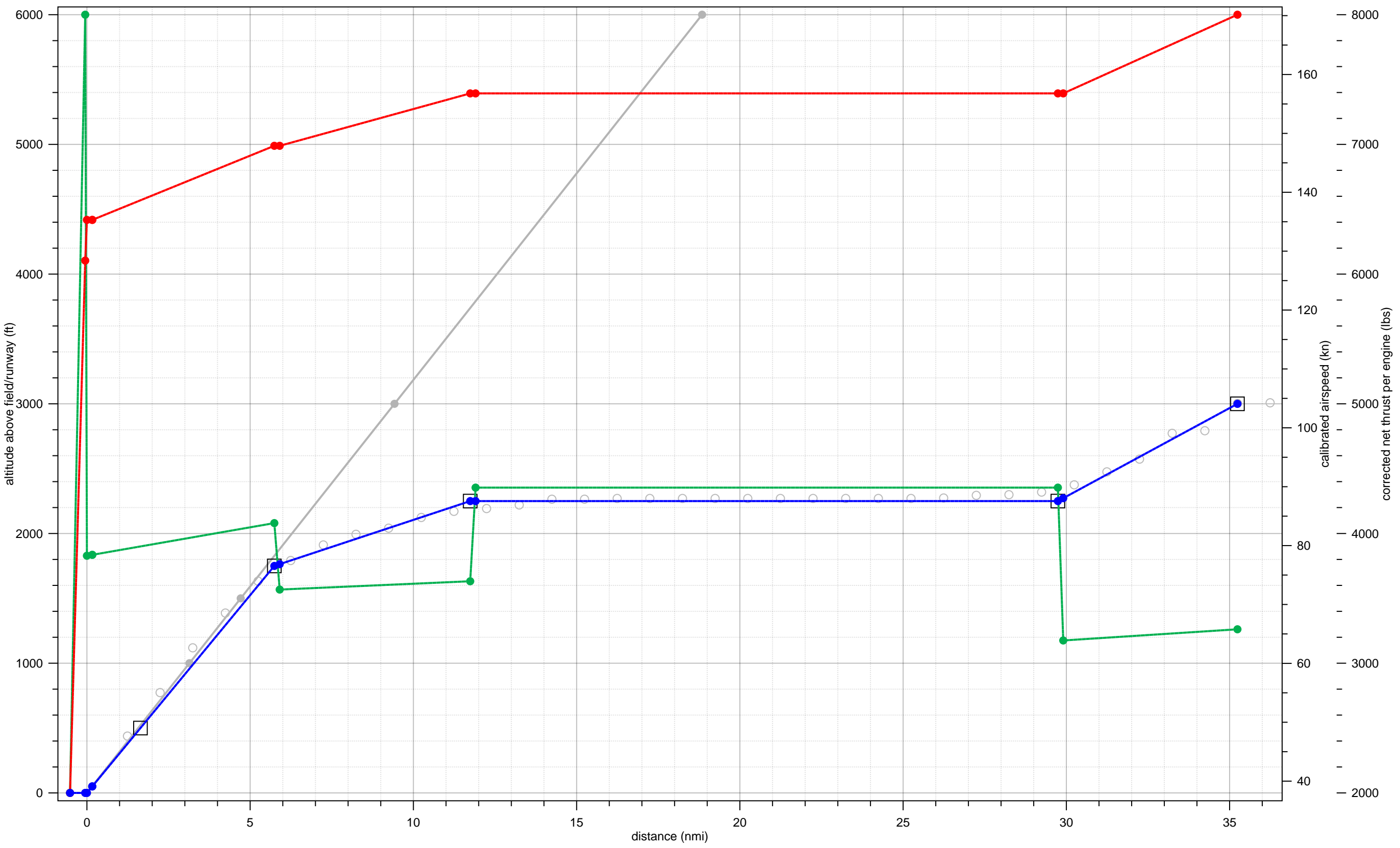
737500 fit to 07-A-B737-LJ-1-2000-20to29-5to14
