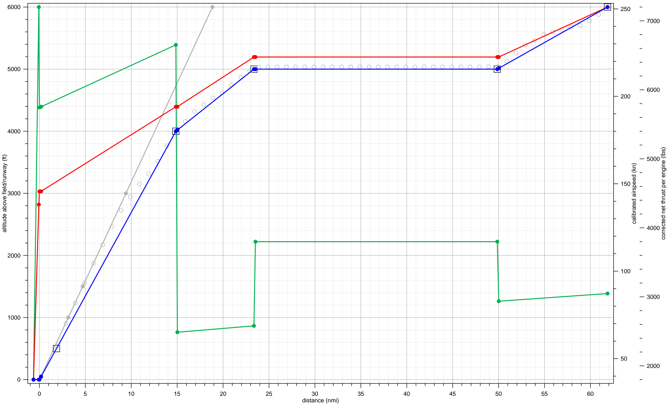
DC850 fit to 06-A-B764-HJ-1-5000-30to39-14to23
