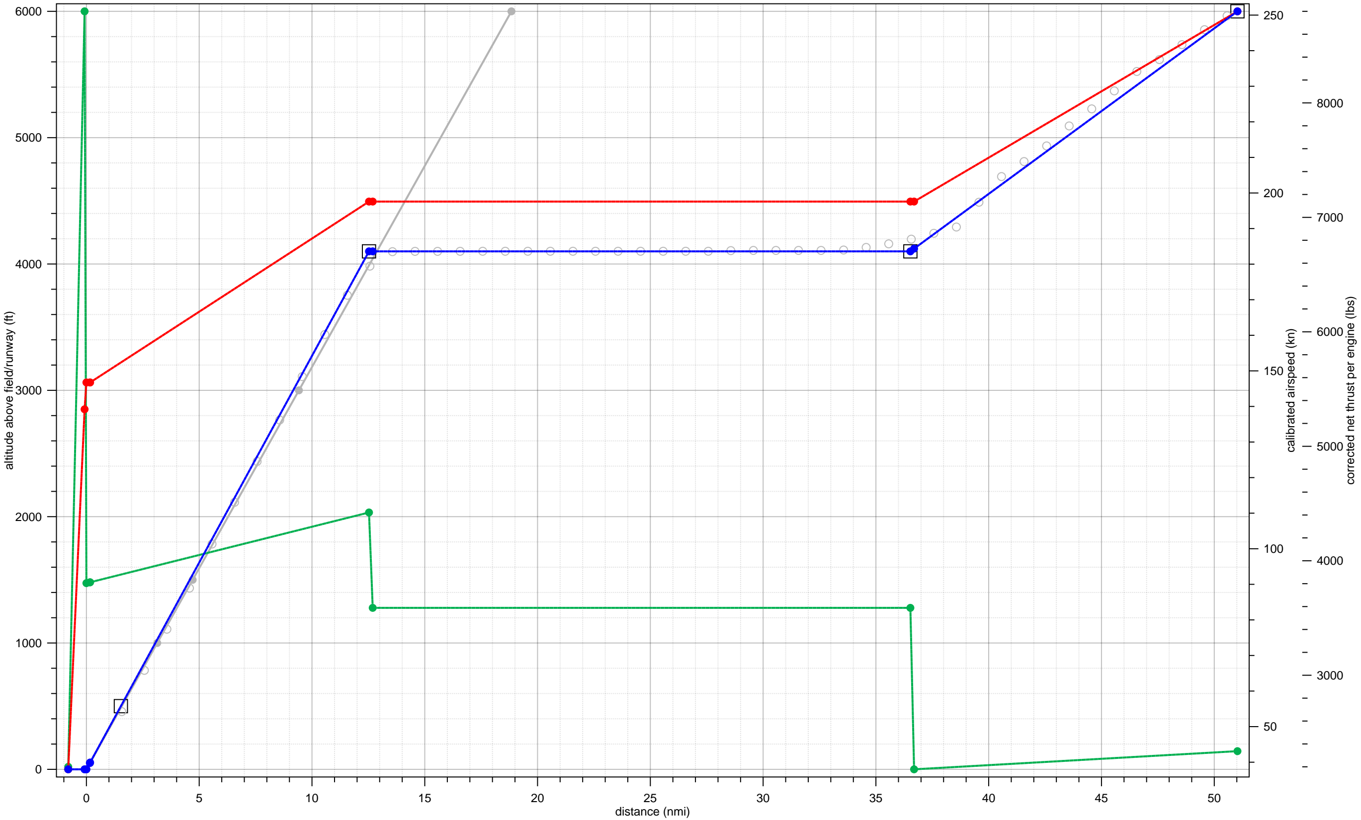
DC870 fit to 04-A-B763-HJ-1-4000-20to29-5to13
