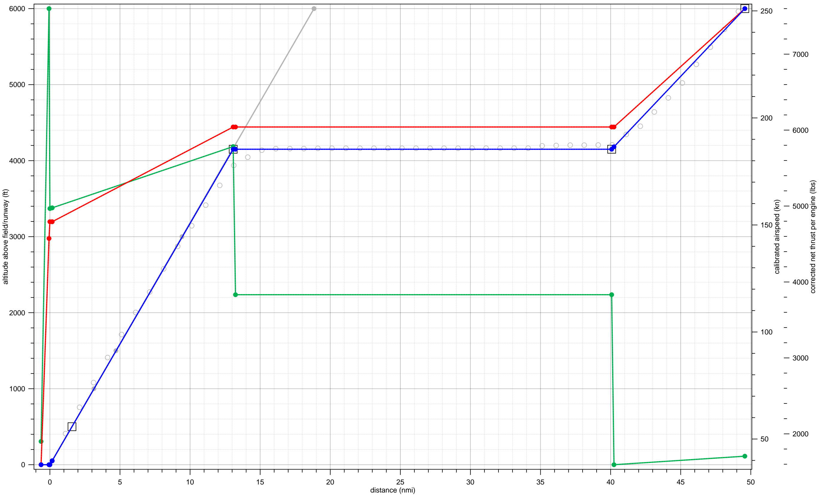
DC860 fit to 03-A-B763-HJ-1-4000-20to29-14to23
