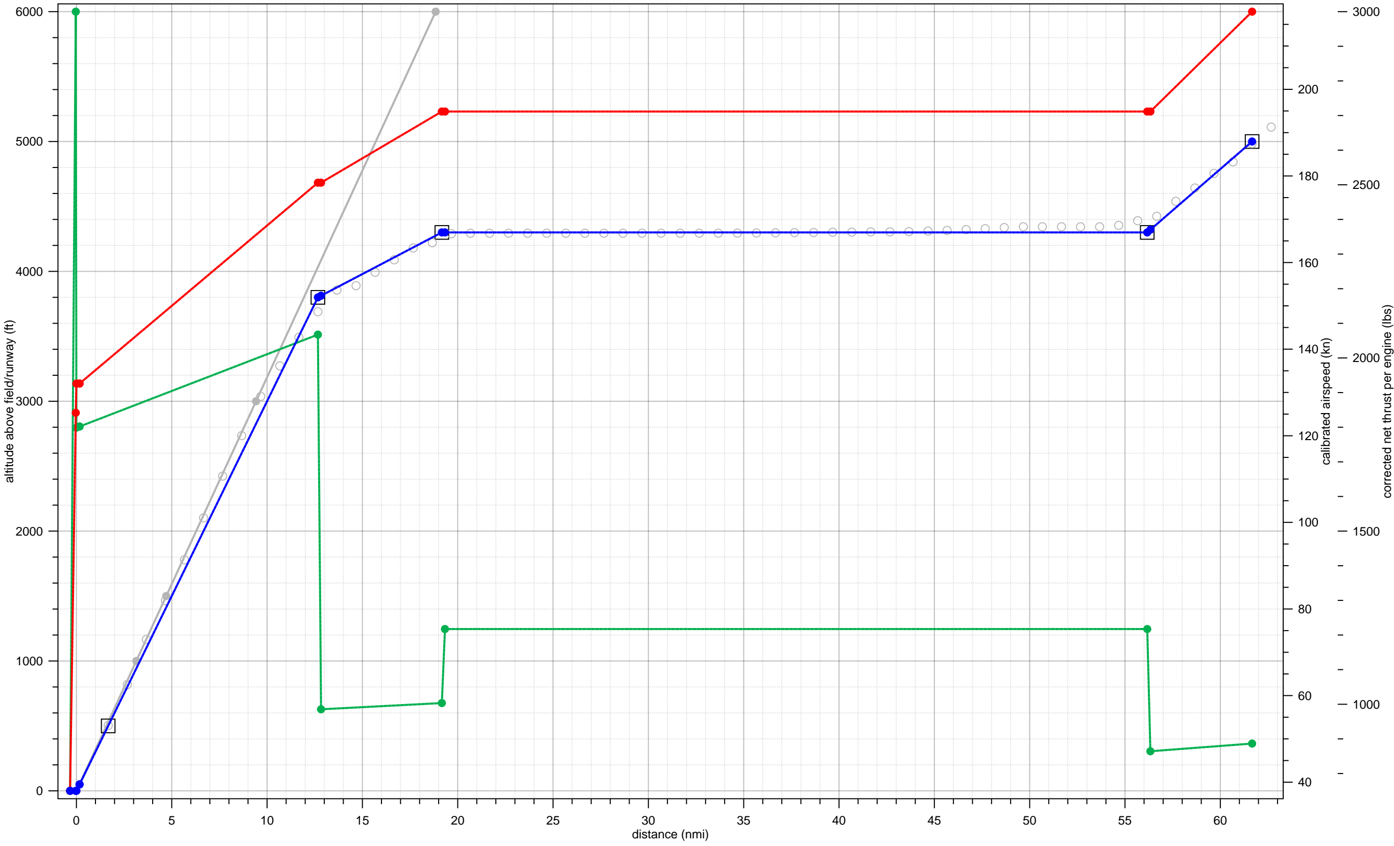
CL600 fit to 08-A-B737-LJ-1-4000-40to49-5to14
