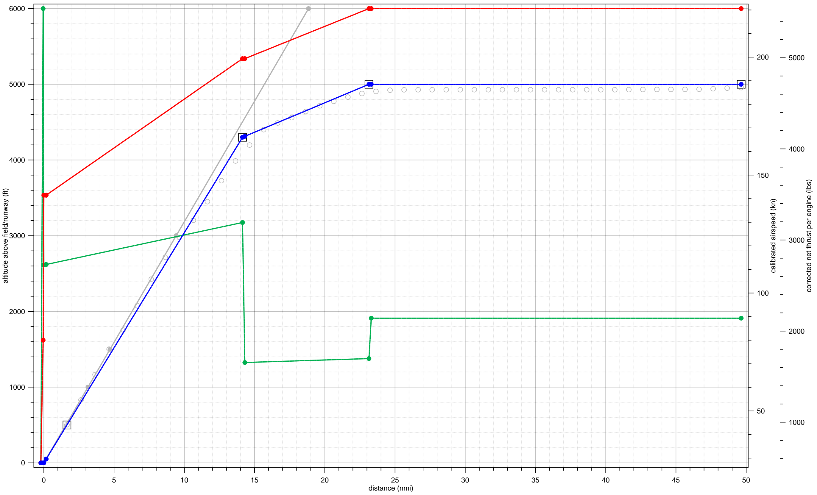
GIV fit to 09-A-B738-LJ-1-5000-30to39-15to24
