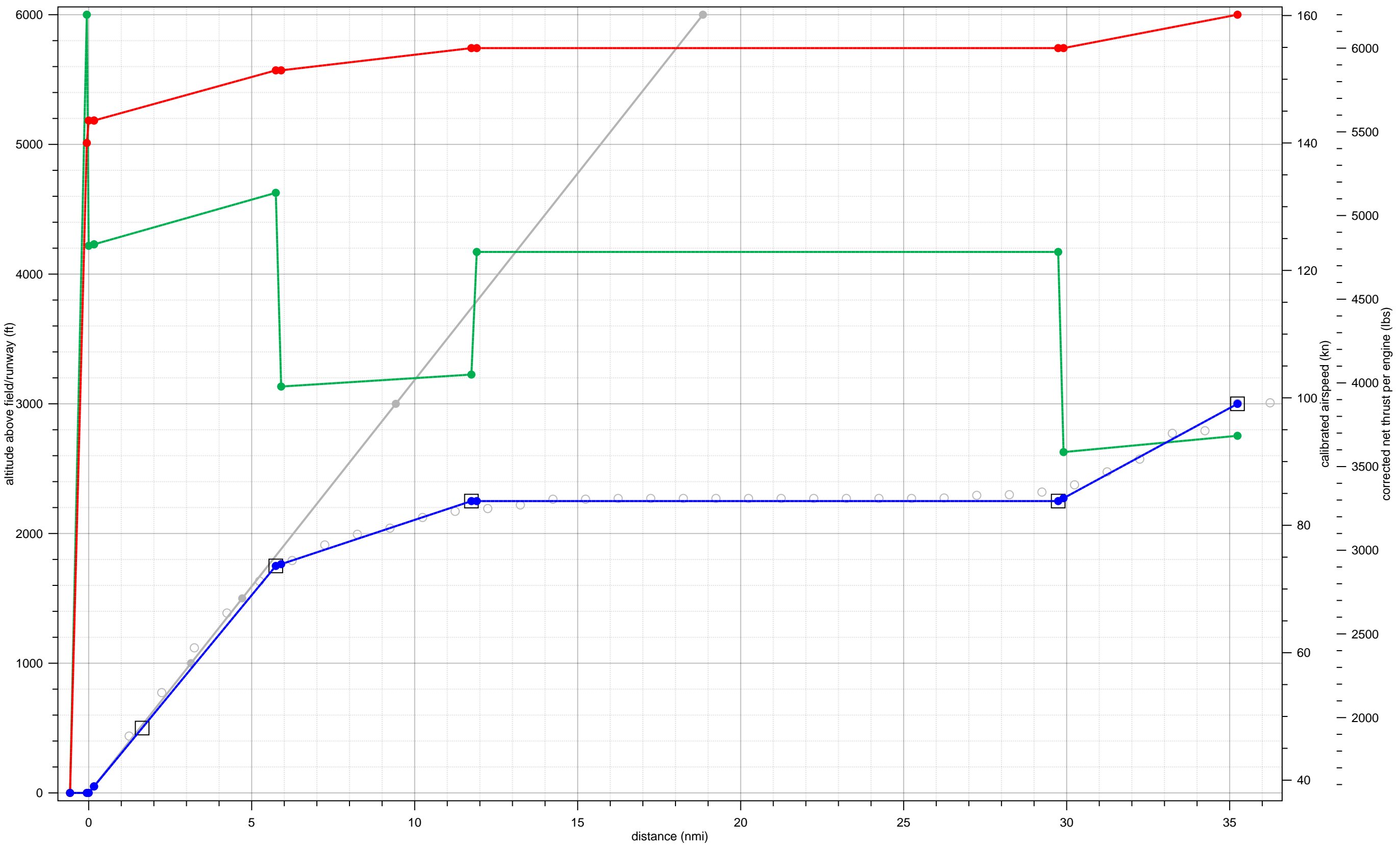
727EM2 fit to 07-A-B737-LJ-1-2000-20to29-5to14
