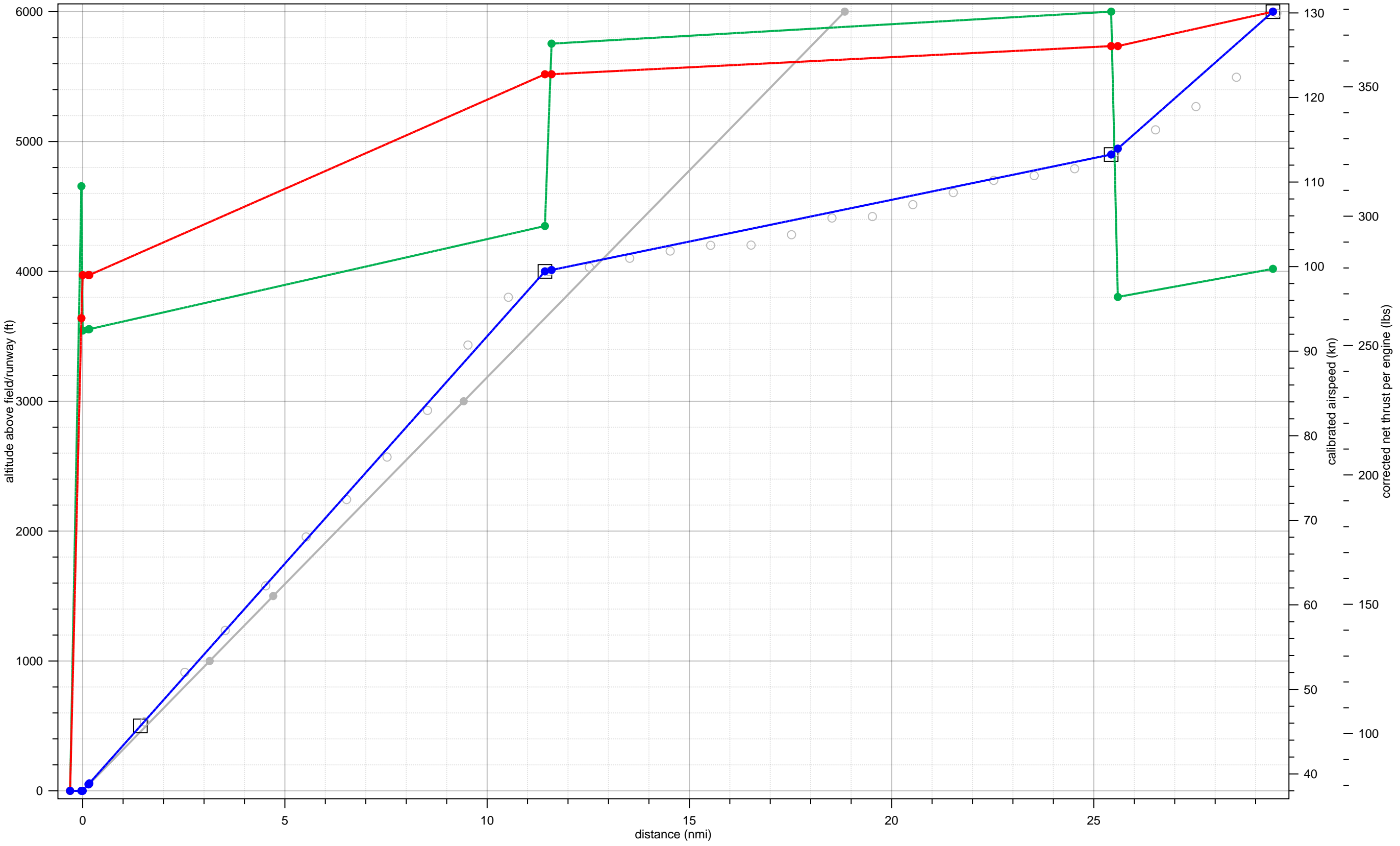
BEC58P fit to 30-A-C182-SP-1-4000-0to20-0to20
