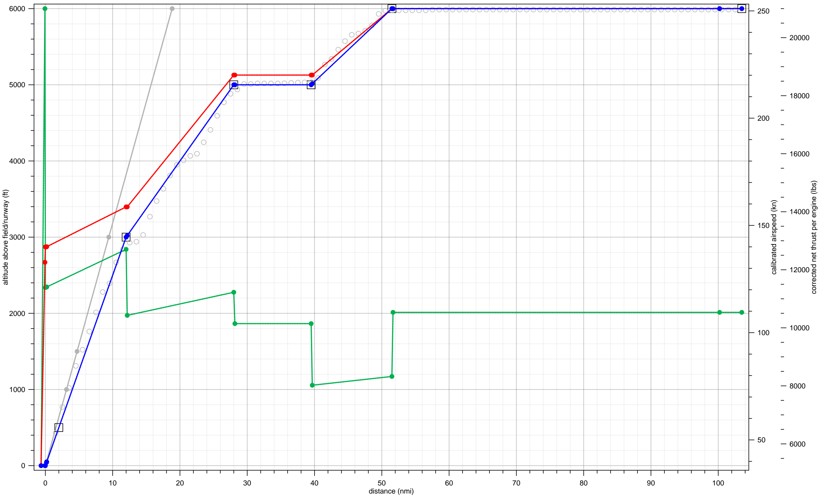
A300B4-203 fit to 01-A-B753-HJ-1-6000-40andup-34andup
