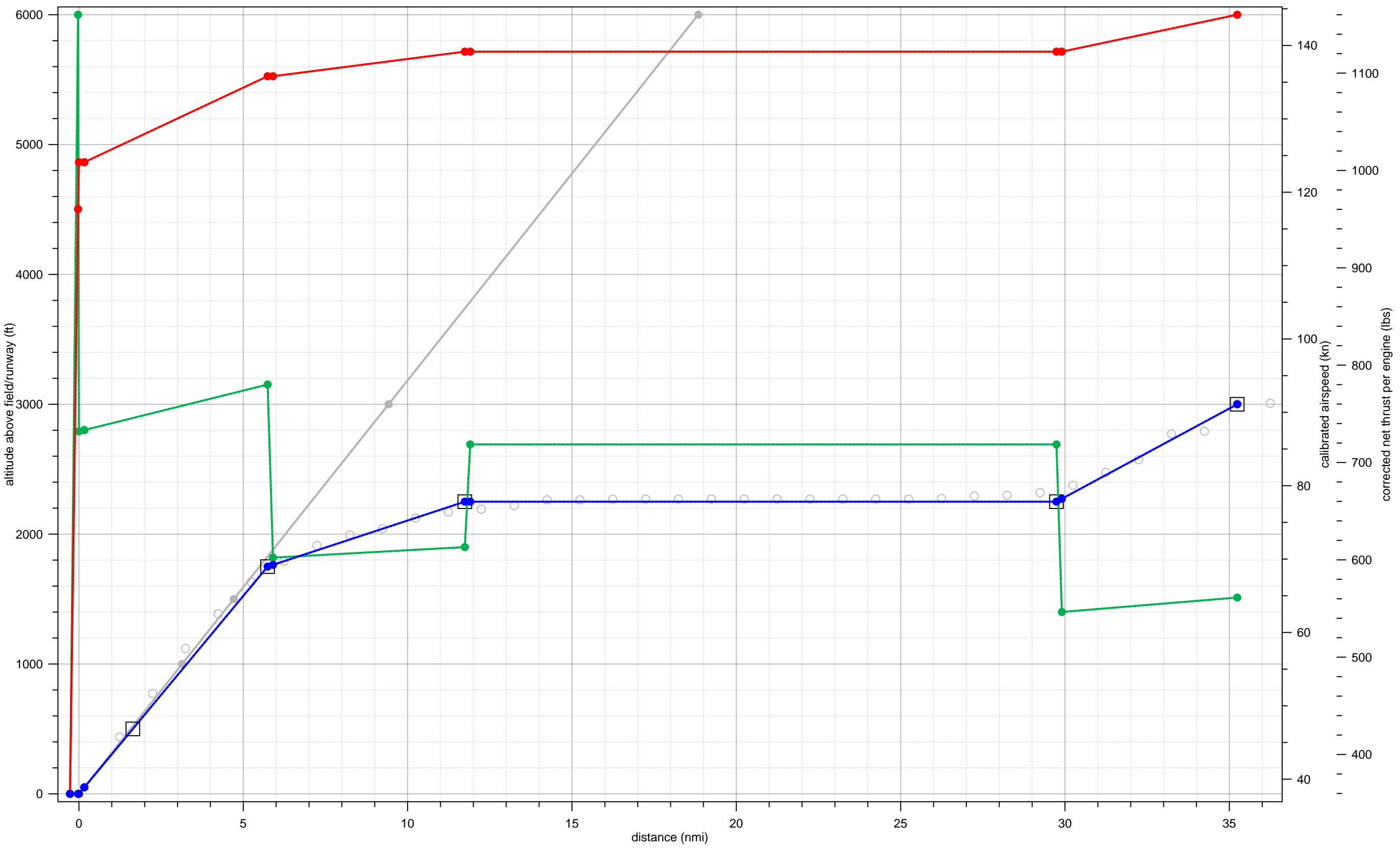
COMJET fit to 07-A-B737-LJ-1-2000-20to29-5to14
