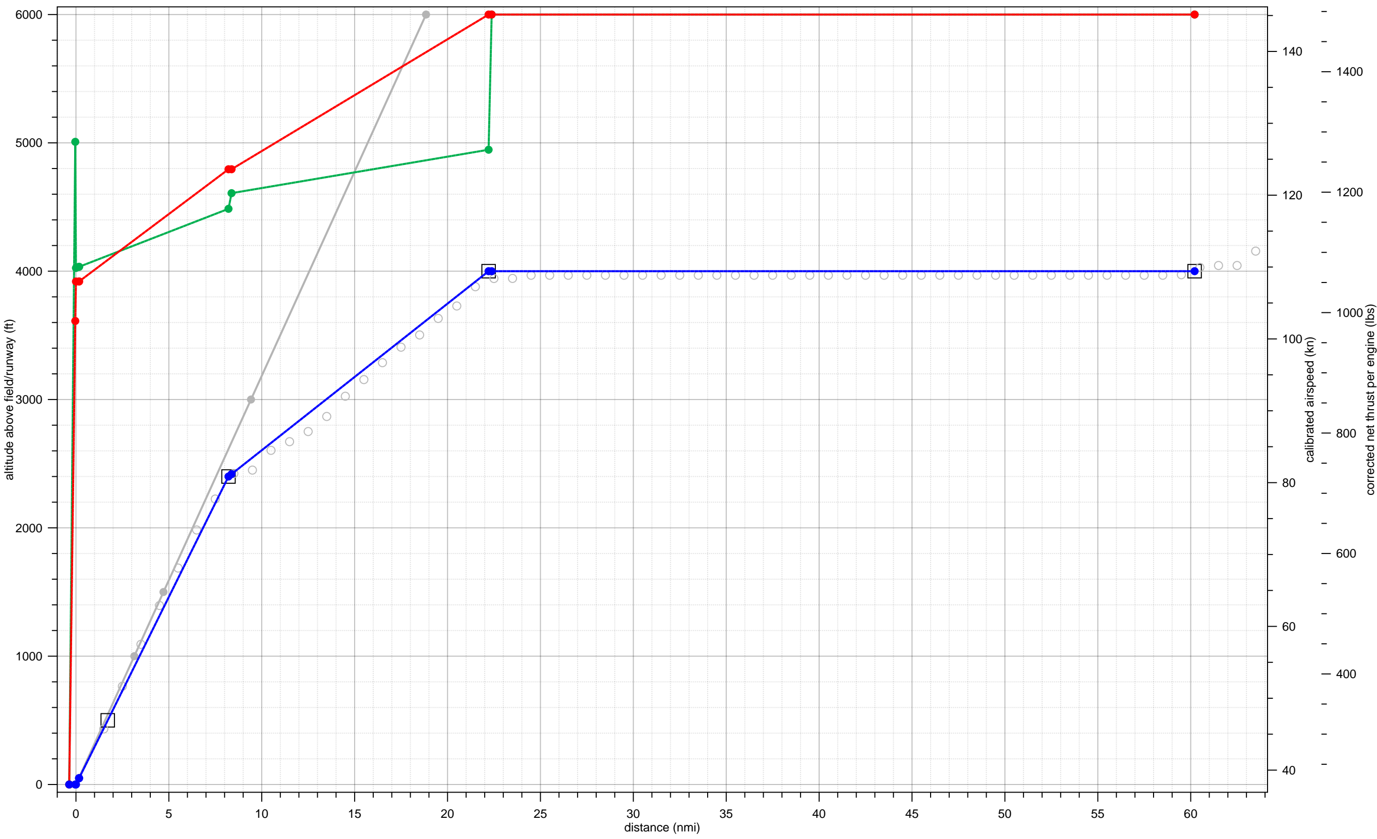
DHC830 fit to 15-A-DH8A-LT-1-4000-40to49-16to25
