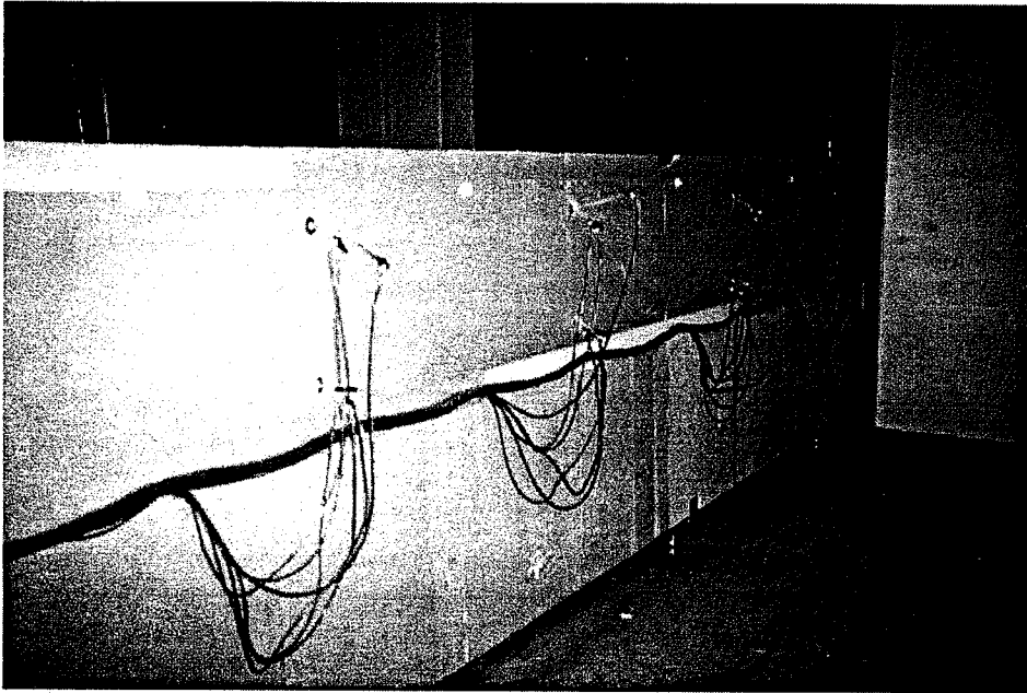
Figure 10. Photograph of test box with tensiometer tubes connected to pressure transducers exiting the side of the box.
