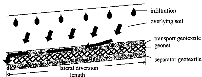
Figure 1. Schematic of Geocomposite Capillary Barrier Drain (GCBD) with overlying soil.
