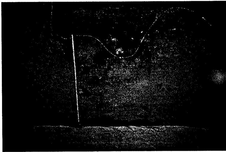
Figure 13. Photograph of the top of the geotextile separator removed from the control section. Staining with soil fines appears to indicate where significant amounts of water flowed through. The location of the crack in the asphalt is highlighted with the chalk line. The black edge suggests that no water migrated across the edges of the separator.
