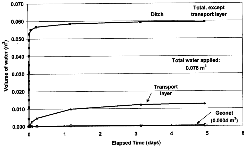
Figure 26. Outflow for one-hour storm with GCBD (Test 9).
