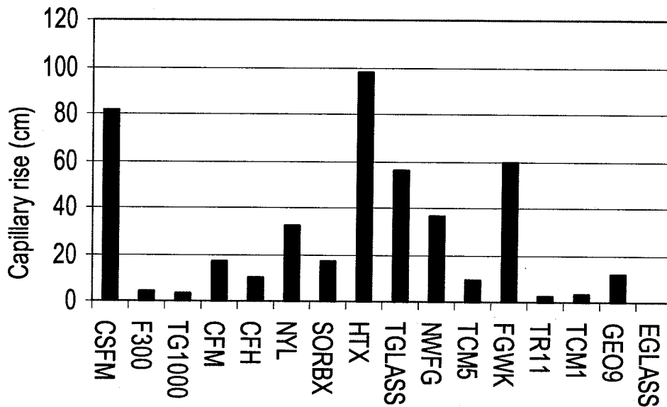
Figure 3. Forty-eight-hour capillary rise measurements.
