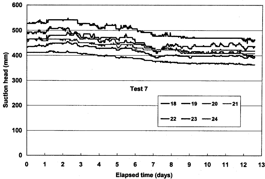
Figure 21. Soil suction heads in the base, 25 mm below the GCBD in a long-term infiltration test (Test 7).
