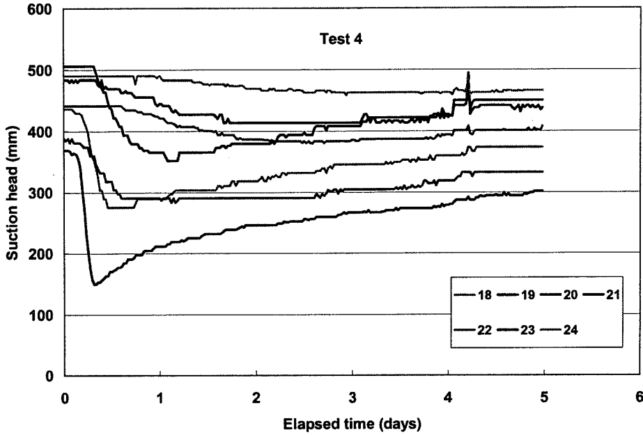
Figure 24. Soil suction heads in the subgrade at 25 mm below the geotextile separator in the control section for Test 4.
