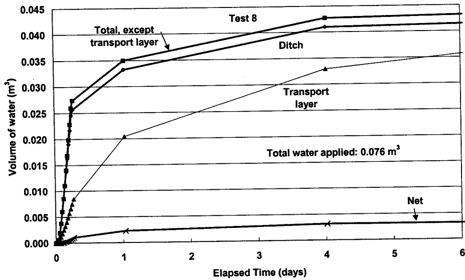
Figure 22. Outflow for six- hour storm in test section with GCBD (Test 8).
