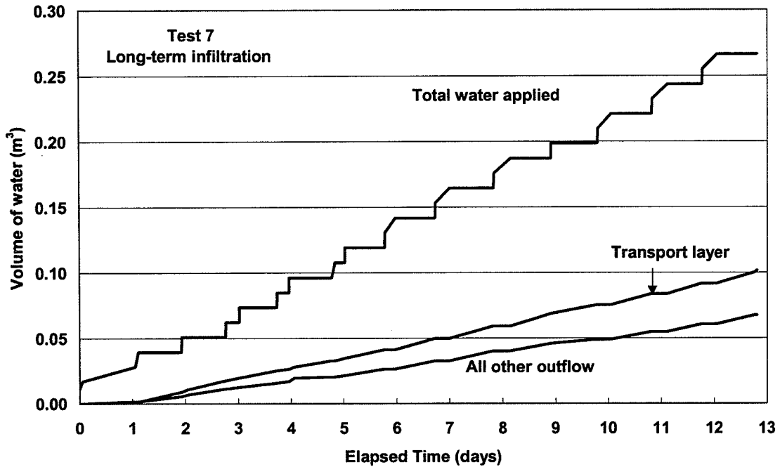
Figure 18. Outflow from long-term infiltration test with GCBD (Test 7).
