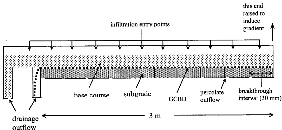
Figure 6. Lateral diversion test apparatus.
