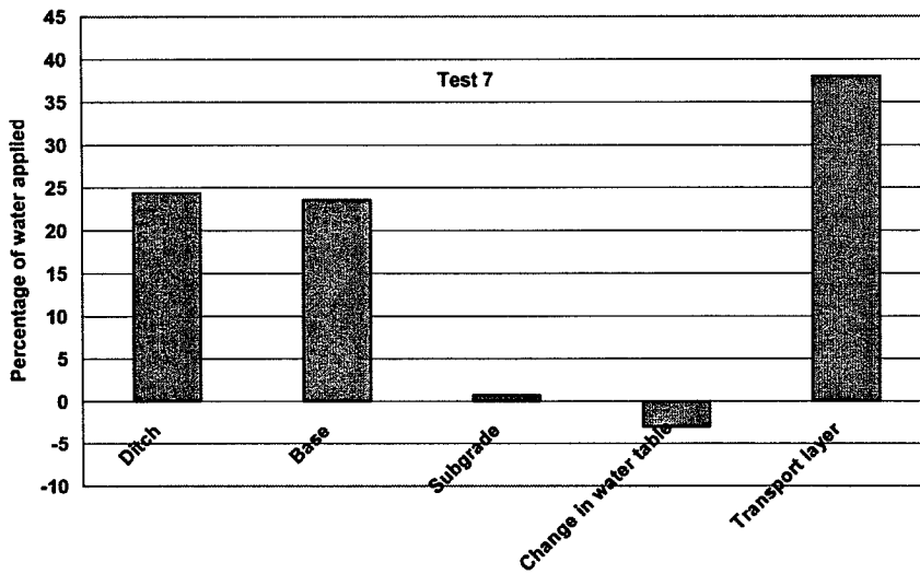
Figure 19. Percentage of water applied that was drained from the ditch, stored in the base and subgrade, in changing the elevation of the water table and drained from the transport layer in long-term infiltration with GCBD (Test 7).
