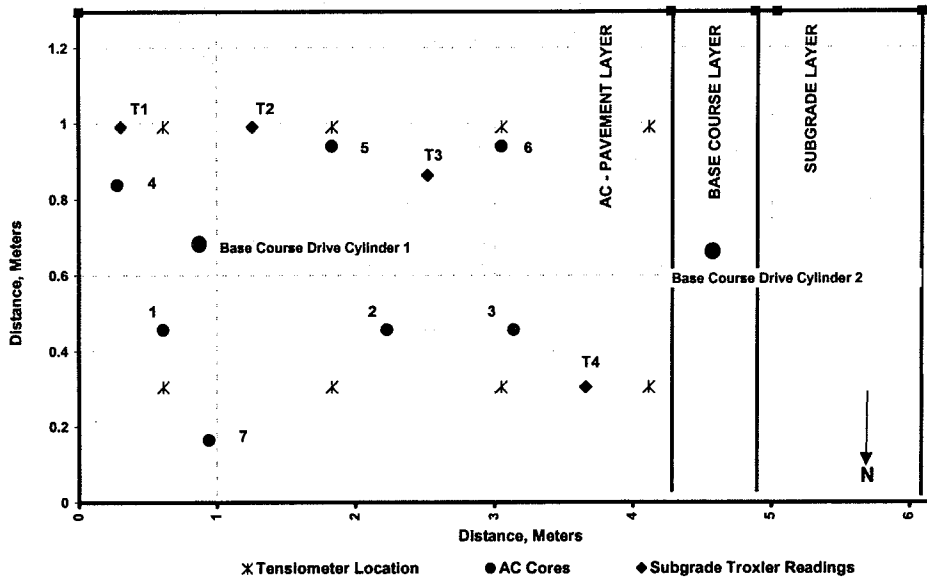
Figure 12. Plan view of test section showing locations of soil testing during deconstruction.
