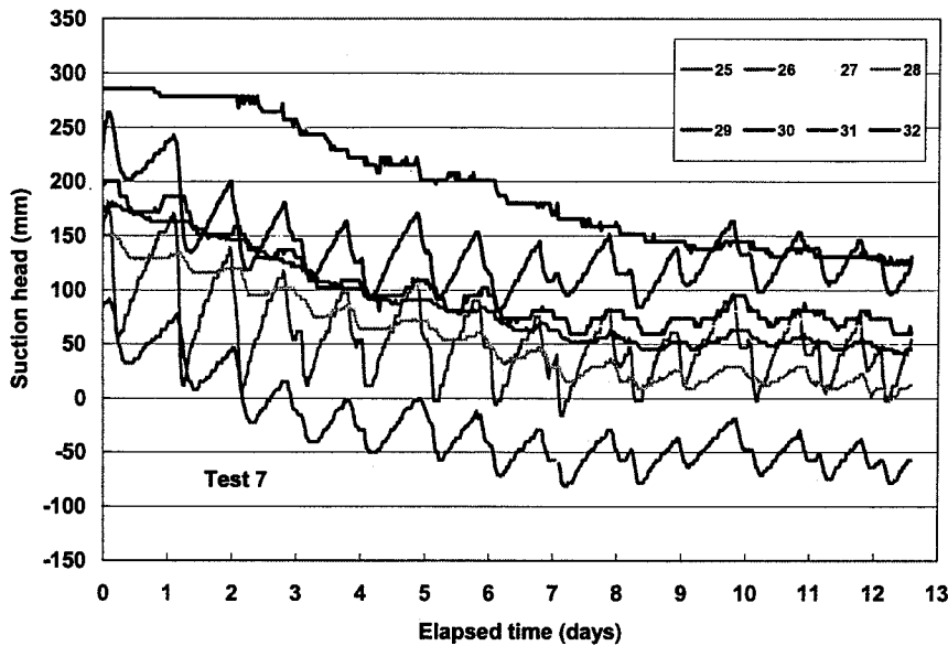
Figure 20. Soil suction heads in the base, 13 mm above the GCBD in a long-term infiltration test (Test 7).
