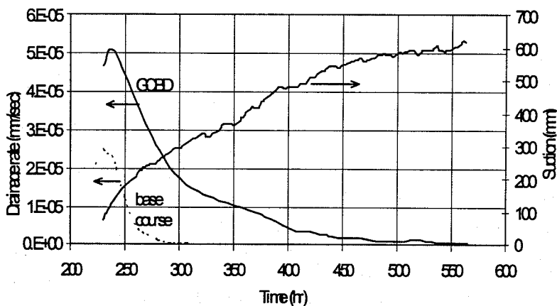
Figure 8. Drainage rate from GCB and overlying soil during period between constant rate infiltration and transient infiltration. The average suction in the overlying soil immediately above the GCB is also shown.
