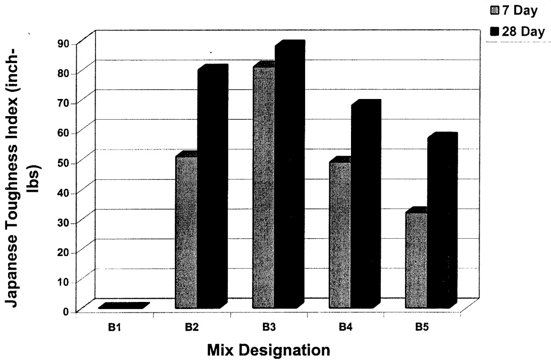
Fig. 4 Comparison of Japanese Toughness Index
