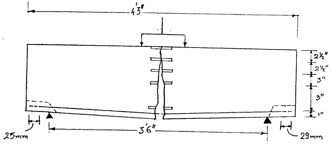
BEAM BRC-A
