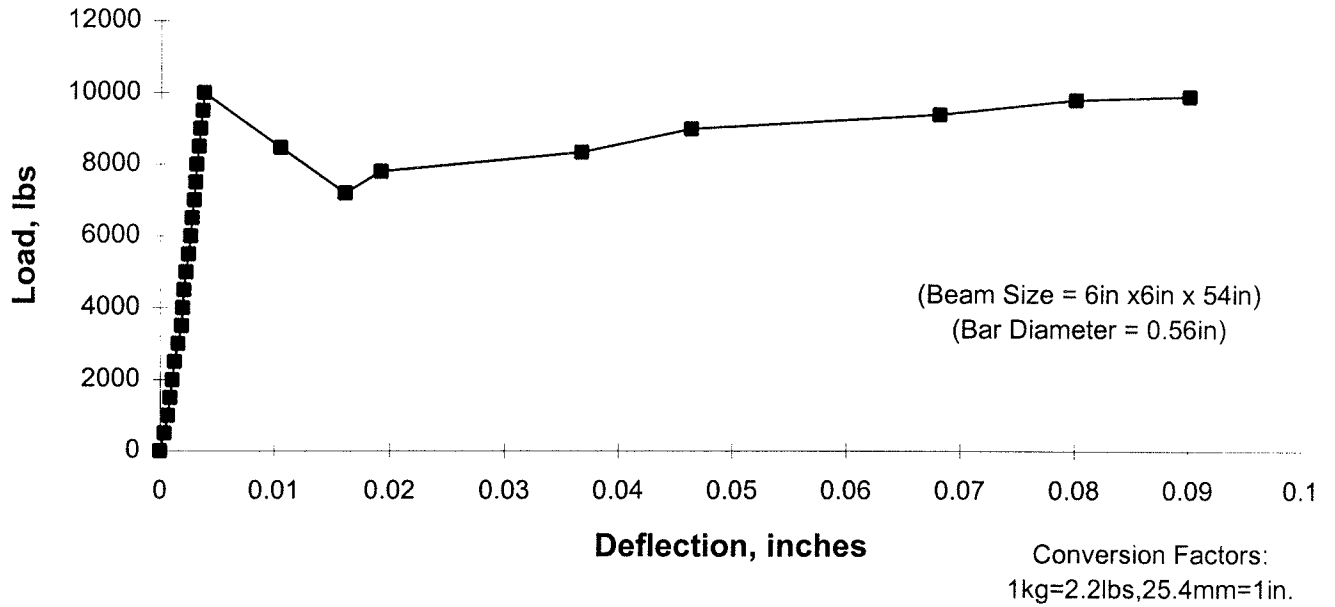
Fig. B5 LOAD DEFLECTION CURVE Sp:BRC-E
