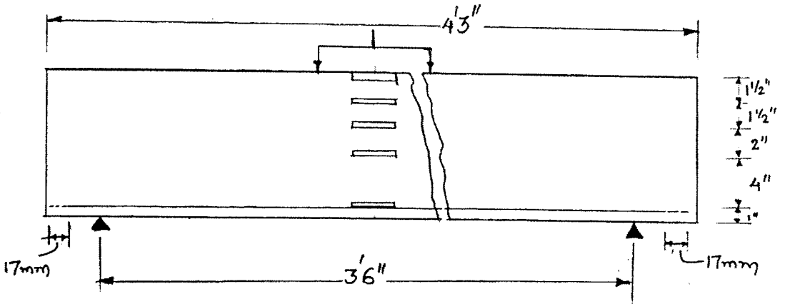
BEAM BRC-B
