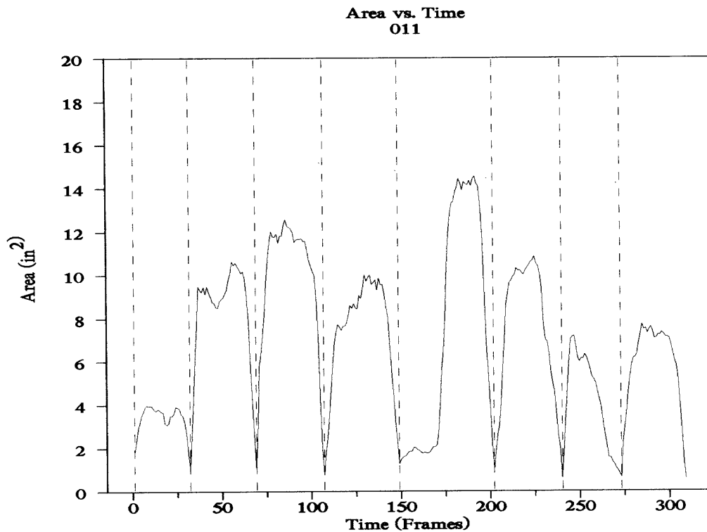
FIGURE 12 Total area under pressure separated by events.
