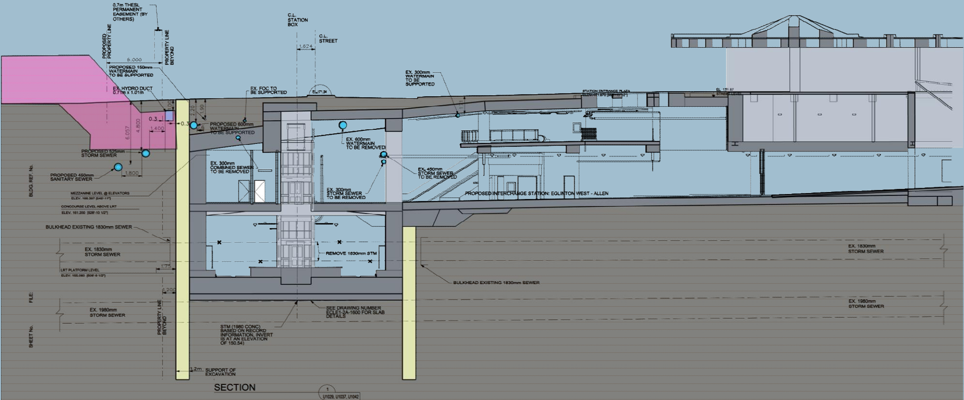
North South Section Through Subway Station
