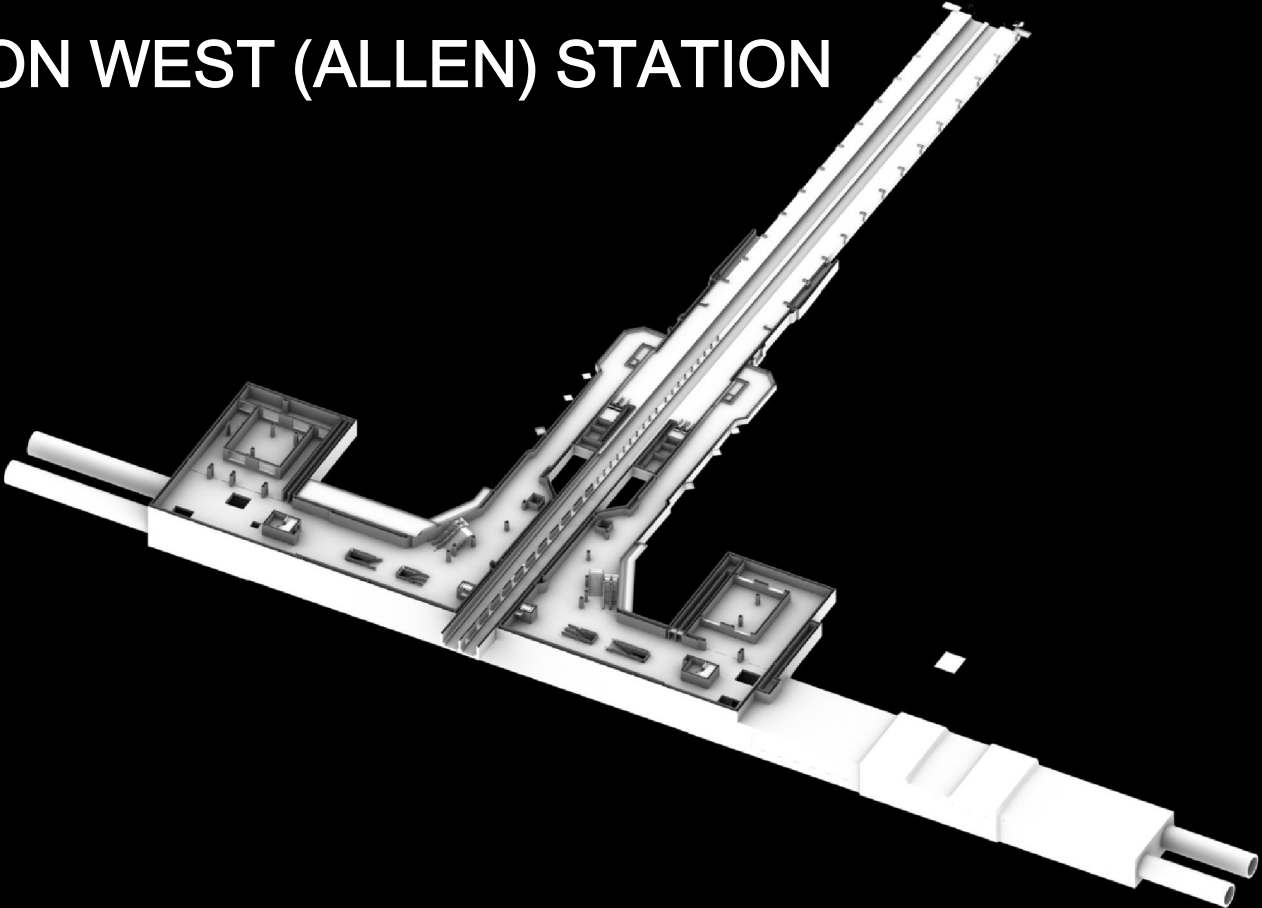
P3 Concepts LRT Lower Concourse | TTC Platform Level
