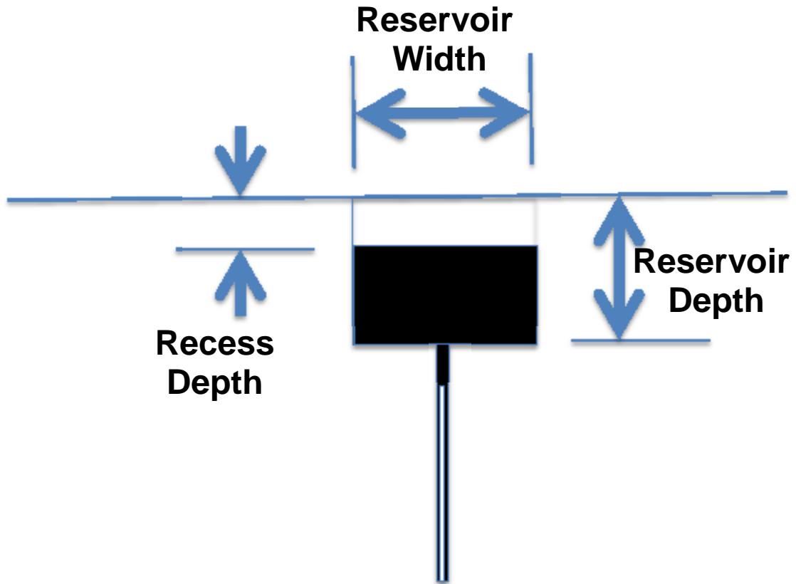
Graphic 3-1: Recessed Crack Treatment Configuration
