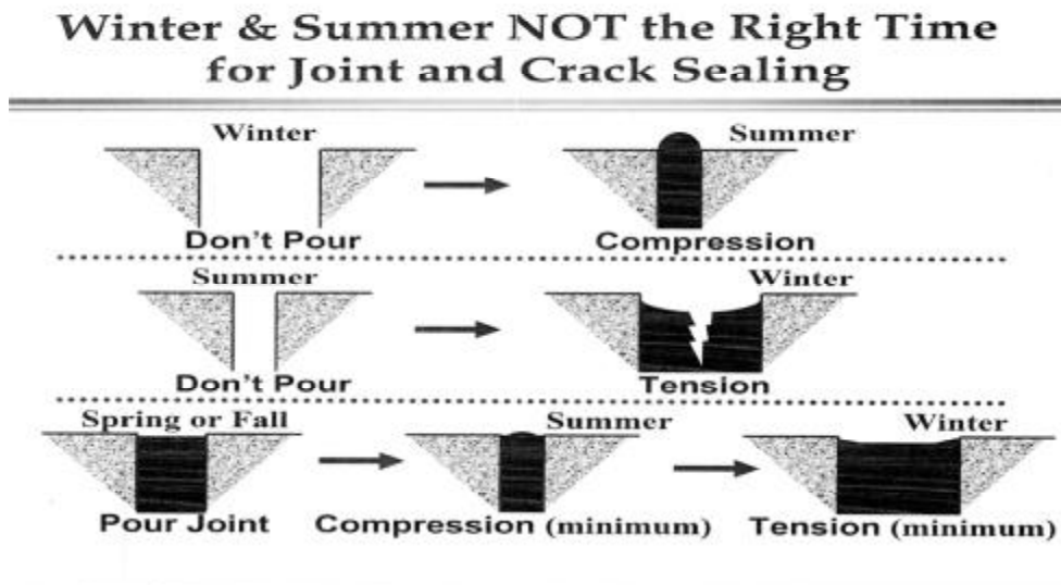
Graphic 4-5: Not the Right Time for Crack Treatment (SS-1)
