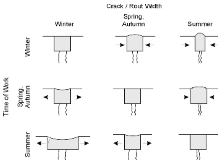
Graphic 2-2: Seasonal Impact on Sealing Operations (24)
