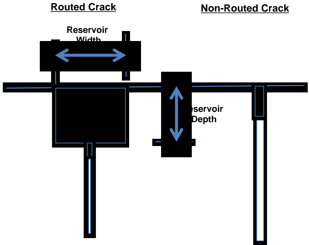
Graphic 3-2: Flush Fill Crack Treatment Configuration, Both Routed (A) and Non-Routed (B)
