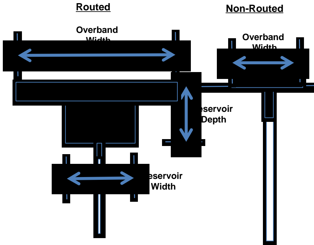
Graphic 4-3: Overband Crack Treatment Configuration
