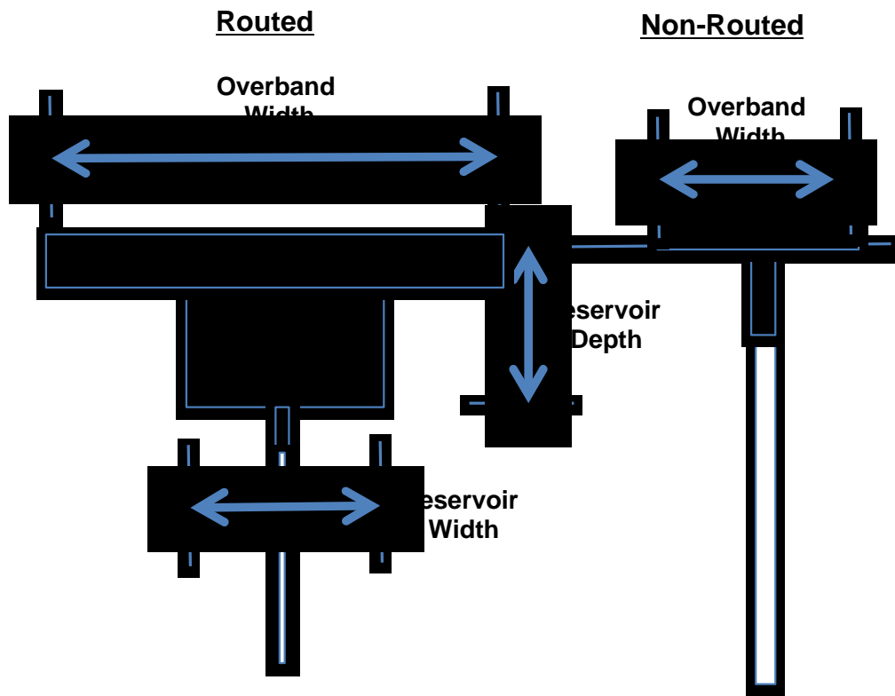
Graphic 2-6: Overband Crack Seal Configuration, Both Routed (A) and Non-Routed (B)
