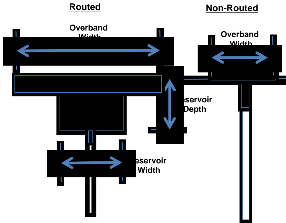
Graphic 3-3: Overband Crack Treatment Configuration, Both Routed (A) and Non-Routed (B)
