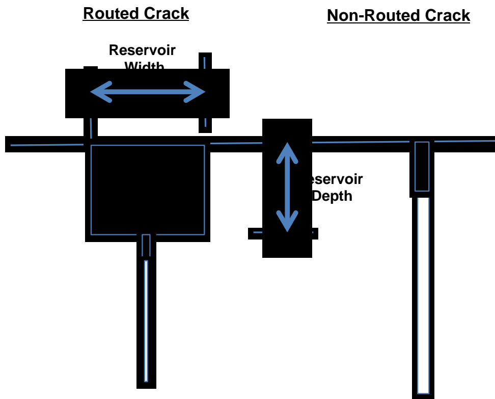
Graphic 4-2: Flush Fill Configurations
