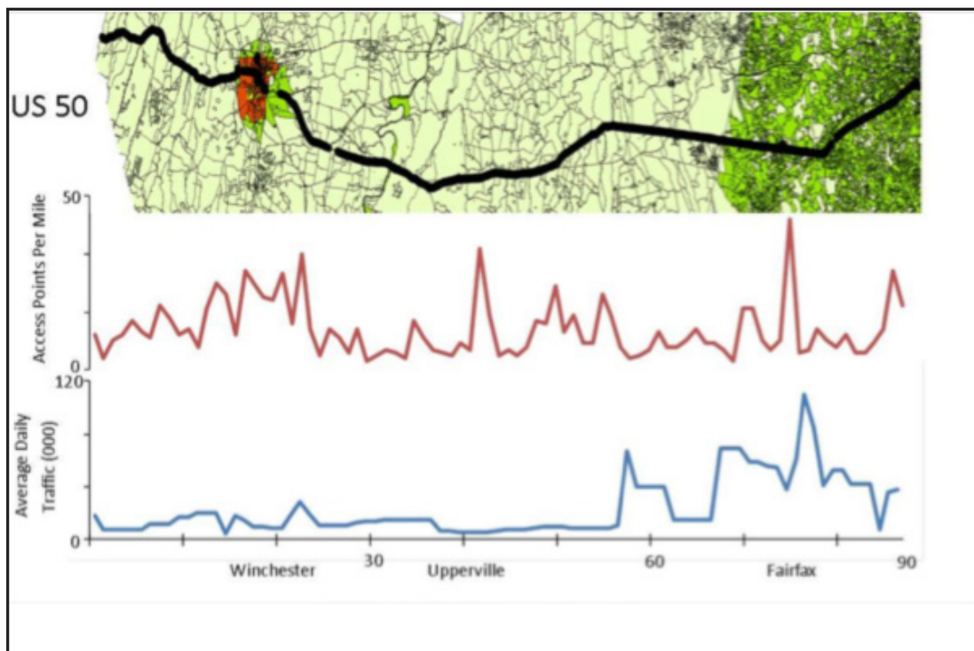
Figure 5.5 Risk-based prioritization of corridor segments based on relationships among access points per mile, risk of land development prediction, and average daily traffic (Source: VDOT, University of Virginia)
