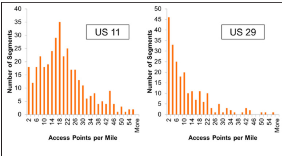
Figure F4 Cross-corridor comparison of transportation corridor access point density outliers using the Virginia ACPS tool (Source: VDOT and University of Virginia)
