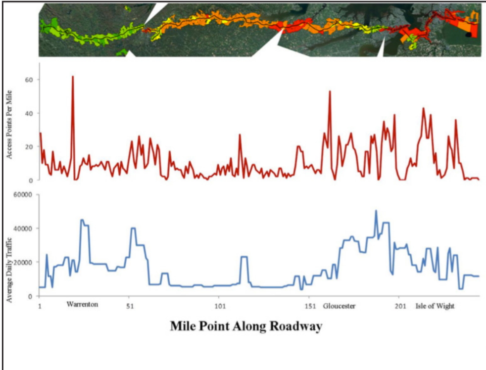
Figure F3 Risk-based prioritization of corridors vulnerable to land use based on Virginia ACPS output for the US 1 corridor (Source: VDOT and University of Virginia)
