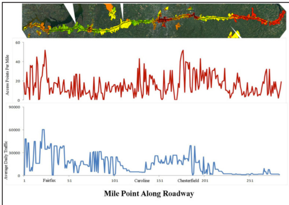
Figure F.2 Risk-based prioritization of corridors vulnerable to land use based on Virginia ACPS output for the US 1 corridor (Source: VDOT and University of Virginia)
