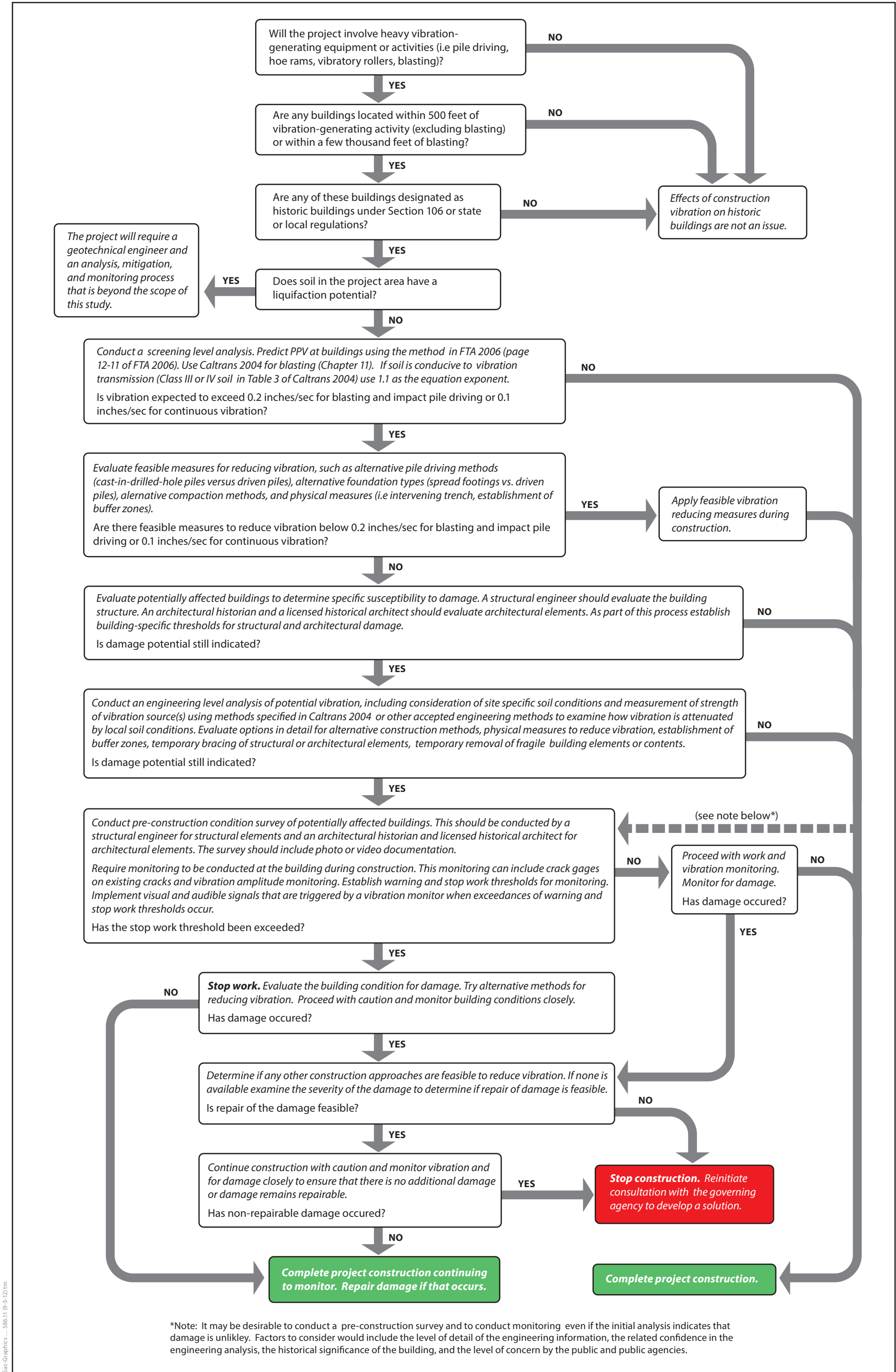
Figure C-1 Flow Chart for Recommended Approach for Addressing Construction Vibration Impacts on Historic Buildings
