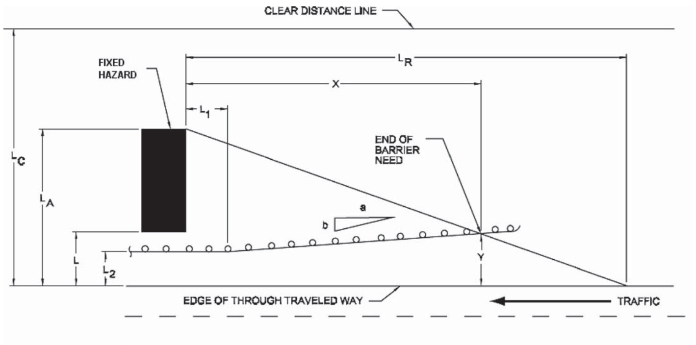
Figure 6. Barrier layout variables for point hazards.
