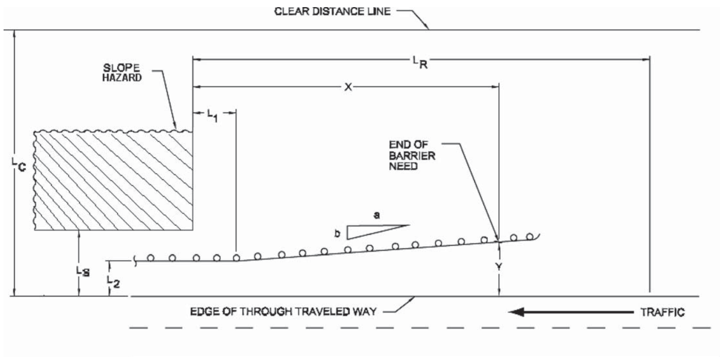
Figure 7. Barrier layout variables for slope hazards.
