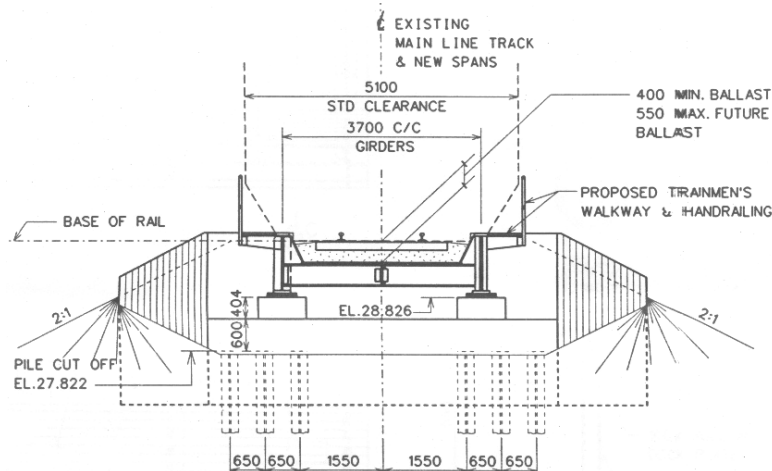
FIGURE 7 Through plate girder railway bridge deck.
