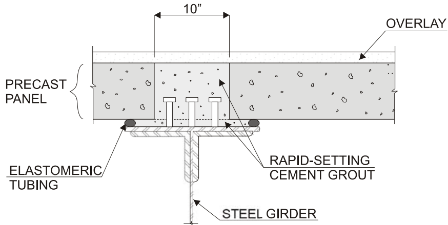
FIGURE 25 Regular shear stud blockout. [Source: Babaei et al. (1).]
