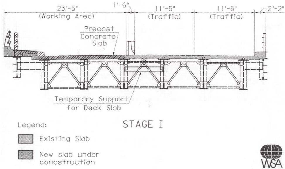
FIGURE 20 Cross section of bridge during first stage of slab replacement. [Source: Babaei et al. (1).]
