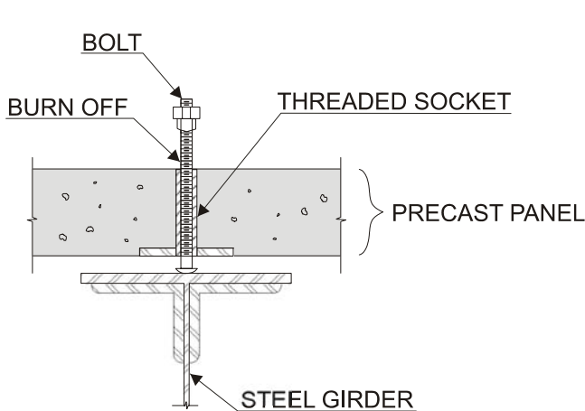
FIGURE 21 Leveling bolt system. [Source: Babaei et al. (1).]
