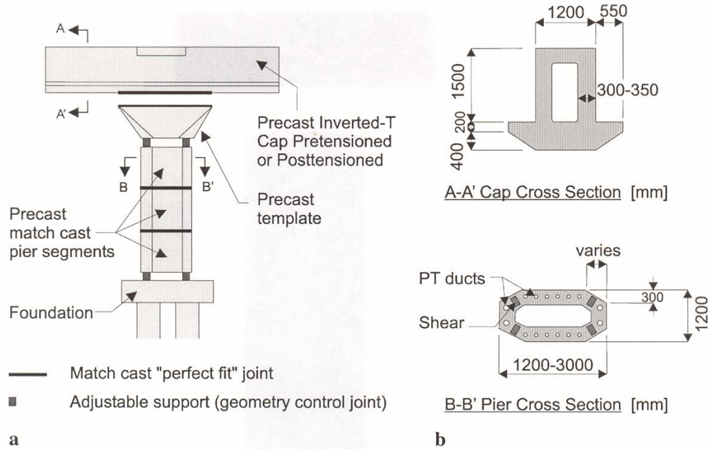
FIGURE 37 (a) Segmental pier system; (b) match-cast column segment, precast temple segment, inverted-T cap match cast, cap and pier cross sections. [Source: Billington et al. (21).]
