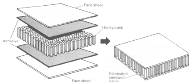
FIGURE 45 Sandwich construction.
