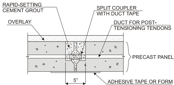
FIGURE 22 Posttensioning duct. [Source: Babaei et al. (1).]
