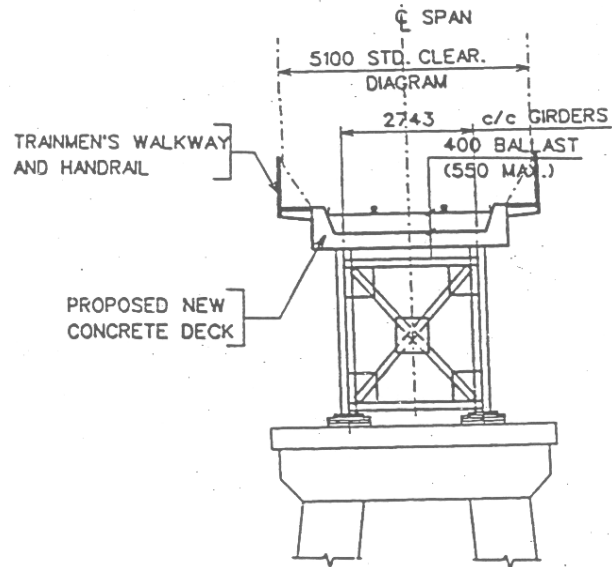
FIGURE 6 Steel deck plate girder railway bridge with prefabricated prestressed concrete slab.
