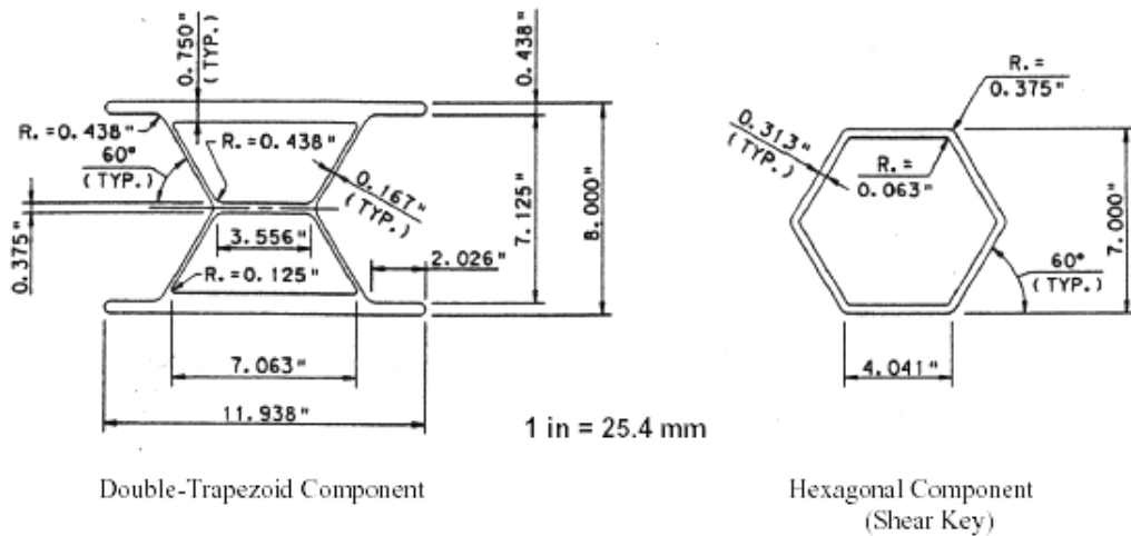
FIGURE 47 Cross section of composite bridge deck. [Source: Shekar et al. (34).]
