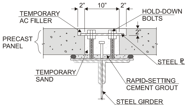
FIGURE 27 Temporary panel restraint for traffic. [Source: Babaei et al. (1).]
