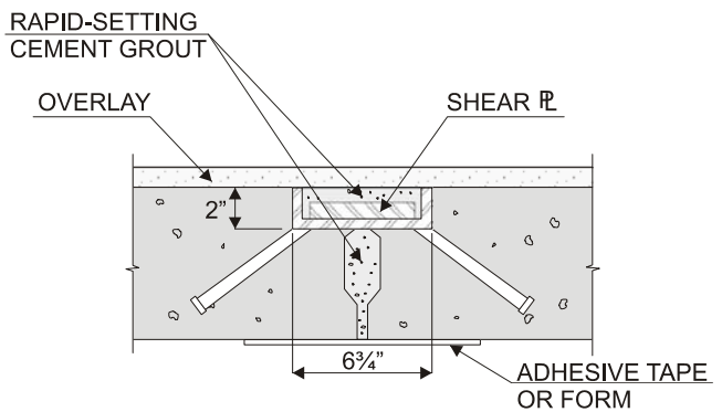
FIGURE 23 Welded sliding shear plates. [Source: Babaei et al. (1).]
