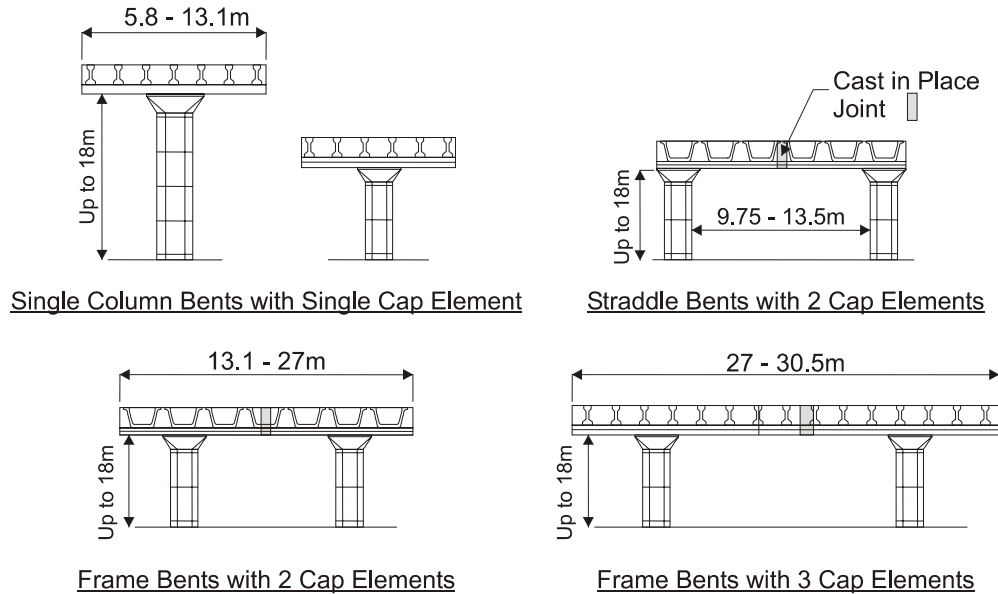
FIGURE 38 Different proposed bent types. [Source: Billington et al. (21).]
