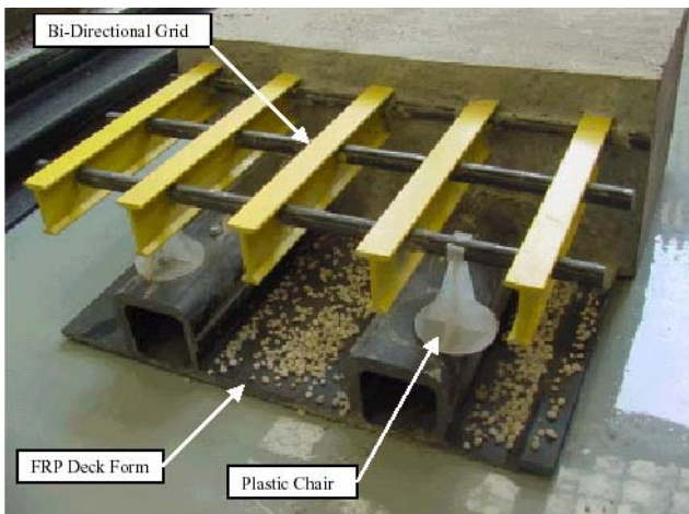
FIGURE 52 Mock-up of FRP reinforcement system. [Source: Dieter et al. (36).]
