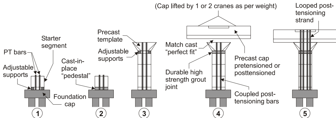
FIGURE 39 Erection sequence for a single-column bent. [Source: Billington et al. (21).]
