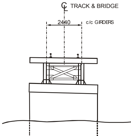
FIGURE 5 Open deck steel span railway bridge.
