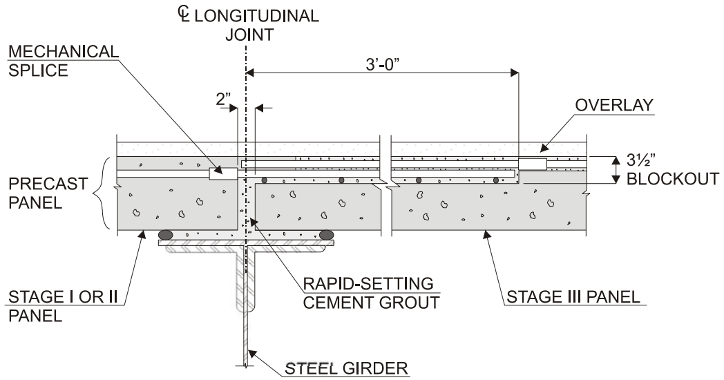
FIGURE 24 Longitudinal connections. [Source: Babaei et al. (1).]
