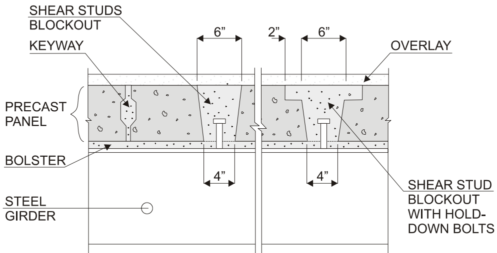
FIGURE 26 Longitudinal section, shear stud blockouts, and shear key. [Source: Babaei et al. (1).]
