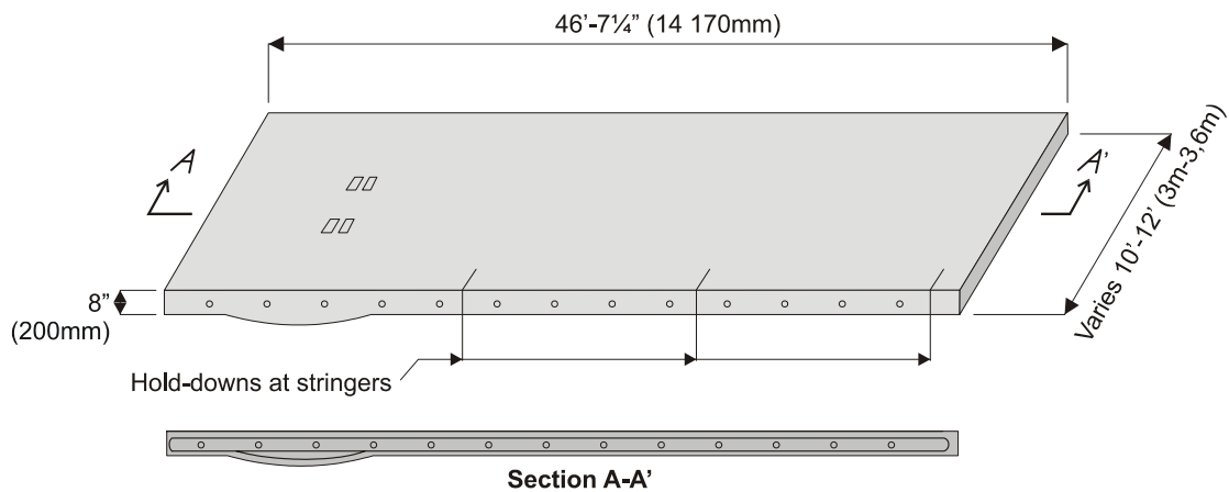
FIGURE 31 Prefabricated concrete deck panel.
