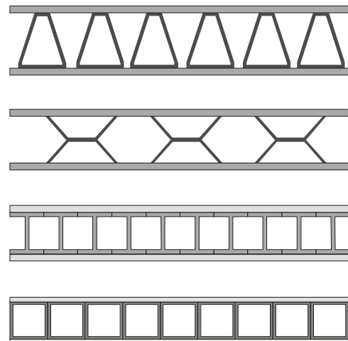
FIGURE 46 FRP decks produced from adhesive-bonded pultruded shapes.
