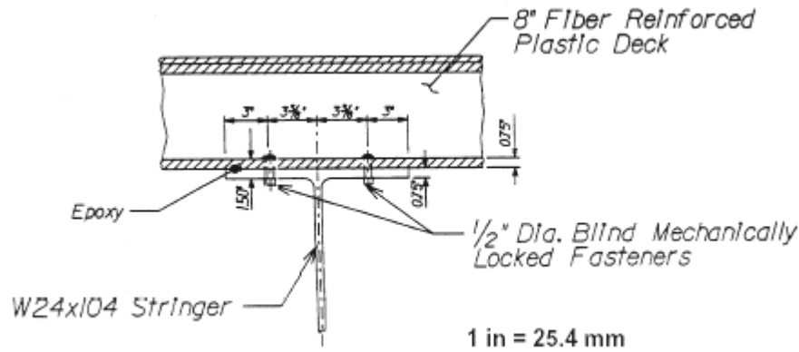
FIGURE 49 Deck to stringer connection using BOM blind bolts. [Source: Shekar et al. (34).]
