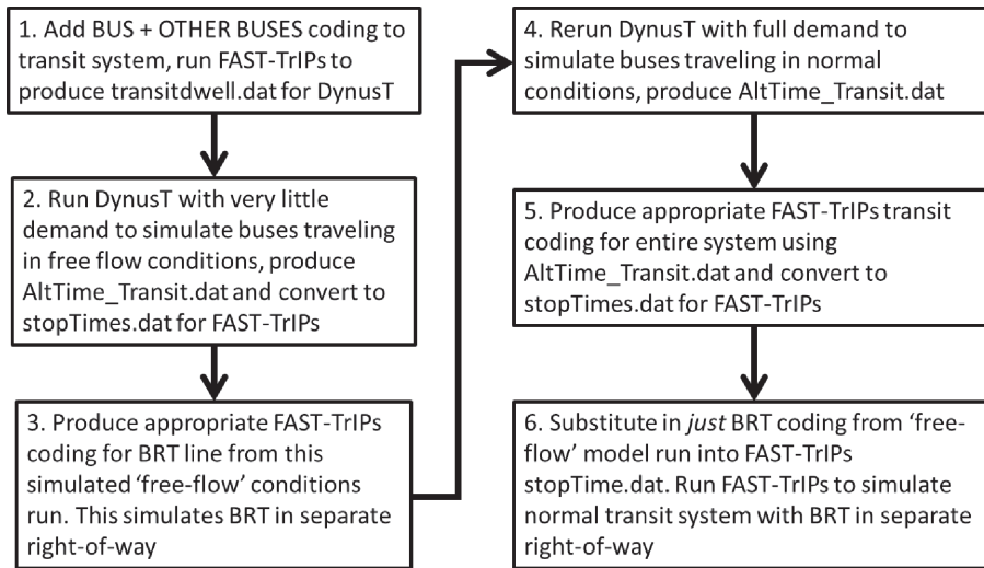
Figure 6.9. Scenario coding flowchart for Scenarios 4, 5, 7, and 8 (BRT in dedicated right-of-way).
