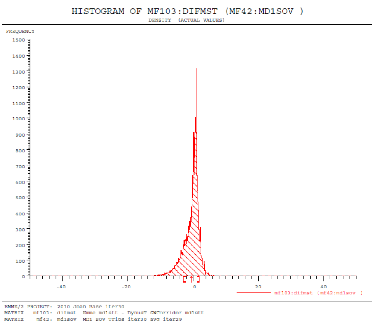
Figure 5.10. Difference in midday SOV automobile travel times for Southwest Corridor zone pairs (weighted by trips): mean = -0.4 min, standard deviation = 2.4 min.
