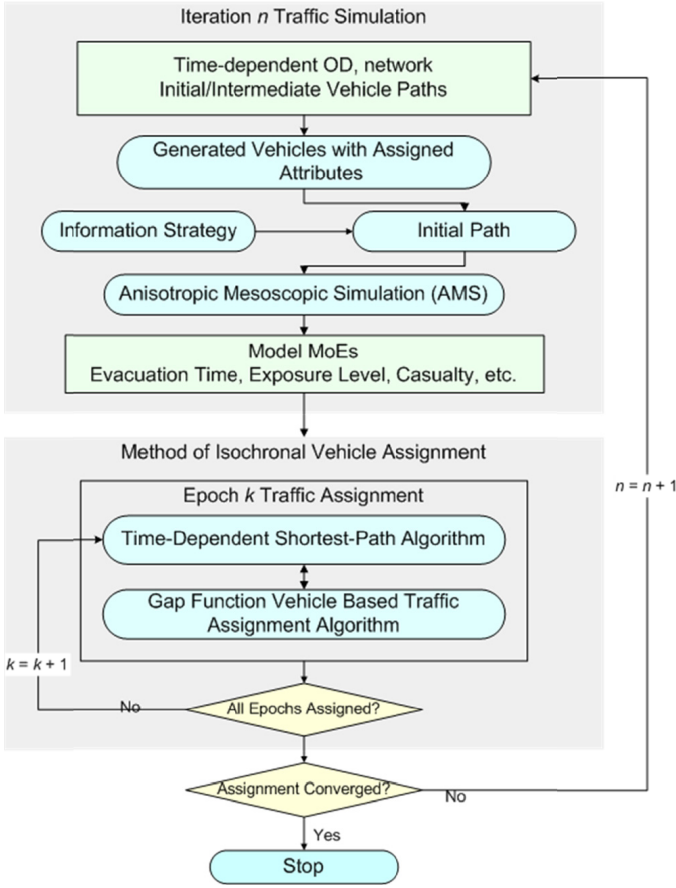
Figure 2.1. DynusT model algorithmic structure.
