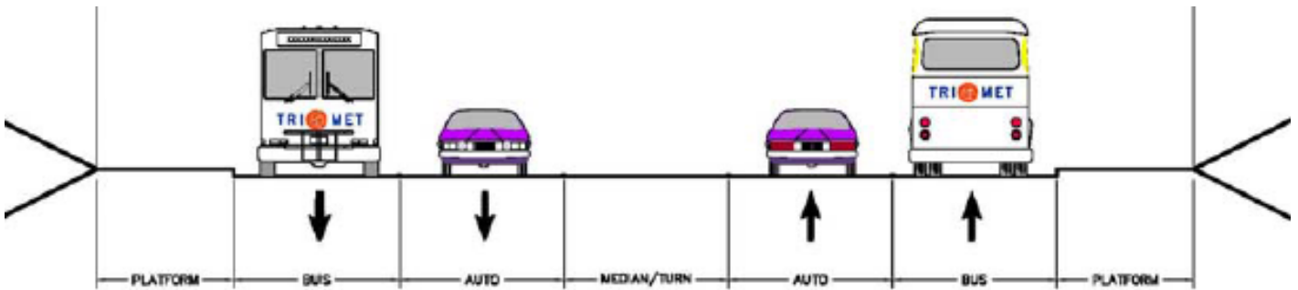
Figure 6.3. Cross sections of Scenarios 4 and 7.
