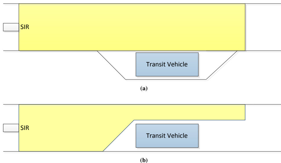
Figure 2.3. (a) SIR area with bus pullout and (b) SIR area without bus pullout.
