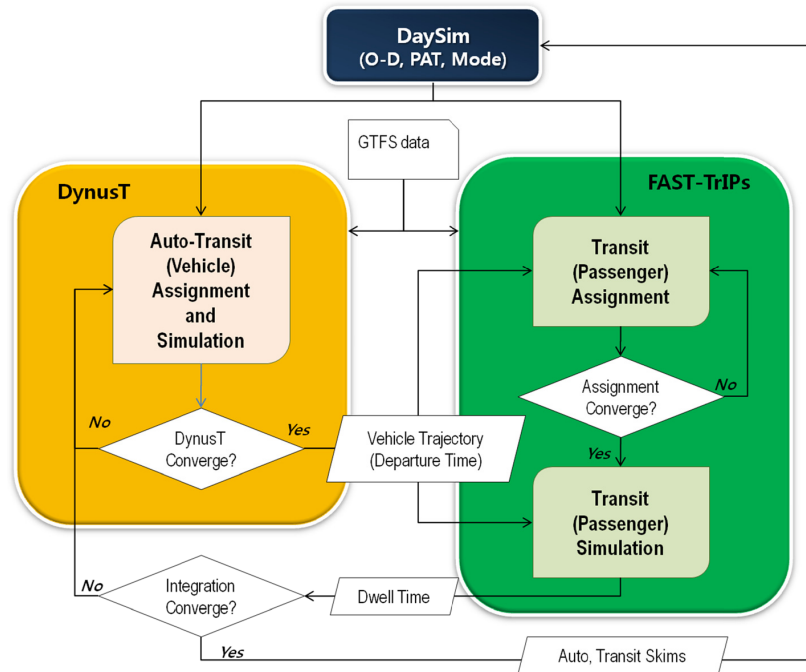
Figure 2.6. DynusT–FAST-TrIPs integration model considering the upper level activity-based model (DaySim is used as an example). PAT = preferred arrival time.
