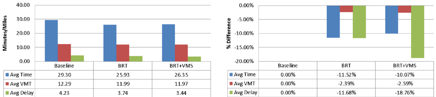
Figure 7.8. Southbound Barbur Boulevard measure of effectiveness (MoE) comparison—with reliability.
