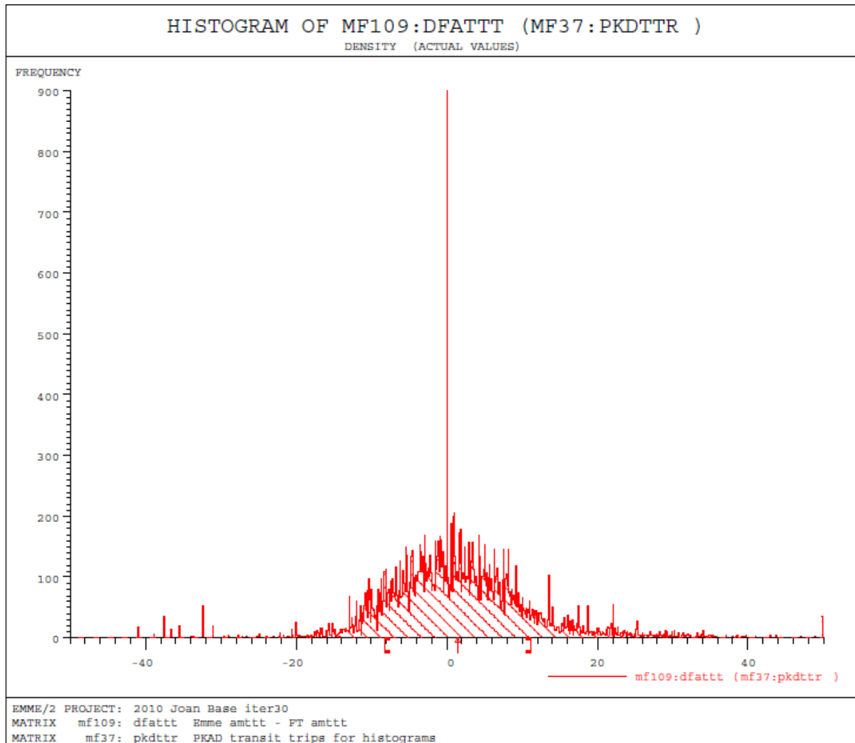
Figure 5.11. Difference in AM peak-period total transit travel times for Southwest Corridor zone pairs (weighted by trips): mean = 1.4 min, standard deviation = 9.7 min.
