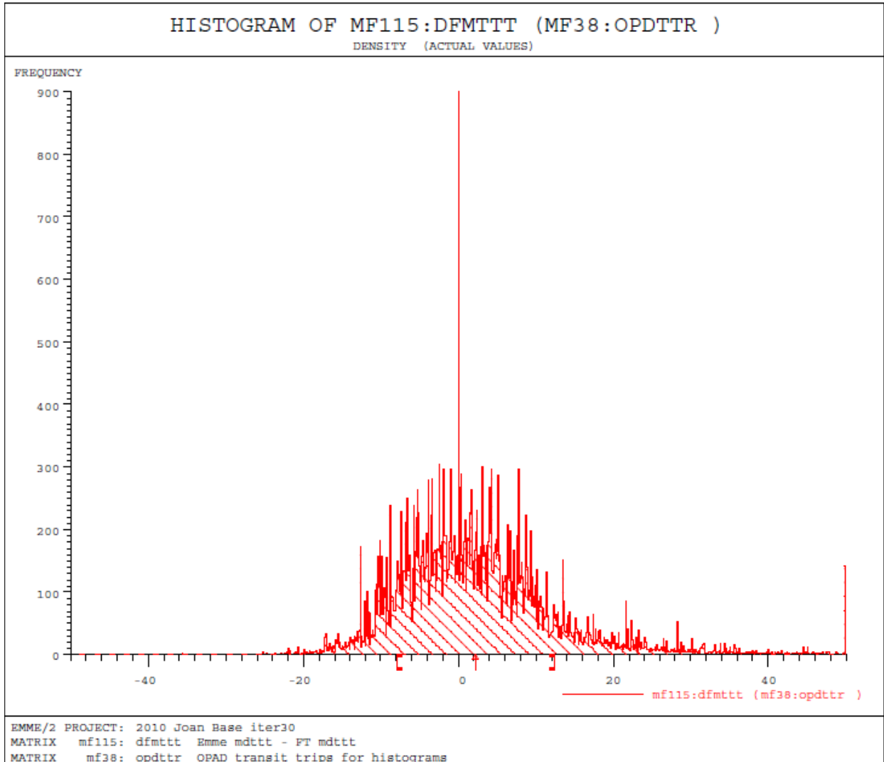
Figure 5.12. Difference in midday total transit travel times for Southwest Corridor zone pairs (weighted by trips): mean = 2.2 min, standard deviation = 10 min.
