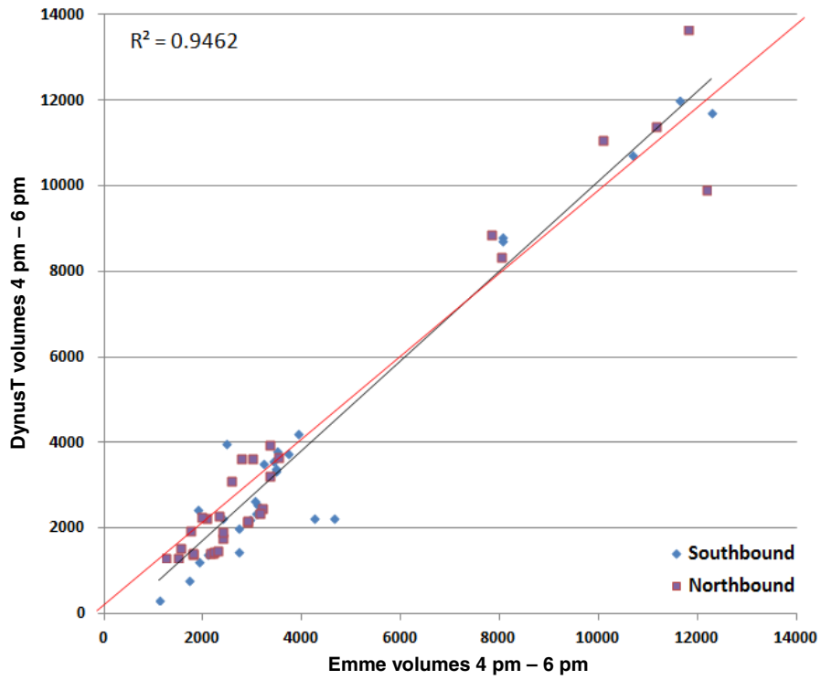
Figure 5.2. Improved 4 p.m. to 6 p.m. volume comparison between DynusT and Emme.
