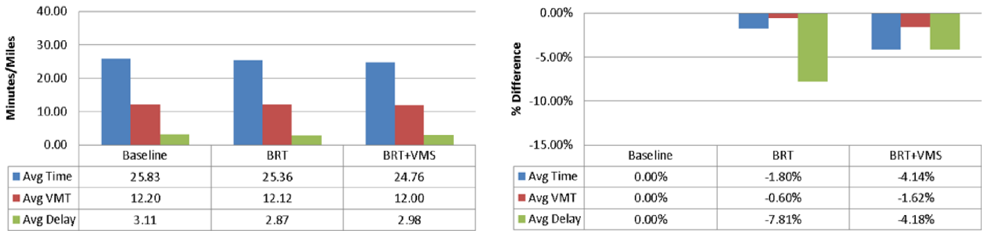
Figure 7.7. Southbound Barbur Boulevard measure of effectiveness (MoE) comparison—without reliability.
