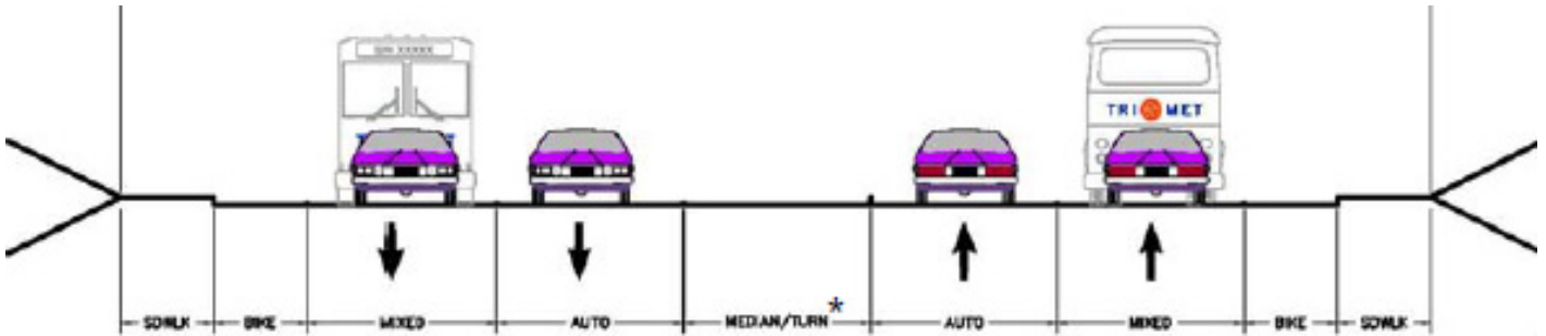
Figure 6.2. Cross sections of Scenarios 1, 2, 3, and 6.
