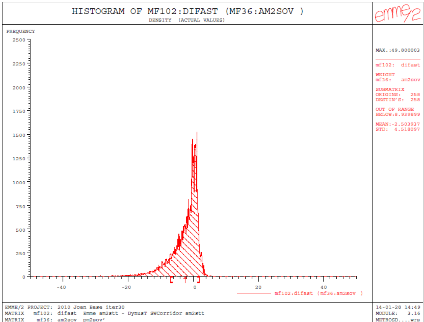
Figure 5.9. Difference in AM peak-period SOV automobile travel times for Southwest Corridor zone pairs (weighted by trips): mean = -2.5 min, standard deviation = 4.5 min.
