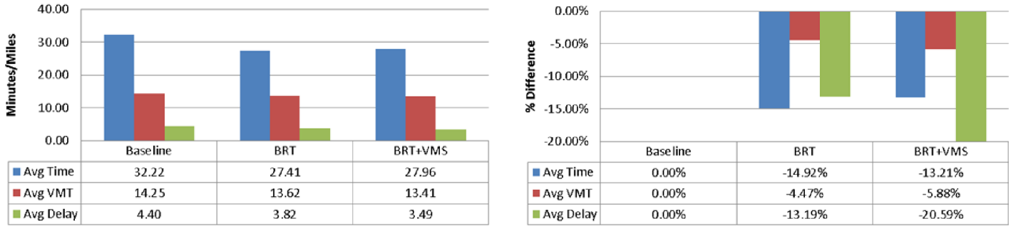
Figure 7.10. Southbound I-5 corridor measure of effectiveness (MoE) comparison – with reliability.
