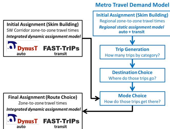
Figure 6.10. Feedback framework.
