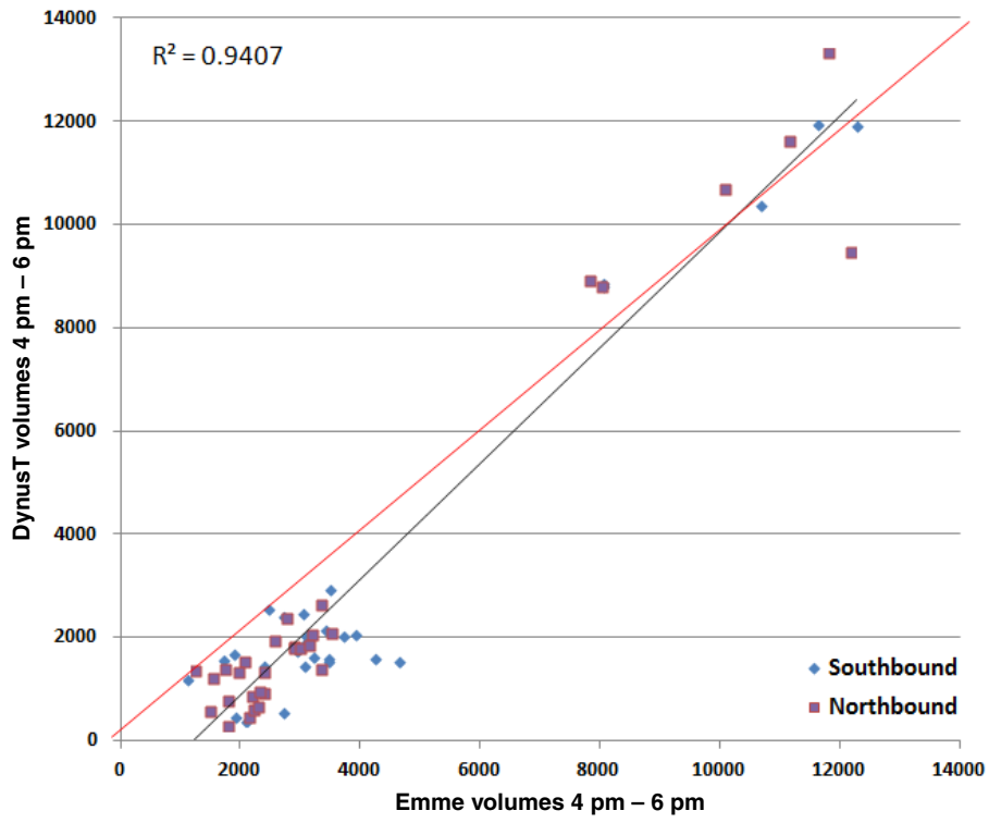
Figure 5.1. Comparison of 4 p.m. to 6 p.m. volumes between DynusT and Emme.
