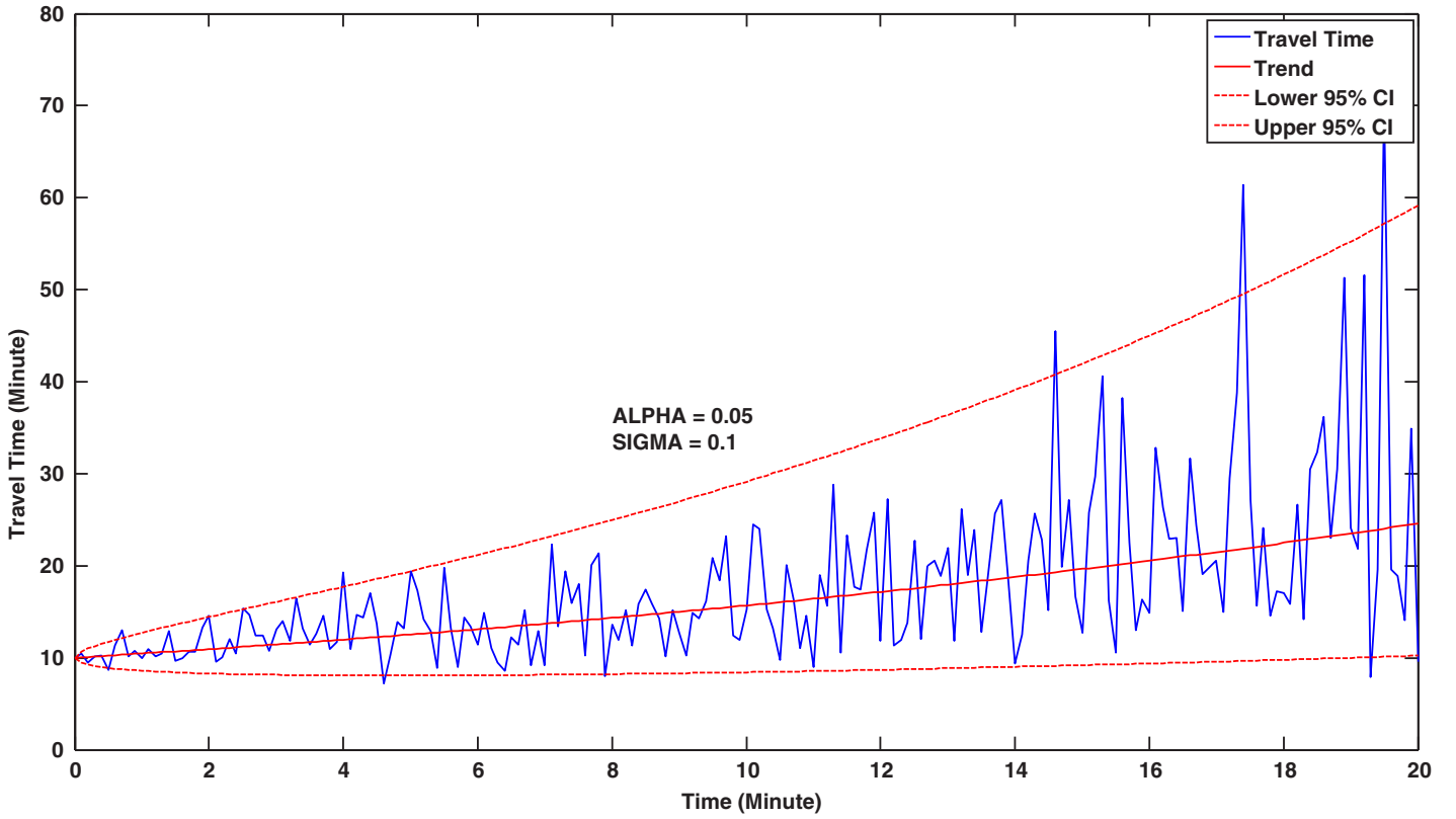
Figure 7.2. Sample travel time evolution path simulated as geometric Brownian motion (GBM) process.
