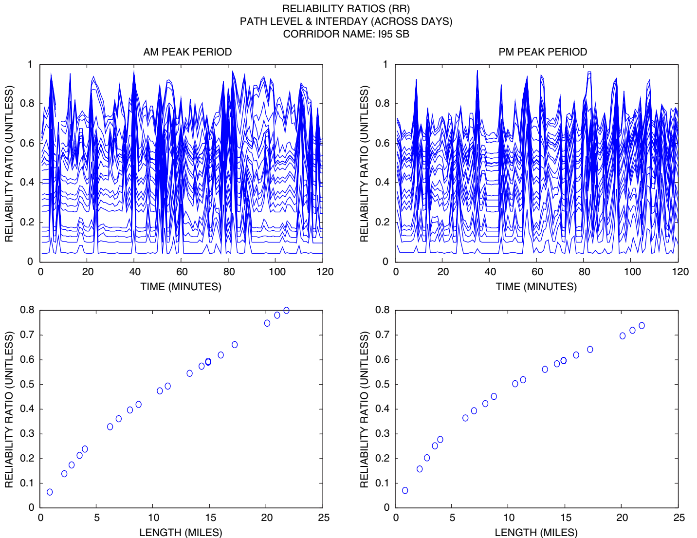
Figure E.6. Analysis results on southbound I-95 corridor: left, AM peak period; right, PM peak period; top, reliability ratio over time; and bottom, average reliability ratio versus length.
