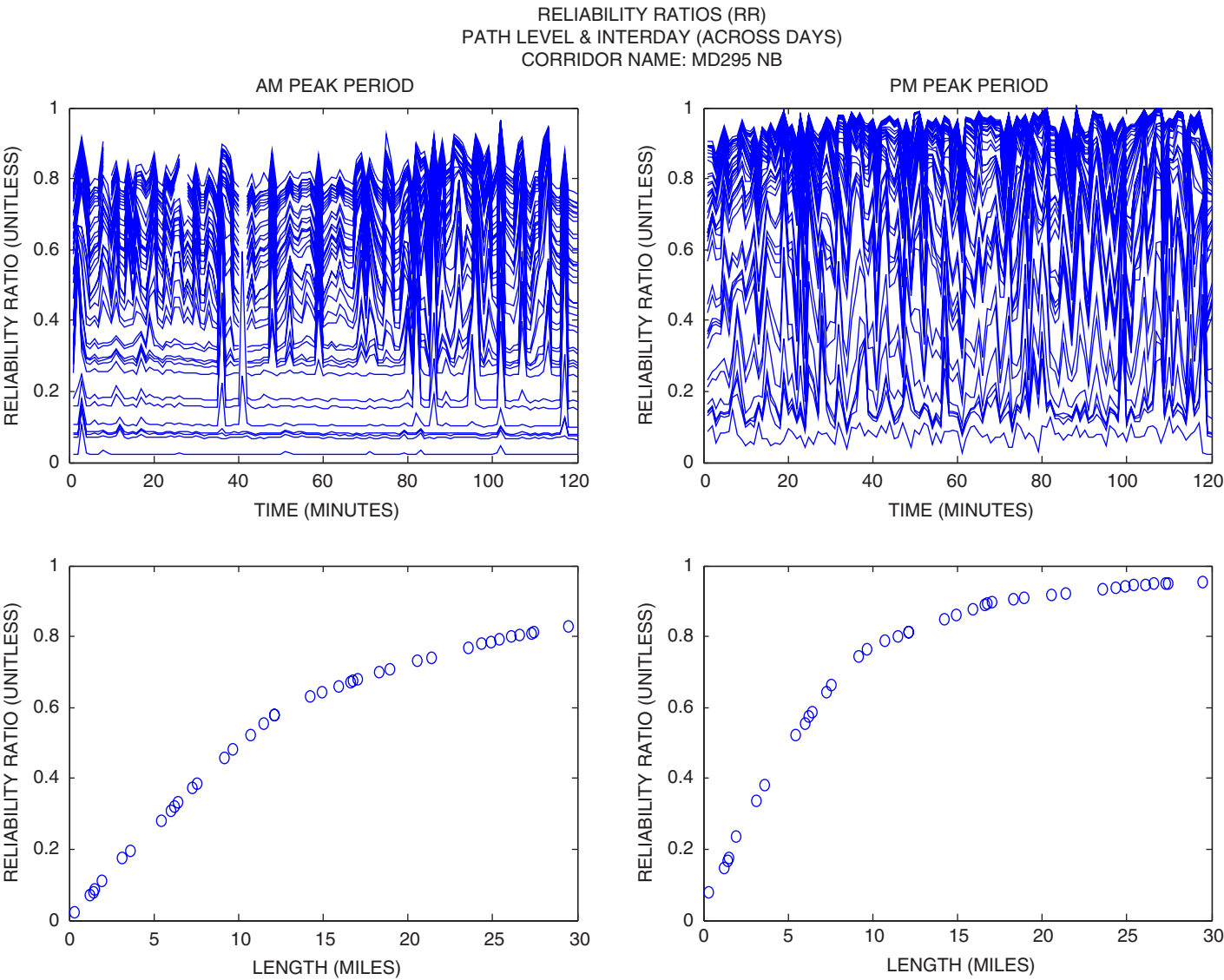
Figure E.21. Analysis results on northbound MD-295 corridor: left, AM peak period; right, PM peak period; top, reliability ratio over time; and bottom, average reliability ratio versus length.
