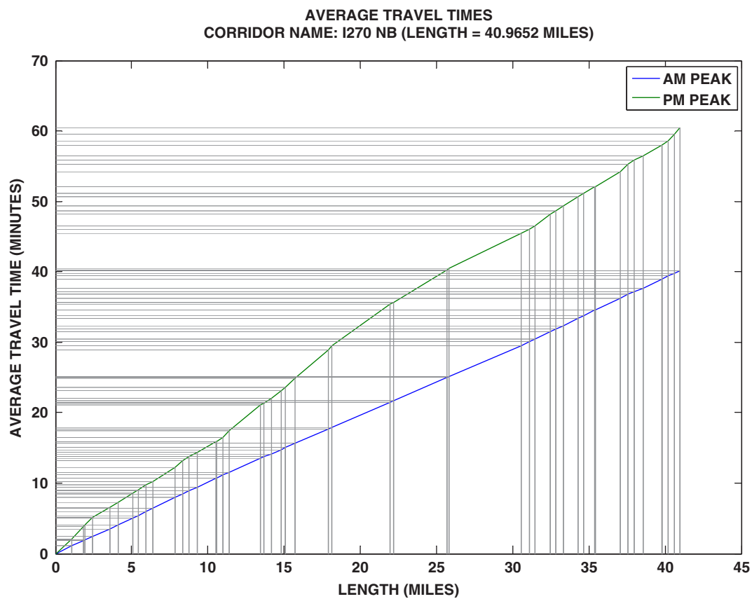
Figure E.7. Average travel time versus length on northbound I-270 corridor.
