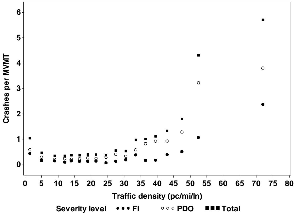
Figure 3.5. Crash Rate vs. Traffic Density for Work Zone Periods in Sacramento
