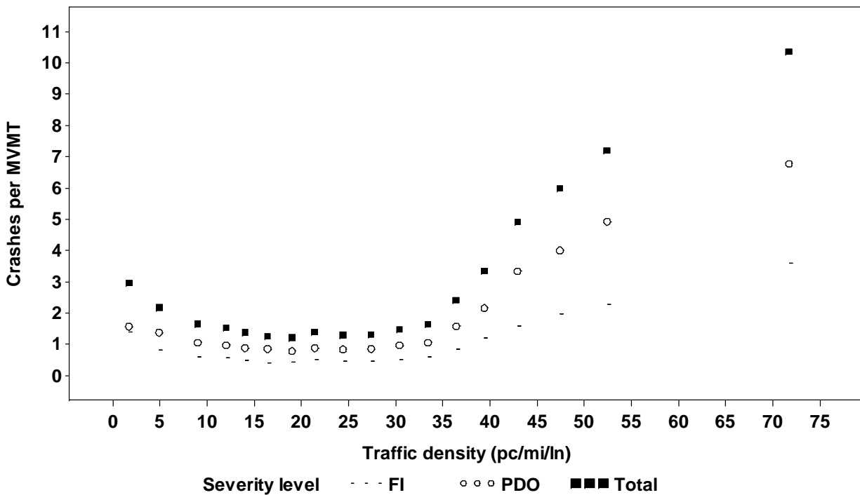
Figure 2.1. Total, FI, and PDO Crash Rates vs. Traffic Density for Directional Freeway Segments in the Seattle Metropolitan Area
