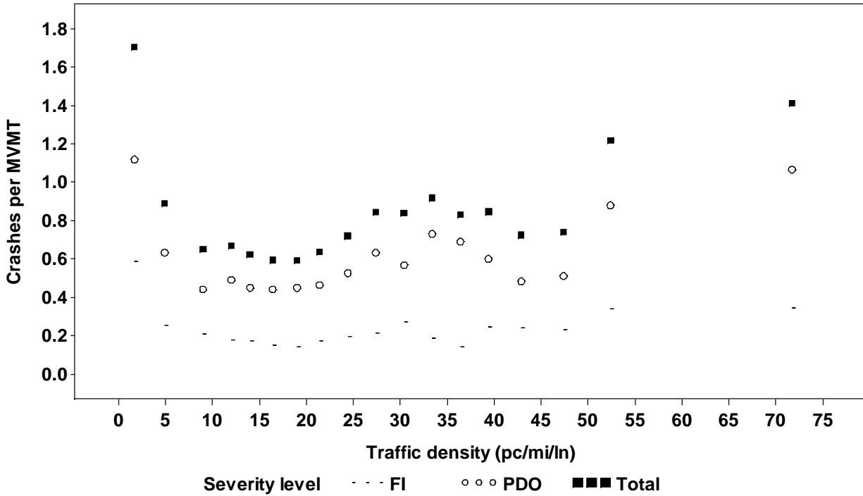
Figure 2.2. Total, FI, and PDO Crash Rates vs. Traffic Density for Directional Freeway Segments in the Minneapolis-St. Paul Metropolitan Area
