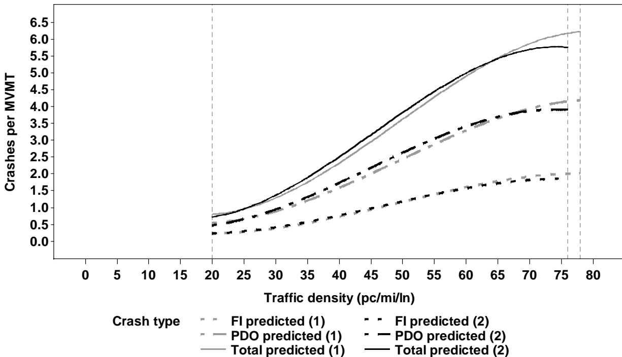
Figure 3.2. Predicted Total, FI, and PDO Crash Rates vs. Traffic Density (1 = Seattle and Minneapolis-St. Paul Areas Combined) (2 = Seattle, Minneapolis-St. Paul, and Sacramento, Areas Combined)
