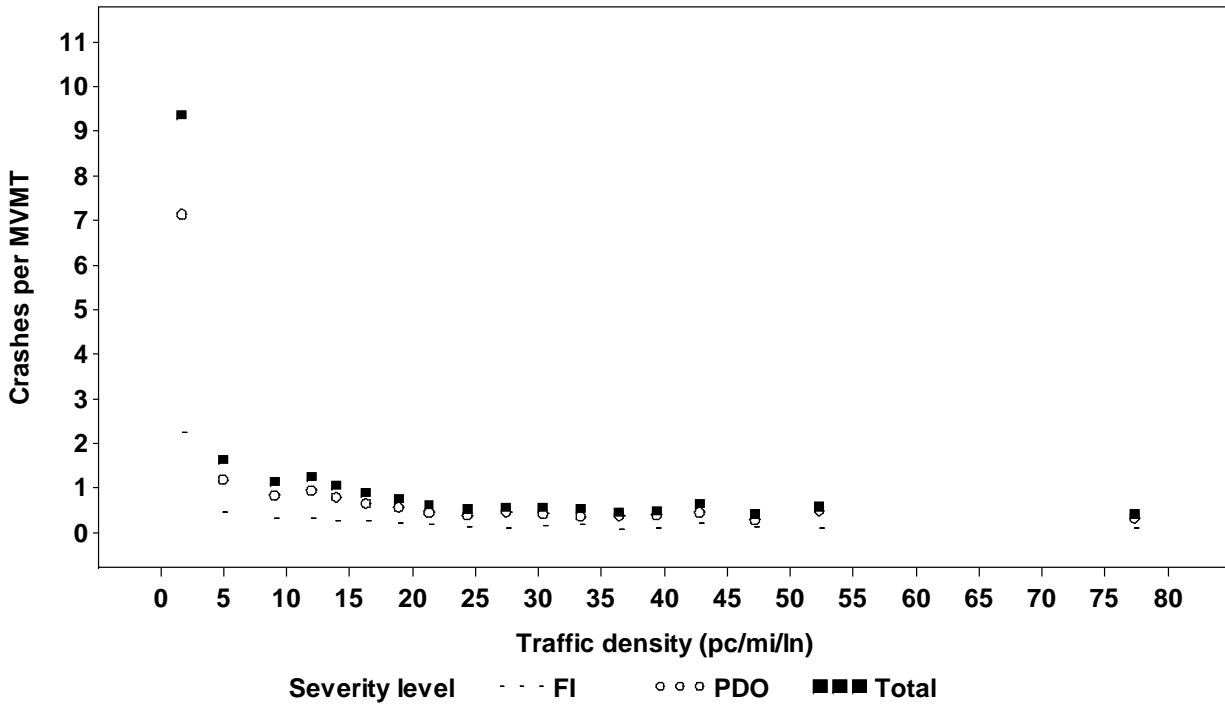
Figure 2.5. Total, FI, and PDO Crash Rates vs. Traffic Density for Directional Freeway Segments in the Missouri Portion of the Kansas City Metropolitan Area
