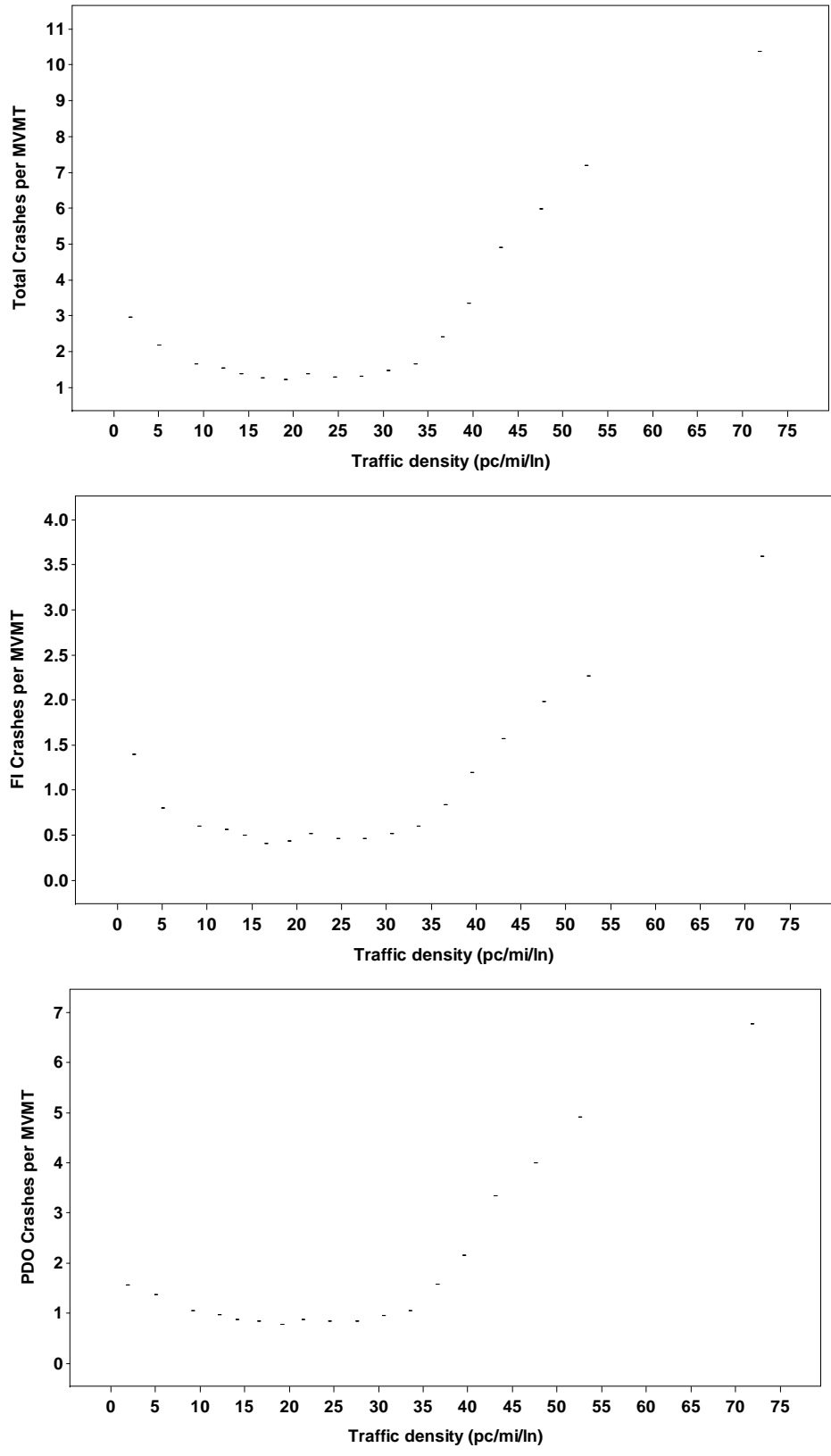
Figure 1.2. Observed Total, FI, and PDO Crash Rates vs. Traffic Density for Freeways in the Seattle Area
