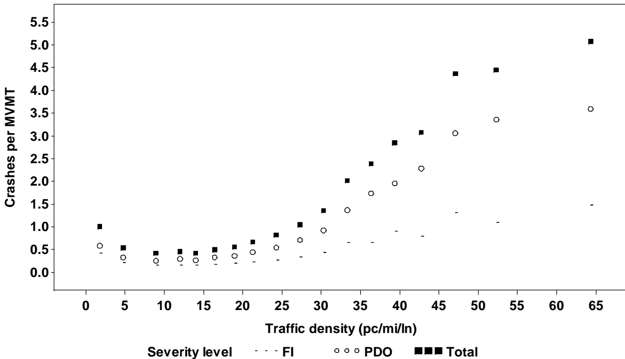
Figure 2.3. Total, FI, and PDO Crash Rates vs. Traffic Density for Directional Freeway Segments in the Sacramento Metropolitan Area
