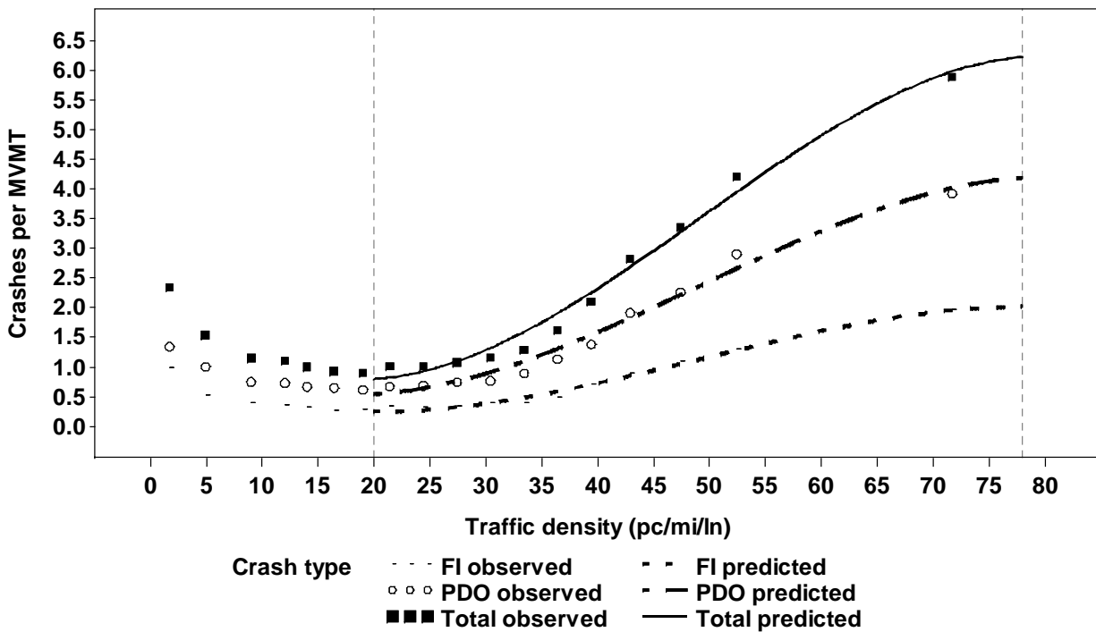
Figure 1.1. Observed and Predicted Total, FI, and PDO Crash Rates vs. Traffic Density for Seattle and Minneapolis-St. Paul Metropolitan Areas Combined (1,4)
