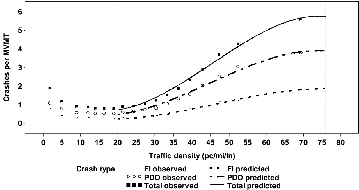
Figure 3.1. Observed and Predicted Total, FI, and PDO Crash Rates vs. Traffic Density (Seattle, Minneapolis-St. Paul, and Sacramento Areas Combined)
