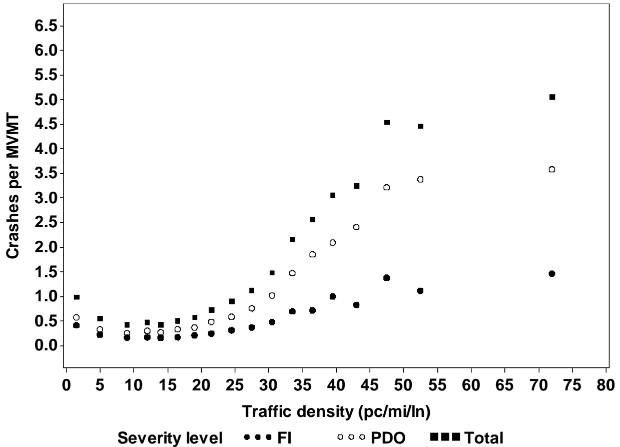
Figure 3.4. Crash Rate vs. Traffic Density for Recurrent Congestion and Normal Uncongested Flow (Non-Work-Zone Periods) in Sacramento
