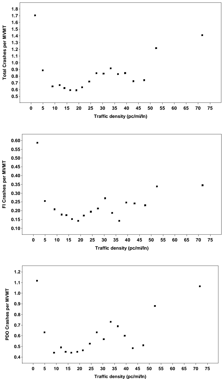
Figure 1.3. Observed Total, FI, and PDO Crash Rates vs. Traffic Density for Freeways in the Minneapolis-St. Paul Area
