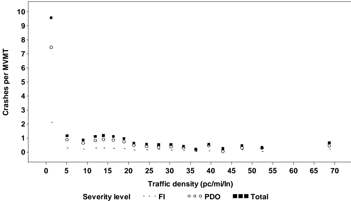
Figure 2.4. Total, FI, and PDO Crash Rates vs. Traffic Density for Directional Freeway Segments in the Kansas Portion of the Kansas City Metropolitan Area
