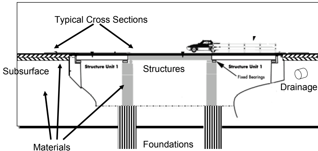
Figure 1: Critical Components of Infrastructure Design
