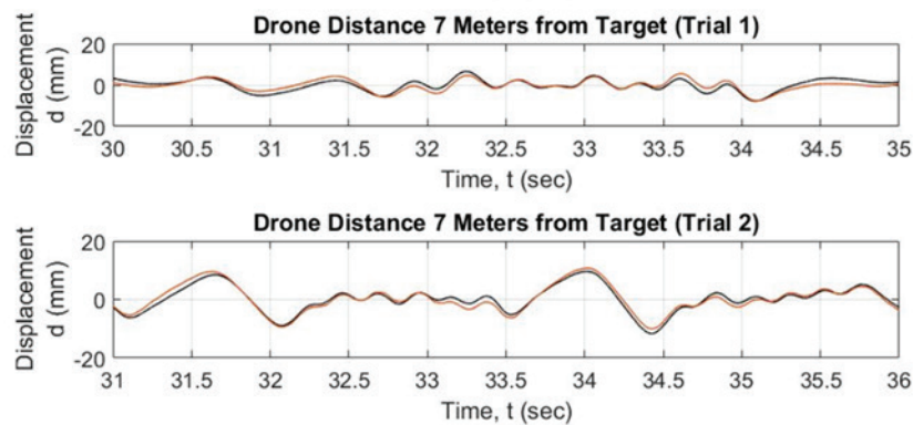
Figure 2. Contact-free, reference-free displacement validation.
