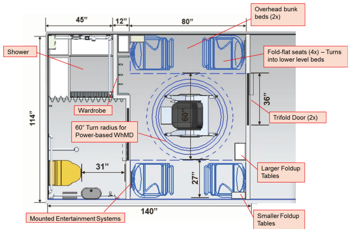
Figure 1: A 2-D rendering with notes and limited dimensions.
