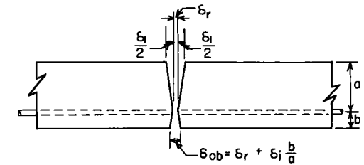
(a) CRACK DUE TO TEMPERATURE DROP
