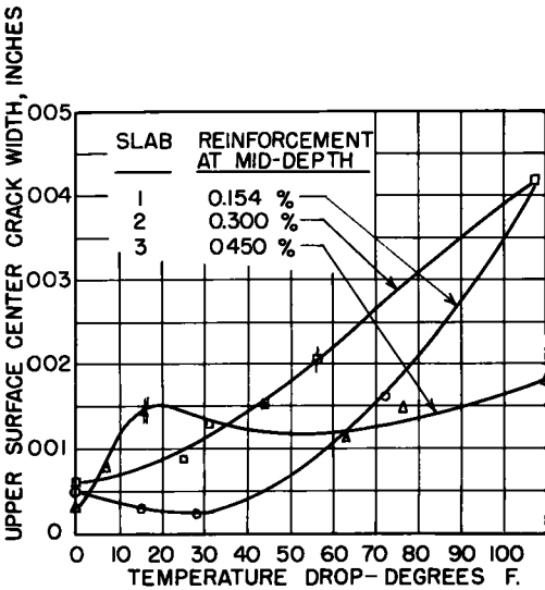
Figure 8. Influence of temperature drop and percentage of reinforcement on upper surface crack widths.
