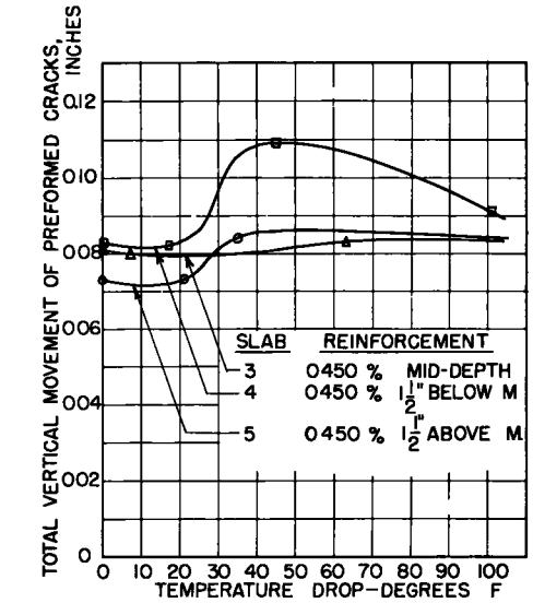
Figure 7. Influence of temperature drop and position of reinforcement on total vertical movement due to 15-kip wheel loads.
