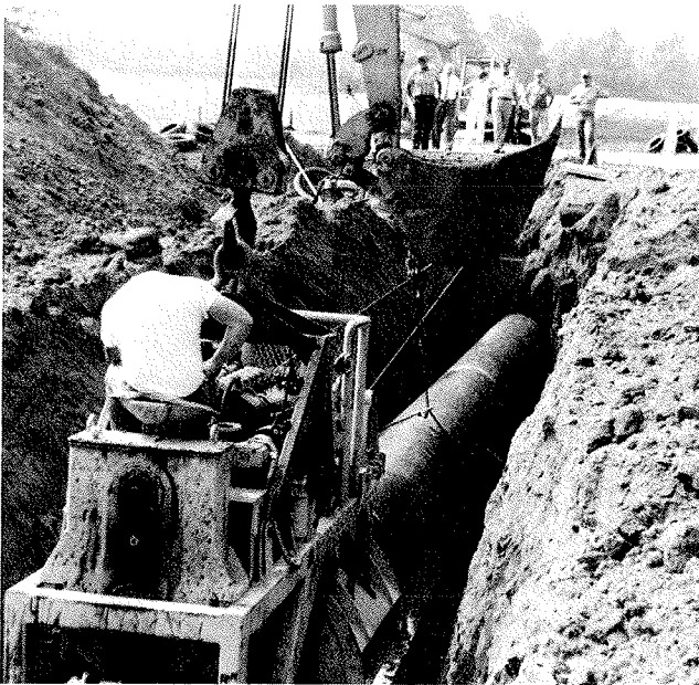
FIGURE 11 Actual field setup of the cradle type auger boring method.
