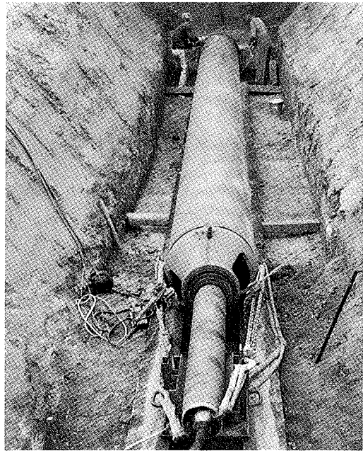
FIGURE 26 Typical field setup for pipe ramming method.
