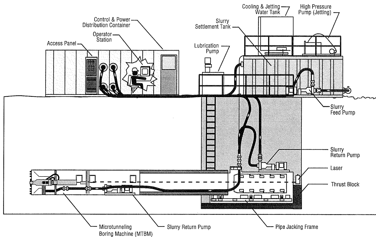
FIGURE 19 Basic components of a microtunneling system.
