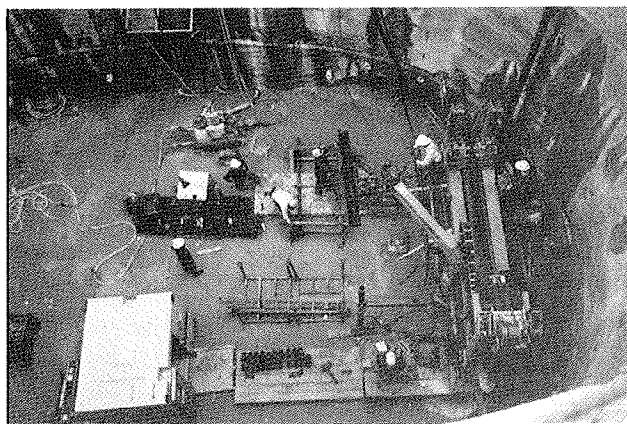
FIGURE 32 Use of horizontal directional drilling (HDD) for strengthening utility tunnel roof (76): (above) HDD rig performs grout drilling inside the drill chambers; (below) view from top of shaft looking at HDD rig and survey hut. Top portion of the tunnel portal can be seen in the upper left and right.
