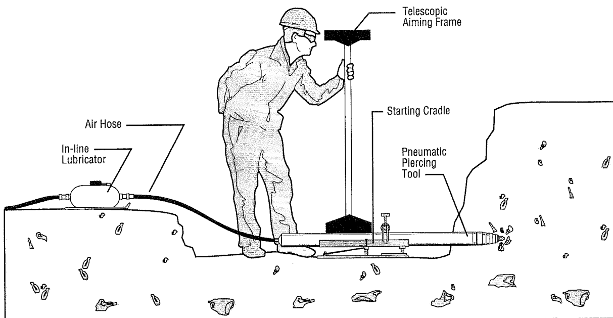
FIGURE 28 Impact moling process.
