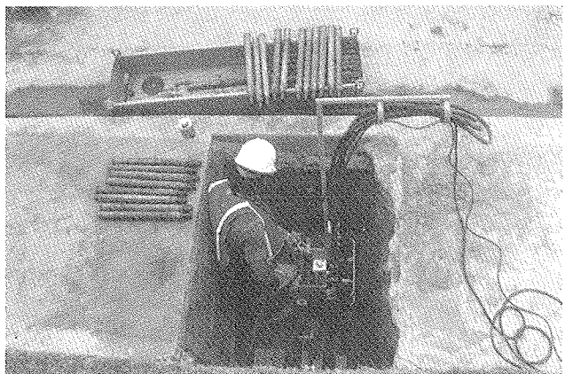
FIGURE 24 Pit launched mini-horizontal directional drilling (63): (Top) The block wall eliminated options for drilling without damage to curb or street. (Bottom) The quick shot requires a compact setup pit. With this model, only a 3-ft by 4-ft pit, half of a sidewalk flag, at this site.
