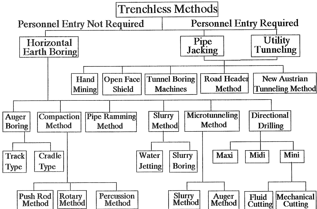
FIGURE 6 Classification systems for trenchless methods.
