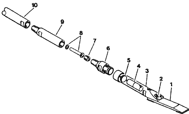
FIGURE 23 Horizontal directional drilling head assembly (60): 1) bit, 2) fluid nozzle, 3) beacon housing, 4) beacon, 5) beacon housing plug, 6) end cap, 7) screen sub plug, 8) screen, 9) screen sub, and 10) drill pipe.
