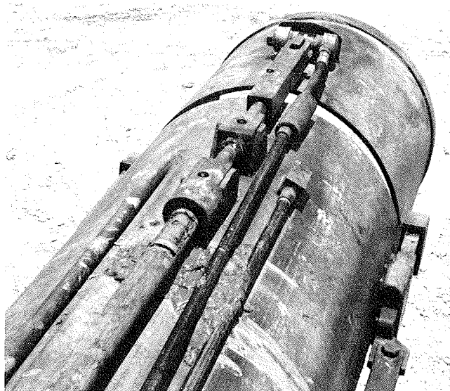
FIGURE 15 Finished LAG steering system for auger boring method.
