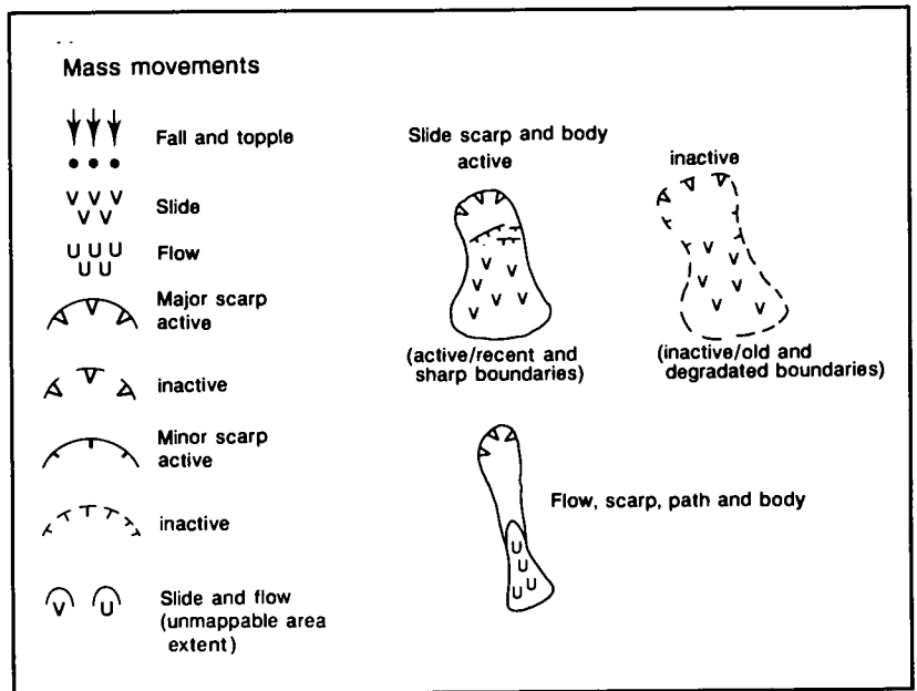
FIGURE 8-8 Example of legend for slope instability map. By use of such symbols, landslide type and activity may be differentiated. Morphologic features and drainage conditions associated with mass movements can also be indicated by symbols (modified from Sissakian et al. 1983).
