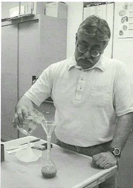
FIGURE 1 KT-50 is a simple method for determining the U-value or percentage of air voids in loosely compacted fine aggregates; the test can be performed in the field.
