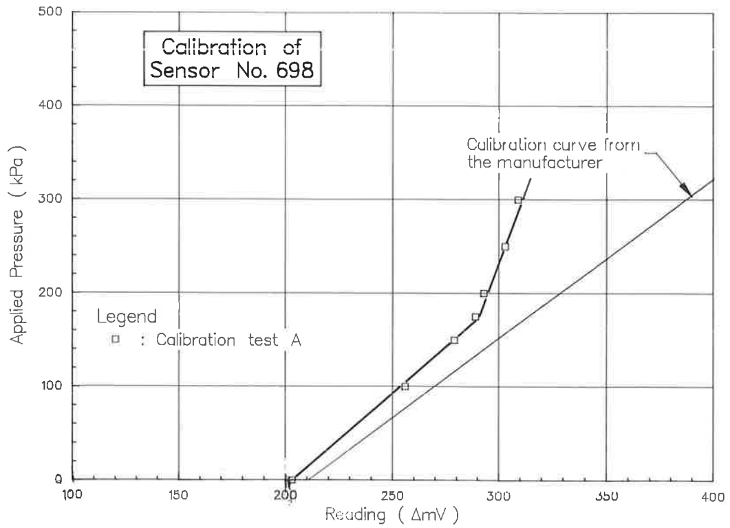
FIGURE 8 Calibration curve for Sensor 698.
