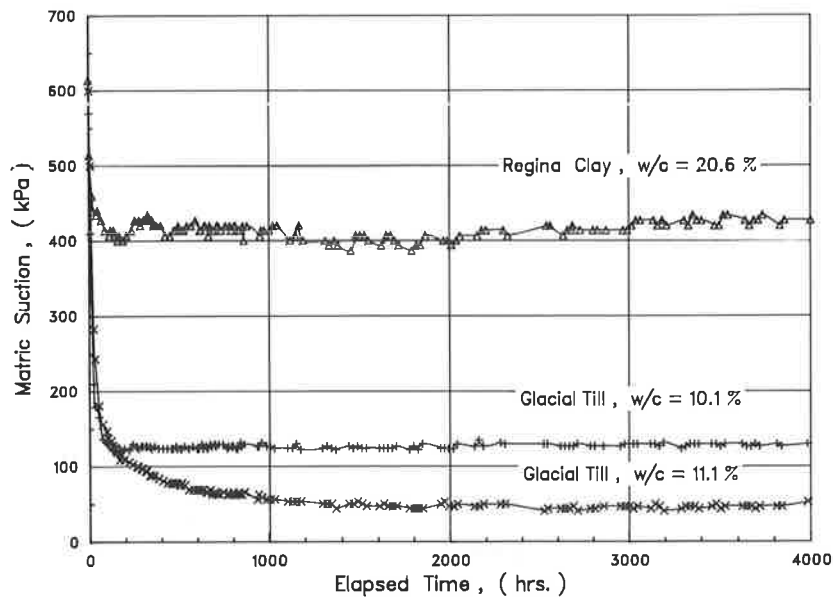
FIGURE 11 Measurements of matric suction on the subgrade of an indoor test track using the AGWA-II sensor.
