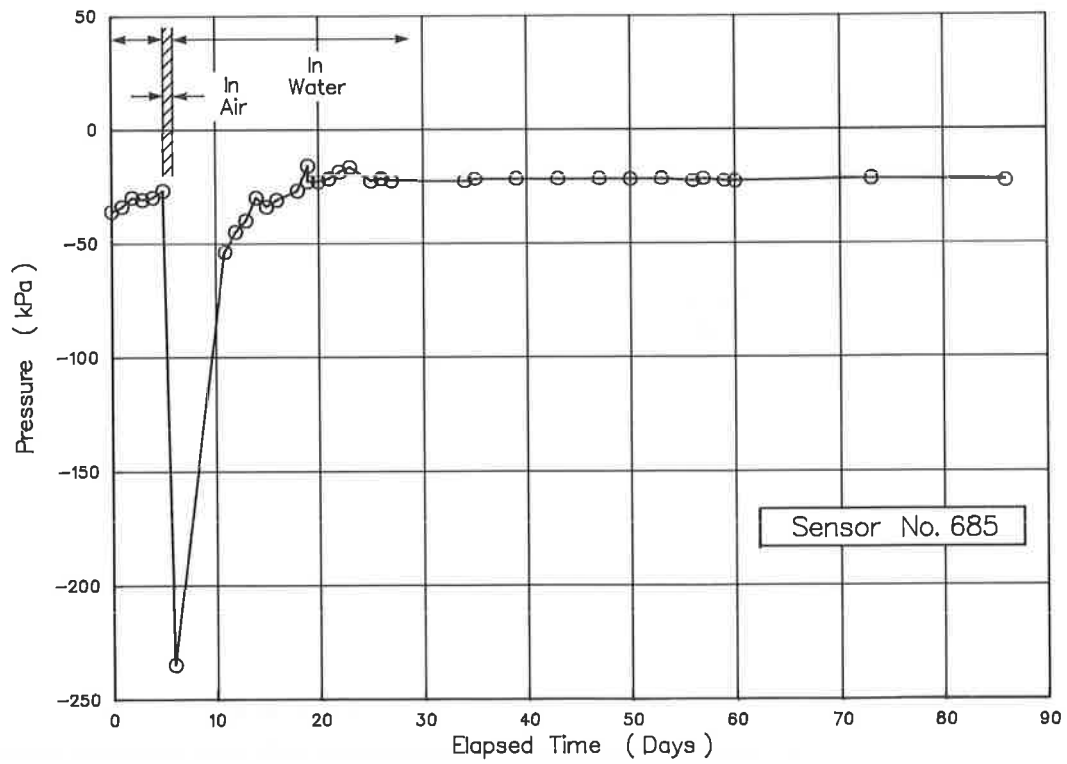
FIGURE 3 Response of Sensor 685 under wetting and drying cycle.
