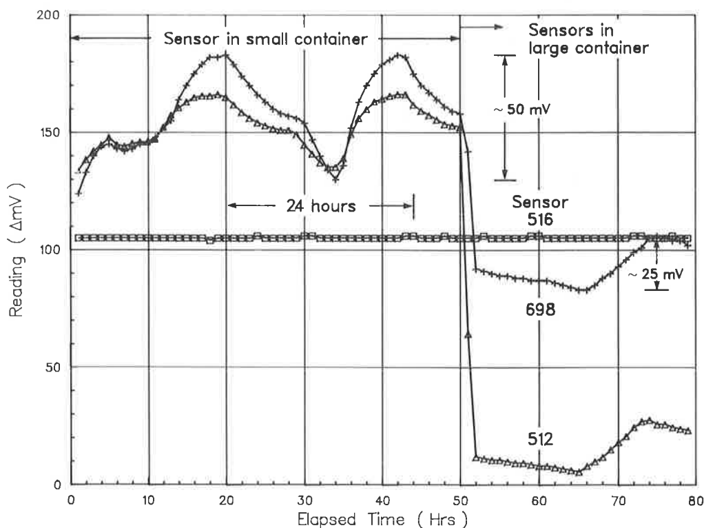
FIGURE 6 Effect of ambient temperature on sensor outputs.
