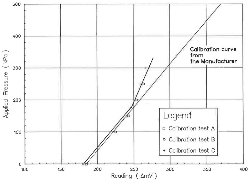
FIGURE 9 Calibration curve for Sensor 901.
