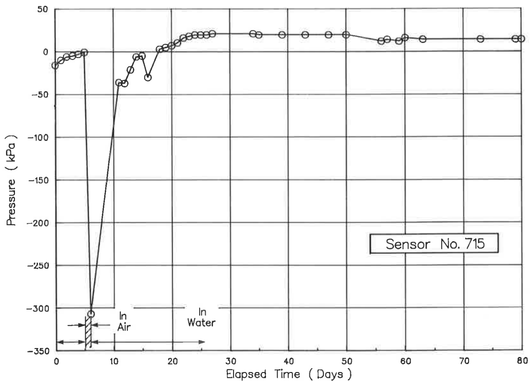
FIGURE 4 Response of Sensor 715 under wetting and drying cycle.
