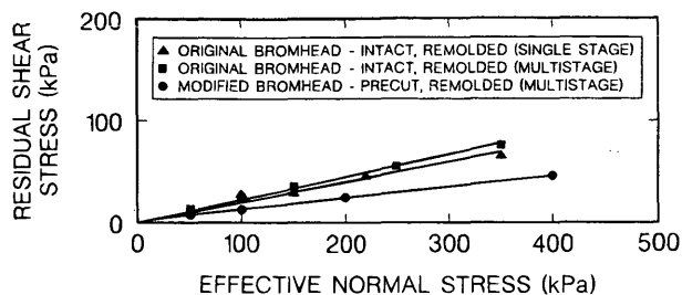
FIGURE 3 Effect of wall friction on measured residual shear strength of Pierre shale (Reliance).
