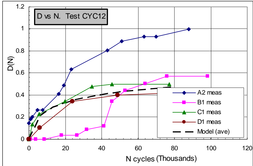
Figure F.26. Debonding vs. Number of Cycles. Test CYC12.
