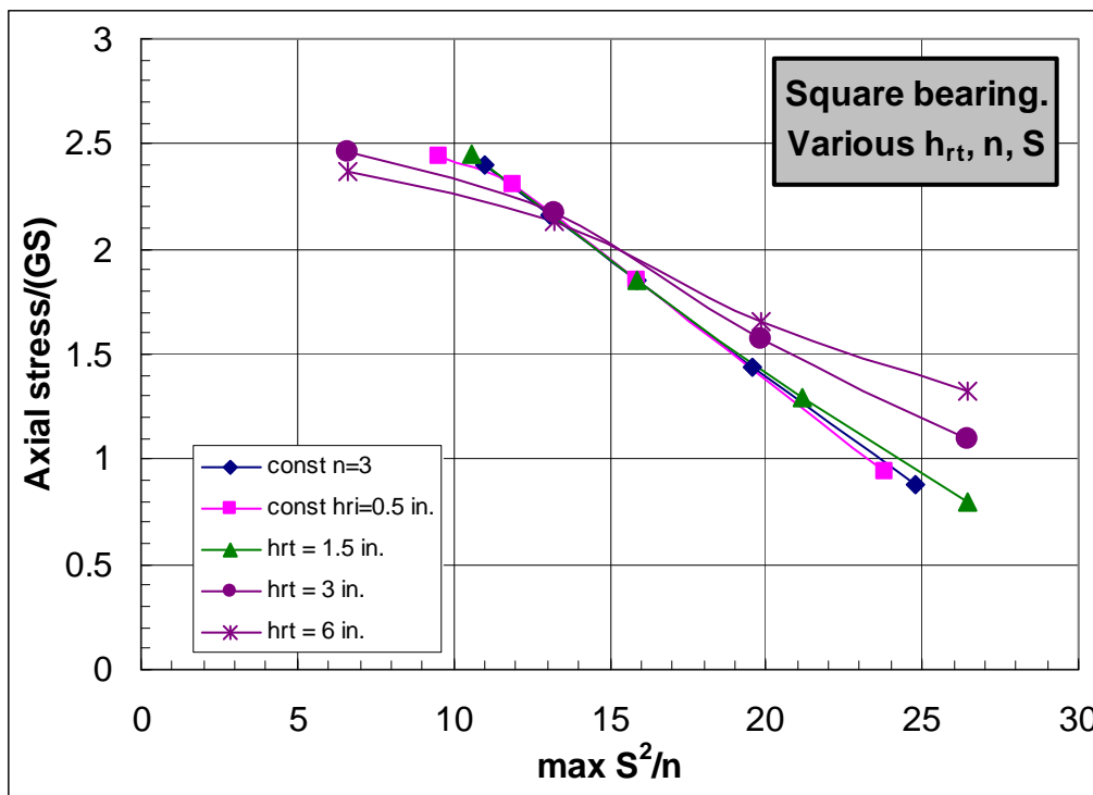
Figure F.46 Allowable normalized axial stress as a function of S^2/n .
