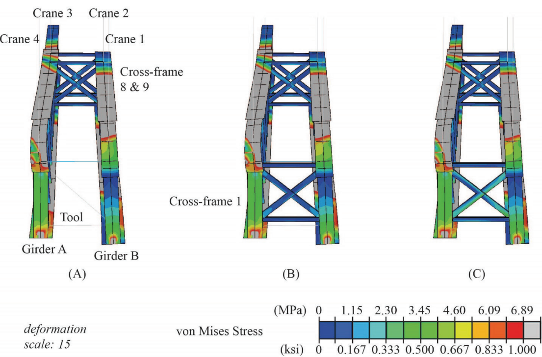
Figure 2 Highly skewed prototype bridge: Behavior when (A) the adjustable cross-frame tool is installed, (B) cross-frame 1 is installed, and (C) the adjustable cross-frame tool is released.
