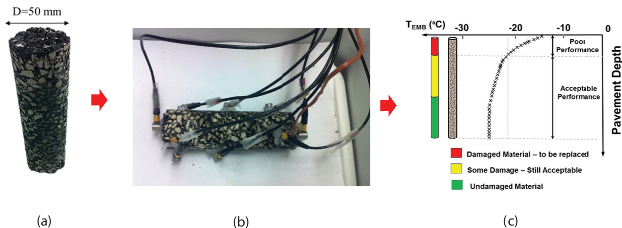
Figure 1 Continuous embrittlement temperature property characterization of age-graded field core materials: (a) 50-mm diameter field core sample, (b) AEA sensing system mounted on mixture sample, and (c) real-time graphical display of embrittlement temperature profile throughout the pavement thickness.
