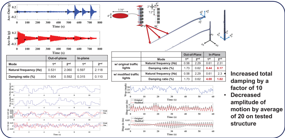
Figure 1 Illustration of DynaSignal and its impact on structural response.
