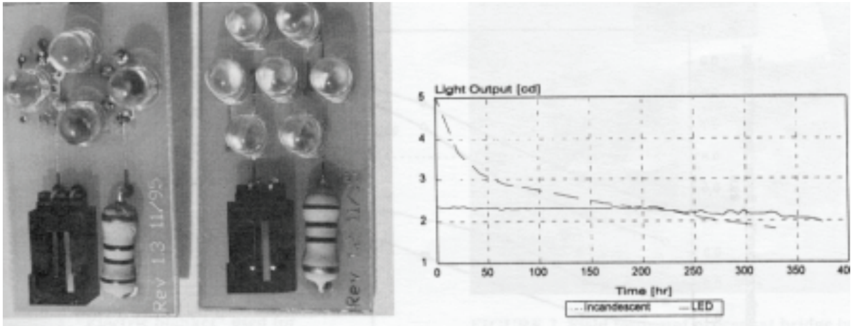
Figure 1 High- and low-intensity LED devices.
