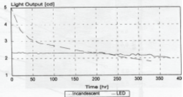
Figure 2 Results of endurance testing.
