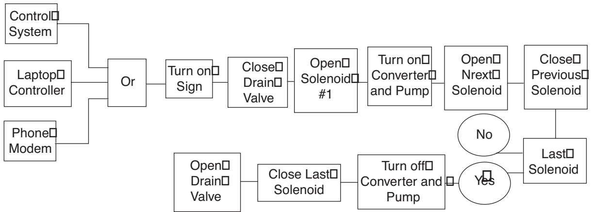
Figure 1 Spray system controller flowchart.
