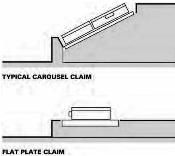
FIGURE 1 Sloped vs. flat plate baggage claim (ACRP Report 10).
