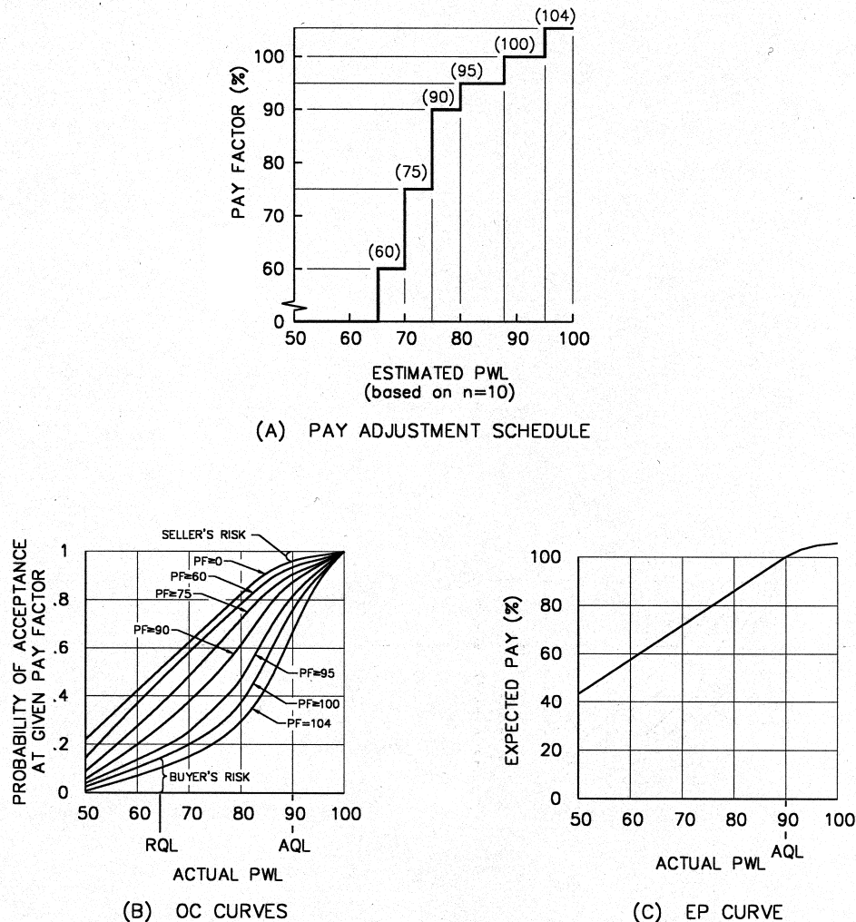
FIGURE 3 Graphic summaries of an acceptance plan (25). Shown above are three types of graphs used to summarize a typical acceptance plan containing a pay adjustment schedule. Figure 3a describes the pay adjustment schedule. Figures 3b and 3c present the corresponding set of OC curves and the corresponding EP curve for the acceptance plan. The OC curves show the probability that a contractor working under the acceptance plan will receive a given payment for various levels of actual (not estimated) submitted lot quality. The EP curve, on the other hand, shows the contractor's average payment in the long run for various levels of actual (not estimated) submitted lot quality. Note that information regarding the buyer's and seller's risks is found in the OC curves, and information regarding average payment in the long run is found in the EP curve. In addition, note that specific \beta_{pf} and \alpha_{pf} risks can also be identified; for example, \beta_{90} is about 29 percent, and \alpha_{90} is about 9 percent. Both the OC curves and the EP curve should be developed and evaluated to assess how an acceptance plan is (or will be) working. By itself, the EP curve for an acceptance plan may seem satisfactory, but the OC curves could show \beta_{pf} and \alpha_{pf} risks that are too high.
