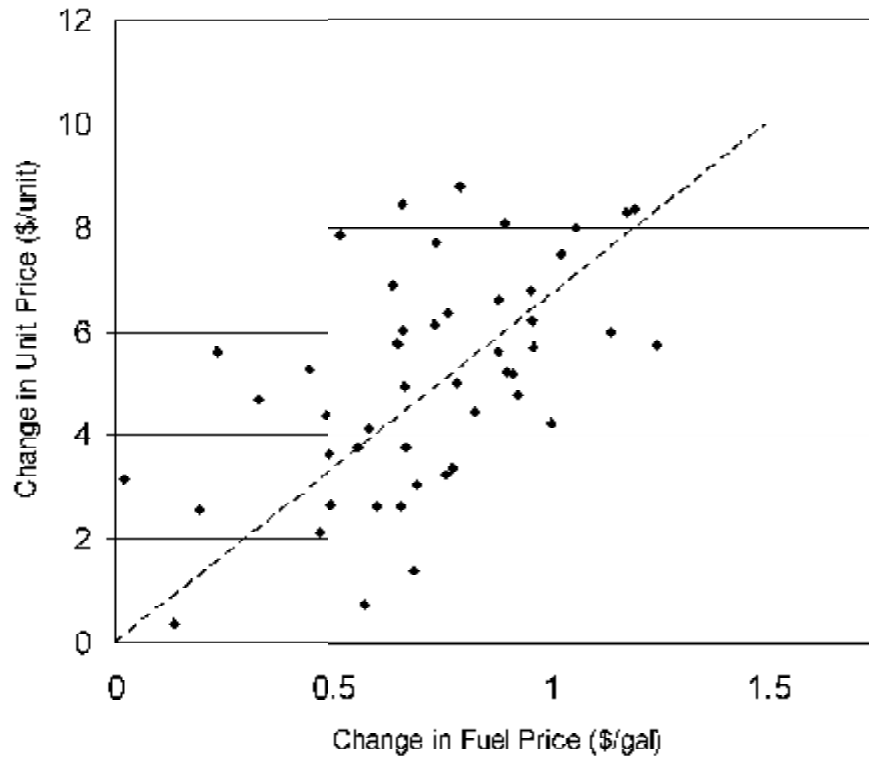
Exhibit 3-31: Trend Line Estimate of Fuel Usage for 1-Variable Model (Slope = ($/Unit)/ ($/Gallon) = Gallon/Unit)
