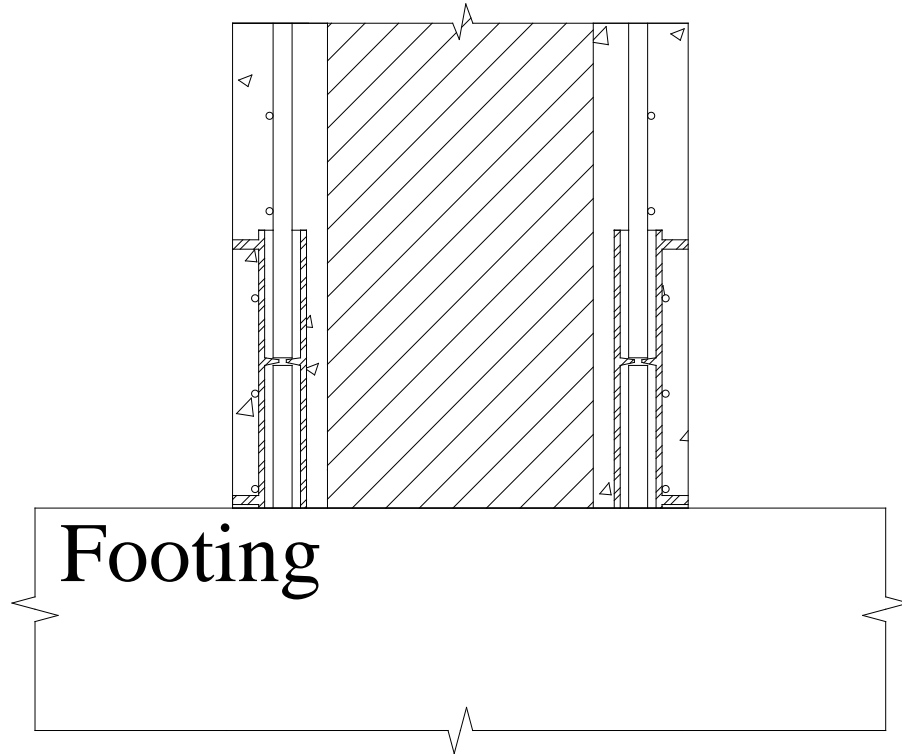
Figure 2.40 Precast column-footing connection model with grouted couplers tested at UNR
