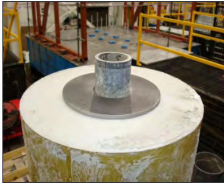
Figure 2.50 Steel pipe pin connection in a concrete-filled FRP tube column at UNR
