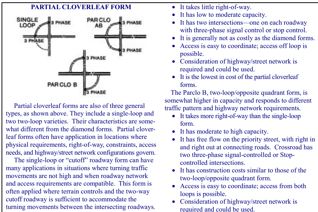
FIGURE 23 Partial Cloverleaf forms (178).
