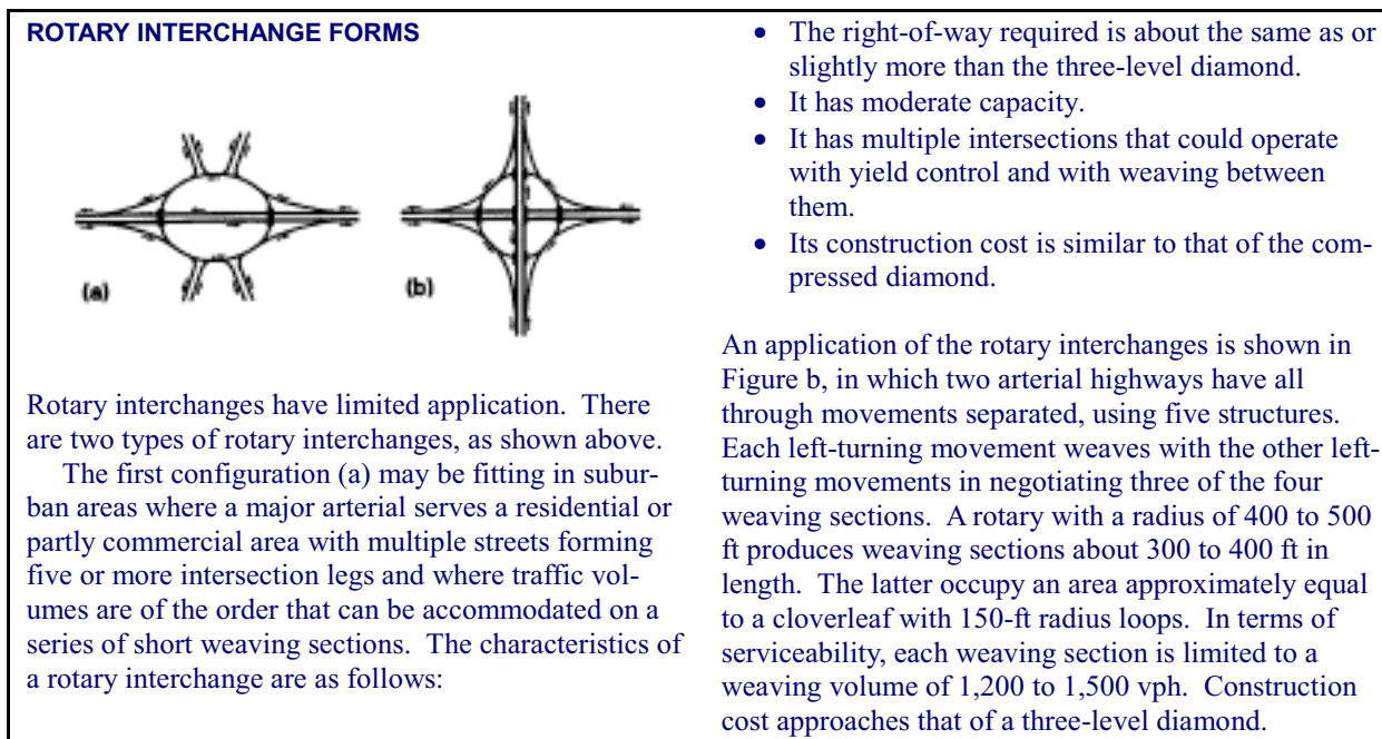
FIGURE 24 Rotary Interchange forms (178).
