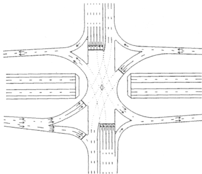
FIGURE 38 Single-point urban interchange (SPUI) (241).
