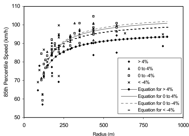
FIGURE 3 Horizontal curves on grades: V_{85} versus R (58).
