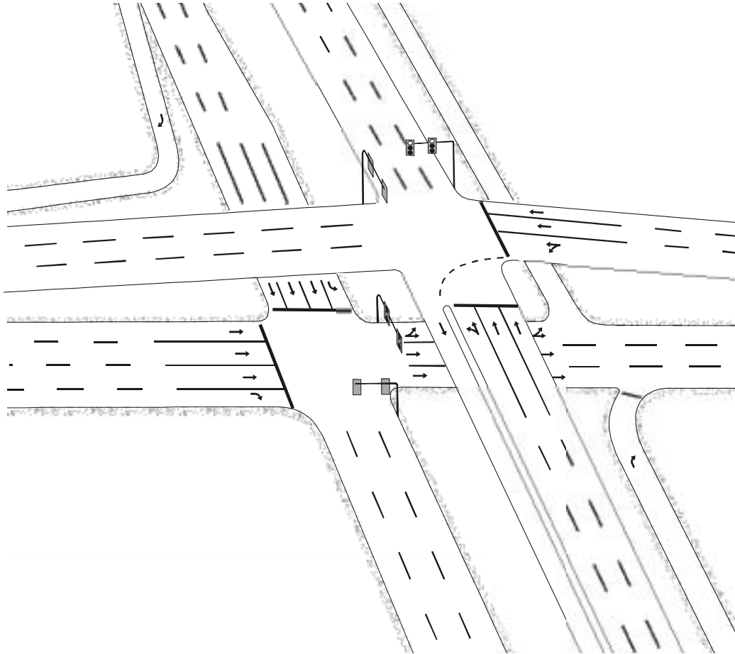
FIGURE 27 Echelon Interchange (180).
