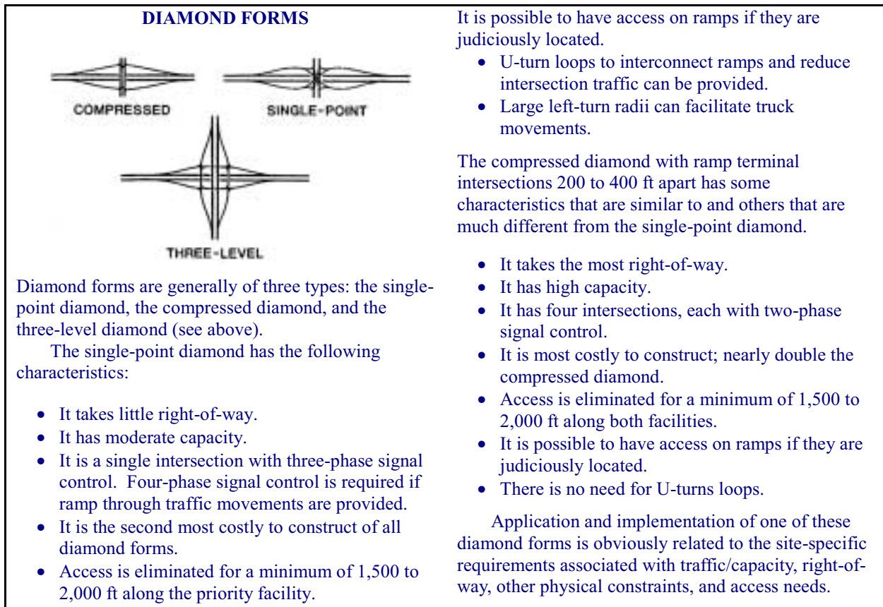
FIGURE 22 Diamond forms (178).
