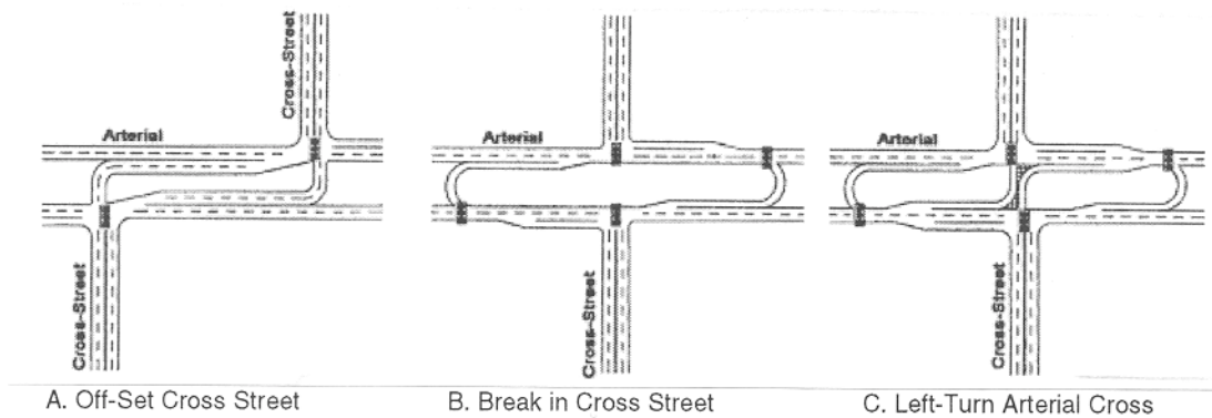
FIGURE 21 Superstreet arterial designs (177).
