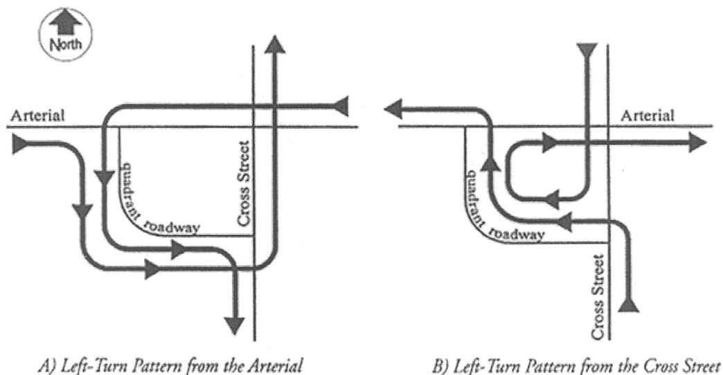
FIGURE 19 QRI left-turn pattern (176).
