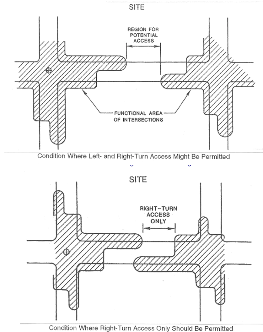
FIGURE 1 Region in which direct access might be provided on the basis of functional boundaries of the intersections adjacent to a site (15).
