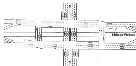
(A) Diamond Interchange
