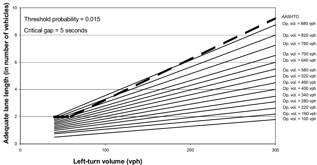
FIGURE 33 Comparison of AASHTO and proposed model lane lengths (209).
