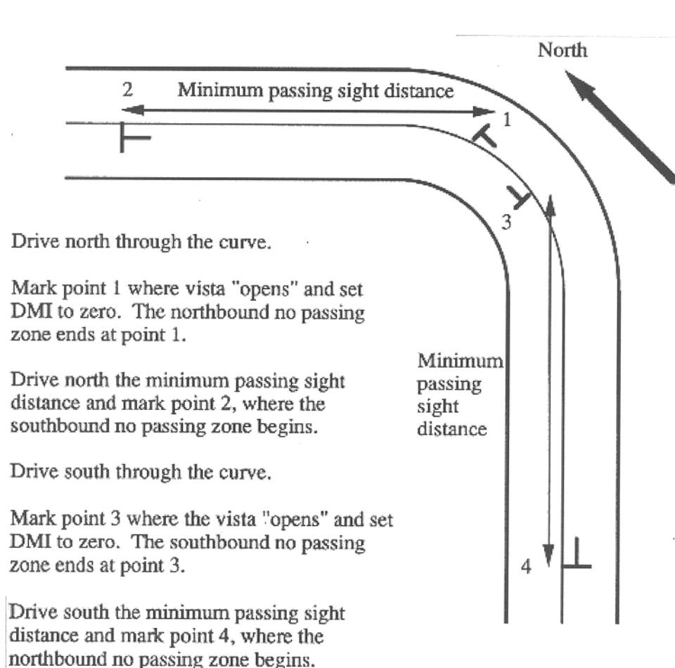
FIGURE 5 Illustration of the one-vehicle method (113).
