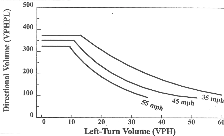
FIGURE 31 TTI left-turn guidelines (207).
