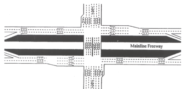
(B) Michigan Urban Diamond Interchange (MUDI)
