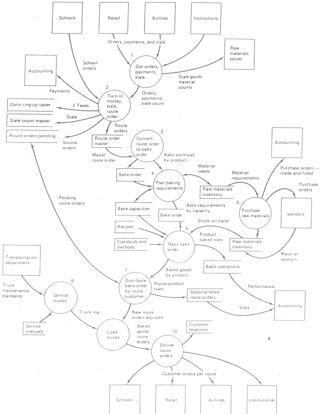
FIGURE C1 Bakery data flow diagram (Level 1) (Leslie 1986). (Reprinted by permission of Pearson Education, Inc., Upper Saddle River, N.J.).
