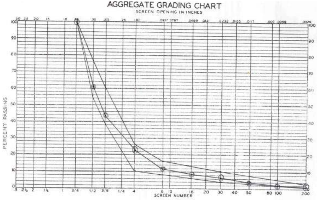
Figure F4 – Aggregate Gradation Chart for RMP Open Graded Mix
