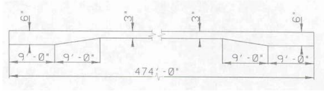
Figure 9 – Elevation view of UTW section
