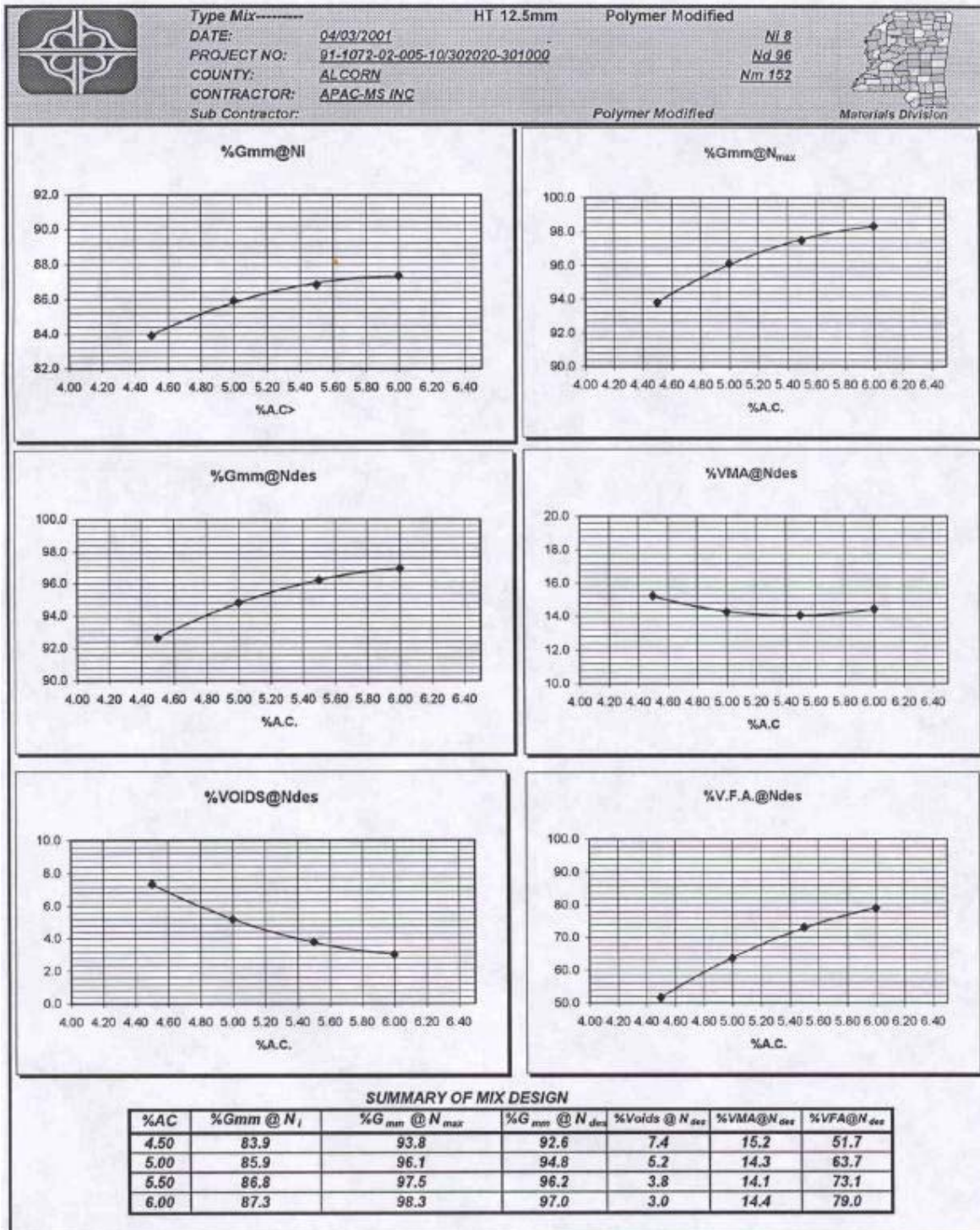
Figure H3 – Summary of PG 82-22 Mix Designs
