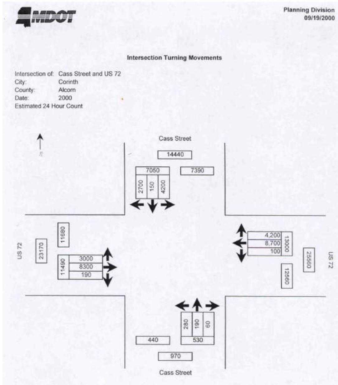
Figure A3 – Year 2000 Projected 24 hour turning movements for US 72 @ Cass Street
