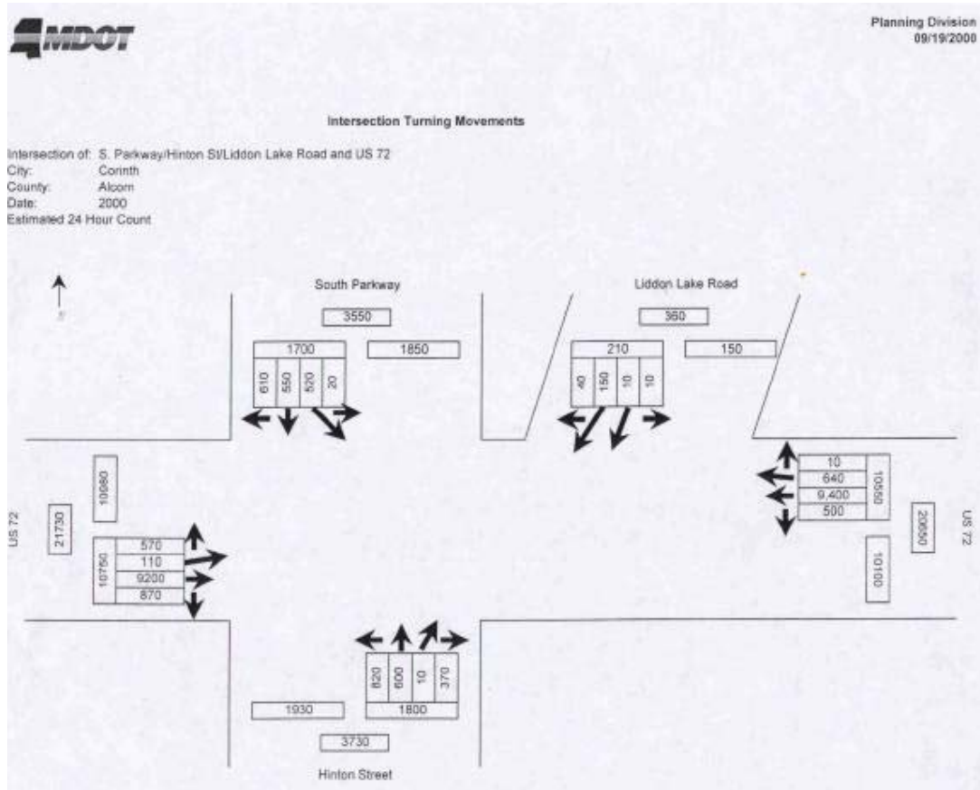
Figure A5 – Year 2000 Projected 24 hour turning movements for US 72 @ Hinton Street
