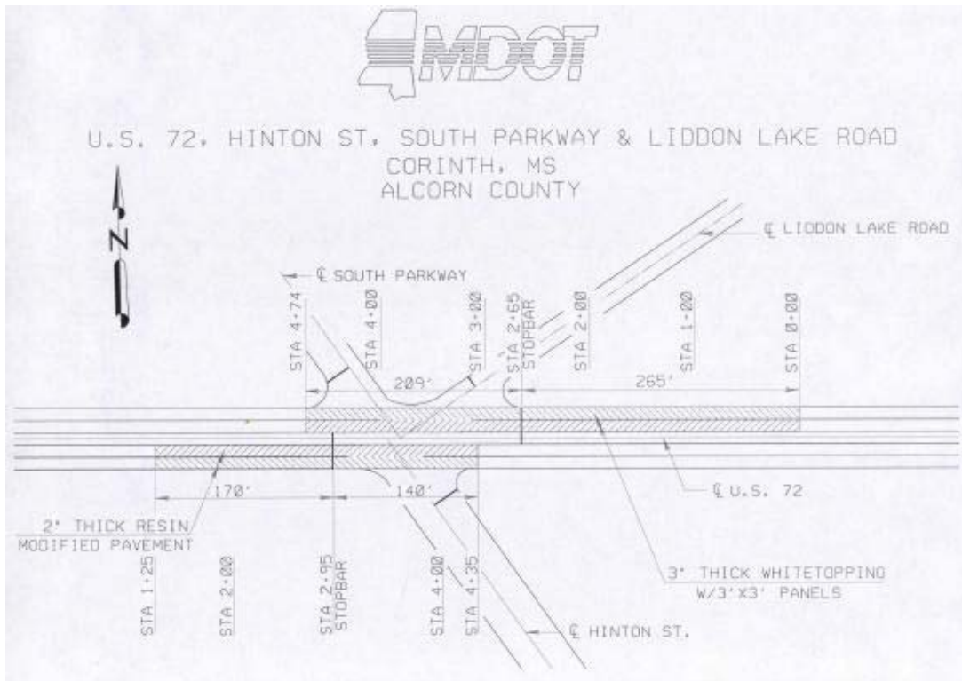
Figure 4 – Plan view intersection of US 72 & Hinton Street
