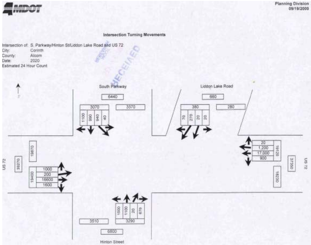
Figure A6 – Year 2020 Projected 24 hour turning movements for US 72 @ Hinton Street
