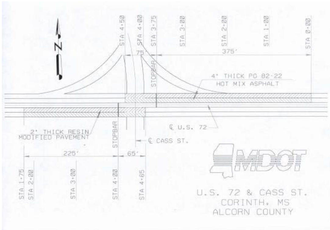
Figure 3 – Plan view intersection of US 72 & Cass Street
