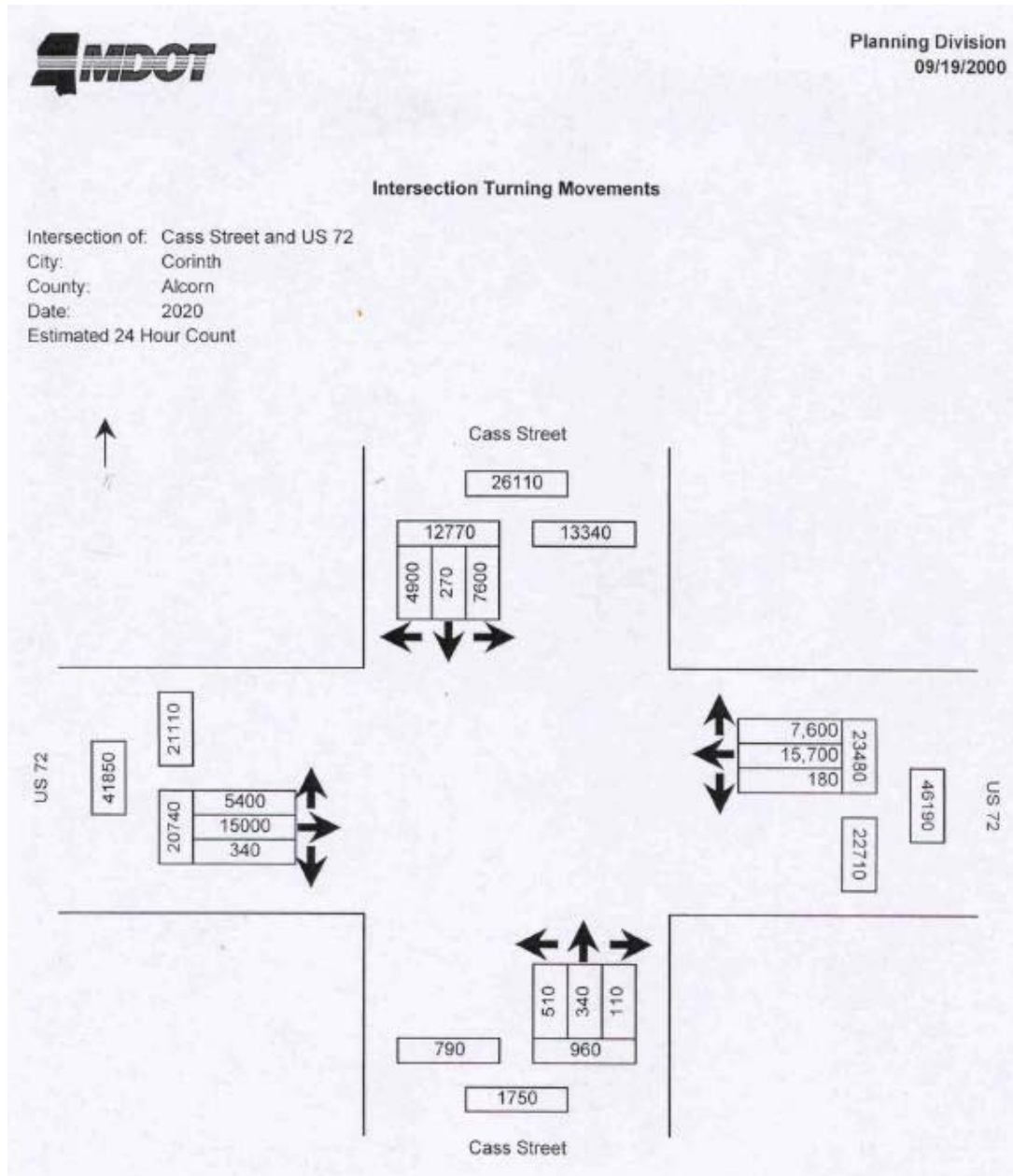
Figure A4 – Year 2020 Projected 24 hour turning movements for US 72 @ Cass Street
