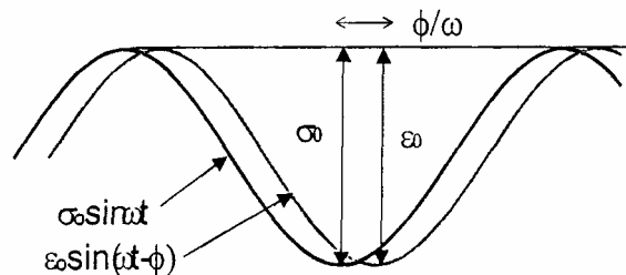
Figure 1 – Dynamic (Complex) Modulus Test
