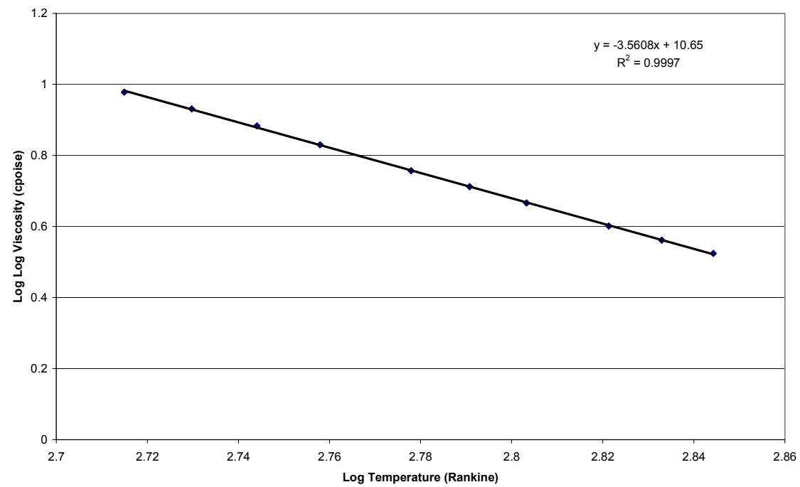
Viscosity-Temperature Relationship
