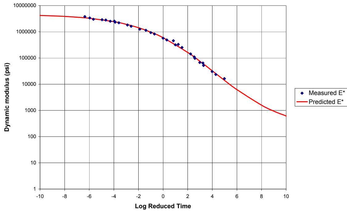
Dynamic Asphalt Modulus - Master Curve
