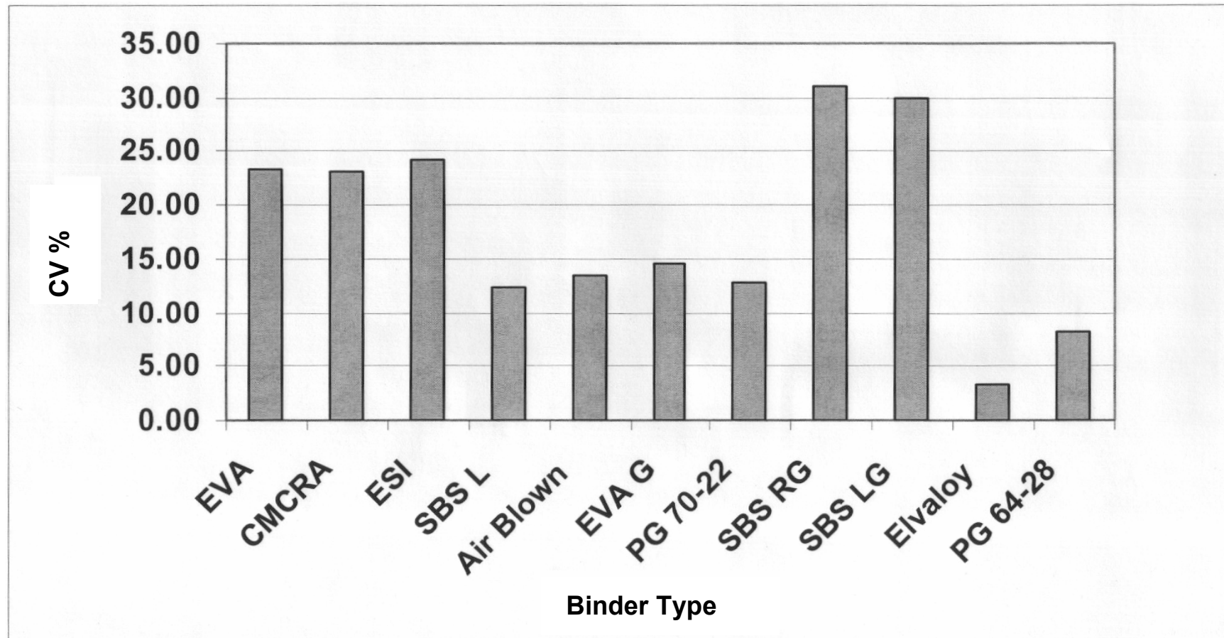
Figure 6 –FHWA-ALF Coefficient of Variation of Measured E^* for Various Asphalt Binders (3 Replicates, 50 °C, 10 Hz)
