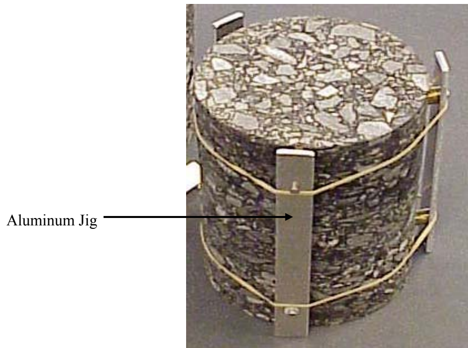
Photo 5 – Aluminum Jig Used to Secure Gauge Plugs on Test Specimens
