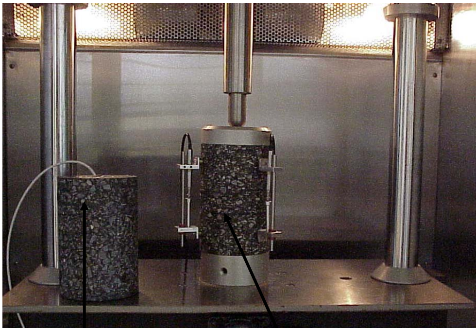
Photo 6 – Instrumented Specimen in the Testing Machine
