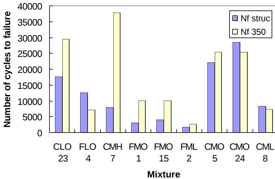
Figure 8.20 Predicted Number of Cycles to Failure Using Structural Analysis Microstrain (Nf struc) and Average 350 Microstrain (Nf 350) Amplitudes
