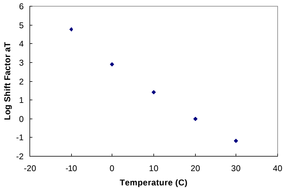
Figure A.5 Time –Temperature Shift Factors Used to Create Creep Compliance and Dynamic Modulus Master Curves
