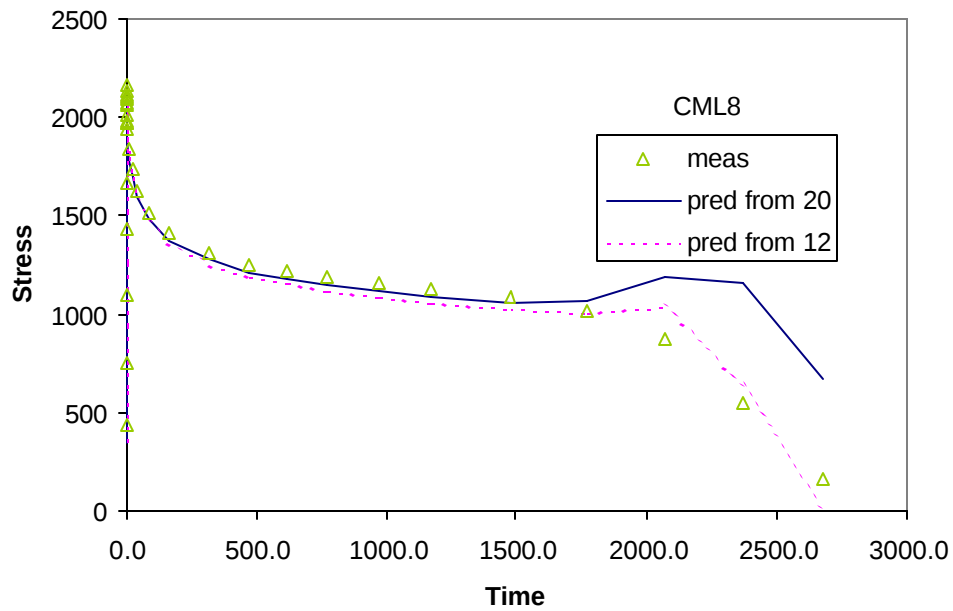
Figure D.49 Measured and Predicted Values for CML8 from 20C and 12C Curves
