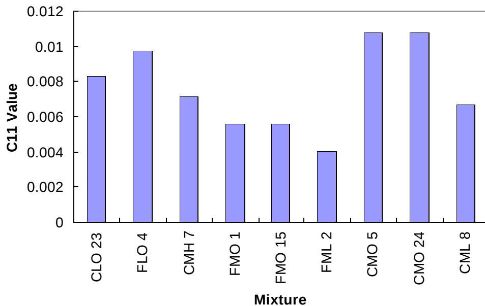
Figure 8.12 Comparison of C_{11} Values among Mixtures
