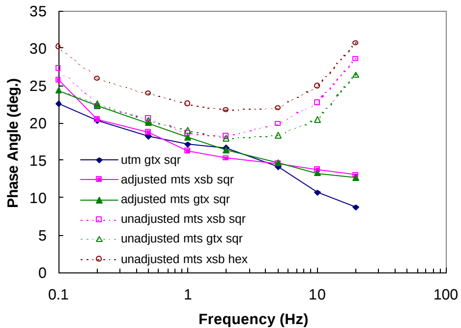
FIGURE B.4 Adjusted and Unadjusted Phase Angle Measurements for Various Machine, LVDT, and Mount Type Combinations
