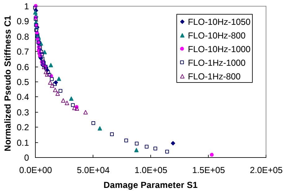
Figure 6.36 Characteristic C_1 versus S_1 Curve for 10 Hz and 1 Hz Cyclic Testing at 20°C on FLO Mixture at Several Strain Amplitudes
