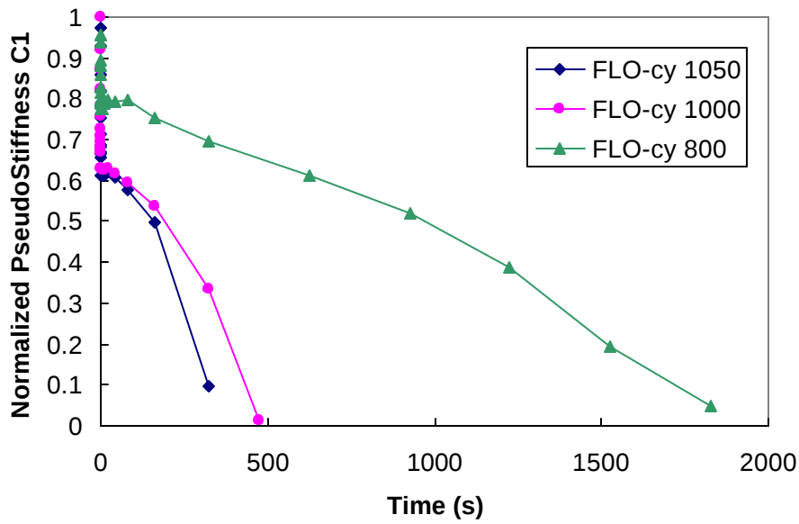
Figure 6.20 Normalized Pseudo stiffness as a Function of Time for FLO Mixture Tested at 10 Hz and Three Cyclic Strain Amplitudes
