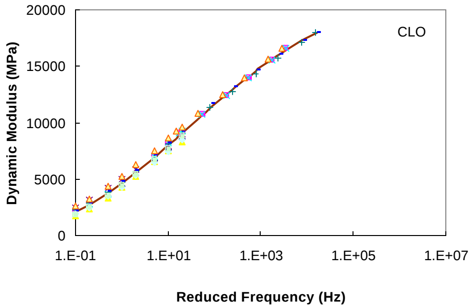
FIGURE C.3 Individual and Average Dynamic Modulus Curves for CLO Mixture
