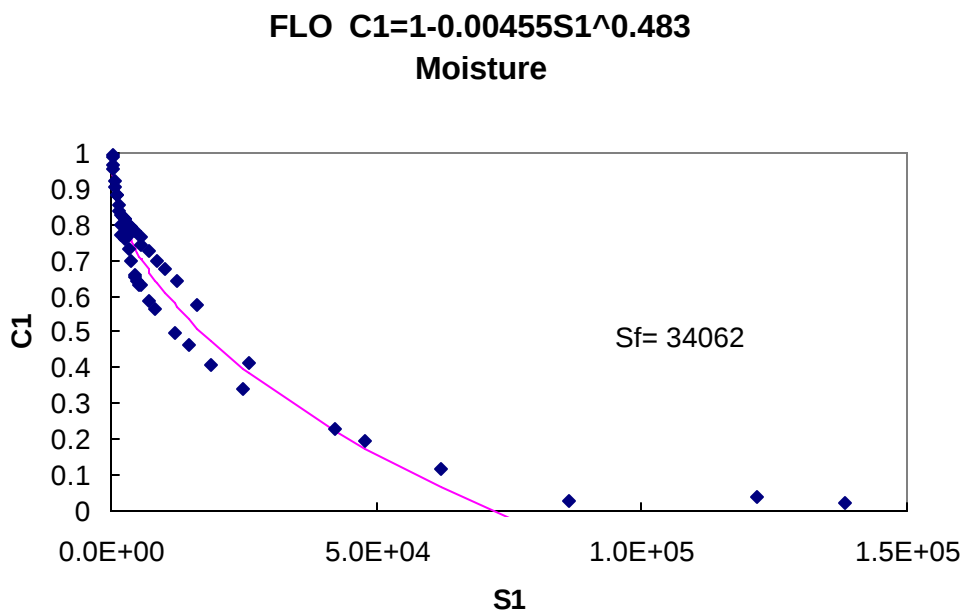
Figure D.10 Characteristic Curve for Moisture Cyclic FLO Data
