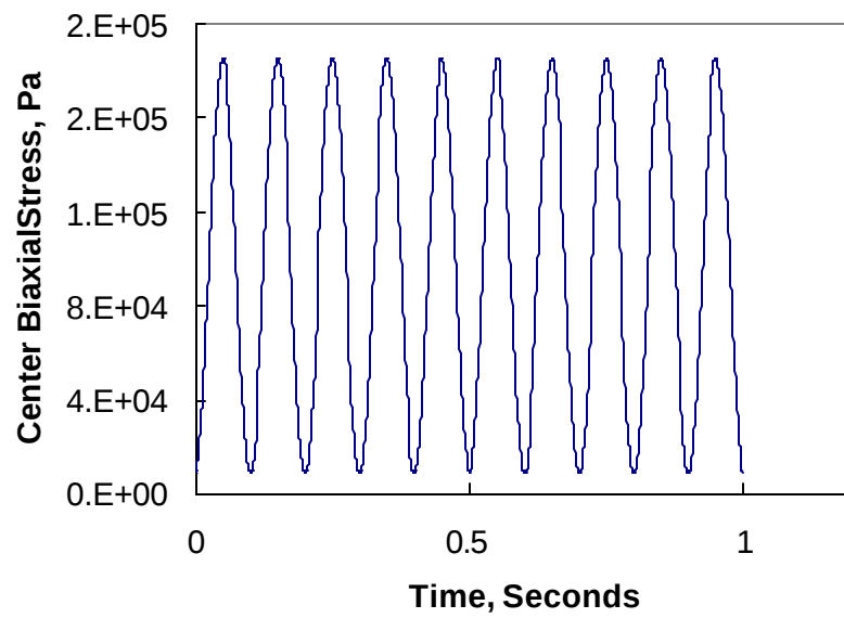
Figure 7.14 Stress vs. Time for Cyclic Tests
