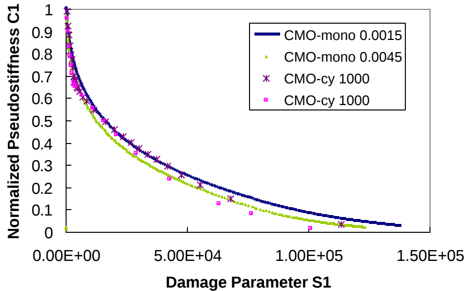
Figure 2.2 Characteristic C_1 versus S_1 Curve for Cyclic and Monotonic Testing on CMO Mixture at 20°C (Cyclic Testing at 1000 Crosshead Microstrain Amplitude, Monotonic Testing at Two Crosshead Strain Rates)
