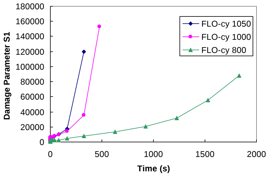
Figure 6.22 Damage Parameter as a Function of Time for FLO Mixture Tested at Three 10Hz Cyclic Strain Amplitudes
