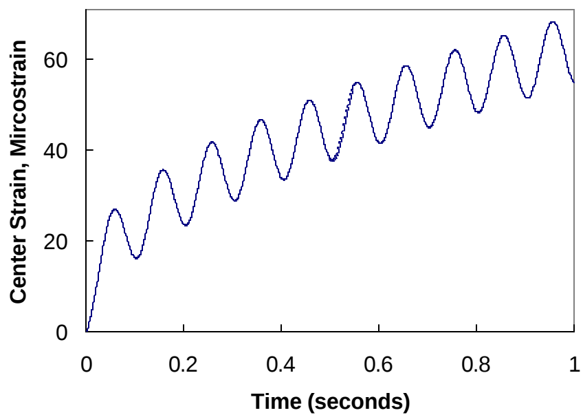
Figure 7.15 Smoothed Center Strain vs. Time
