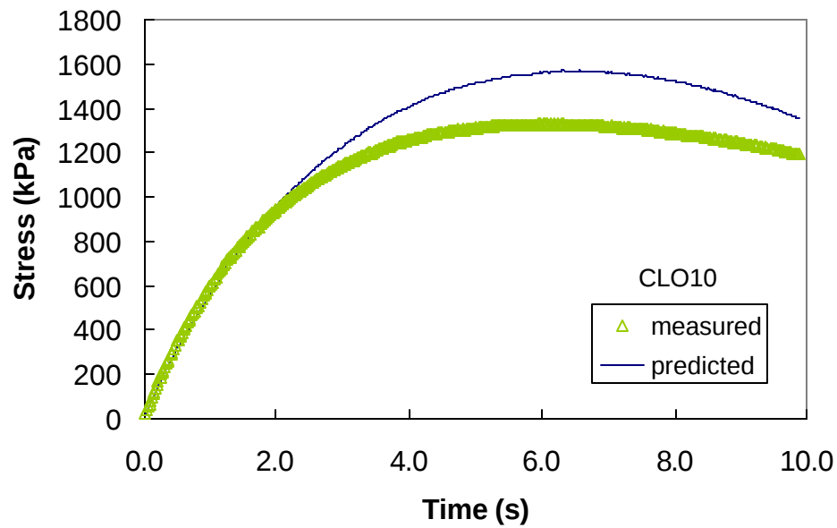
Figure 6.40 Measured and Predicted Stress Values for CLO10 Monotonic Test
