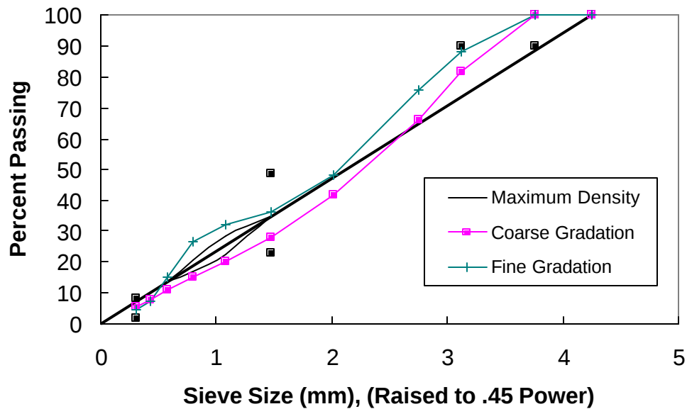
Figure 5.3 WesTrack Coarse and Fine Gradations
