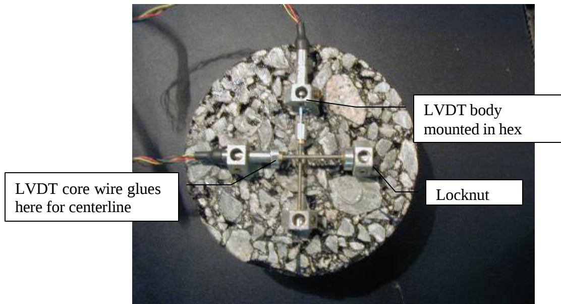
Figure 5.8 Plan View of LVDTs Glued to a Specimen
