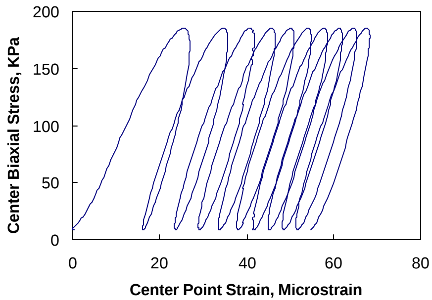
Figure 7.16 Biaxial Stress vs. Center Strain
