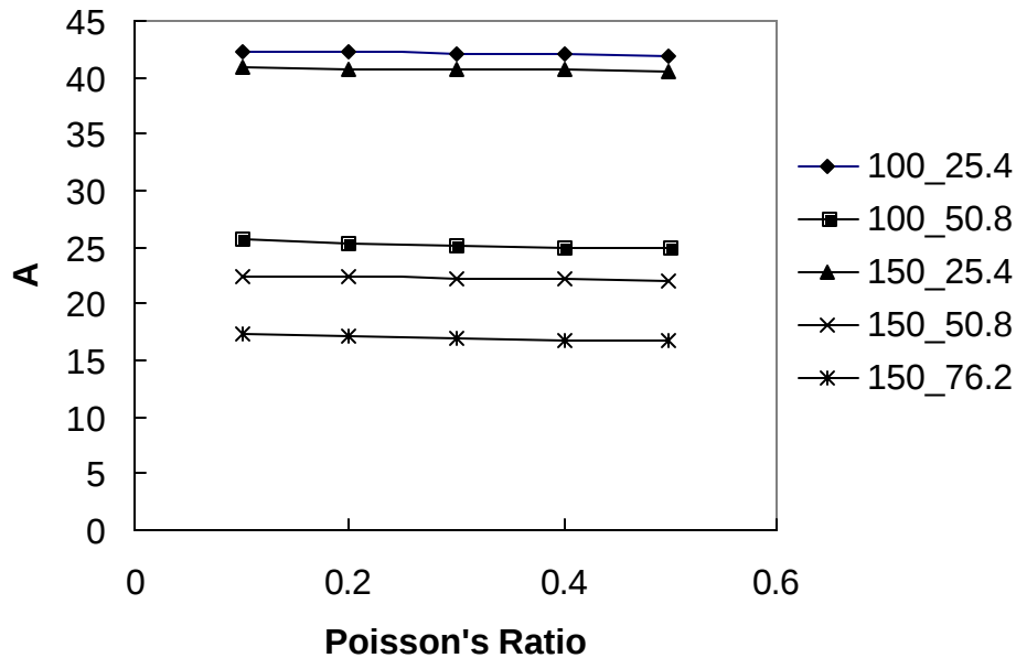
Figure 7.1 Effect of Change in Poisson's Ratio on Strain Calculation
