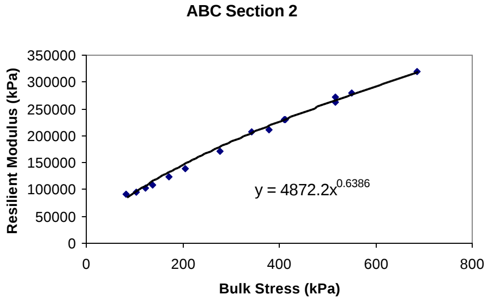
Figure D.20 ABC Resilient Modulus Data for WesTrack Section 2
