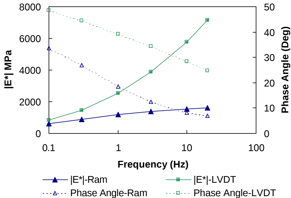
FIGURE B.2 Comparison of Ram and LVDT Dynamic Modulus and Phase Angle Measurements
