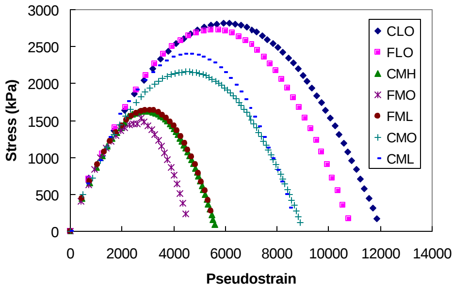
Figure 8.17 Predicted Stress-Pseudo strain Curves for Constant Crosshead Rate Test at 0.0045 strain/sec
