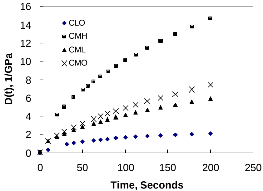
Figure 8.3 Creep Compliance of Four Coarse Gradation Mixtures
