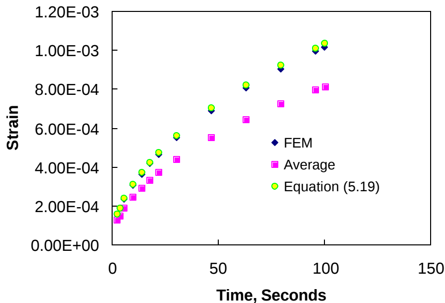
Figure 7.4 Verification of Center Strain Calculation
