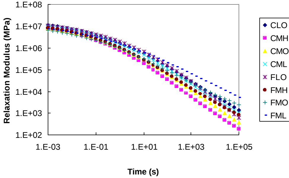
Figure 6.11 Relaxation Modulus Curves for All Mixtures
