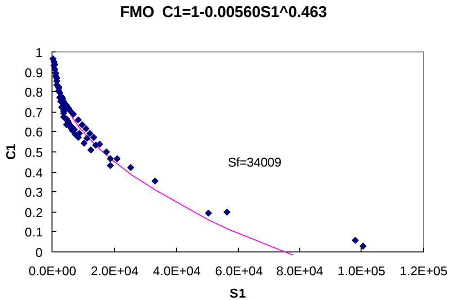
Figure D.12 Characteristic Curve for Cyclic FMO Data
