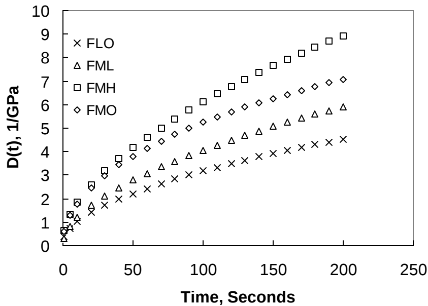
Figure 8.4 Creep Compliance of Four Fine Gradation Mixtures
