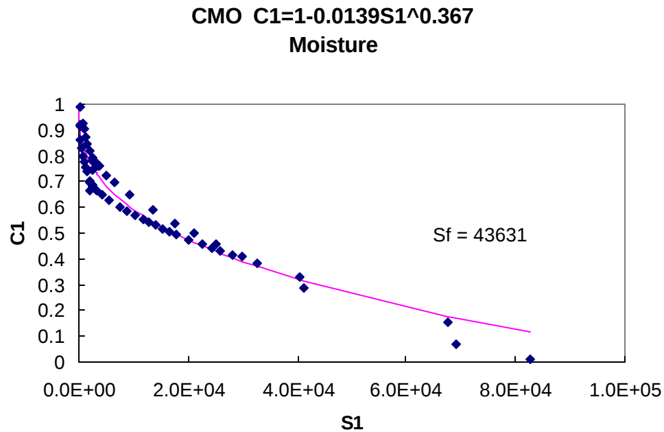
Figure D.18 Characteristic Curve for Moisture Cyclic CMO Data
