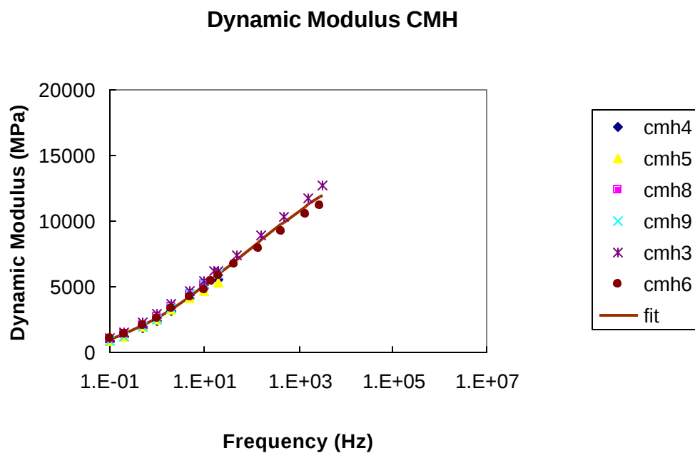
Figure D.8 Dynamic Modulus Master Curves for CMH Mixture
