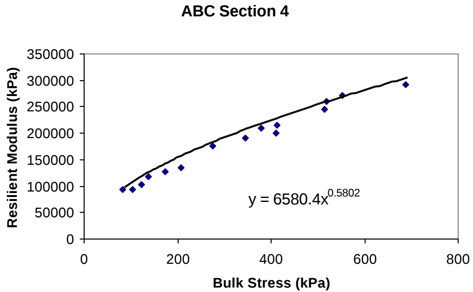
Figure D.21 ABC Resilient Modulus Data for WesTrack Section 4
