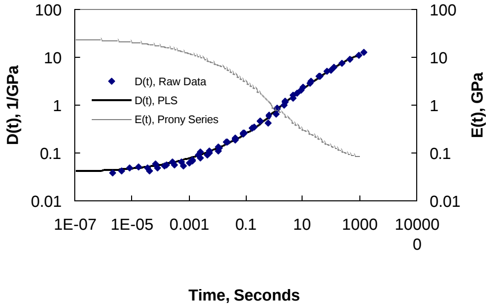
Figure 7.12 Creep Compliance and Converted Relaxation Modulus
