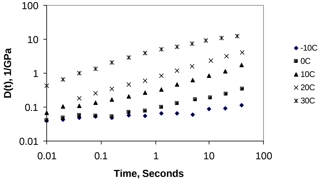
Figure 7.8 Creep Compliance Curves at Different Temperatures before Shifting
