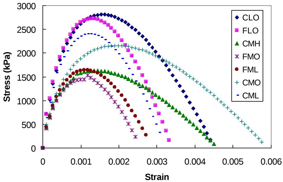
Figure 8.16 Predicted Stress-Strain Curves for Constant Crosshead Rate Test at 0.0045 strain/sec
