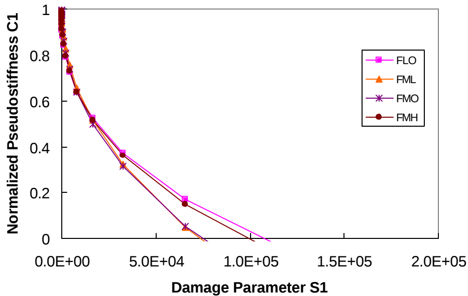
Figure 6.29 Characteristic C_1 versus S_1 Curves for Fine Mixtures
