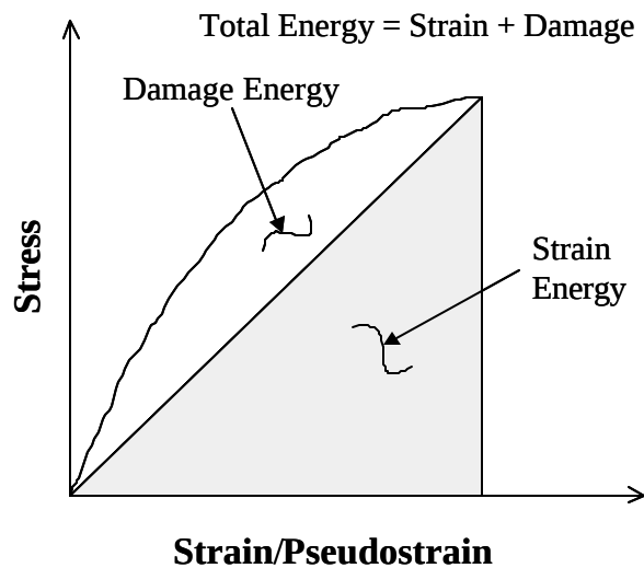
Figure 4.11 Definition of Energies
