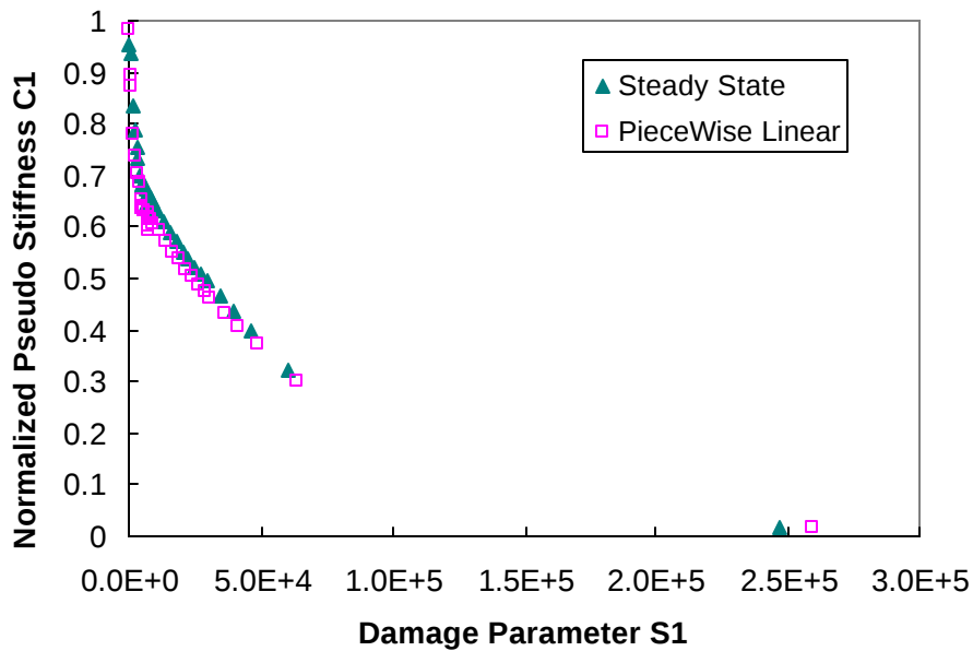
Figure 6.17 Difference in C_1 - S_1 Curve Using Piece Wise Linear Approach and Steady State Assumption
