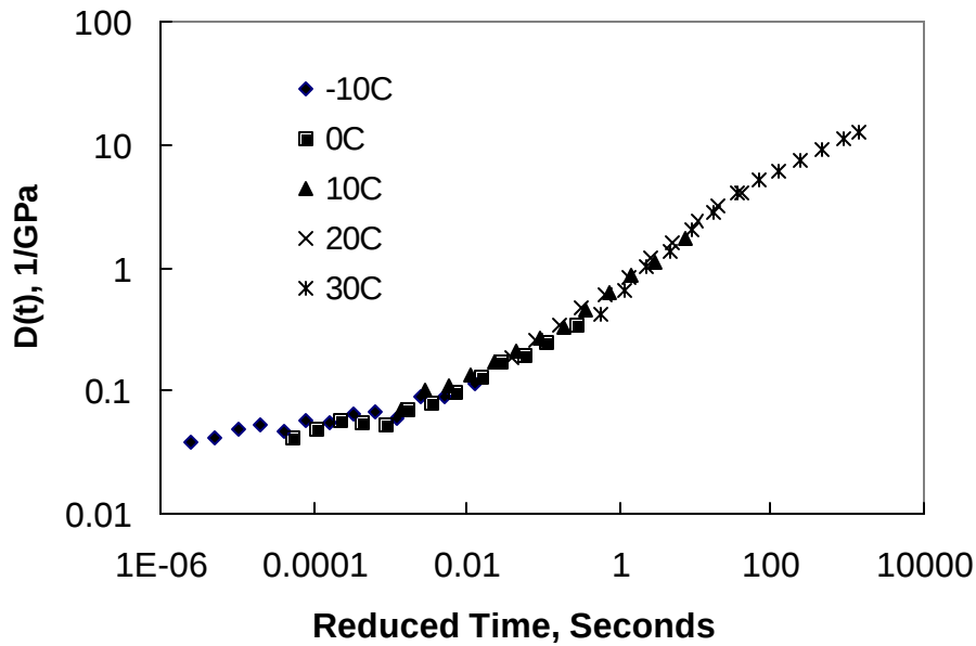
Figure 7.9 Creep Compliance Master Curve after Shifting on IDT Specimens
