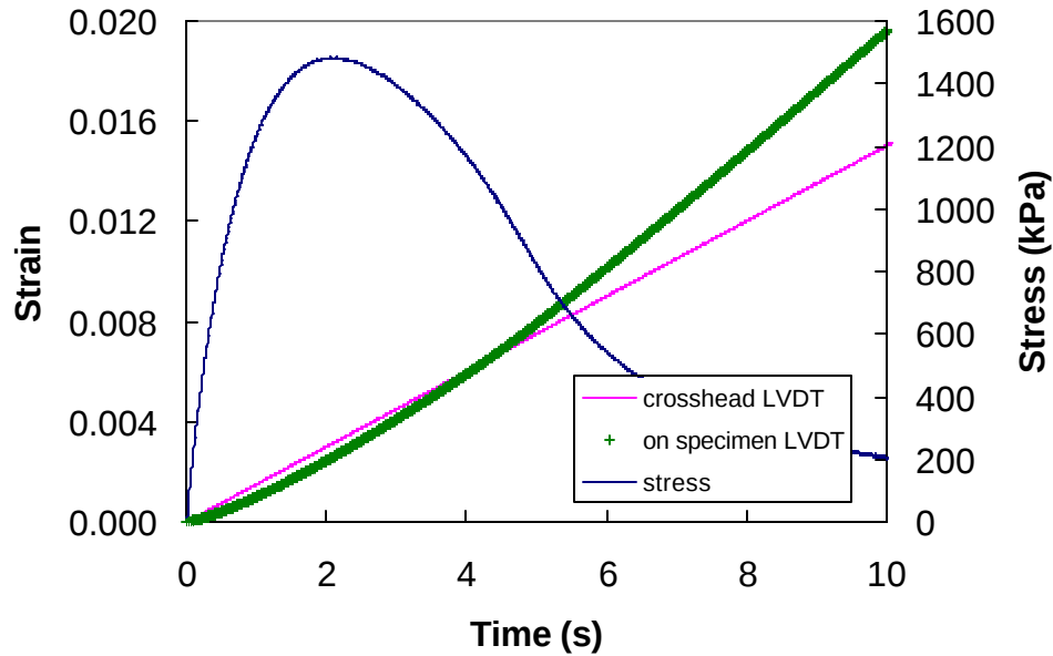
Figure 6.12 Constant Crosshead Rate Test
