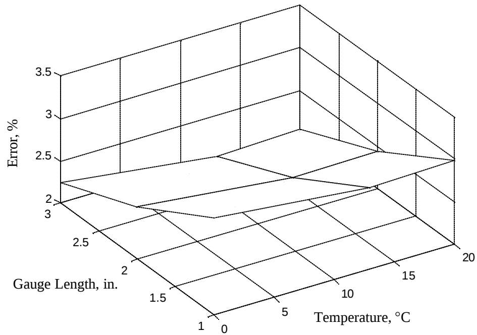
Figure 7.23 Effect of Bulging on Horizontal Measurement
