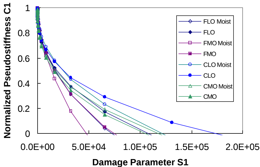
Figure 6.35 Effect of Moisture on Characteristic C_1 versus S_1 Curves
