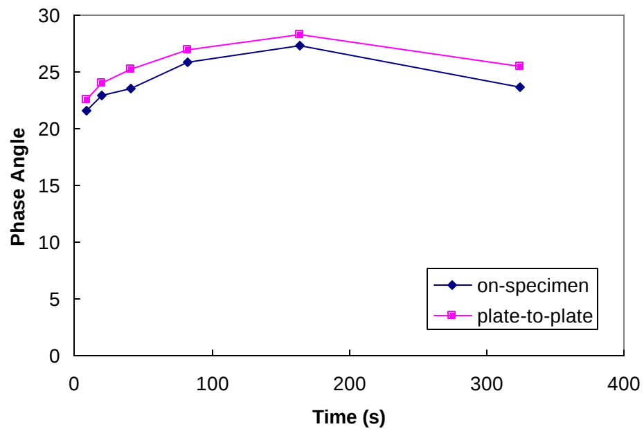
Figure 4.8 Phase Angle as a Function of Time from On-Specimen and Plate-to-Plate LVDT Measurements
