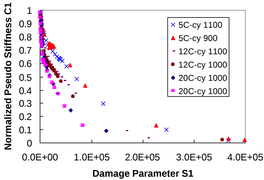
Figure 6.28 Characteristic C_1 versus S_1 Curves for Cyclic Testing at Two Strain Amplitudes and Three Temperatures on CML Mixture
