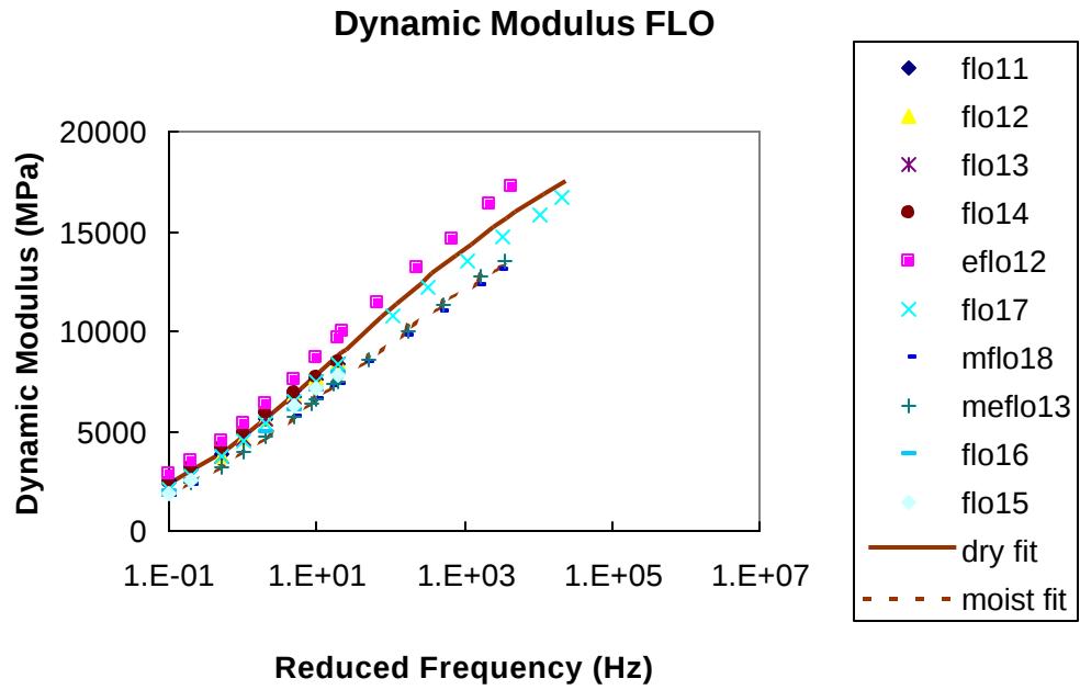
Figure D.1 Dynamic Modulus Master Curves for FLO Mixture
