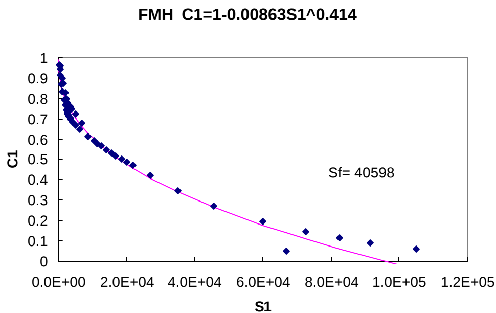
Figure D.14 Characteristic Curve for Cyclic FMH Data
