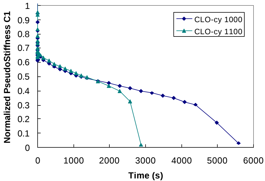
Figure 6.21 Normalized Pseudo stiffness as a Function of Time for CLO Mixture Tested at Two 10 Hz Cyclic Strain Amplitudes
