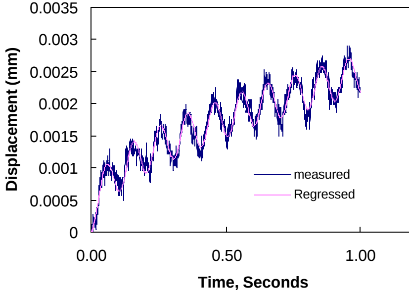
Figure 7.13 Measured and Regressed Horizontal Displacements
