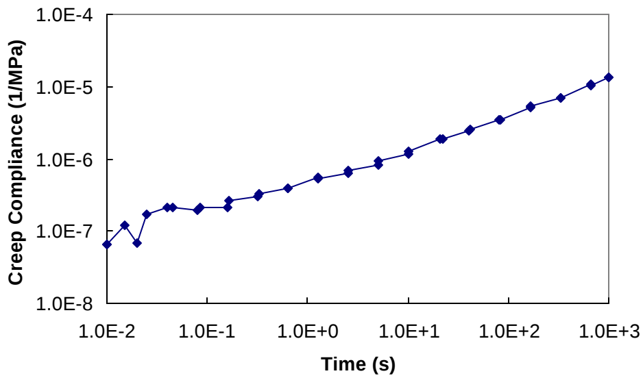
Figure 4.4 Typical Creep Compliance Curve
