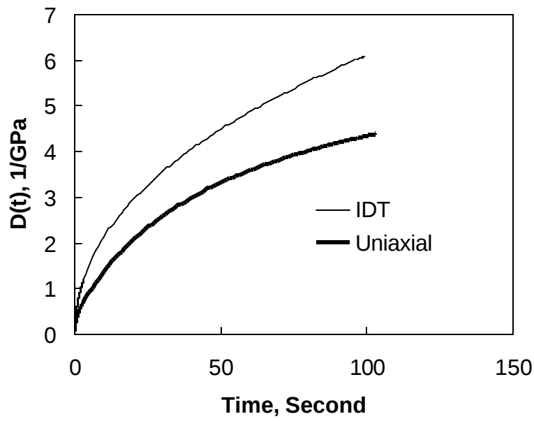
Figure 7.6 Comparison of Creep Compliance from IDT and Uniaxial Test
