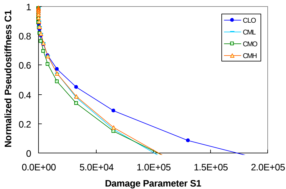
Figure 6.30 Characteristic C_1 versus S_1 Curves for Coarse Mixtures
