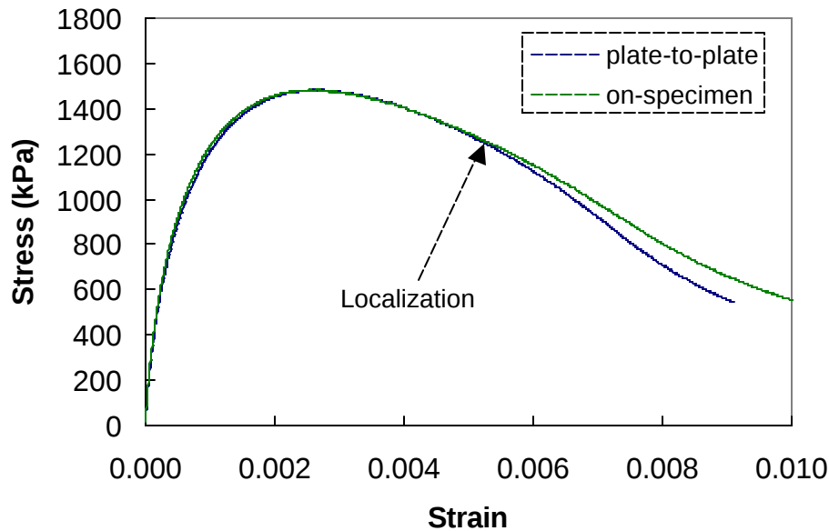
Figure 6.34 Point of Localization in a Constant Crosshead Rate Test
