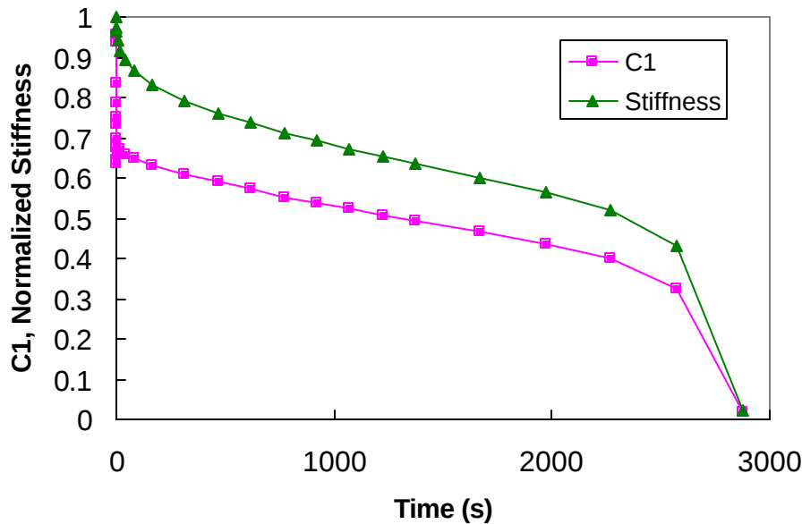
Figure 6.32 Normalized Stiffness and C_1 as a Function of Time for Specimen CLO7
