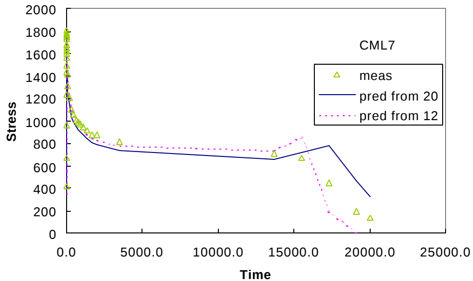
Figure D.48 Measured and Predicted Values for CML7 from 20C and 12C Curves
