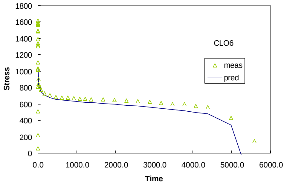
Figure D.41 Measured and Predicted Values for CLO6
