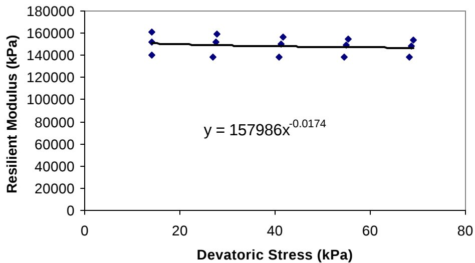
Figure D.25 Fill Resilient Modulus Data for WesTrack Section 2
