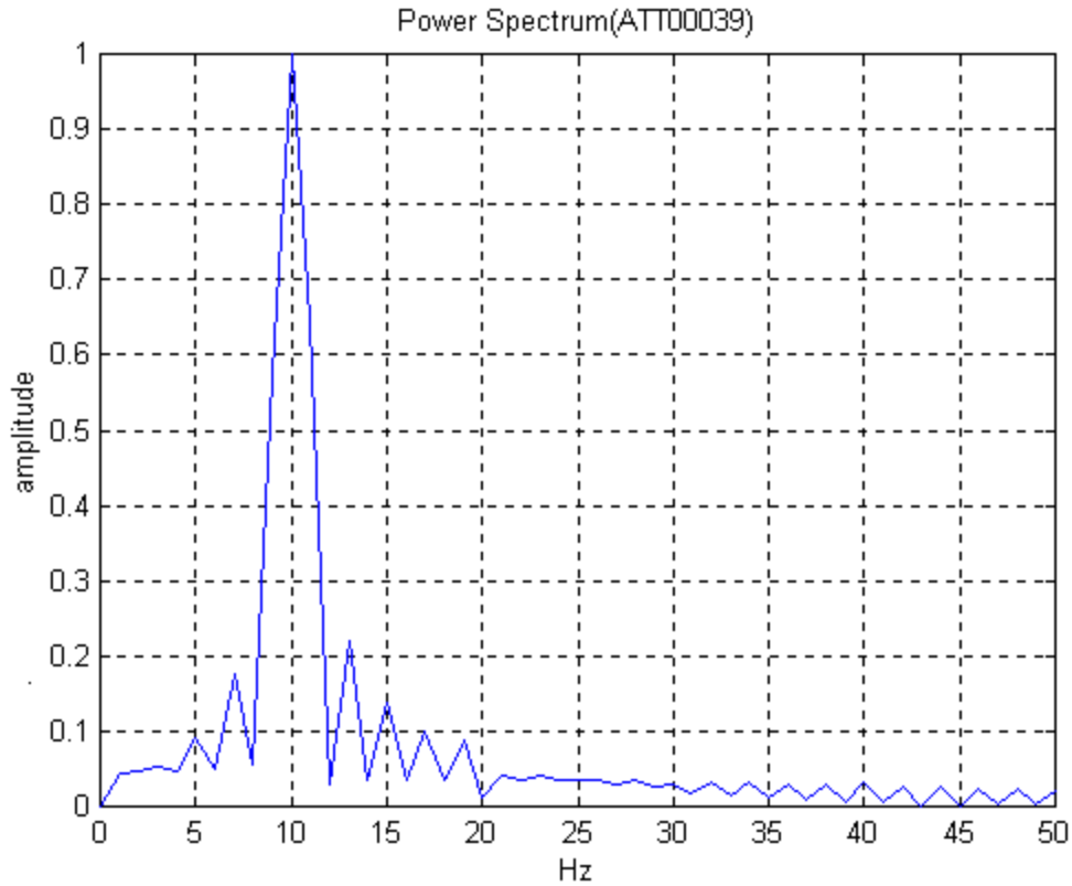
Figure 6.15 Power Spectrum from FFT Analysis of Cyclic Strain Data
