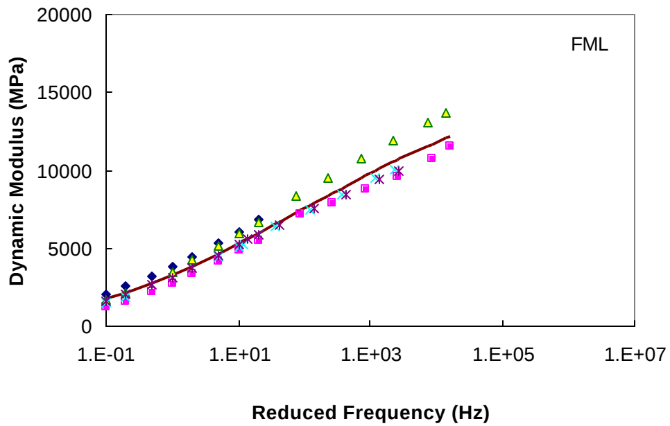
FIGURE C.2 Individual and Average Dynamic Modulus Curves for FML Mixture
