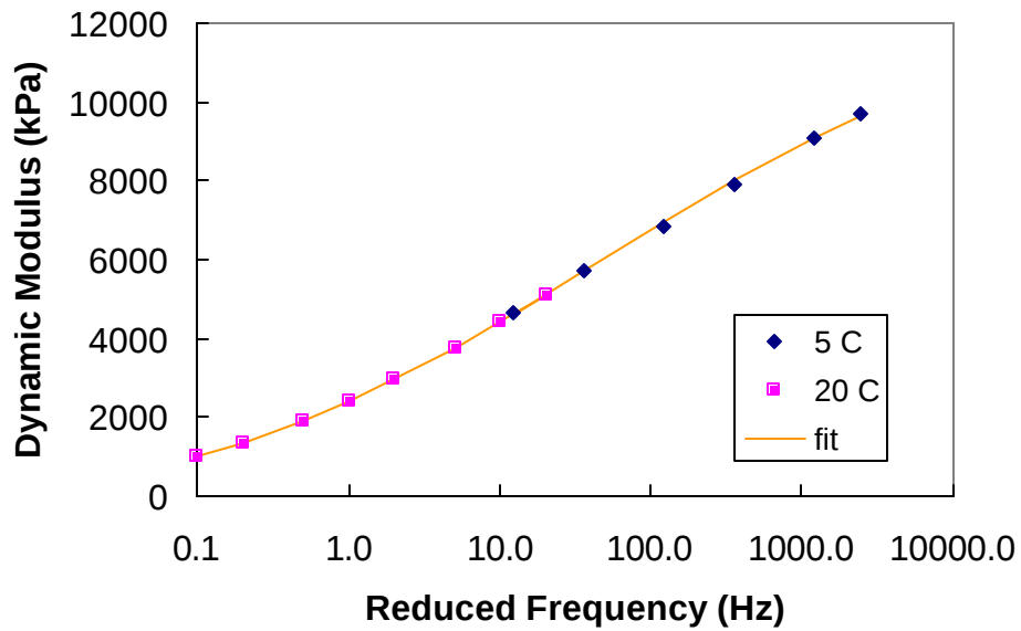
Figure 6.3 Dynamic Modulus Master Curve for Specimen FMO12 at Reference Temperature of 20°C
