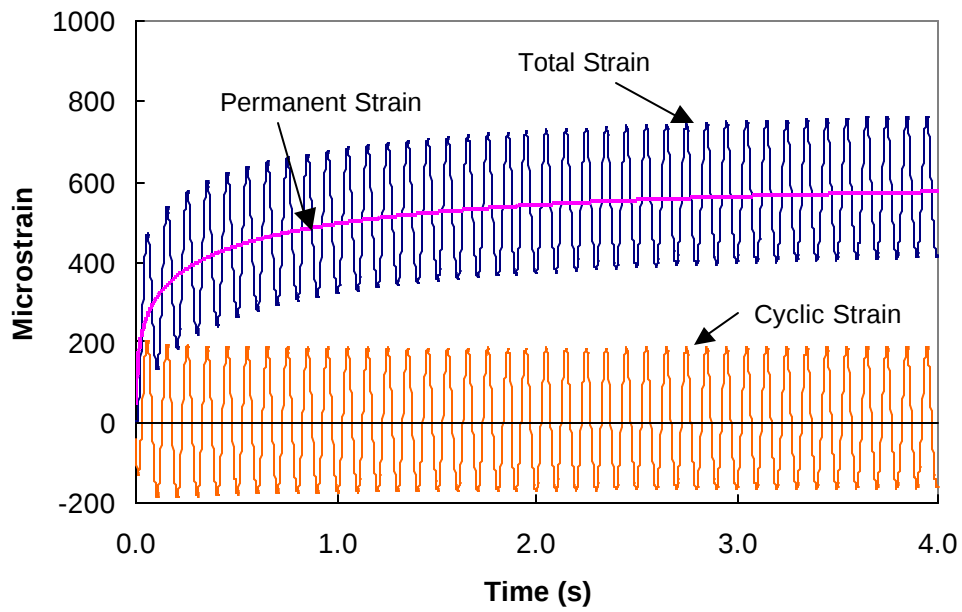
Figure 6.13 Total, Permanent, and Cyclic Strains
