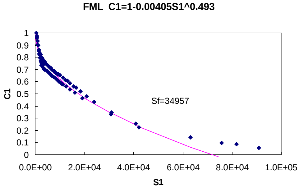
Figure D.11 Characteristic Curve for Cyclic FML Data
