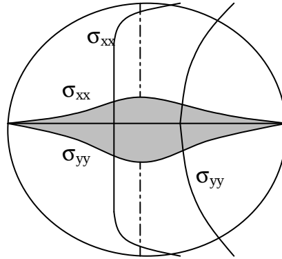
Figure 3.3 Stress Distribution along Horizontal and Vertical Diameters
