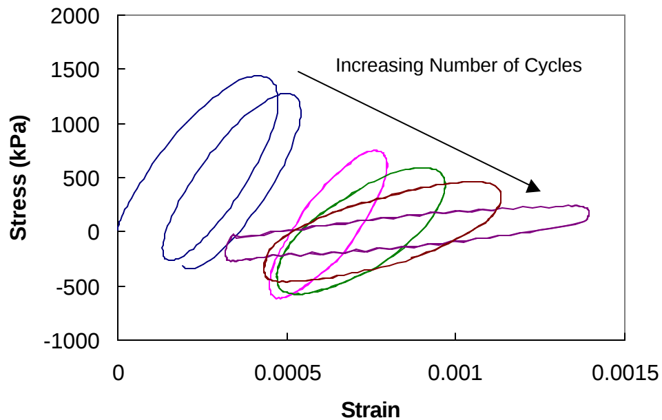
Figure 4.6 Stress-Strain Loops in Cyclic Test Measured Using LVDT Displacements
