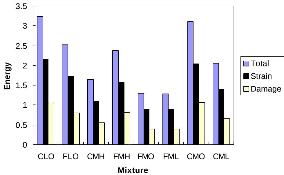
Figure 8.18 Fracture Energies for All Mixtures
