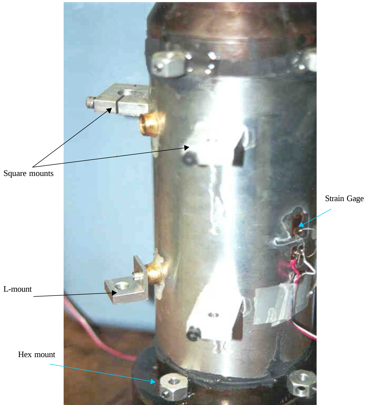
FIGURE B.5 Different LVDT Mount Types on Aluminum Specimen
