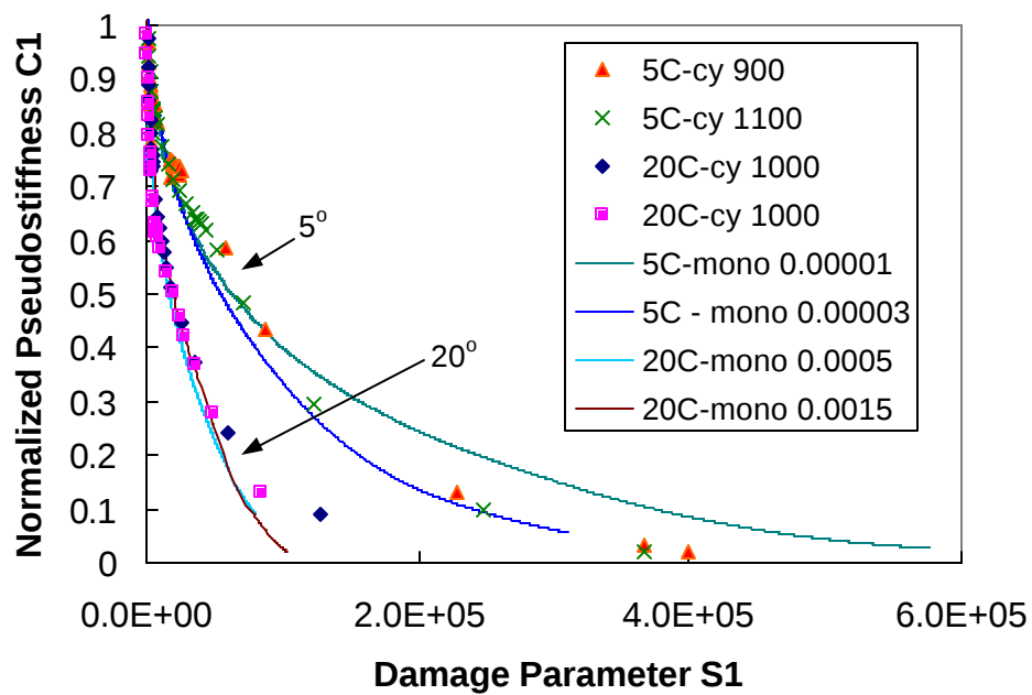
Figure 6.39 Characteristic C_1 versus S_1 Curves for Cyclic and Monotonic Testing on CML Mixture at Two Temperatures
