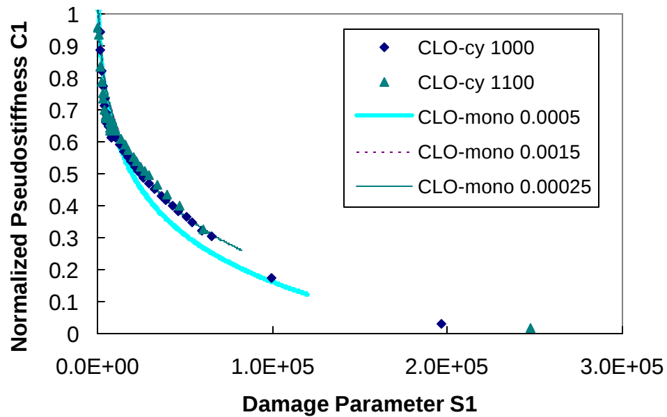
Figure 6.37 Characteristic C_1 versus S_1 Curve for Cyclic and Monotonic Testing on CLO Mixture at 20°C
