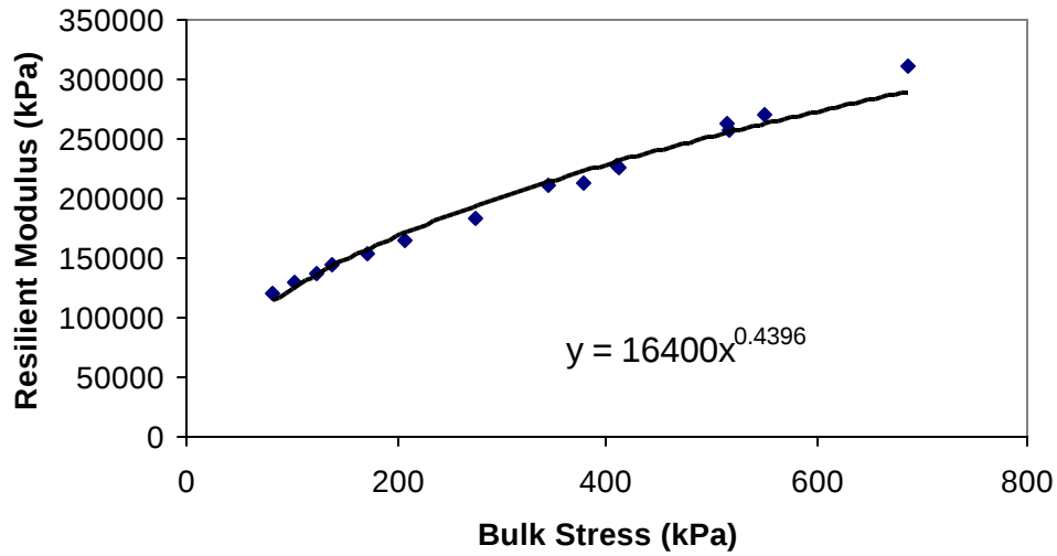
Figure D.24 ABC Resilient Modulus Data for WesTrack Section 22
