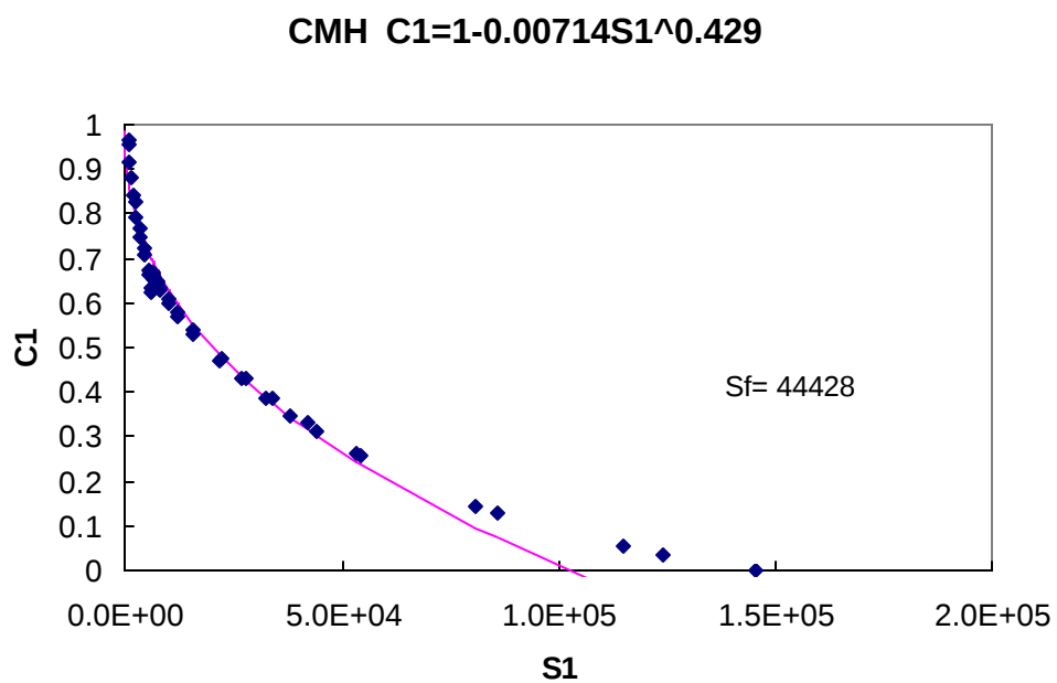
Figure D.19 Characteristic Curve for Cyclic CMH Data
