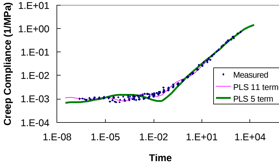
Figure A.7 Least Squares Method for Power Law Series Fit
