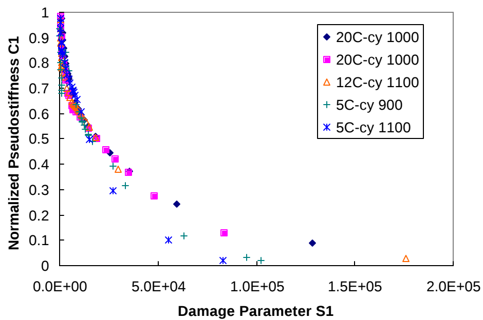
Figure 2.4 Cyclic Characteristic C_1 versus S_1 Curves Shifted to Reference Temperature of 20°C for CML Mixture
