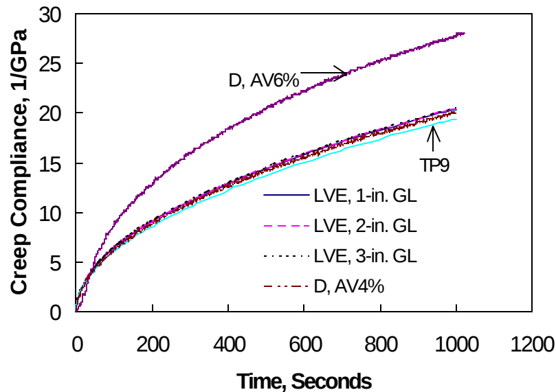
Figure 7.19 Finite Element Analysis Results for Case I
