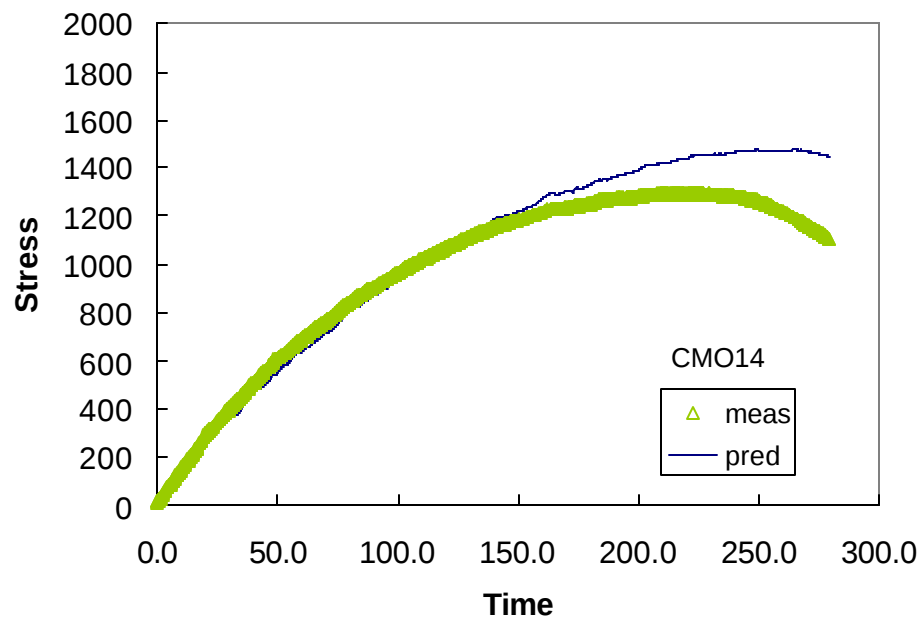
Figure D.32 Measured and Predicted Values for CMO14
