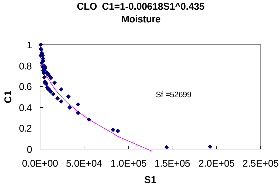
Figure D.16 Characteristic Curve for Moisture Cyclic CLO Data
