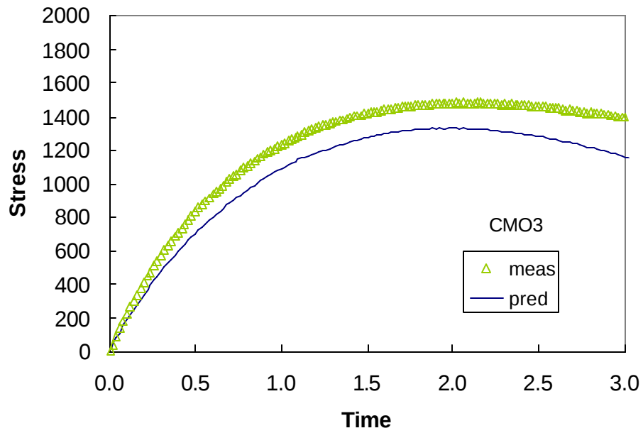
Figure D.31 Measured and Predicted Values for CMO3
