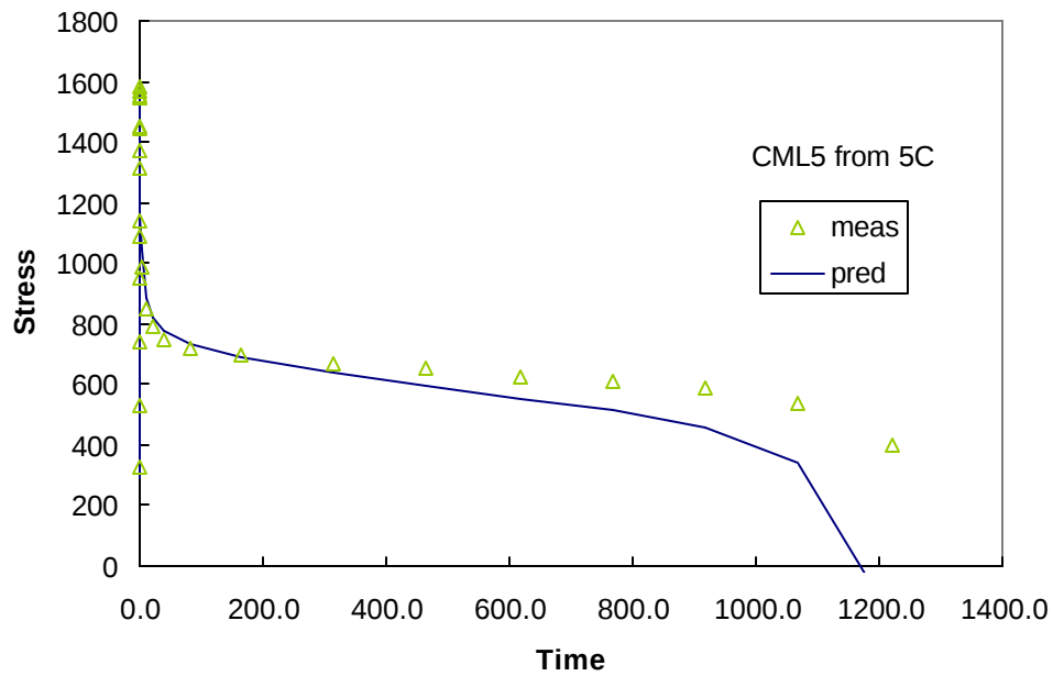
Figure D.45 Measured and Predicted Values for CML5 from 5C Curve
