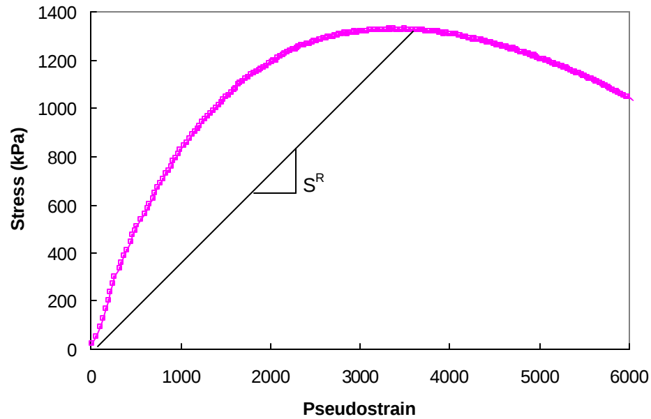
Figure 6.18 Definition of Pseudo stiffness
