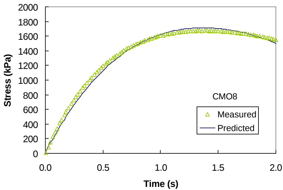
Figure 6.41 Measured and Predicted Stress Values for CMO8 Monotonic Test
