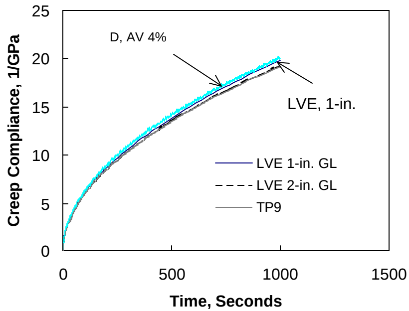
Figure 7.21 Finite Element Results for Case III
