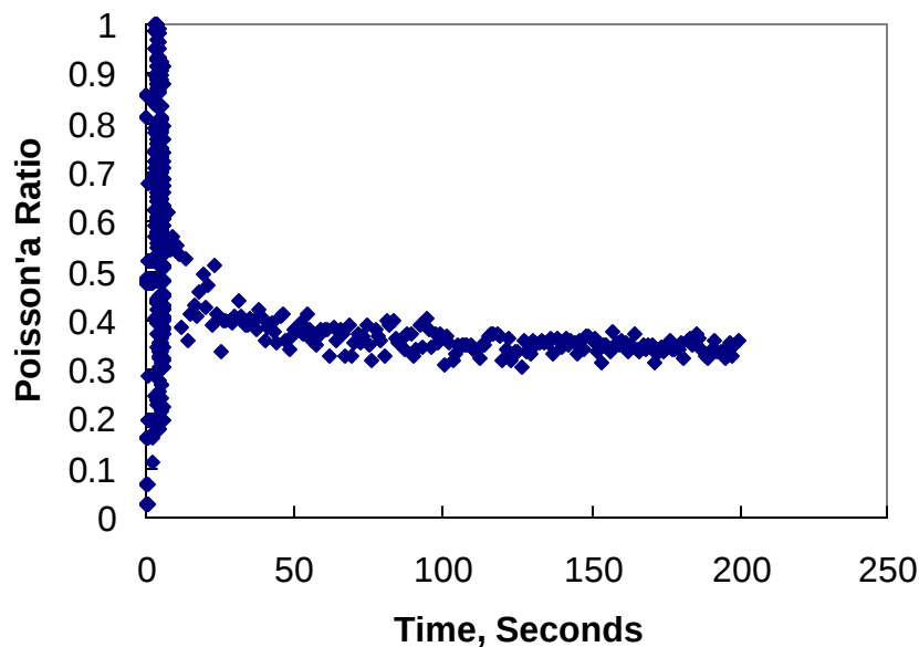
Figure 8.1 Poisson's Ratio in Creep Test
