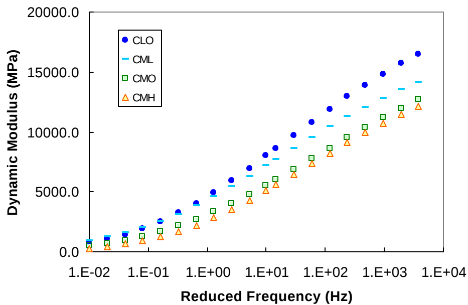
Figure 6.5 Dynamic Modulus Master Curves for Coarse Mixtures
