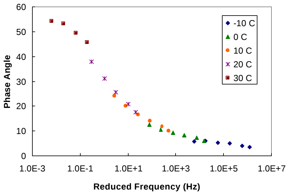
Figure A.6 Master Phase Angle Curve Created Using Shift Factors in Figure A.5
