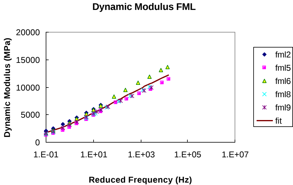
Figure D.2 Dynamic Modulus Master Curves for FML Mixture
