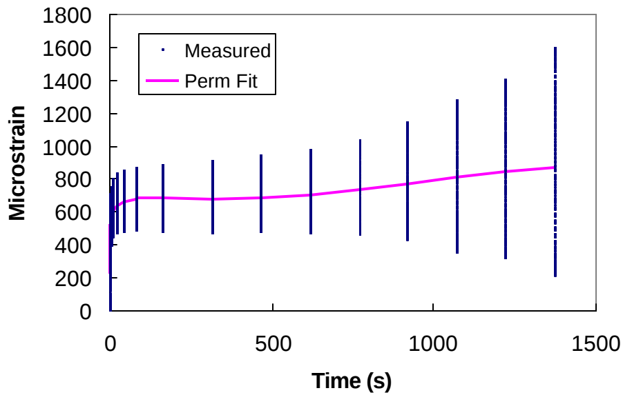
Figure 6.14 Entire Strain History for Cyclic Fatigue Test
