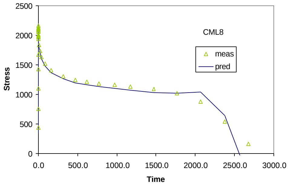
Figure D.44 Measured and Predicted Values for CML8
