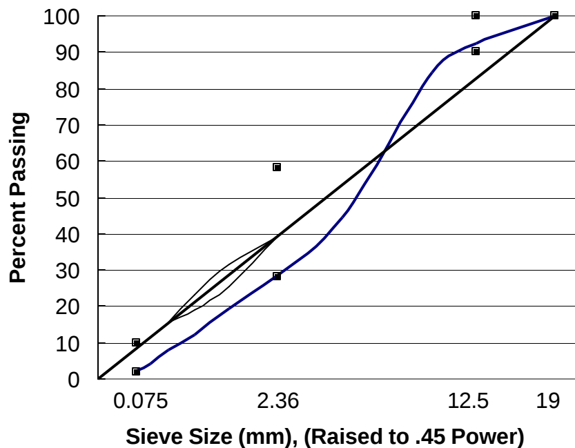
Figure 5.1 Aggregate Gradation of North Carolina Mix
