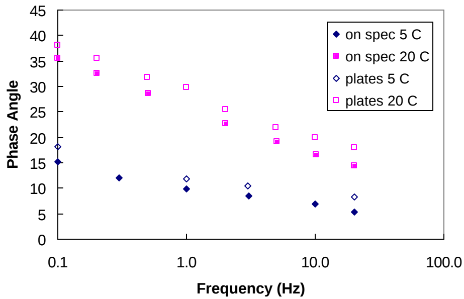
Figure 6.2 Phase Angle Values for Specimen FMO12 at 20°C and 5°C
