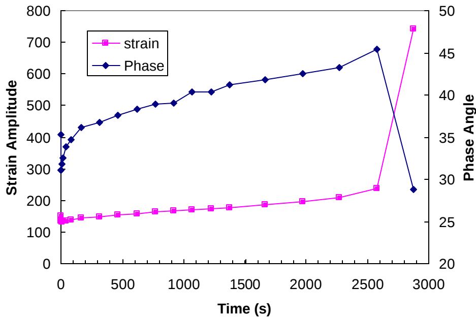
Figure 6.33 Phase Angle and On-Specimen LVDT Microstrain Amplitude as a Function of Time for Specimen CLO7
