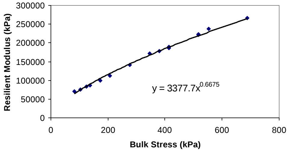
Figure D.22 ABC Resilient Modulus Data for WesTrack Section 6
