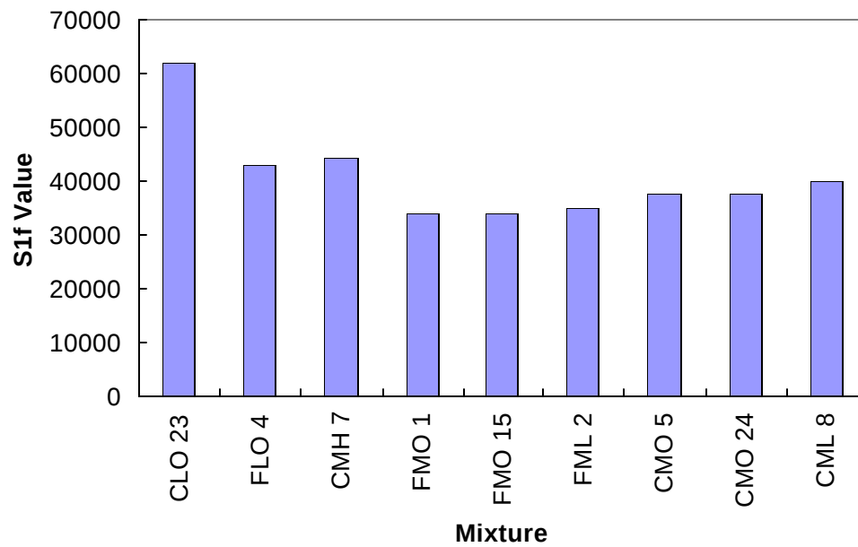
Figure 8.14 Comparison of S_{1f} Values among Mixtures
