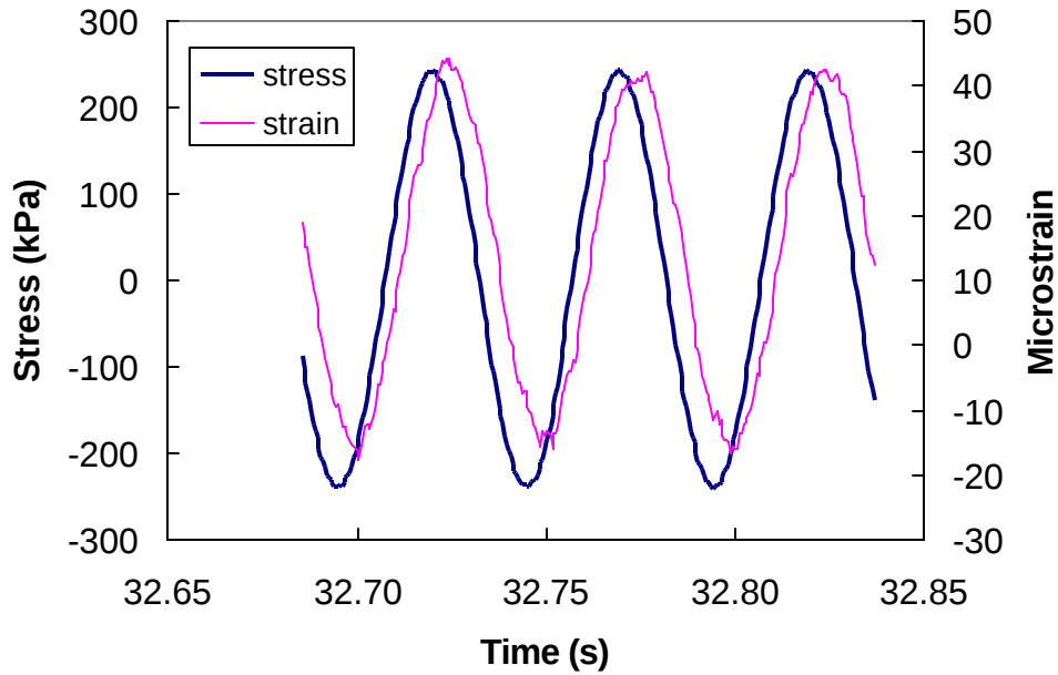
Figure 4.1 Frequency Sweep Test
