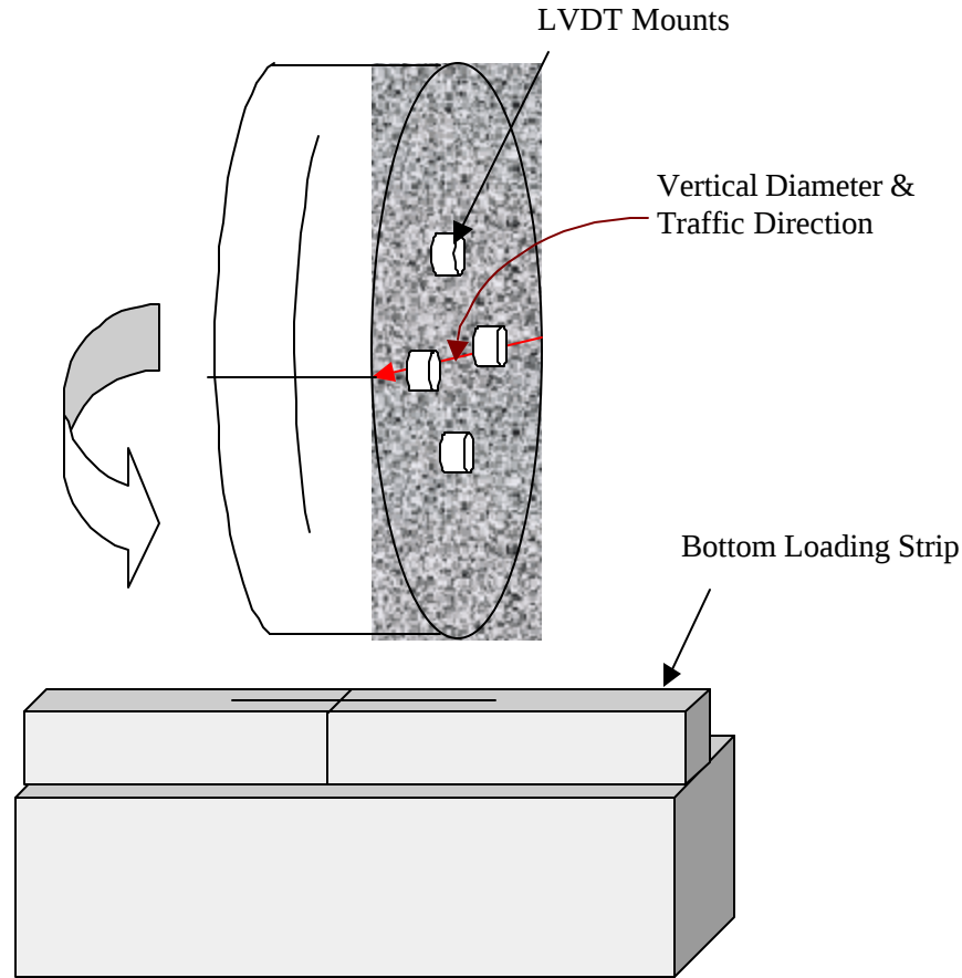
Figure 5.9 Positioning Specimen on Loading Strip
