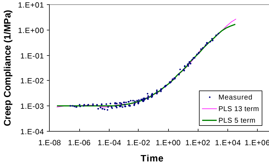
Figure A.8 Weighted Least Squares Method for Power Law Series Fit
