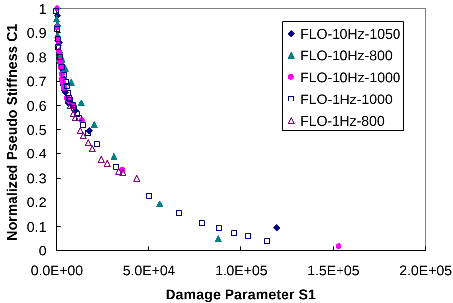
Figure 2.3 Characteristic C_1 versus S_1 Curve for 10 Hz and 1 Hz Cyclic Testing at 20°C on FLO Mixture at Several Strain Amplitudes (Crosshead Microstrain Values Range between 800 and 1050)
