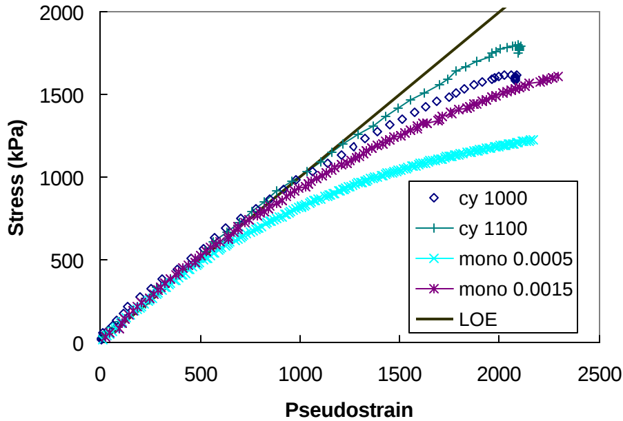
Figure 6.19 Initial Stress-Pseudo strain Curves for Cyclic and Monotonic Tests on CLO Mixture
