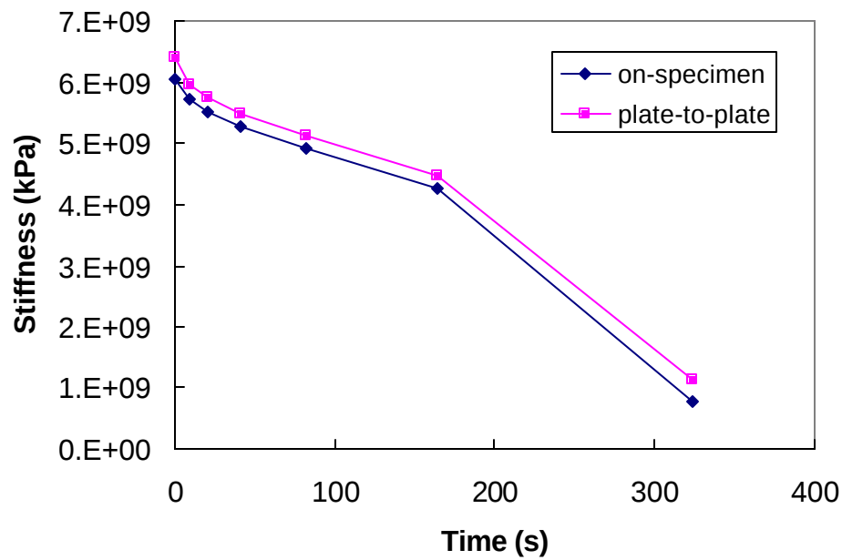
Figure 4.7 Stiffness Reduction over Time from On-Specimen and Plate-to-Plate LVDT Measurements
