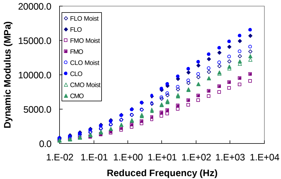
Figure 6.9 Effect of Moisture on Dynamic Modulus
