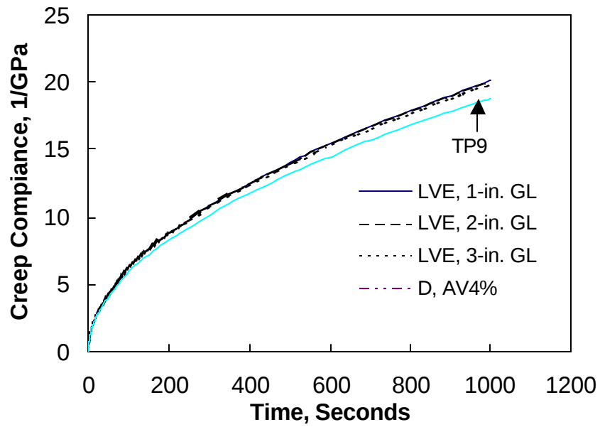
Figure 7.20 Finite Element Analysis Result for Case II
