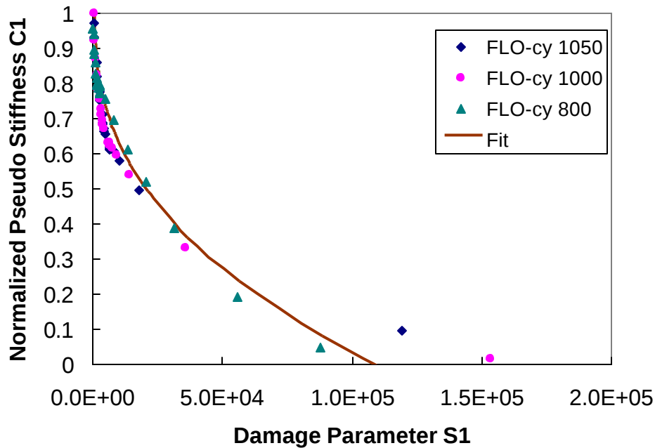
Figure 6.24 Characteristic C_1 versus S_1 Curve for FLO Mixture Tested at Three 10 Hz Cyclic Strain Amplitudes
