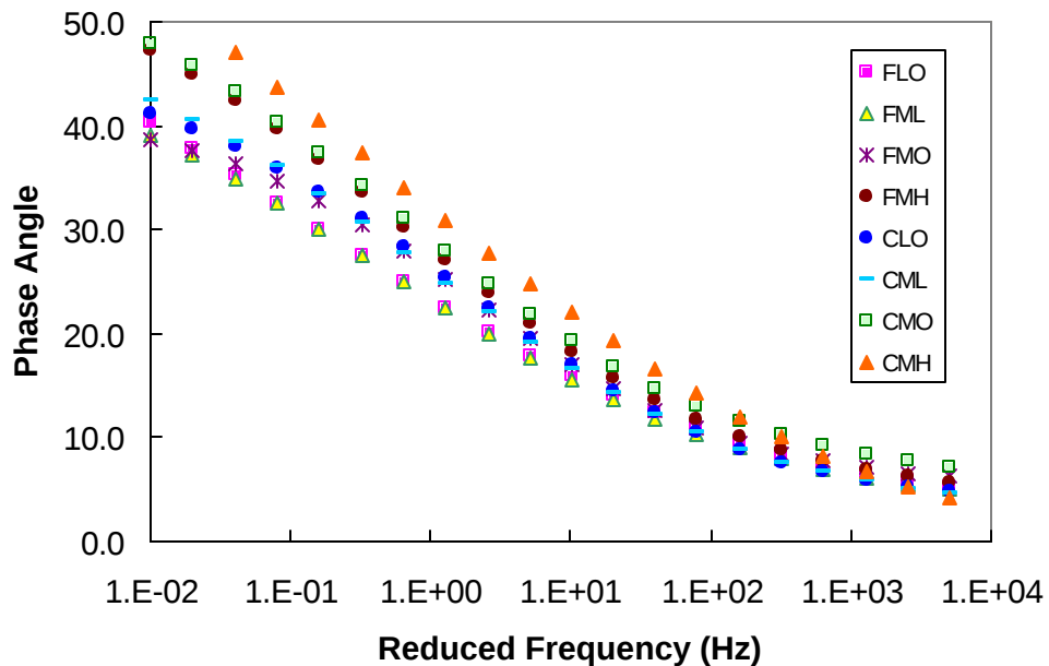
Figure 6.8 Phase Angle Master Curves for All Mixtures
