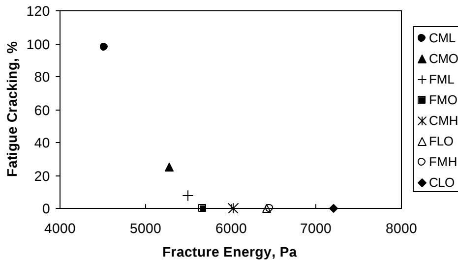
Figure 8.6 Evaluation of Fracture Energy As a Performance Indicator Using LMLC Specimens
