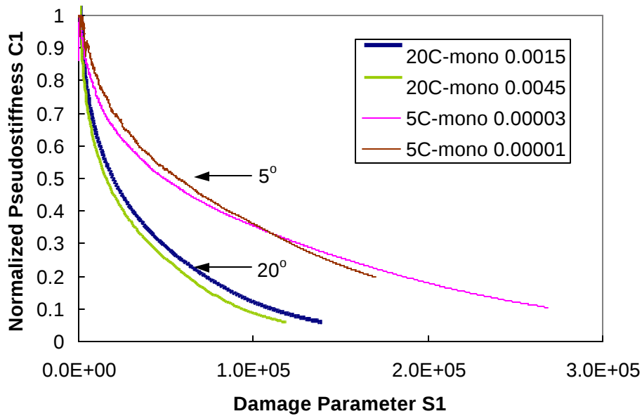
Figure 6.27 Characteristic C_1 versus S_1 Curves for Monotonic Testing at Two Rates and Temperatures on CMO Mixture
