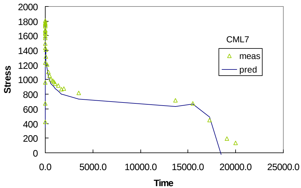
Figure D.43 Measured and Predicted Values for CML7
