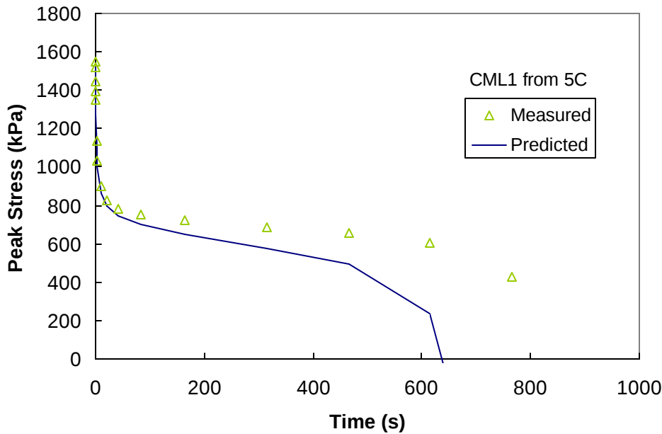
Figure 6.45 Measured and Predicted Stress Values from 5°C for CML1 Cyclic Test
