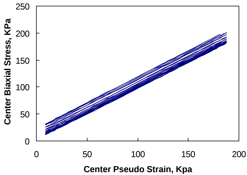
Figure 7.17 Biaxial Stress vs. Pseudo Strain
