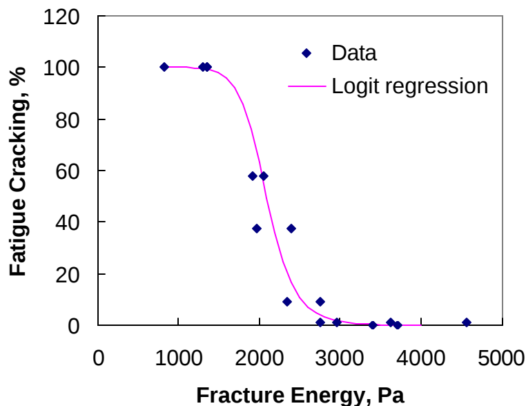
Figure 2.1 Relationship between Field Performance and Fracture Energy
