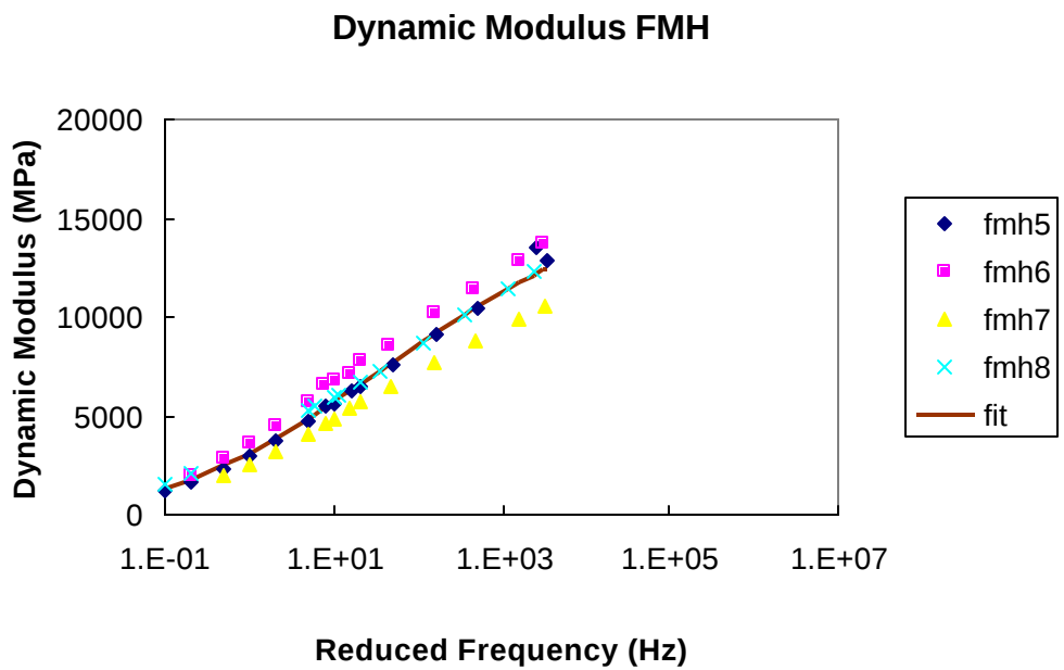
Figure D.4 Dynamic Modulus Master Curves for FMH Mixture
