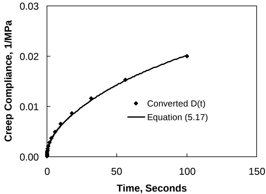
Figure 7.3 Verification of Creep Compliance Calculation
