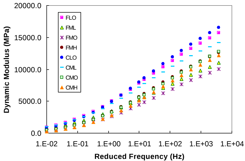
Figure 6.7 Dynamic Modulus Master Curves for All Mixtures
