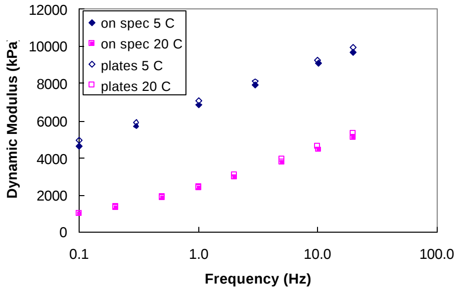
Figure 6.1 Dynamic Modulus Values for Specimen FMO12 at 20°C and 5°C
