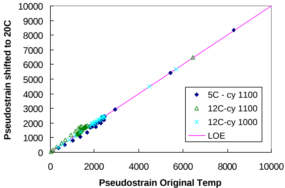
Figure 6.46 Pseudo strains Calculated at 20°C and at Original Test Temperature
