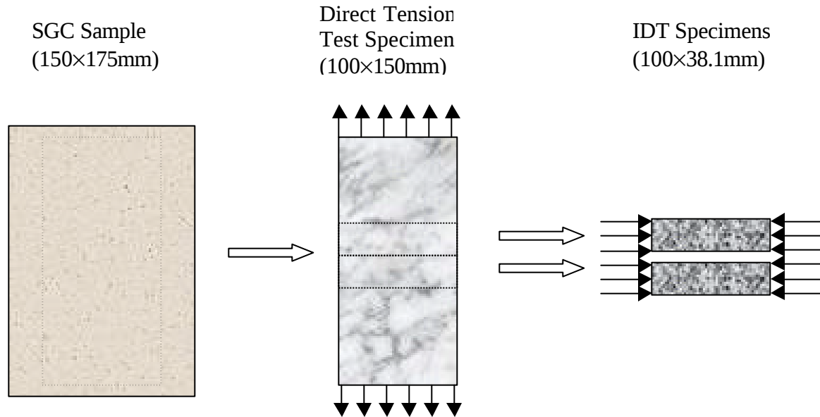
Figure 7.5 Preparation for Direct Tension Specimen and Indirect Tension Specimen
