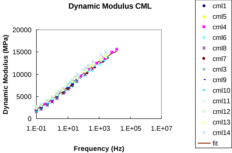
Figure D.6 Dynamic Modulus Master Curves for CML Mixture
