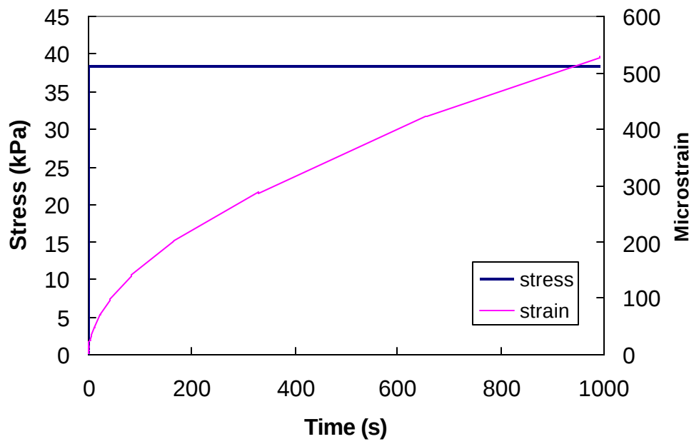
Figure 4.3 Creep Test
