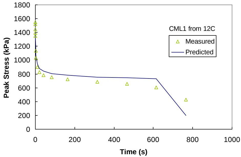
Figure D.47 Measured and Predicted Values for CML1 from 12C Curve
