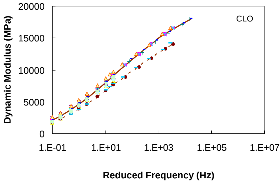
Figure 6.4 Dynamic Modulus Master Curves for CLO Mixture
