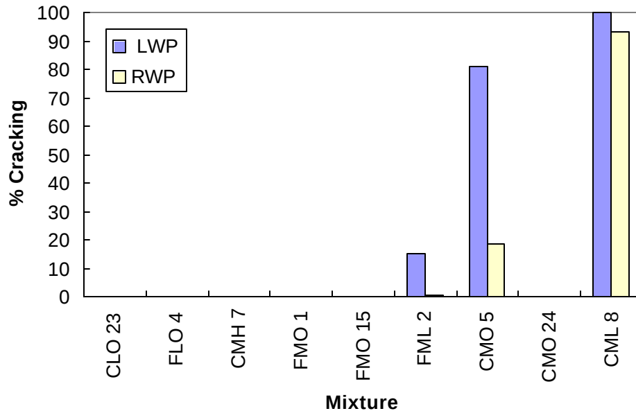
Figure 8.10 Field Performance of WesTrack Mixtures at 2.8 Million ESALs
