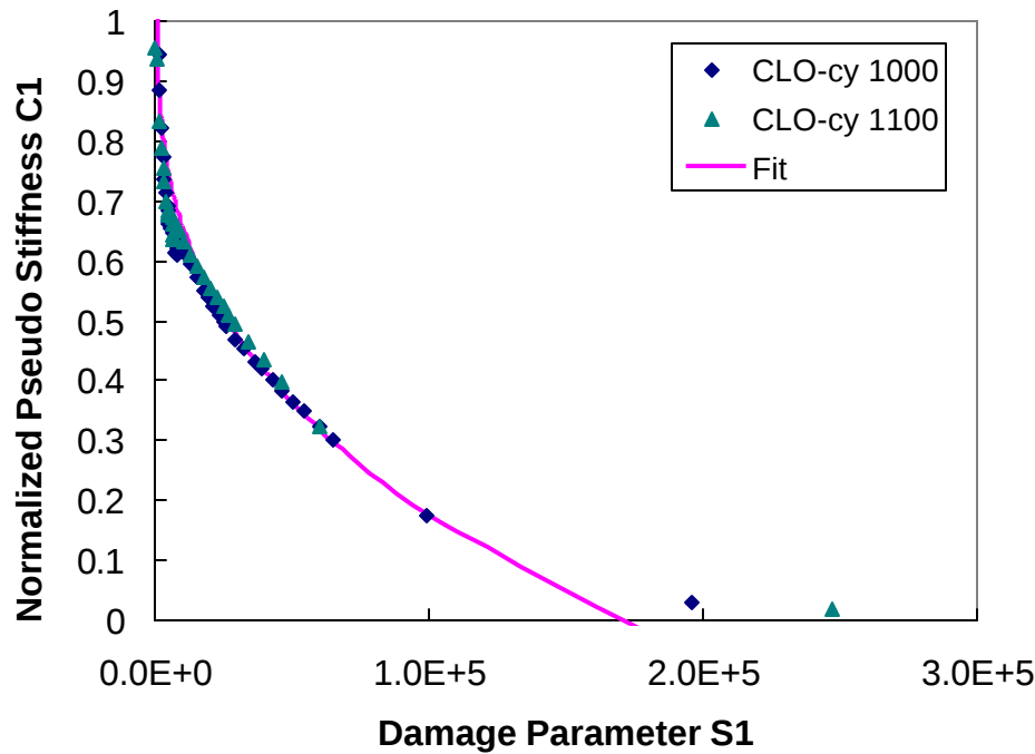
Figure 6.25 Characteristic C_1 versus S_1 Curve for CLO Mixture Tested at Two 10 Hz Cyclic Strain Amplitudes
