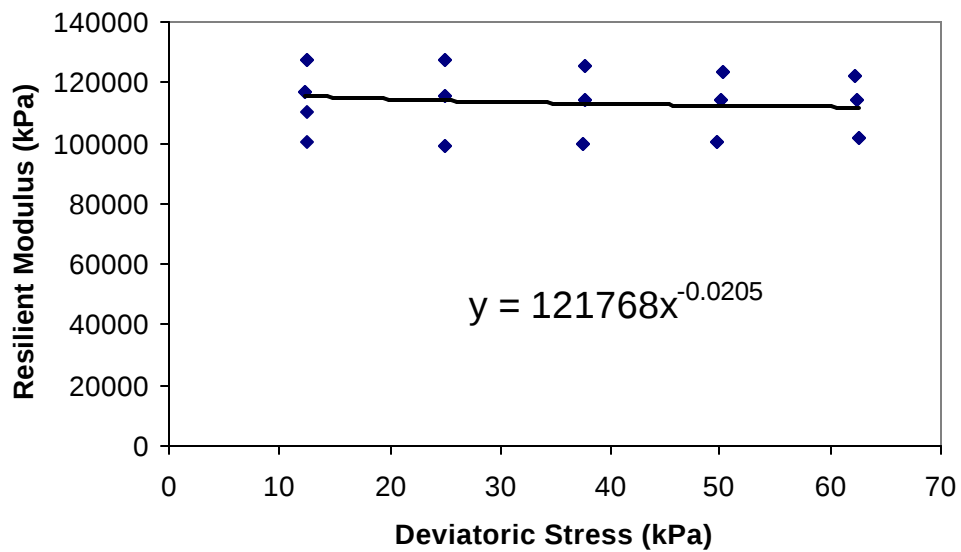
Figure D.27 Fill Resilient Modulus Data for WesTrack Section 9
