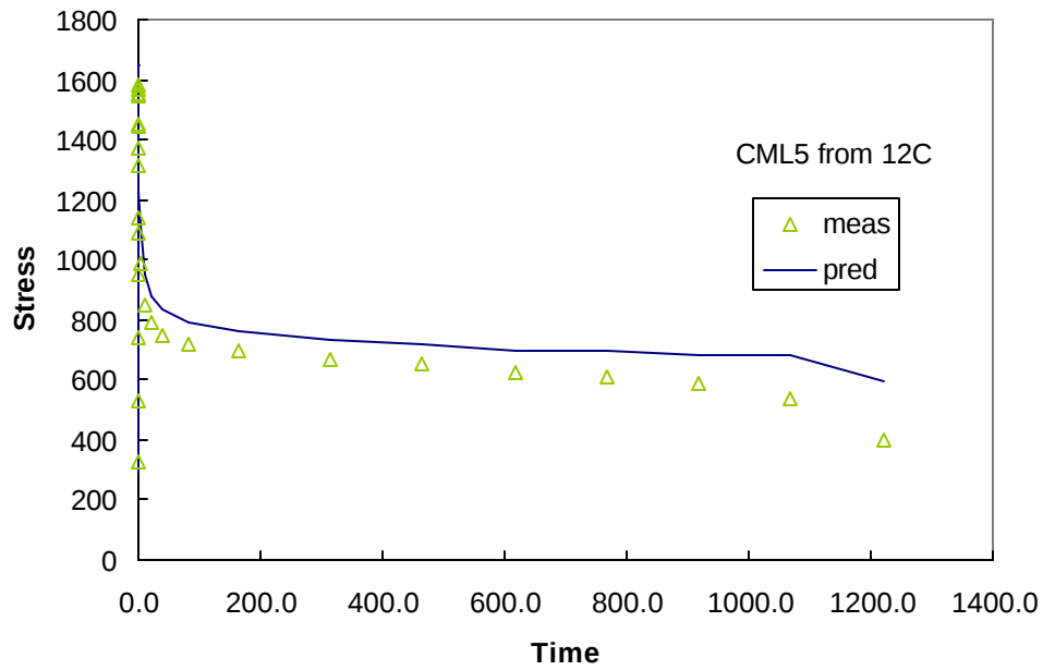
Figure D.46 Measured and Predicted Values for CML5 from 12C Curve
