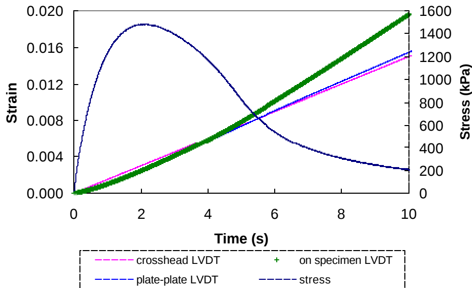
Figure 4.9 Stress and Strain Measurements for Constant Crosshead Rate Test
