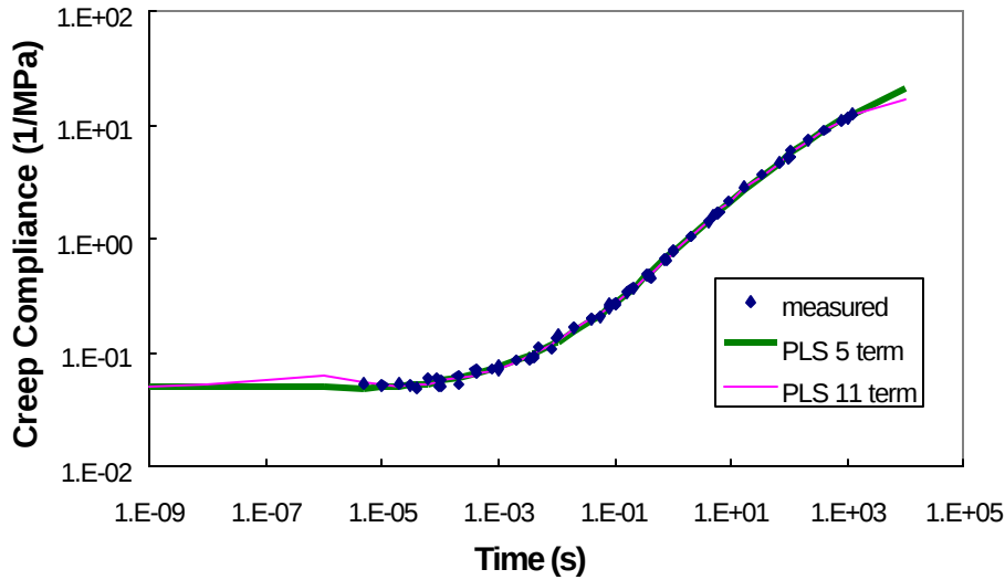
Figure A.9 Power Law Series Fit of Second Data Set
