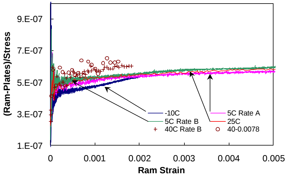
FIGURE B.3 Machine Compliance Evaluated at Different Temperatures and Crosshead Strain Rates for UTM Machine
