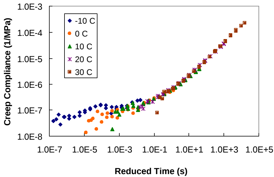
Figure A.3 Master Creep Compliance Curve at Reference Temperature of 20°C
