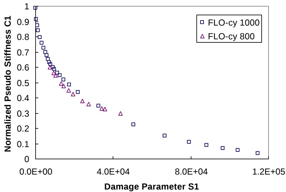
Figure 6.26 Characteristic C_1 versus S_1 Curve for 1 Hz Cyclic Testing on FLO Mixture at Two Strain Amplitudes
