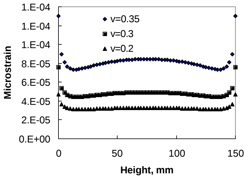
Figure 7.7 Strain Distribution along Axis of Uniaxial Direct Tension Specimen with End Plates
