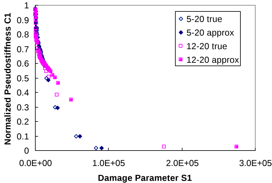
Figure 6.47 Effect of Pseudo Strain Approximation on Characteristic C_1 versus S_1 Curve
