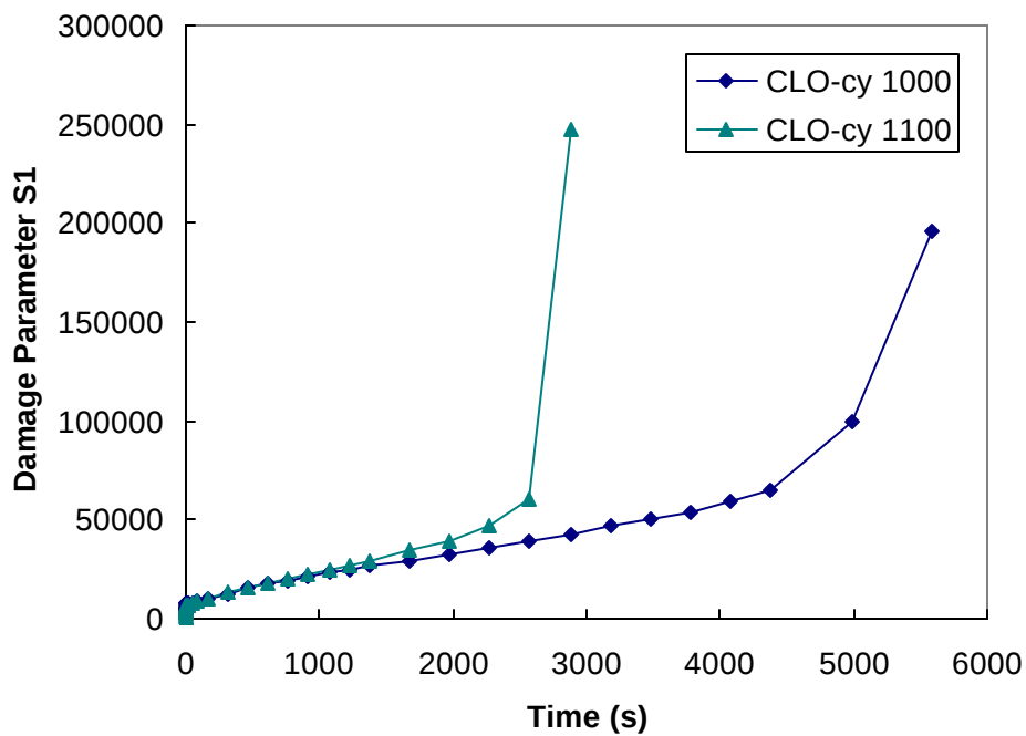
Figure 6.23 Damage Parameter as a Function of Time for CLO Mixture Tested at Two 10 Hz Cyclic Strain Amplitudes
