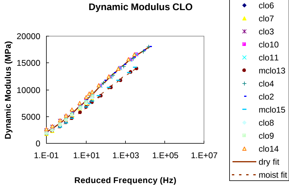
Figure D.5 Dynamic Modulus Master Curves for CLO Mixture
