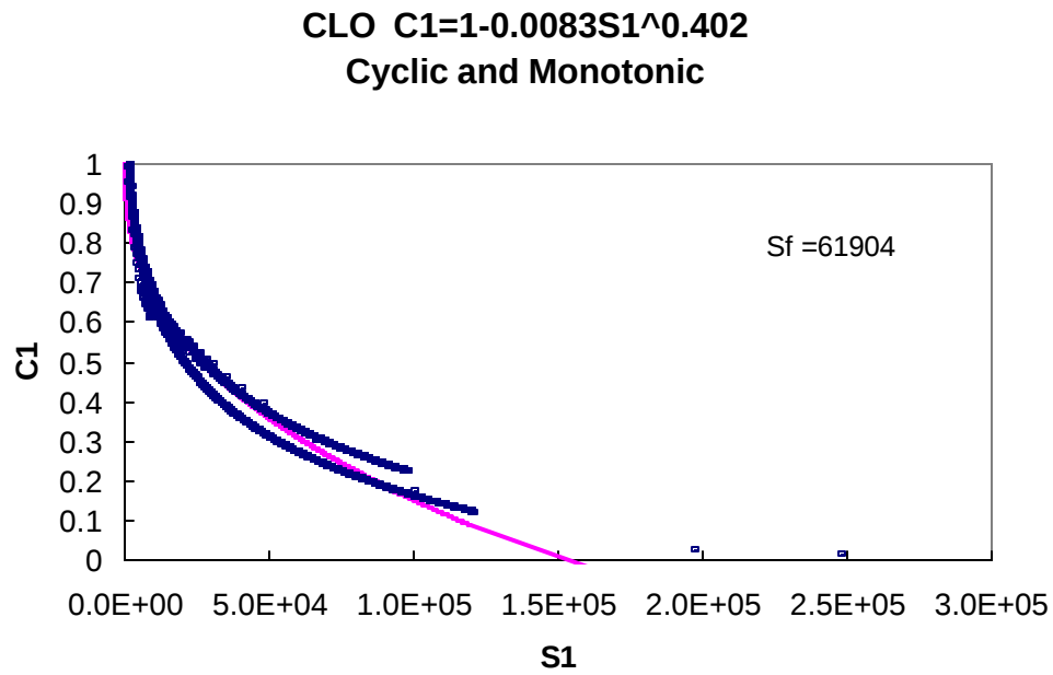
Figure D.15 Characteristic Curve for Cyclic and Monotonic CLO Data
