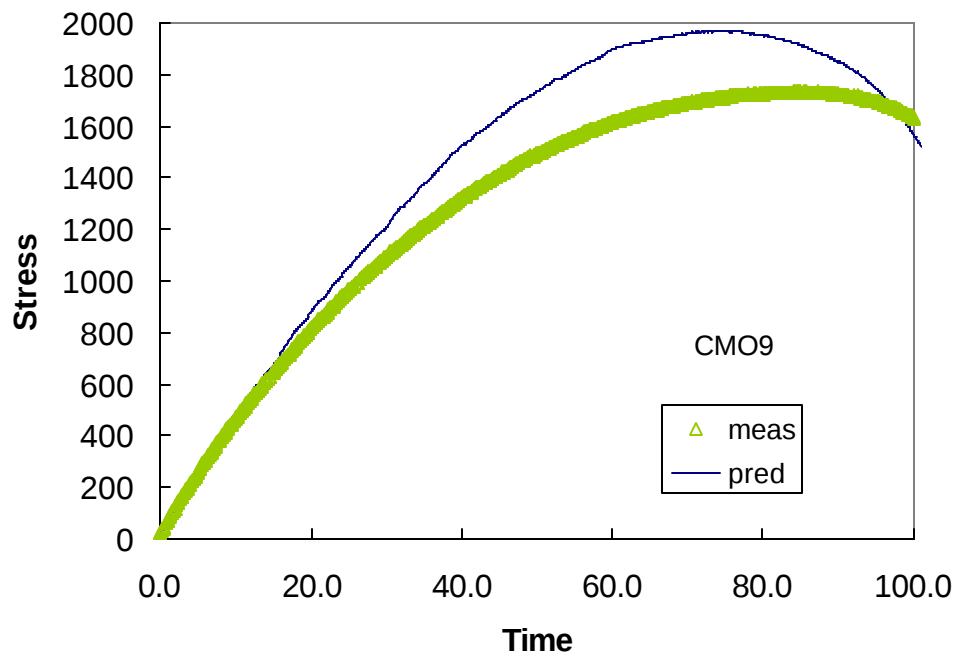
Figure D.33 Measured and Predicted Values for CMO9
