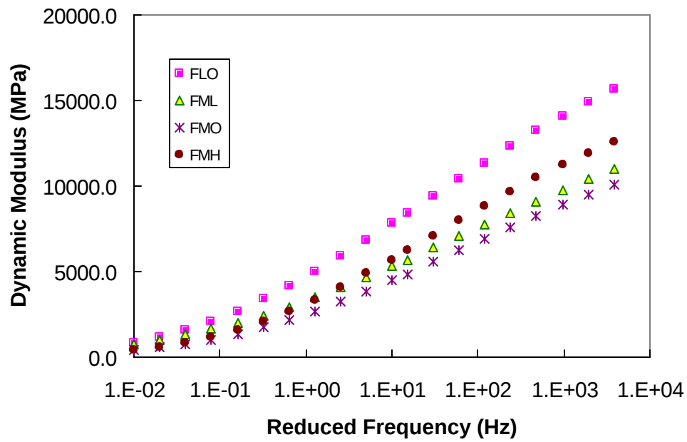
Figure 6.6 Dynamic Modulus Master Curves for Fine Mixtures
