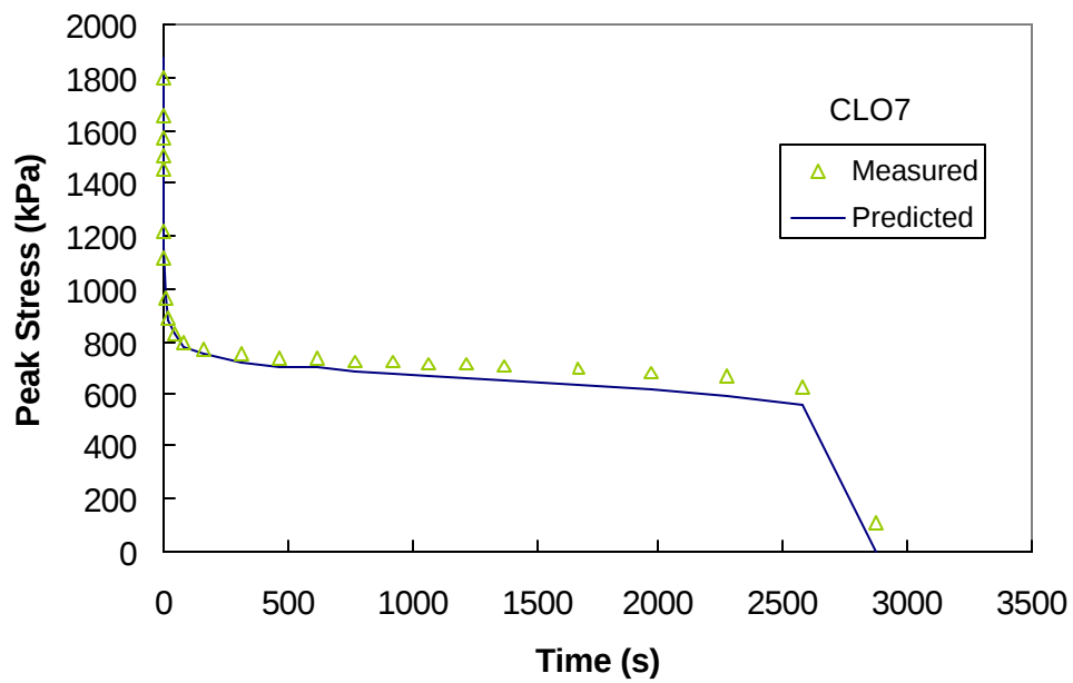
Figure 6.43 Measured and Predicted Stress Values for CLO7 Cyclic Test
