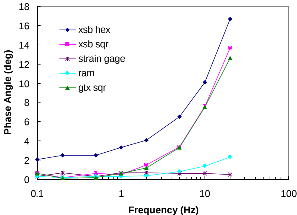
FIGURE B.6 Phase Angle Measurements from Aluminum Specimen Tested with MTS
