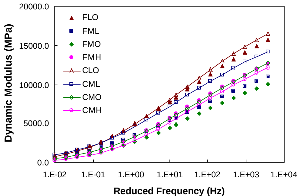
FIGURE C.1 AVERAGE DYNAMIC MODULUS CURVES FOR COARSE AND FINE WESTRACK MIXTURES
