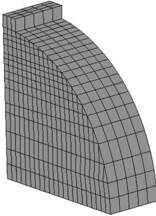
Figure 7.2 3-D Finite Element Model Mesh of Indirect Tension Specimen
