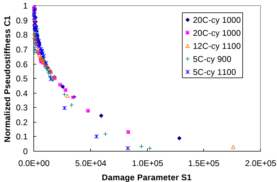
Figure 6.44 Cyclic Characteristic C_1 versus S_1 Curves Shifted to Reference Temperature of 20°C for CML Mixture
