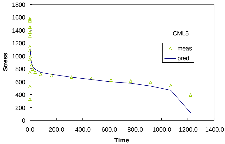
Figure D.42 Measured and Predicted Values for CML5
