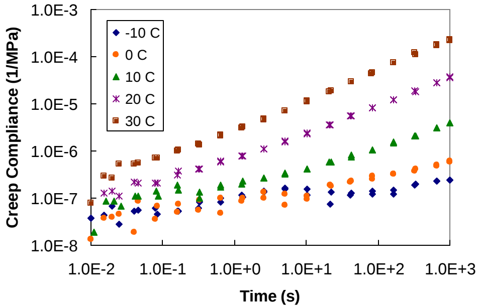
Figure A.1 Individual Creep Compliance Curves at Various Temperatures
