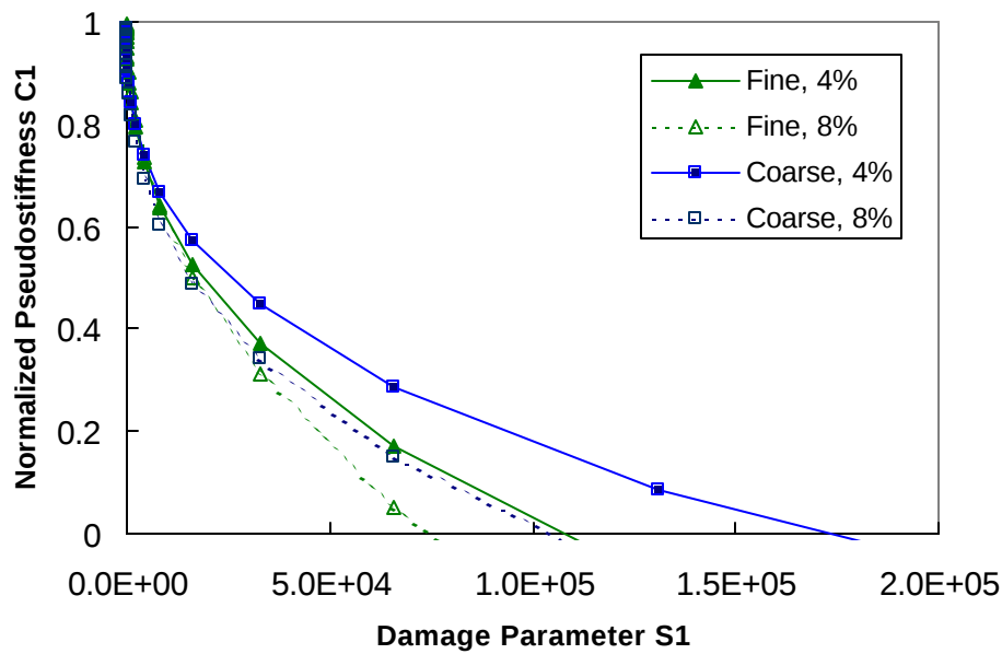
Figure 6.31 Comparison of Characteristic C_1 versus S_1 Curves for Coarse and Fine Gradations
