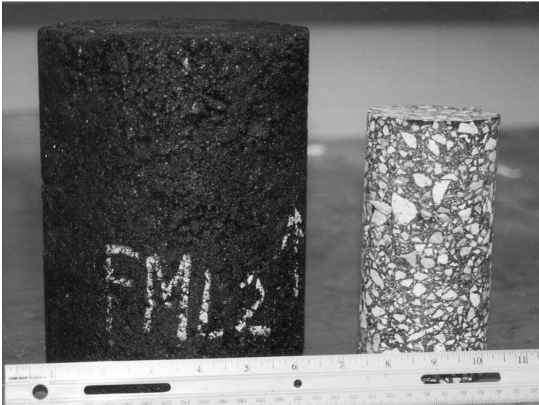
Figure 5.4 Whole and Cut Gyratory Specimens
