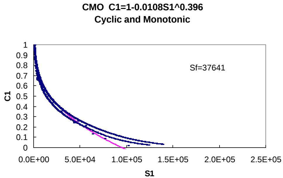
Figure D.17 Characteristic Curve for Cyclic and Monotonic CMO Data
