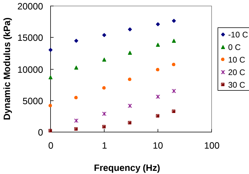
Figure A.2 Individual Dynamic Modulus Curves at Various Temperatures
