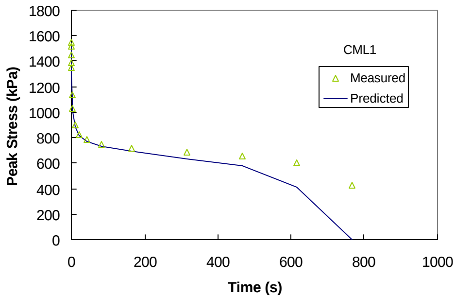
Figure 6.42 Measured and Predicted Stress Values for CML1 Cyclic Test
