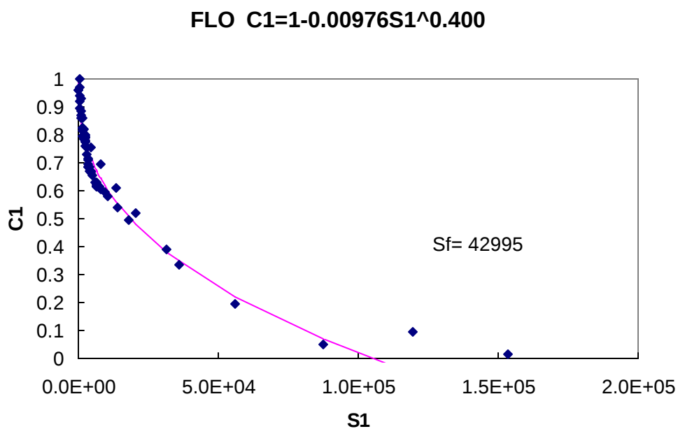
Figure D.9 Characteristic Curve for Cyclic FLO Data
