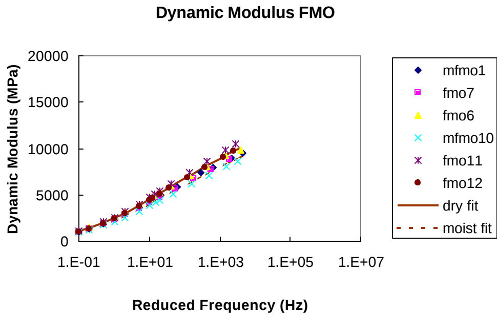
Figure D.3 Dynamic Modulus Master Curves for FMO Mixture
