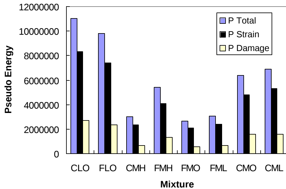
Figure 8.19 Fracture Pseudo Energies for All Mixtures
