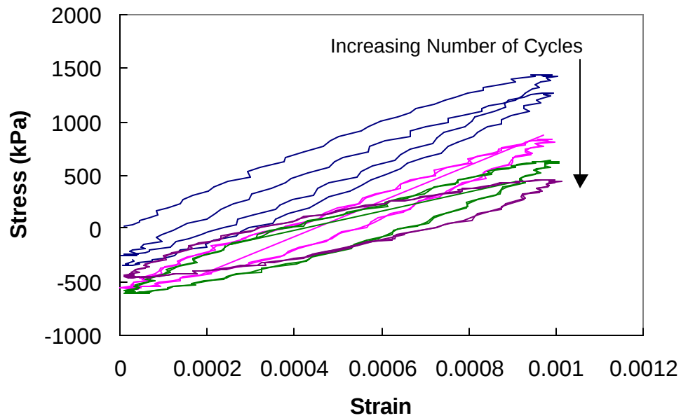
Figure 4.5 Stress-Strain Loops in Cyclic Test Measured Using Ram Displacements
