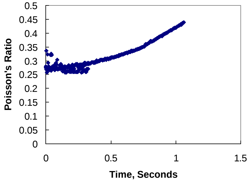
Figure 8.2 Poisson's Ratio in Tensile Strength Test
