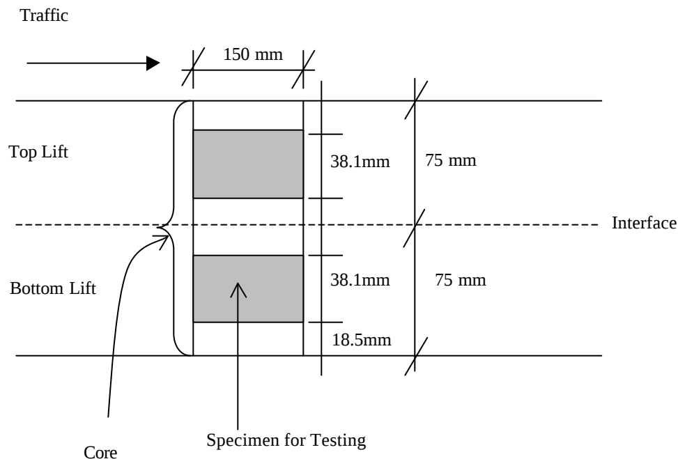
Figure 5.5 Locations of Specimens Cored from Field Core
