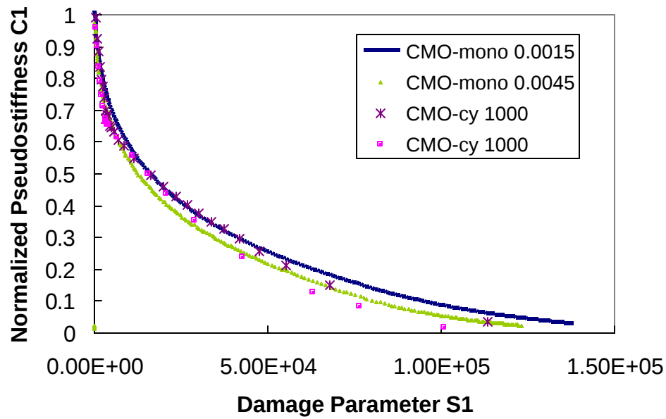
Figure 6.38 Characteristic C_1 versus S_1 Curve for Cyclic and Monotonic Testing on CMO Mixture at 20°C
