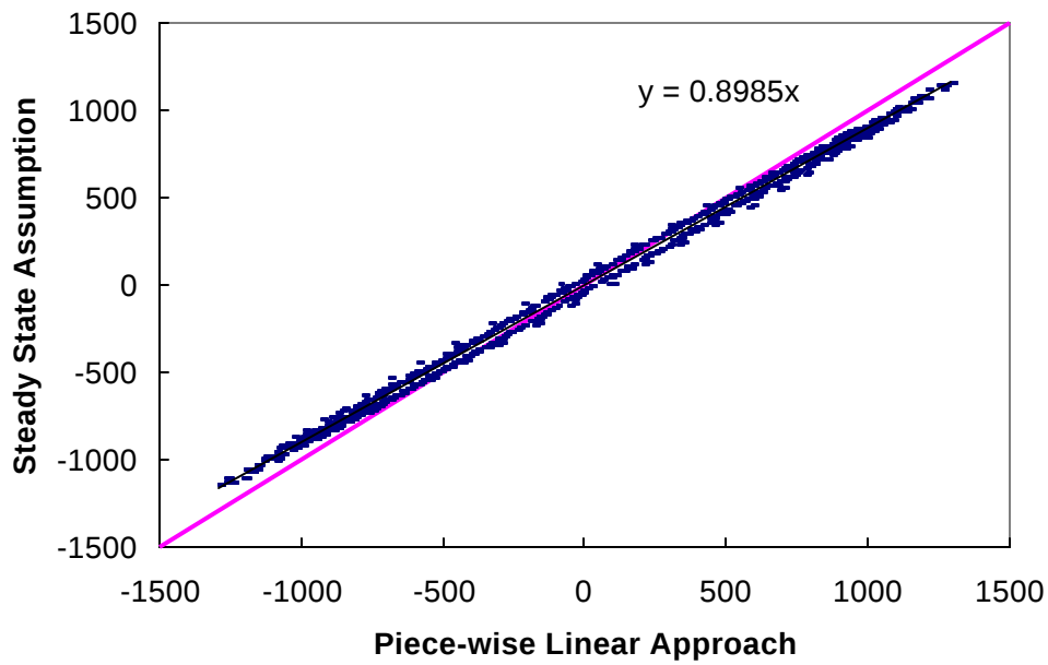
Figure 6.16 Comparison of Cyclic Pseudo strains Calculated Using Piece-Wise Linear Approach and Steady State Assumption
