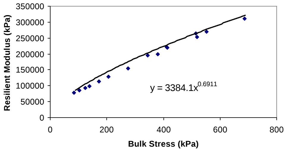
Figure D.23 ABC Resilient Modulus Data for WesTrack Section 15
