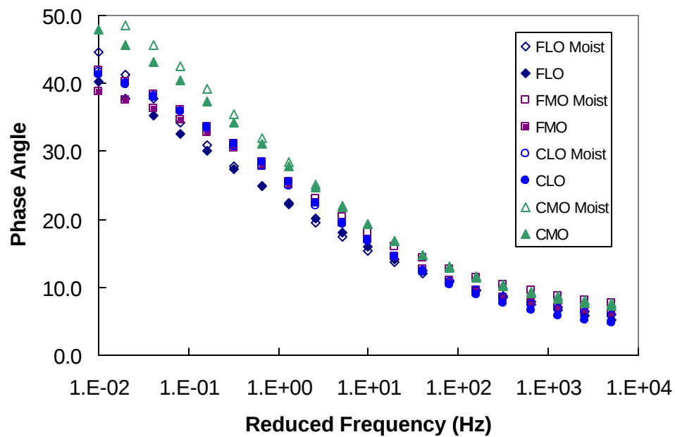
Figure 6.10 Effect of Moisture on Phase Angle
