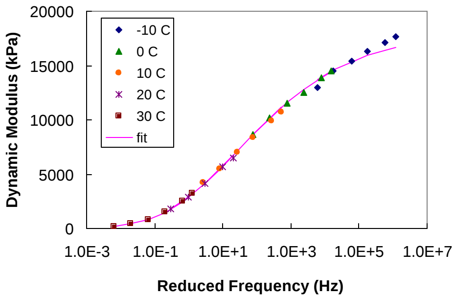
Figure A.4 Master Dynamic Modulus Curve at Reference Temperature of 20°C
