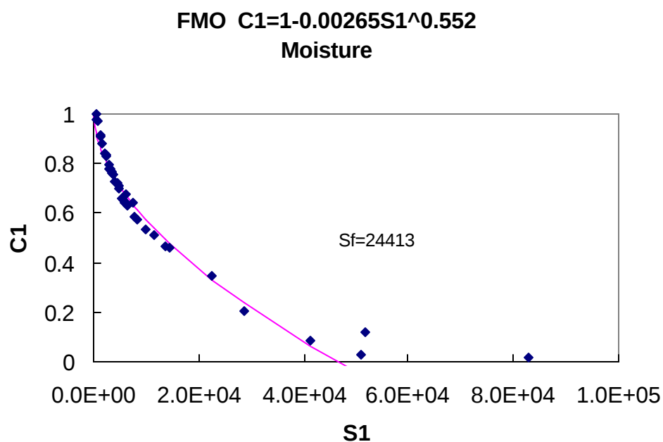
Figure D.13 Characteristic Curve for Moisture Cyclic FMO Data
