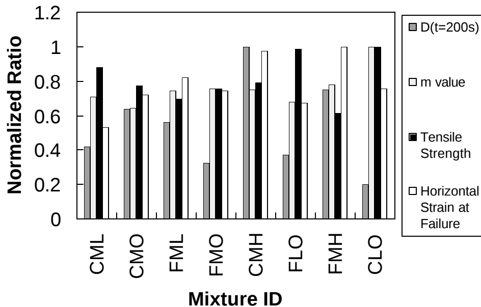
Figure 8.5 Evaluation of Four Engineering Parameters As Performance Indicators Using LMLC Specimens
