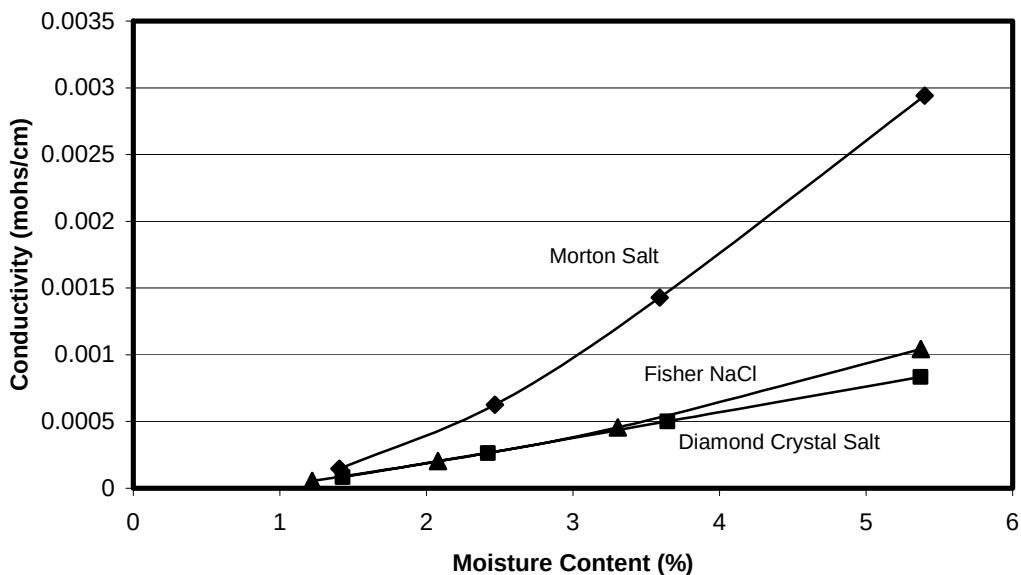
Figure 5.15 Conductivity vs Moisture Content Morton and Diamond Crystal Tables Salts and Fisher Reagent NaCl
